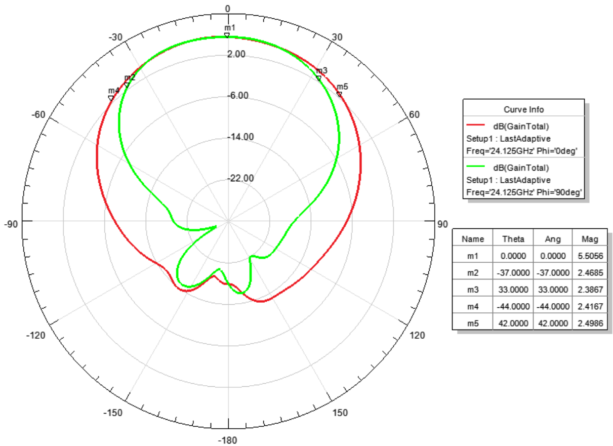
Gain Plot 3
