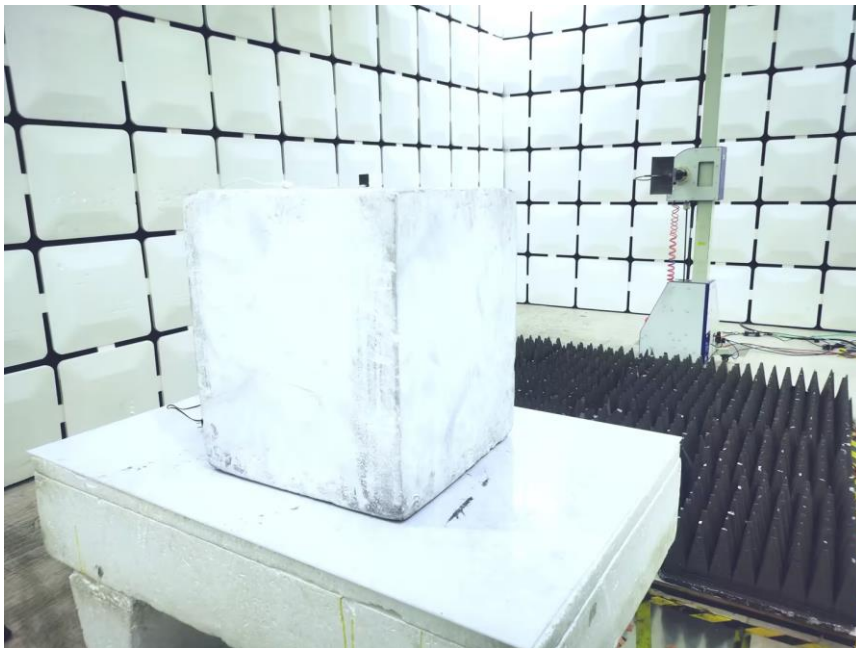
RF Radiated Test (1-18GHz)
