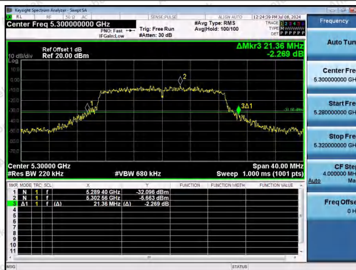
11AC20SISO-Ant1-5300
