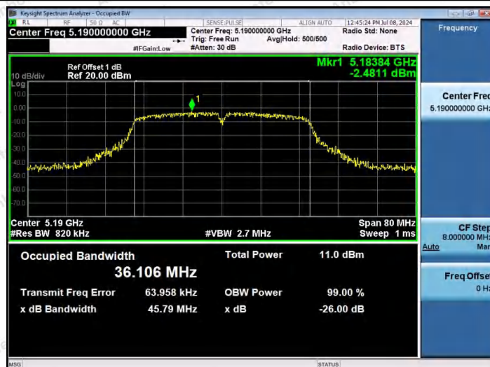
11AC40SISO-Ant1-5190
