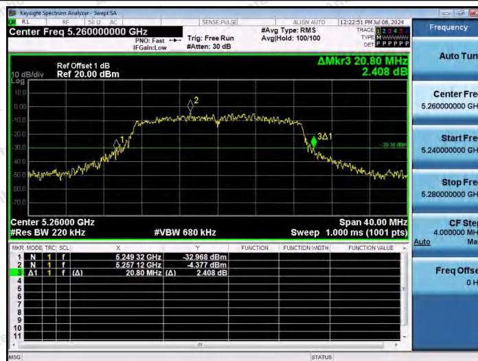
11AC20SISO-Ant1-5260
