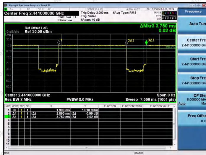
NTNV-2DH5-Ant1-2441
