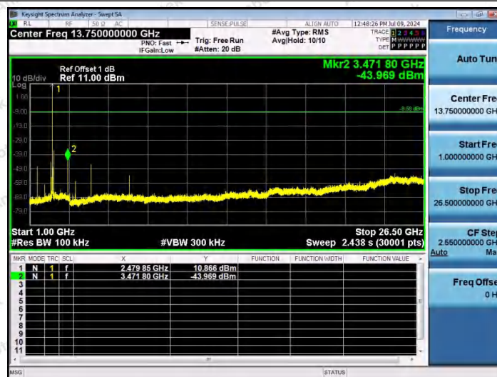
DH5-Ant1-2480-1000~26500-PASS
