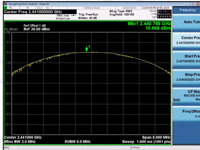
3DH5-Ant1-2441-PASS
