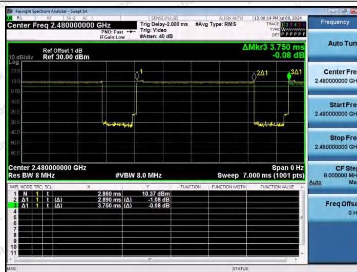
NTNV-3DH5-Ant1-2480
