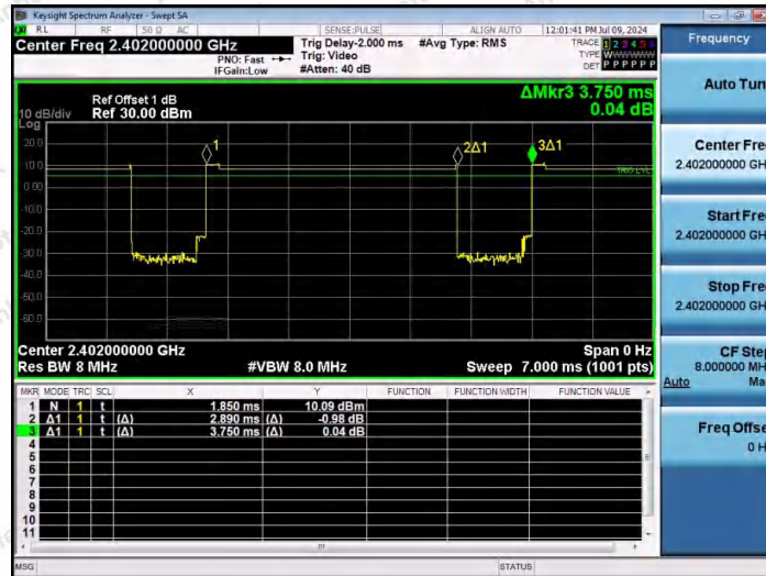
NTNV-3DH5-Ant1-2402
