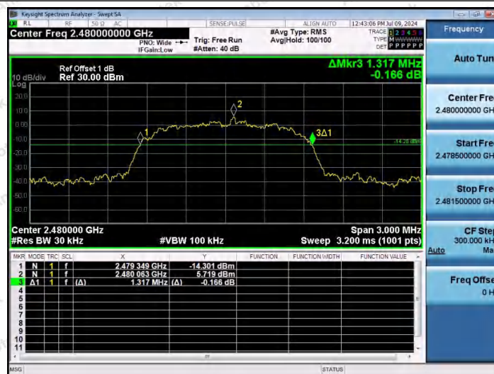
3DH5-Ant1-2480
