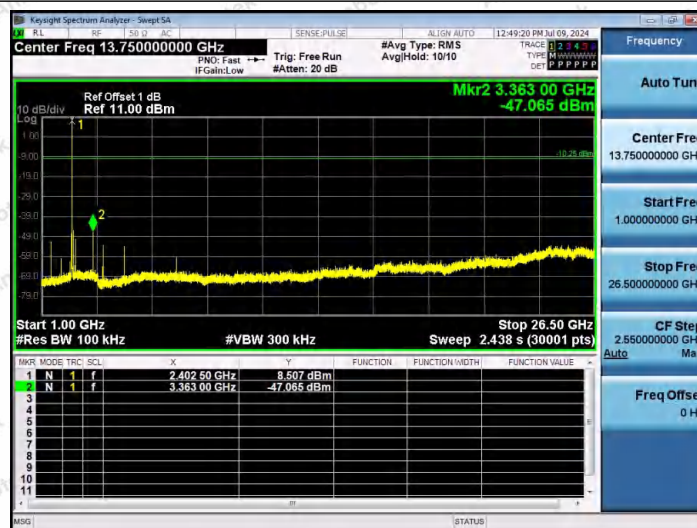
2DH5-Ant1-2402-1000~26500-PASS
