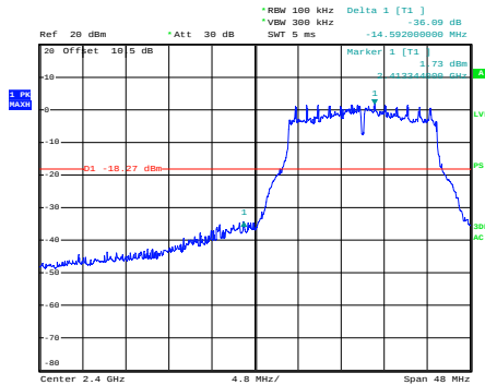
g_2412MHz
