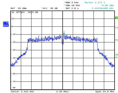
g_2412MHz
