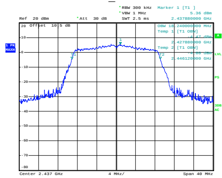
n20_2437MHz
