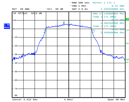
g_2412MHz
