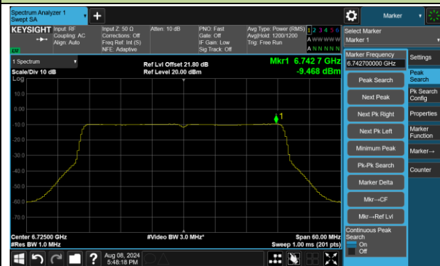
Channel 155 (6725MHz)
