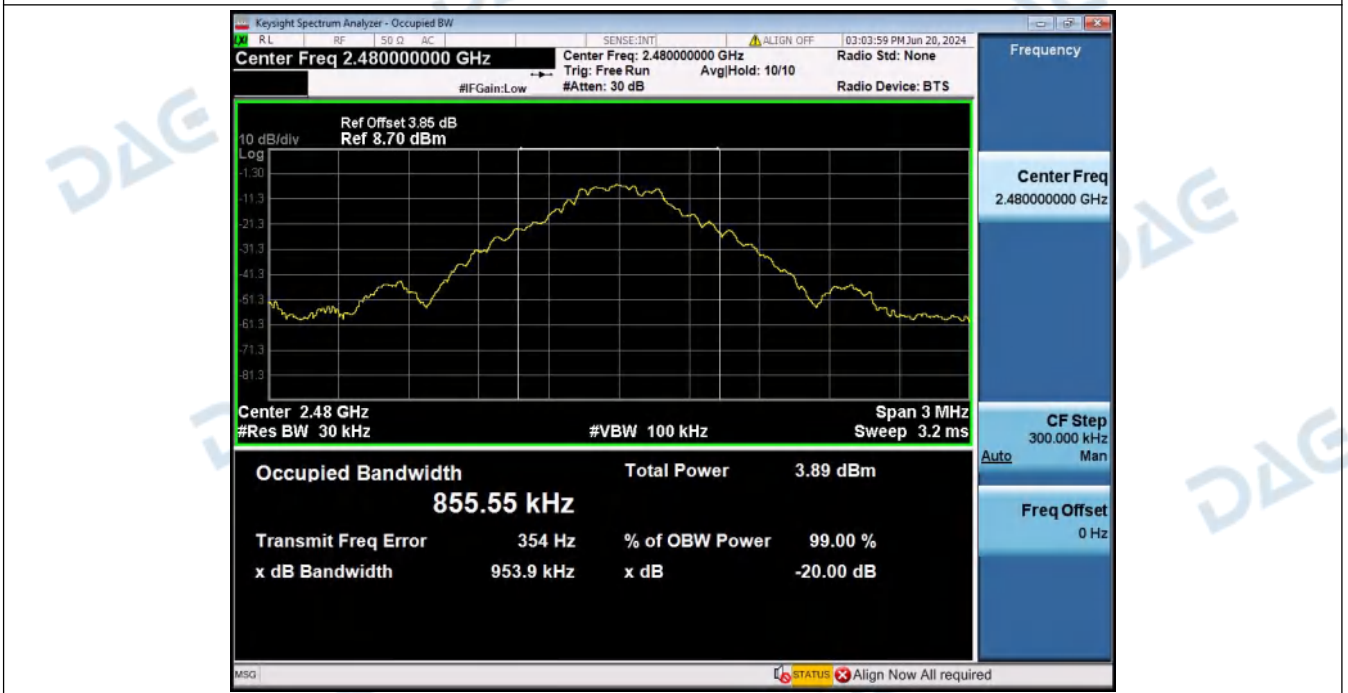
-20dB_Bandwidth_NVNT_ANT1_1-DH5_2480_00
