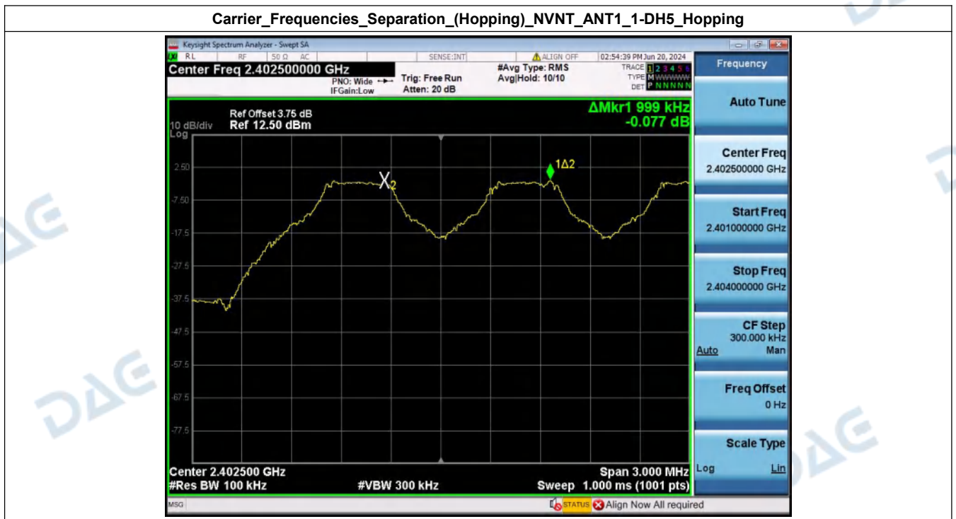
Carrier_Frequencies_Separation_(Hopping)_NVNT_ANT1_1-DH5_Hopping
