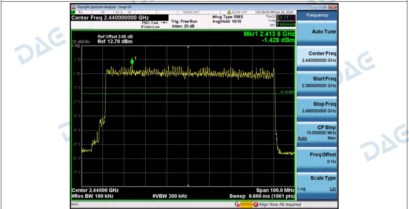
2_Band_Edge_(Hopping)_NVNT_ANT1_2-DH5_Hopping
