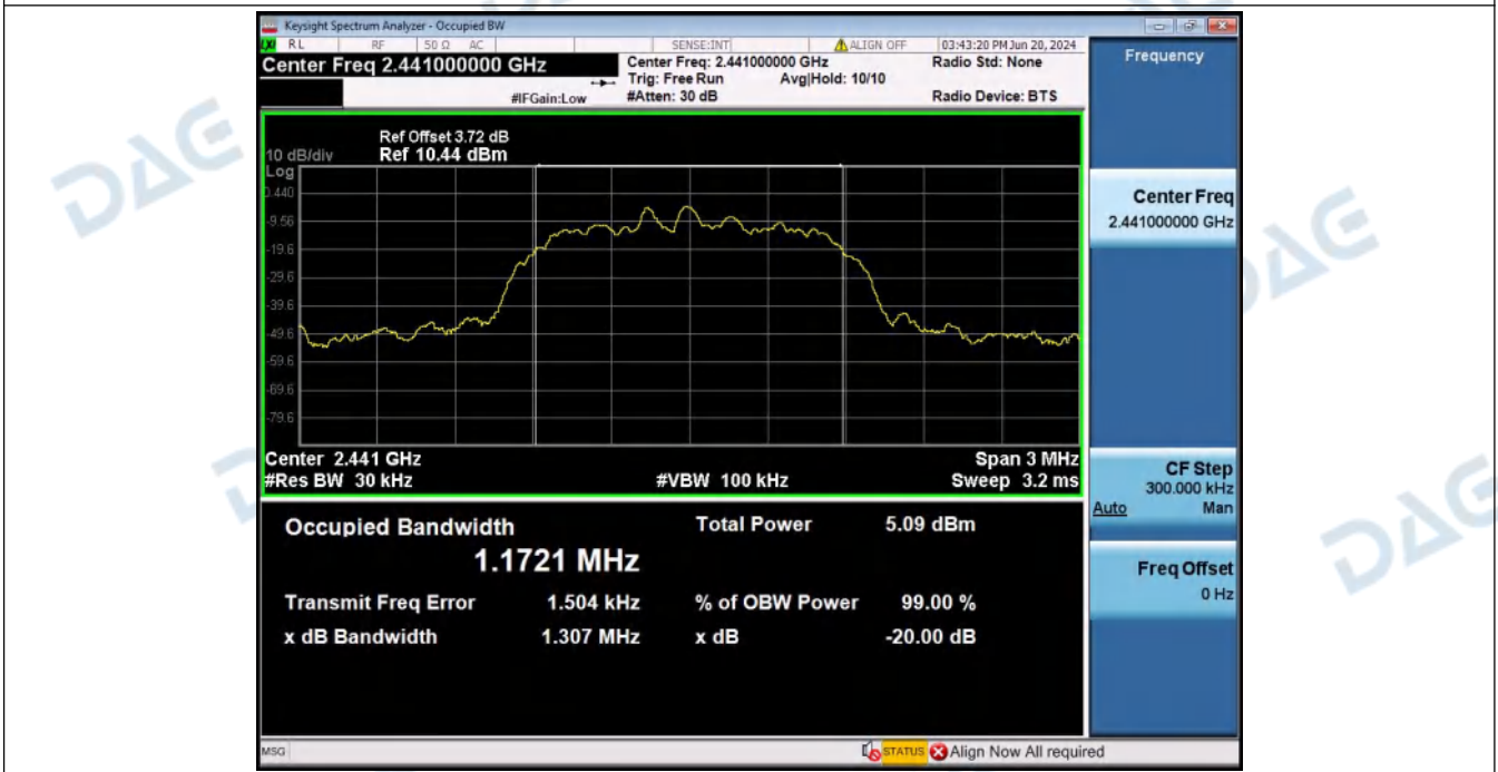
-20dB_Bandwidth_NVNT_ANT1_2-DH5_2441_00
