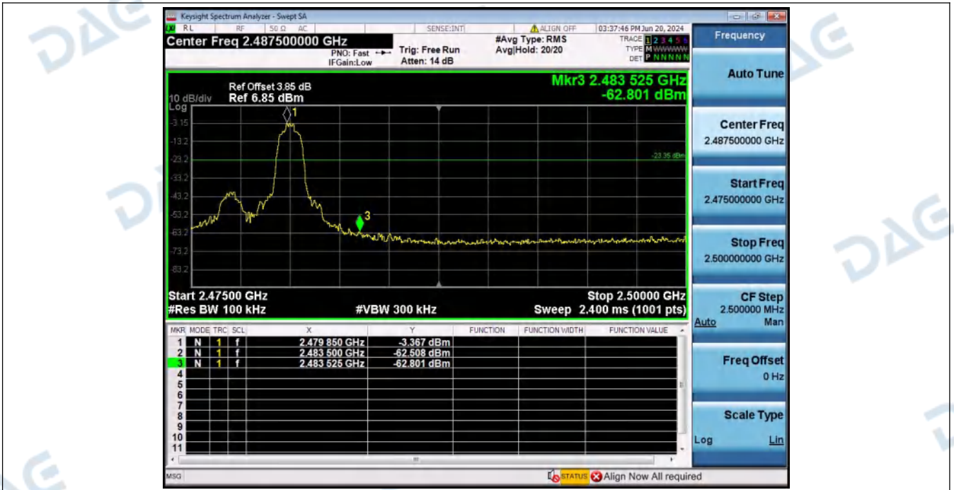
1_Reference_Level_Hopping_NVNT_ANT1_2-DH5_Hopping
