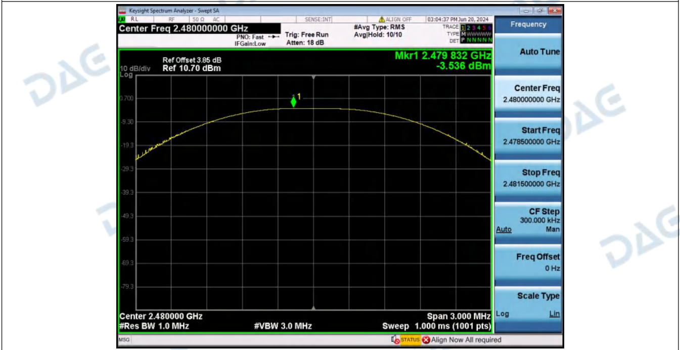
Peak_Output_Power_NVNT_ANT1_1-DH5_2480_00
