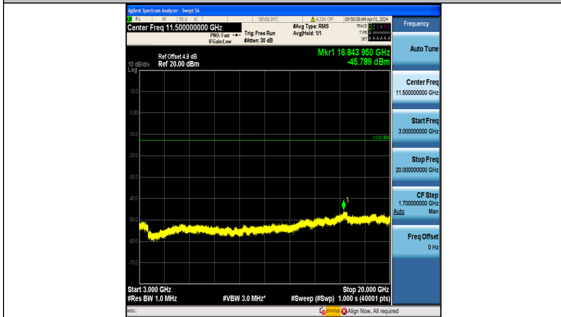
Band2_5MHz_QPSK_18625_25RB#0_3000~20000_3000~20000
