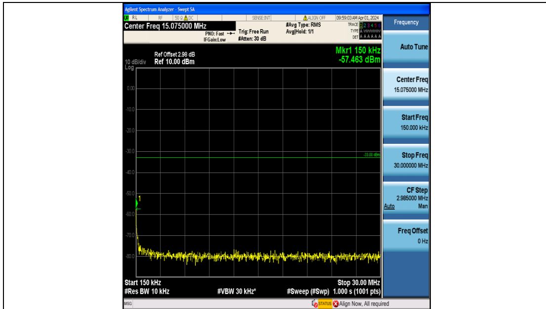
Band2_5MHz_QPSK_18900_25RB#0_0.15~30_0.15~30
