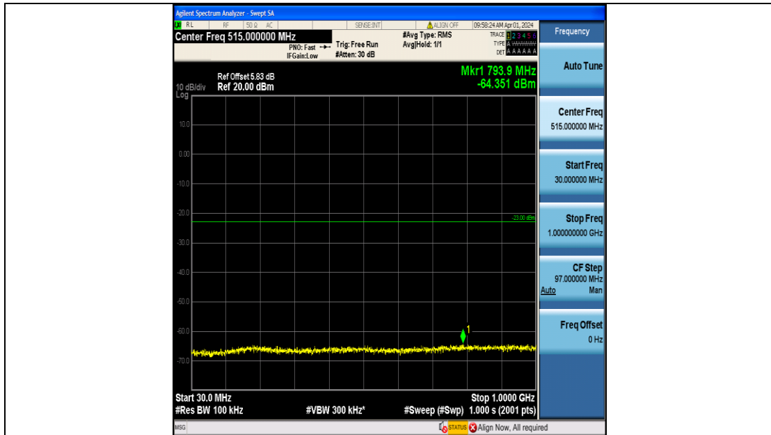
Band2_5MHz_16QAM_18625_25RB#0_30~1000_30~1000
