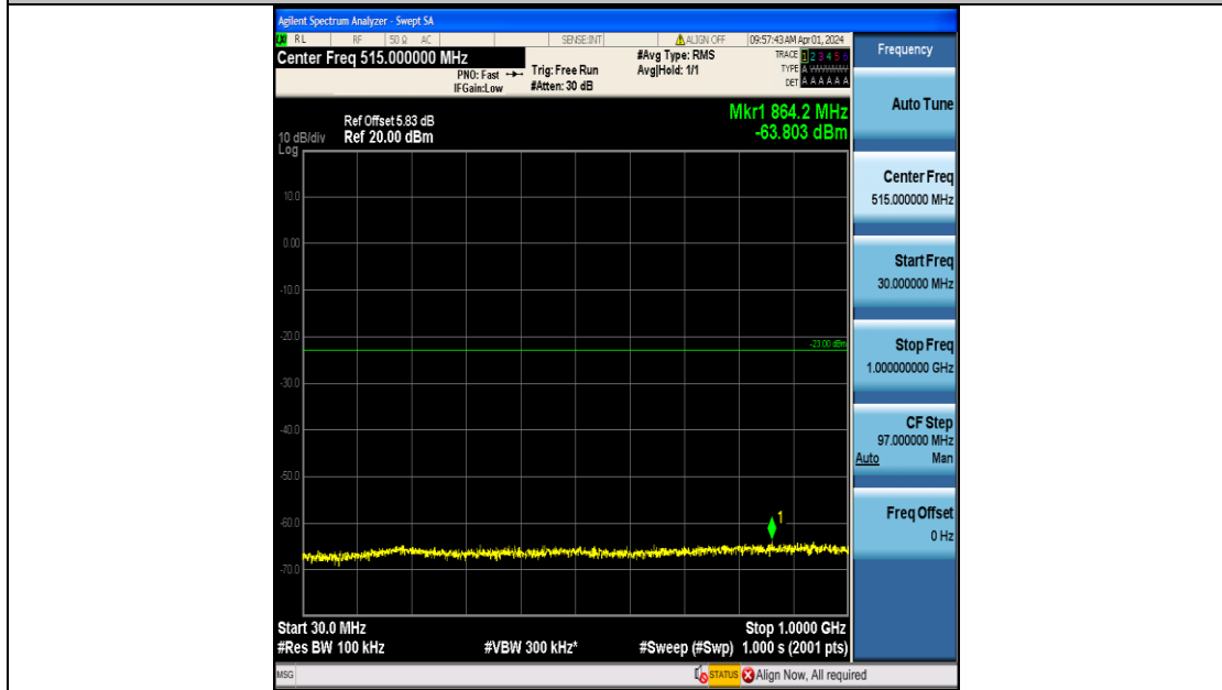
Band2_5MHz_QPSK_18625_25RB#0_30~1000_30~1000
