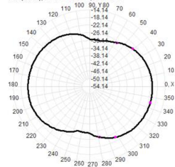
Total(H-XY), Max=-21.12dBi, CirD=9.03
