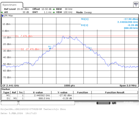
GFSK_Mid_DH1
