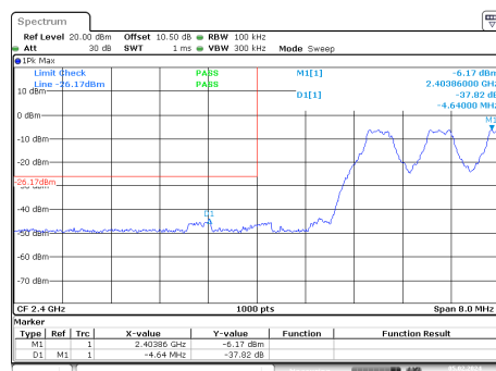
GFSK_Hopping_Lower_DH1
