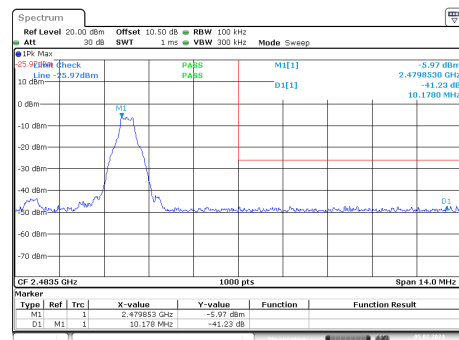
GFSK_High_DH1
