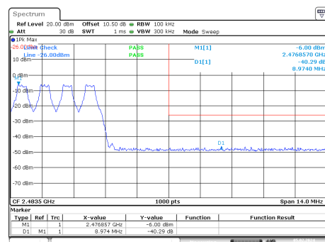
GFSK_Hopping_Upper_DH1
