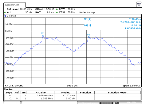
GFSK_High_DH1
