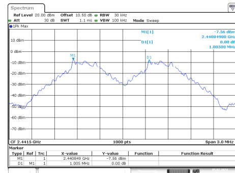
GFSK_Mid_DH1
