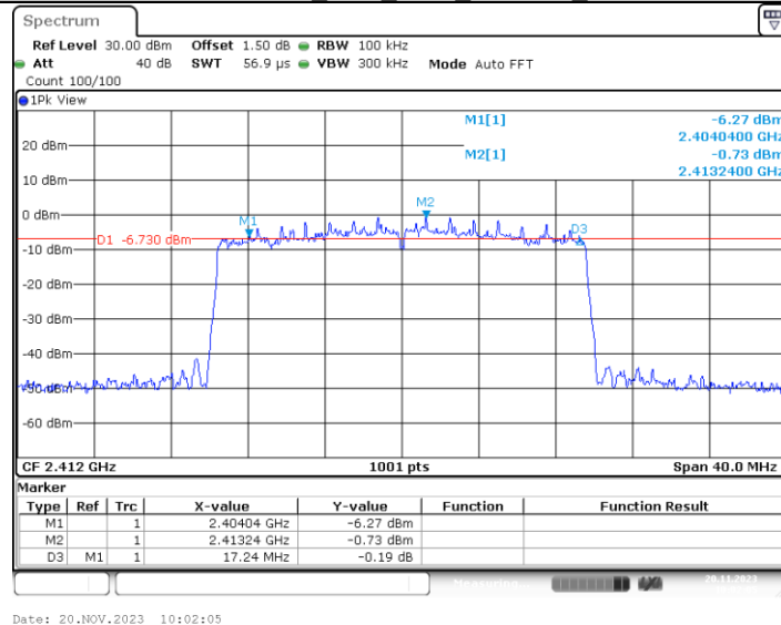
11AX20MIMO Ant2 2412 242Tone RU61
