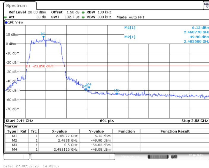
11G_Ant2_High_2462
