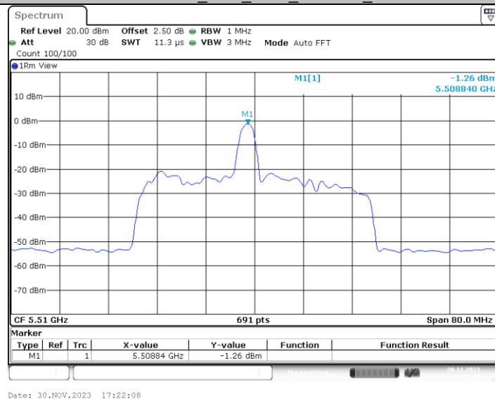
11AX40MIMO Ant2 5510 26Tone RU8
