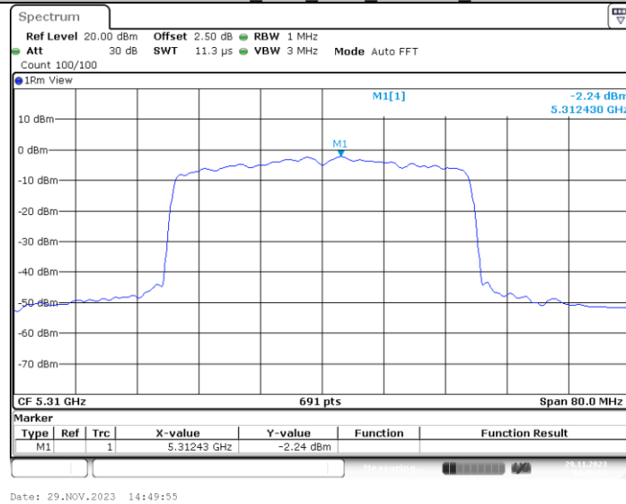
11AX40MIMO Ant2 5310 484Tone RU65
