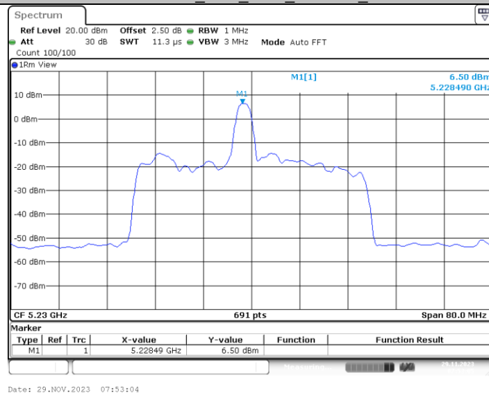
11AX40MIMO Ant2 5230 26Tone RU8
