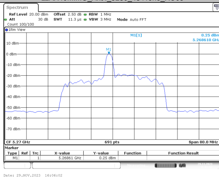
11AX40MIMO Ant1 5270 26Tone RU8
