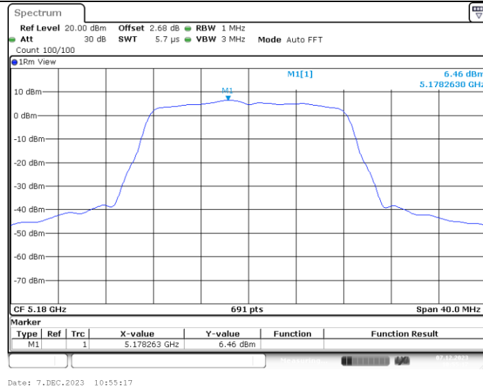
11A_Ant4_5180
