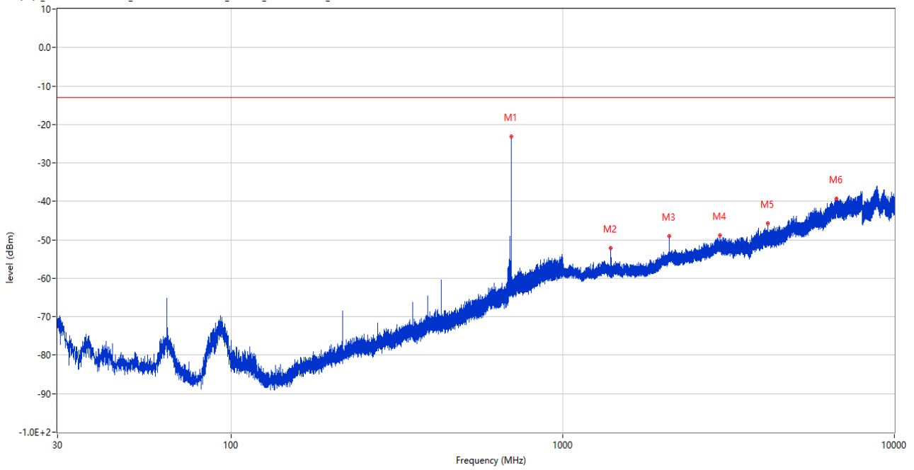
RSE (RF) _FCC PART22&24&27_LTE B12 & B17 & B28 _699-748_30MHz-10GHz_
