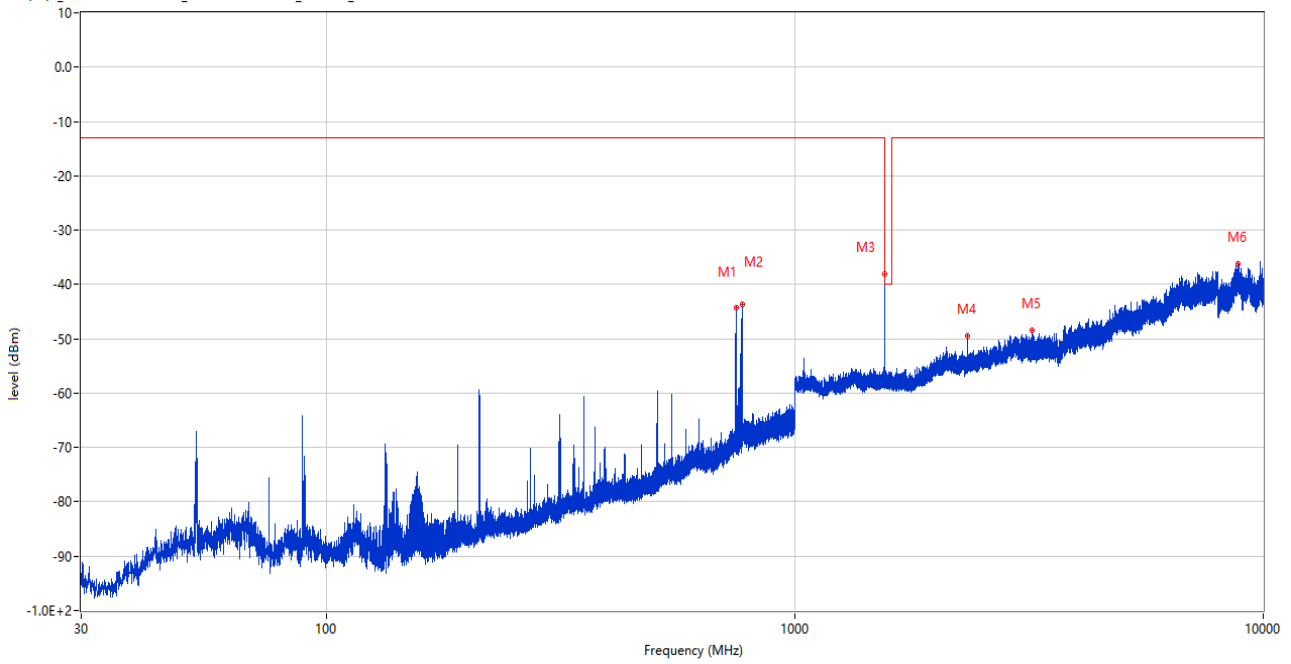
RSE (RF) _FCC PART22&24&27_LTE Band 13 & 14 _777-803_30MHz-10GHz
