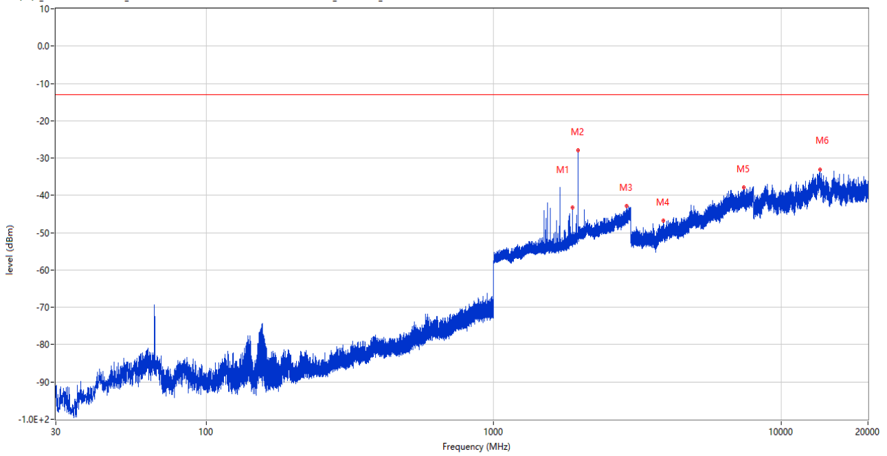
RSE (RF) _FCC PART22&24&27_CDMA BC1 & WCDMA Band 2 & LTE Band 2 & 25 _1830-1920_30MHz-20GHz
