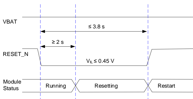
Figure 14: Reset Timing
