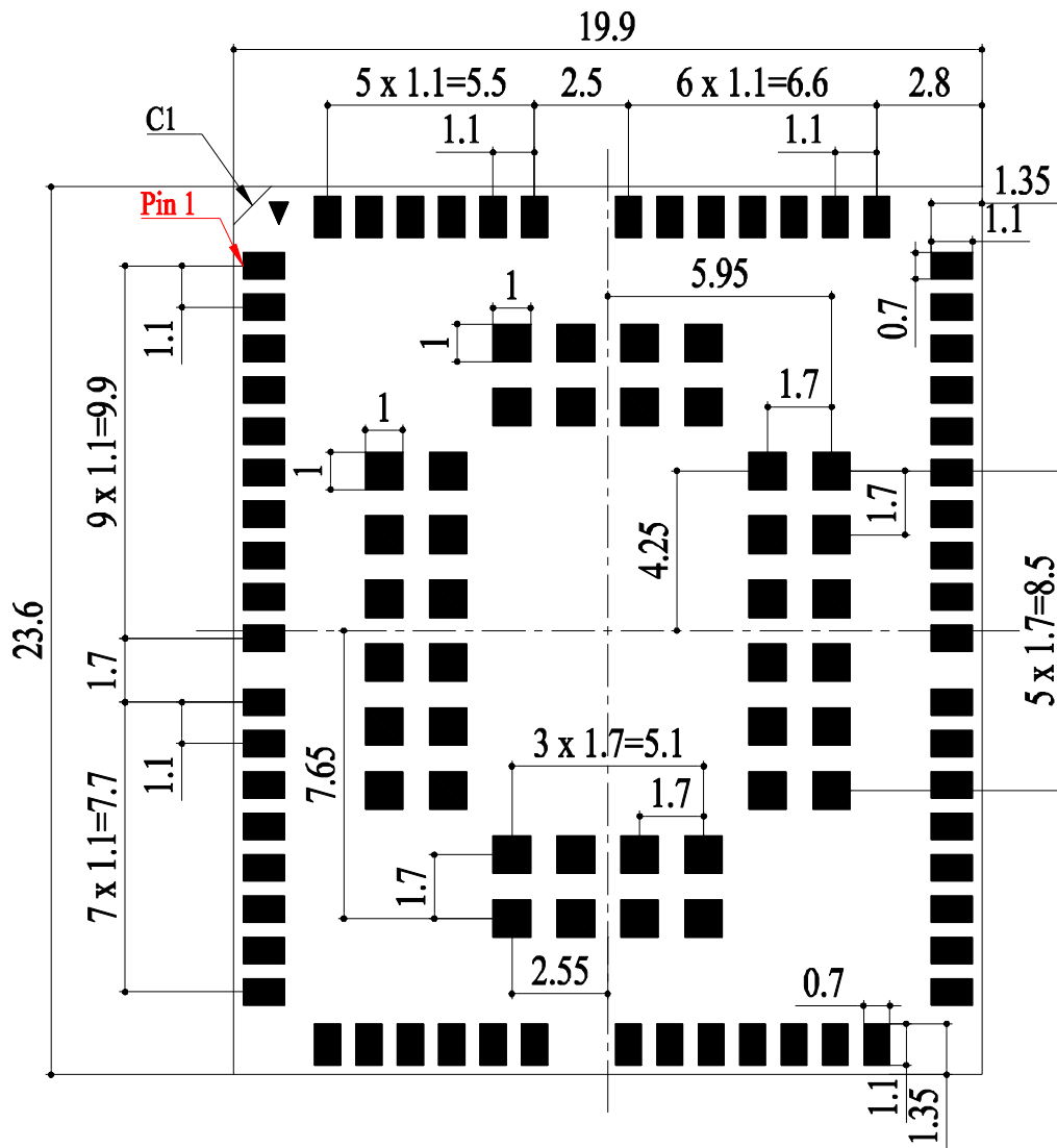
Figure 38: Recommended Footprint
