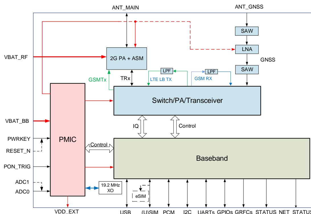
Figure 2: Functional Diagram of PCUL11-LD
