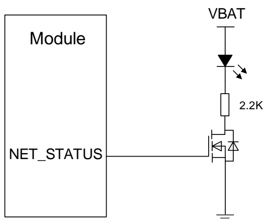
Figure 23: Reference Design of the Network Status Indicator
