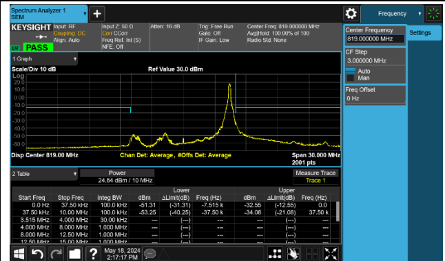
Middle Channel_1RB_High
