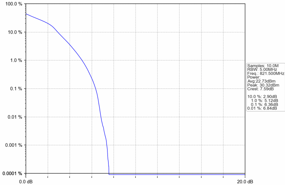
Band26a_5MHz_16QAM_HCH_821.5MHz_RB_25_0_NTNV
