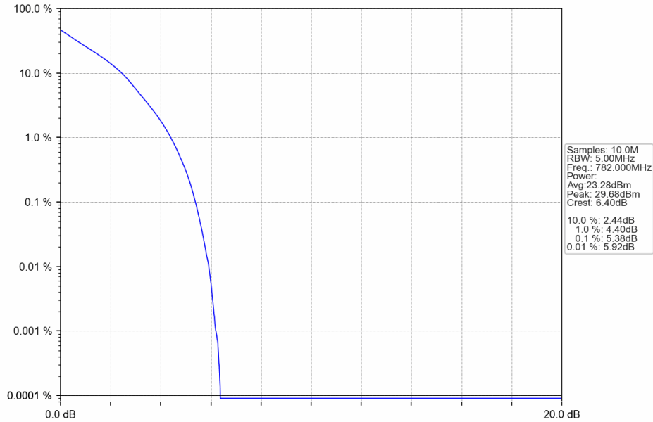
Band13_5MHz_QPSK_MCH_782MHz_RB_25_0_NTNV
