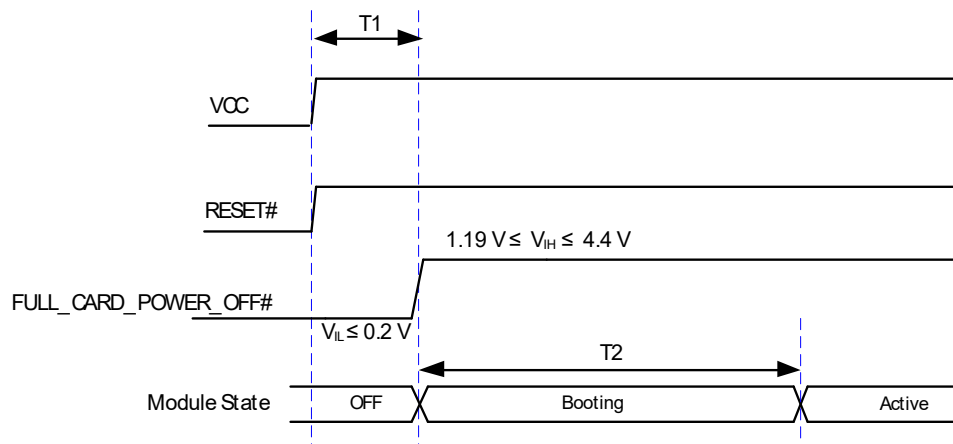
Figure 9: Turn-on Timing
