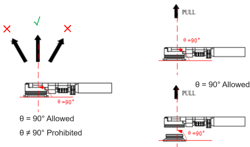
Figure 27: Pull out a Coaxial Cable Plug
