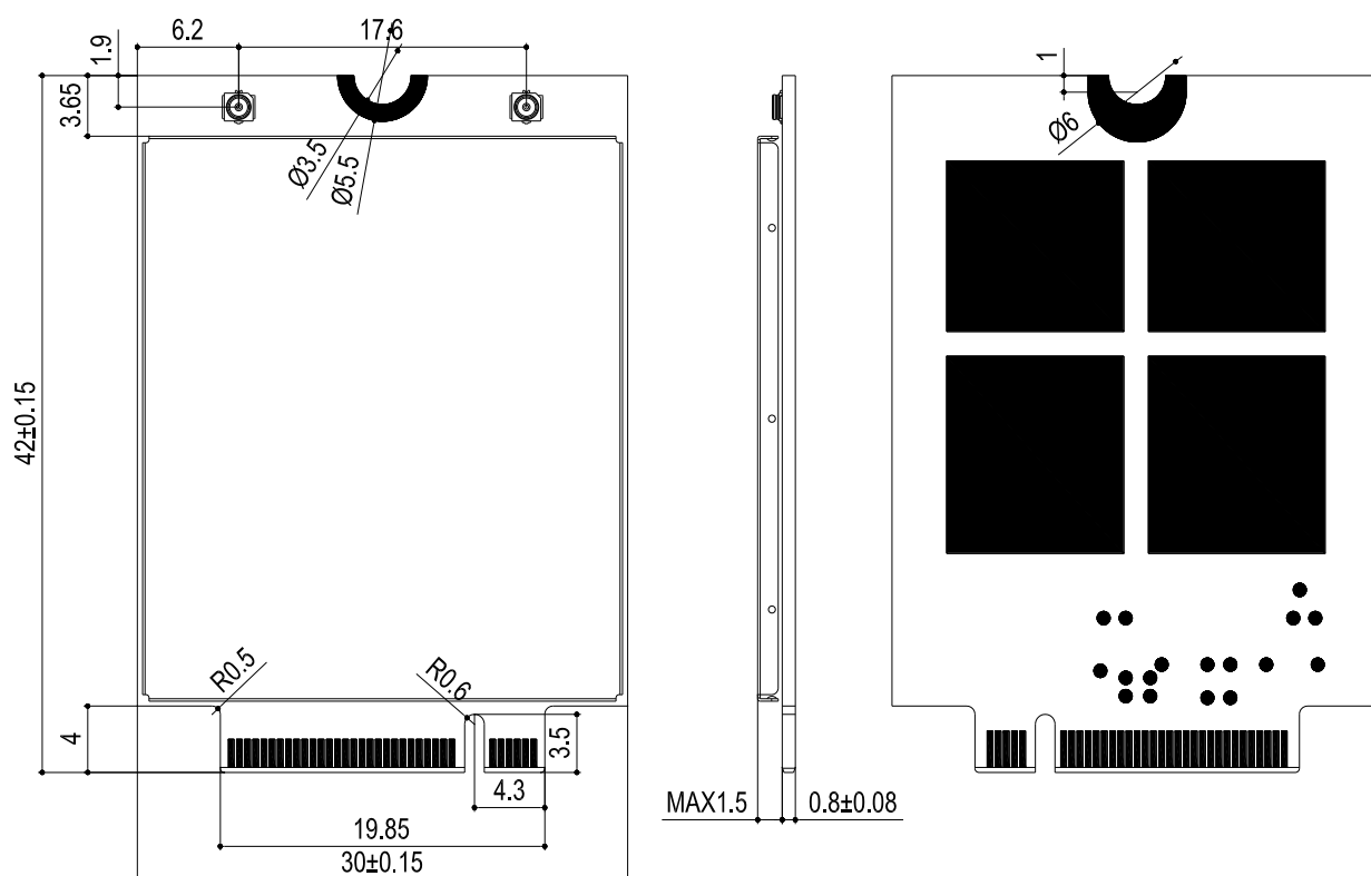
Figure 32: Mechanical Dimensions (Unit: mm)
