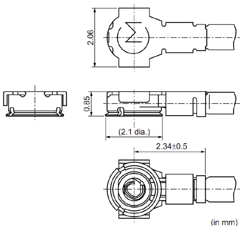
Figure 23: Dimensions of Mated Plugs (Ø0.81/Ø1.13 mm Coaxial Cables)
