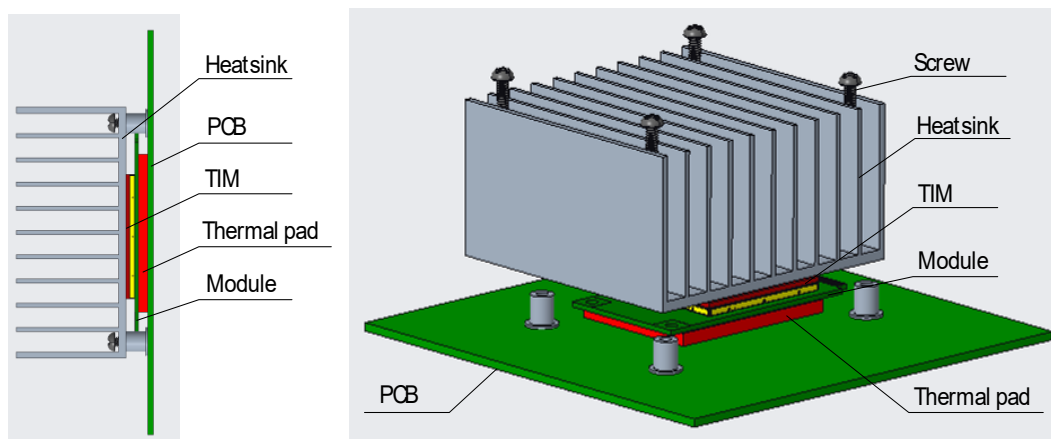
Figure 30: Placement and Fixing of the Heatsink
