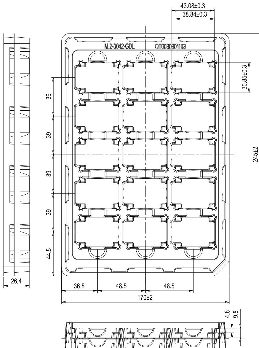
Figure 34: Blister Tray Dimension Drawing (Unit: mm)
