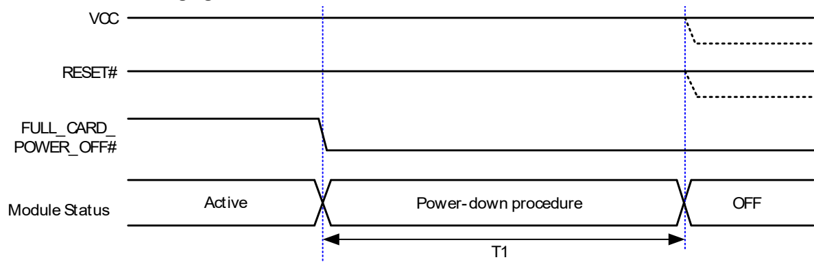
Figure 10: Turn-off Timing
