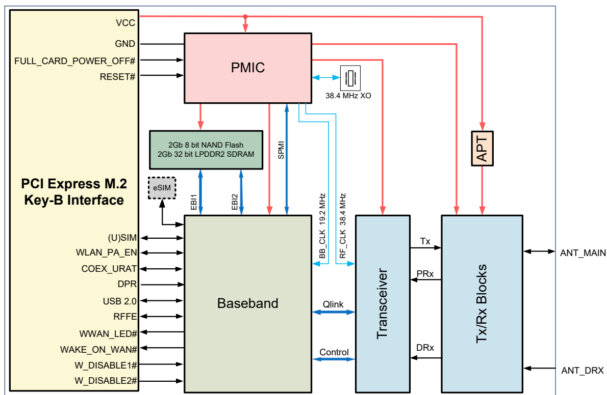
Figure 1: Functional Diagram
