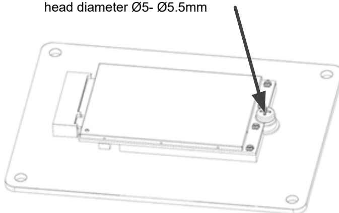
Figure 31: Installation Schematic
