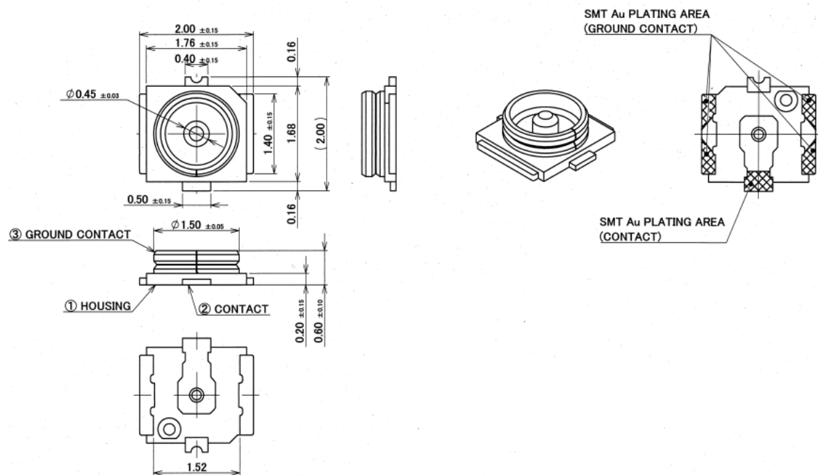
Figure 22: Dimensions of the Receptacle (Unit: mm)
