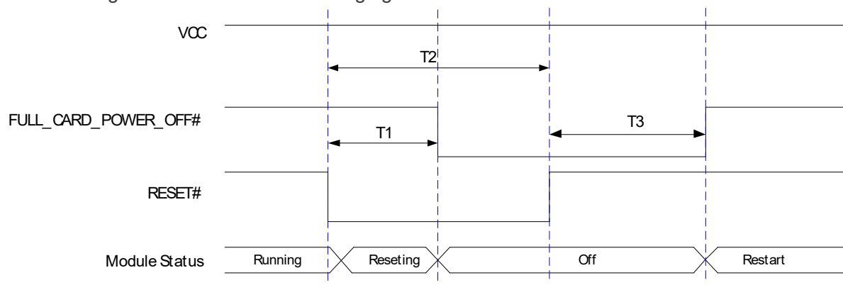
Figure 12: Reset Timing
