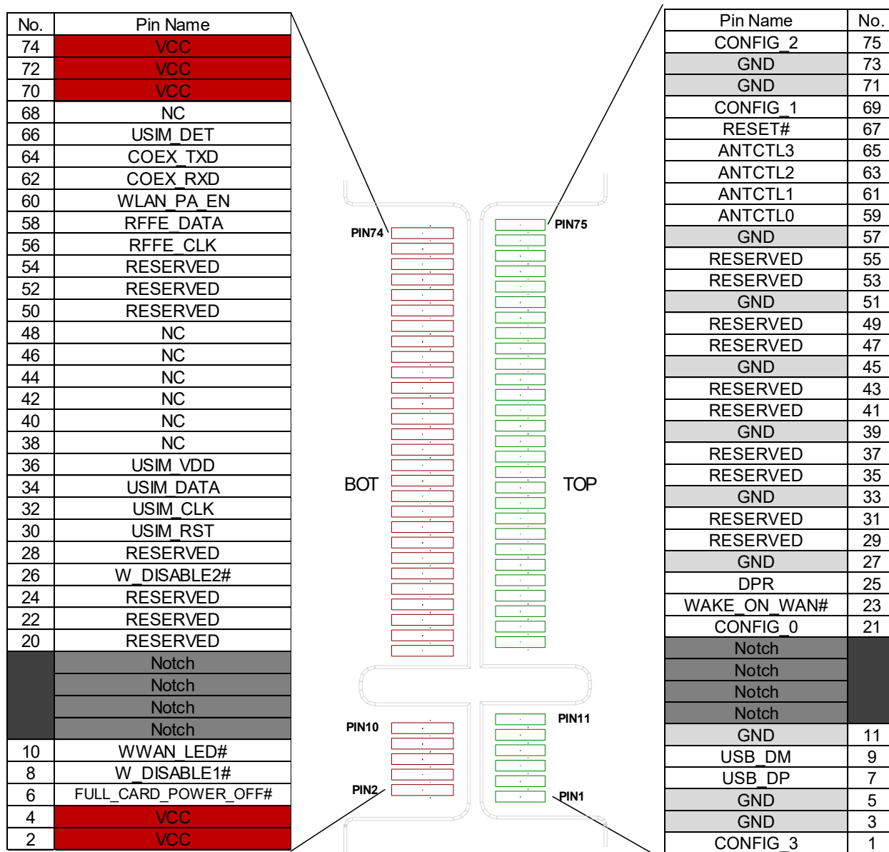
Figure 2: Pin Assignment
