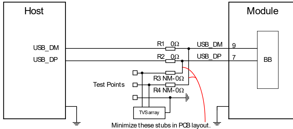
Figure 15: Reference Circuit for USB Interface
