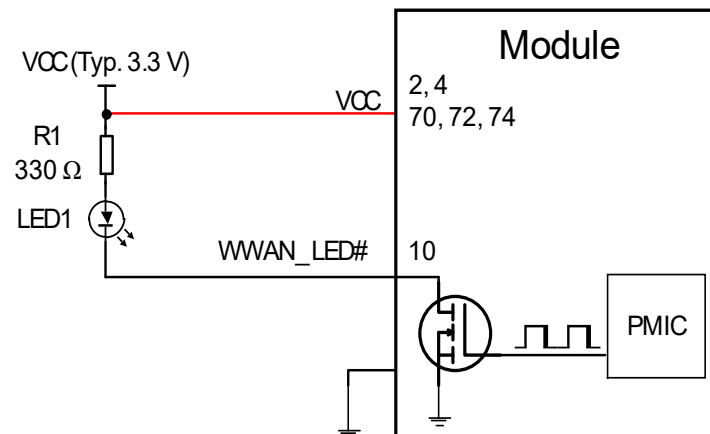
Figure 17: WWAN_LED# Reference Circuit
