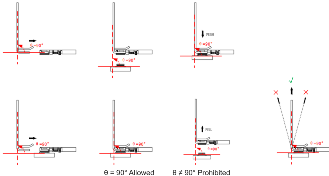
Figure 28: Install the Coaxial Cable Plug with Jig
