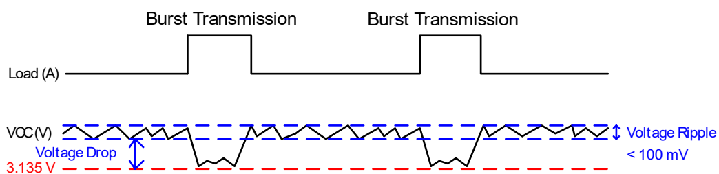
Figure 6: Power Supply Limits During Burst Transmission
