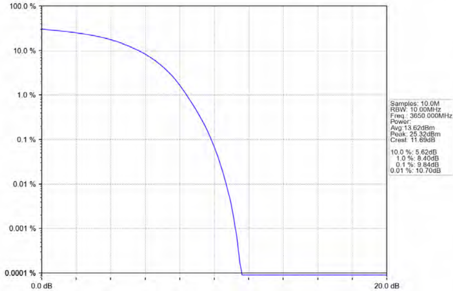
Band43 15MHz 16QAM MCH 3650MHz RB 75_0 NTN
