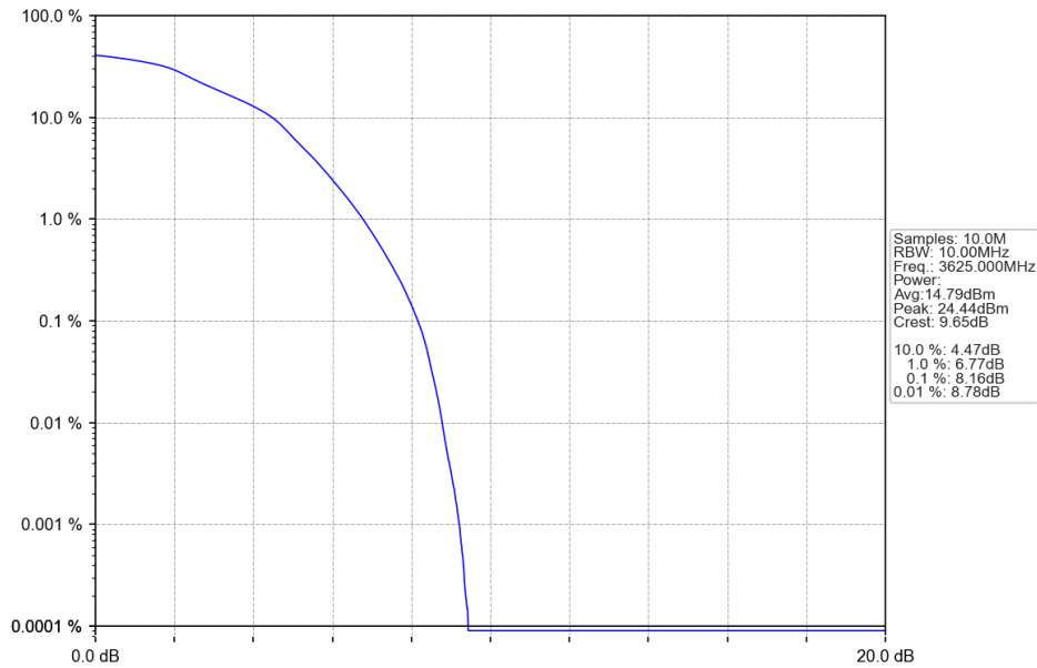
Band48 10MHz 16QAM MCH 3625MHz RB 50 0 NTN
