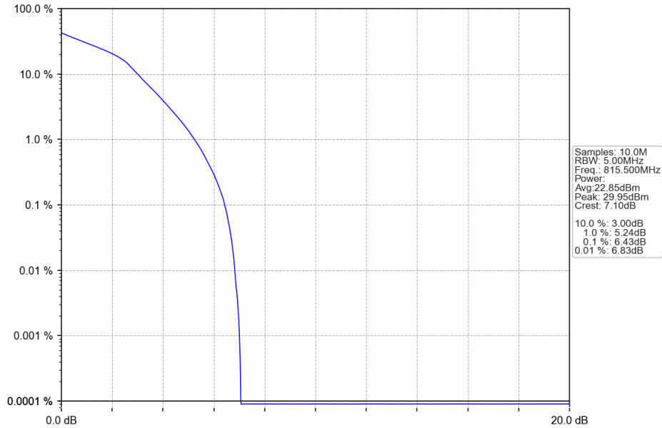
Band26a_3MHz_16QAM_LCH_815.5MHz_RB_15_0_NTNV
