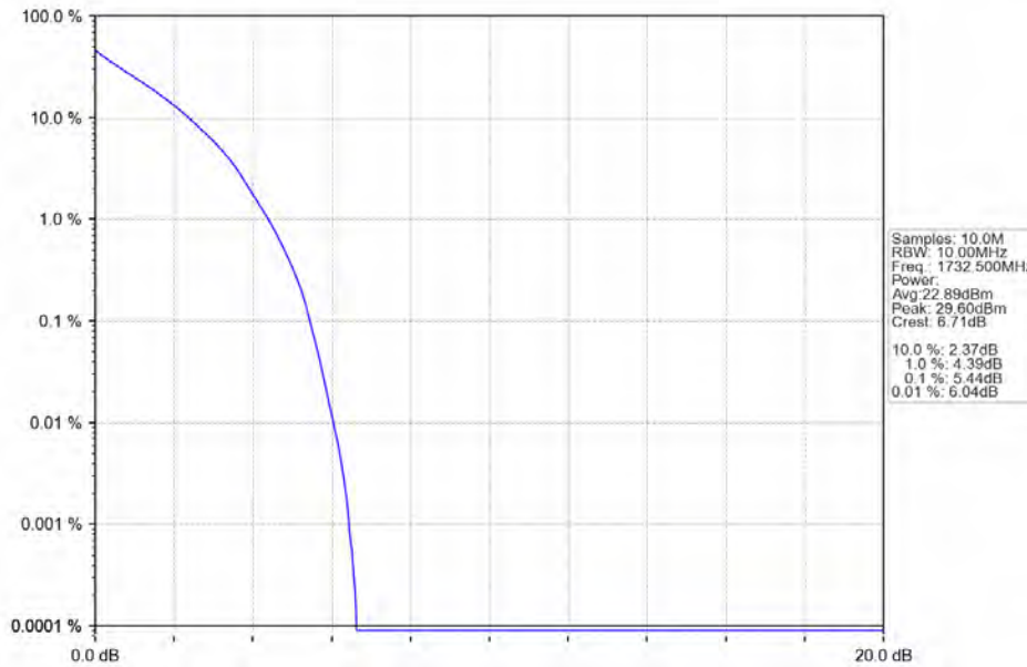
Band4_10MHz_QPSK_MCH_1732.5MHz_RB_50_0_NTNV
