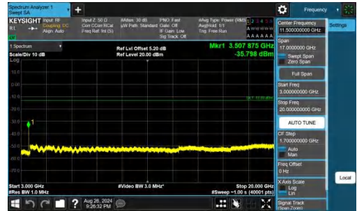
Band66-20MHz-QPSK-132322-1RB#99-3000~20000-PASS
