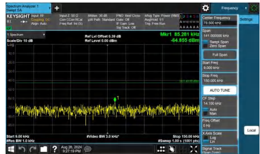
Band66-20MHz-QPSK-132572-1RB#99-0.009~0.15-PASS
