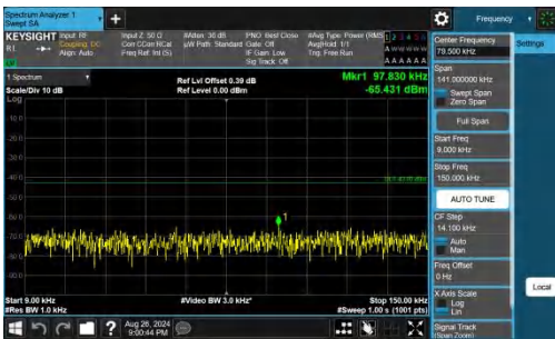
Band66-5MHz-QPSK-131997-1RB#0-0.009~0.15-PASS
