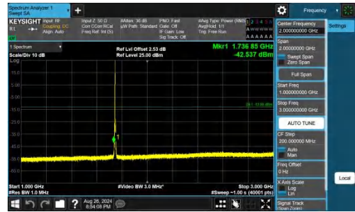
Band66-3MHz-QPSK-132322-1RB#0-1000~3000-PASS
