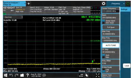
Band66-20MHz-QPSK-132572-1RB#99-30~1000-PASS
