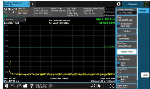
Band66-15MHz-QPSK-132047-1RB#0-0.15~30-PASS
