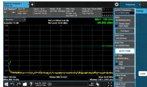
Band66-5MHz-QPSK-132322-1RB#0-0.15~30-PASS
