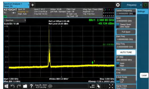
Band66-20MHz-QPSK-132572-1RB#0-1000~3000-PASS
