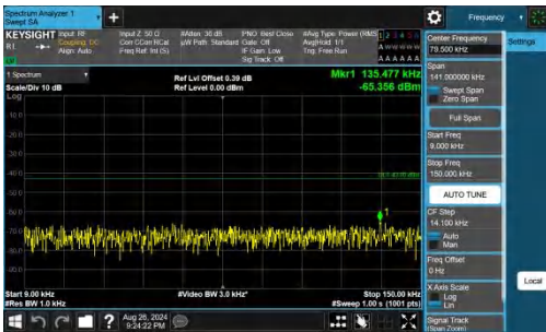
Band66-20MHz-QPSK-132072-1RB#0-0.009~0.15-PASS
