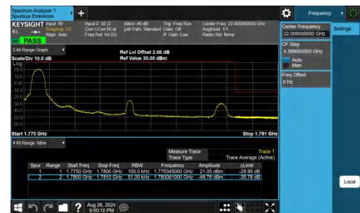
Band66-5MHz-QPSK-132647-1RB#0-PASS
