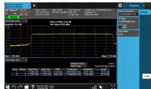
Band66-5MHz-QPSK-132657-1RB#14-PASS
