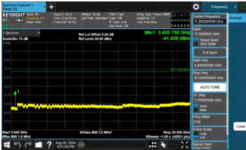
Band66-5MHz-QPSK-131997-1RB#0-3000~20000-PASS
