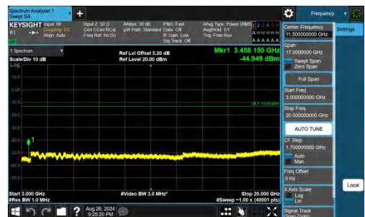
Band66-20MHz-QPSK-132072-1RB#99-3000~20000-PASS
