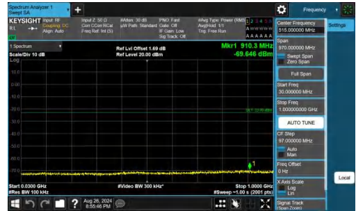
Band66-3MHz-QPSK-132657-1RB#14-30~1000-PASS
