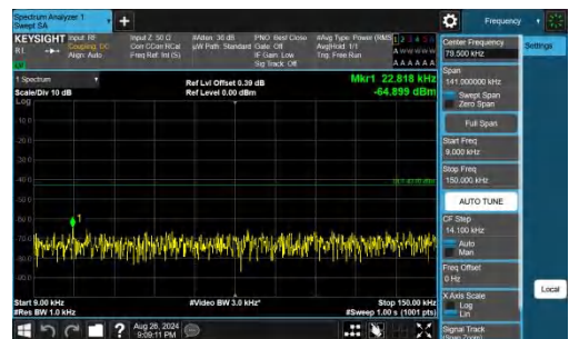
Band66-10MHz-QPSK-132022-1RB#49-0.009~0.15-PASS
