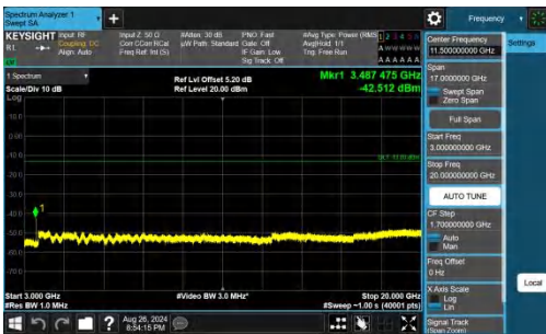
Band66-3MHz-QPSK-132322-1RB#0-3000~20000-PASS
