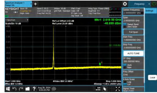
Band66-5MHz-QPSK-132647-1RB#0-1000~3000-PASS
