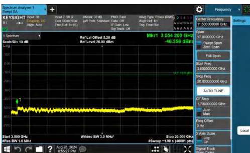
Band66-3MHz-QPSK-132657-1RB#0-3000~20000-PASS
