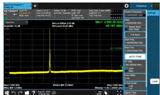
Band66-10MHz-QPSK-132022-1RB#0-1000~3000-PASS
