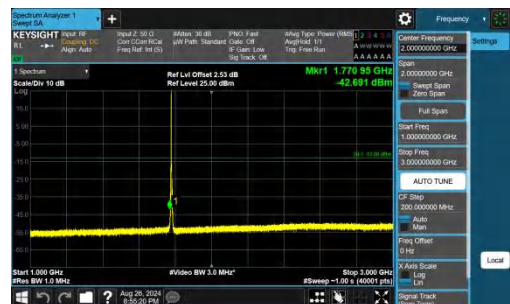
Band66-3MHz-QPSK-132657-1RB#0-1000~3000-PASS
