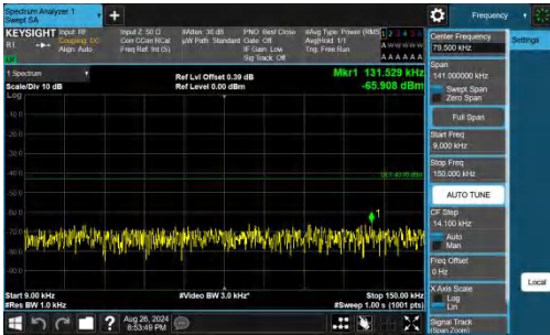
Band66-3MHz-QPSK-132322-1RB#0-0.009~0.15-PASS
