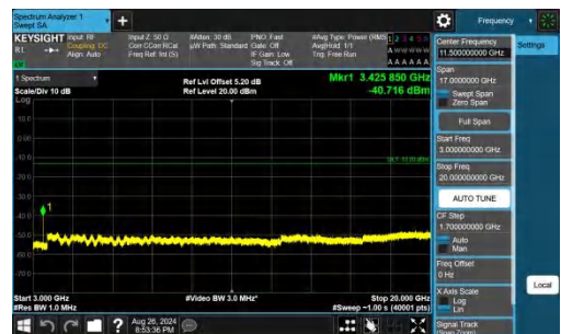
Band66-3MHz-QPSK-131987-1RB#14-3000~20000-PASS
