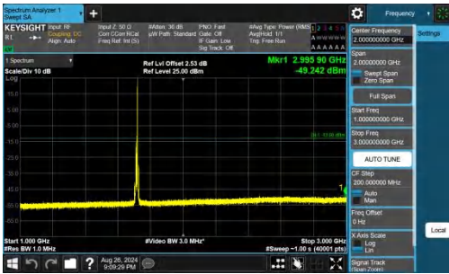
Band66-10MHz-QPSK-132022-1RB#49-1000~3000-PASS
