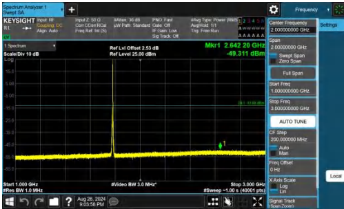
Band66-5MHz-QPSK-132647-1RB#24-1000~3000-PASS
