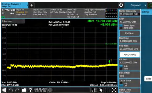
Band66-5MHz-QPSK-132647-1RB#0-3000~20000-PASS
