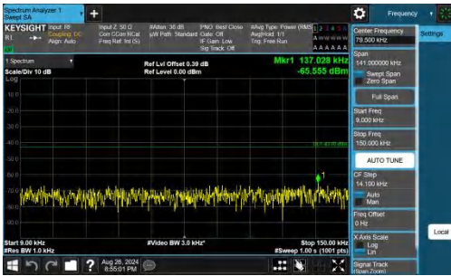
Band66-3MHz-QPSK-132657-1RB#0-0.009~0.15-PASS
