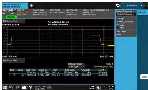
Band66-10MHz-QPSK-132622-50RB#0-PASS
