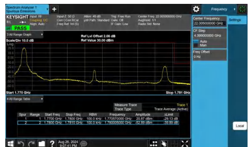
Band66-10MHz-QPSK-132622-1RB#0-PASS
