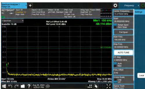
Band66-20MHz-QPSK-132072-1RB#99-0.15~30-PASS
