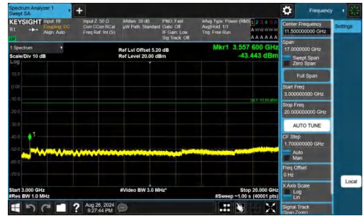
Band66-20MHz-QPSK-132572-1RB#99-3000~20000-PASS
