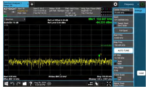
Band66-20MHz-QPSK-132072-1RB#99-0.009~0.15-PASS
