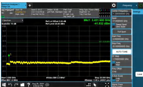
Band66-10MHz-QPSK-132022-1RB#0-3000~20000-PASS
