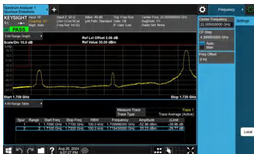
Band66-10MHz-QPSK-132022-1RB#49-PASS
