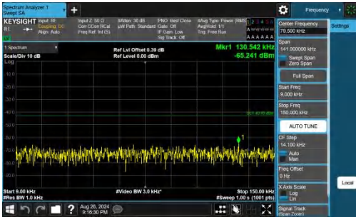
Band66-15MHz-QPSK-132047-1RB#0-0.009~0.15-PASS
