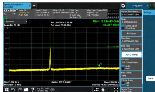
Band66-10MHz-QPSK-132322-1RB#0-1000~3000-PASS
