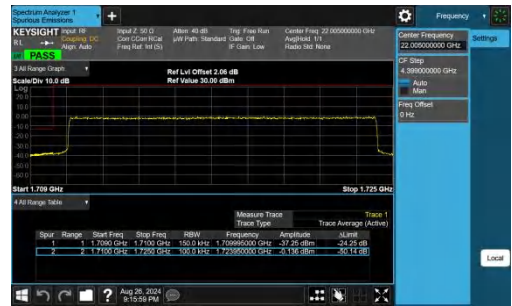
Band66-15MHz-QPSK-132047-75RB#0-PASS
