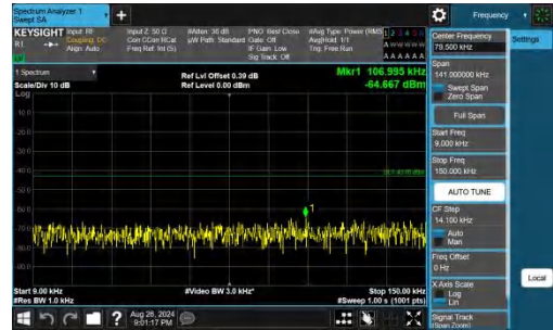
Band66-5MHz-QPSK-131997-1RB#24-0.009~0.15-PASS
