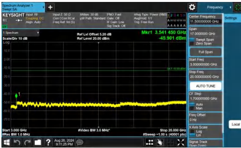
Band66-10MHz-QPSK-132622-1RB#0-3000~20000-PASS
