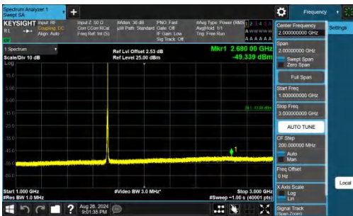
Band66-5MHz-QPSK-131997-1RB#24-1000~3000-PASS
