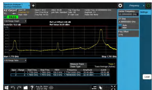
Band66-10MHz-QPSK-132622-1RB#49-PASS
