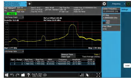
Band66-3MHz-QPSK-132657-1RB#14-PASS
