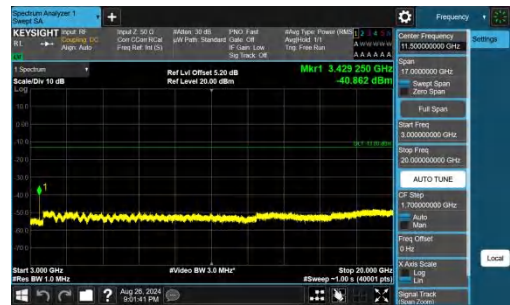
Band66-5MHz-QPSK-131997-1RB#24-3000~20000-PASS
