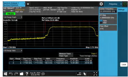
Band66-1.4MHz-QPSK-131979-6RB#0-PASS
