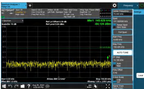
Band66-10MHz-QPSK-132322-1RB#0-0.009~0.15-PASS
