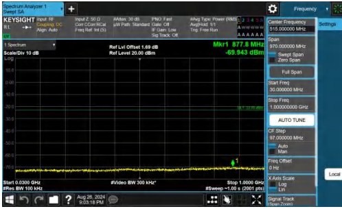
Band66-5MHz-QPSK-132647-1RB#0-30~1000-PASS
