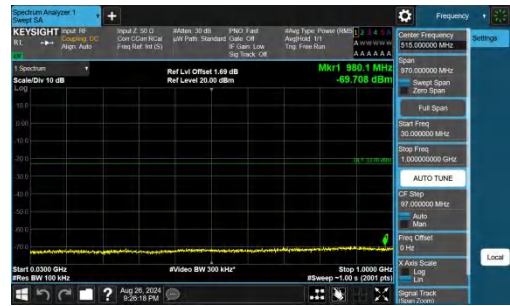
Band66-20MHz-QPSK-132322-1RB#99-30~1000-PASS
