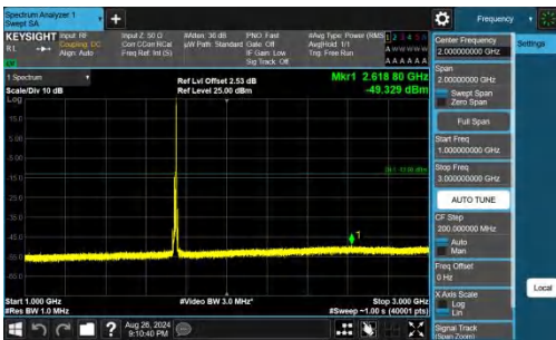
Band66-10MHz-QPSK-132322-1RB#49-1000~3000-PASS
