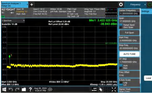
Band66-20MHz-QPSK-132072-1RB#0-3000~20000-PASS
