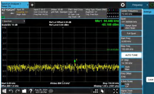
Band66-5MHz-QPSK-132322-1RB#0-0.009~0.15-PASS
