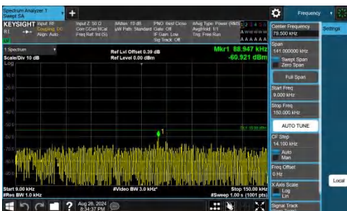
Band41-20MHz-QPSK-40620-1RB#0-0.009~0.15-PASS
