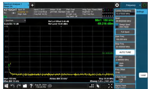
Band41-5MHz-QPSK-39675-1RB#0-0.15~30-PASS
