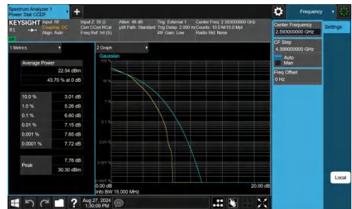
Band41-15MHz-16QAM-40620-27RB#0-PASS
