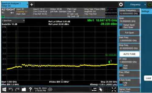
Band41-5MHz-QPSK-40620-1RB#24-1000~20000-PASS
