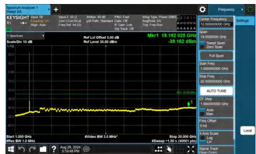
Band41-15MHz-QPSK-39725-1RB#0-1000~20000-PASS
