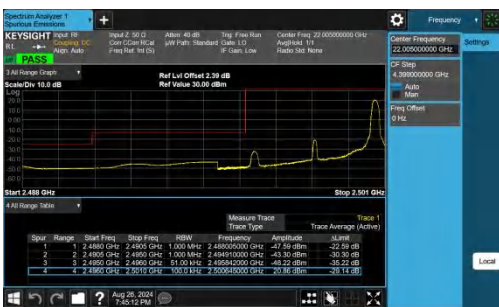
Band41-5MHz-QPSK-39675-1RB#24-PASS
