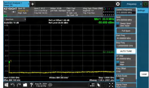
Band41-5MHz-QPSK-40620-1RB#24-30~1000-PASS
