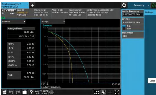
Band41-15MHz-QPSK-40620-75RB#0-PASS
