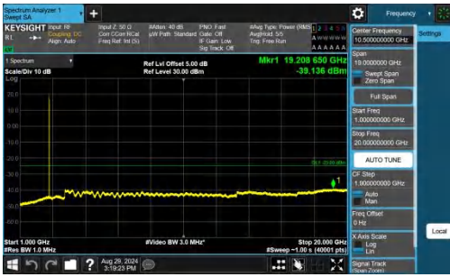
Band41-10MHz-QPSK-41540-1RB#49-1000~20000-PASS
