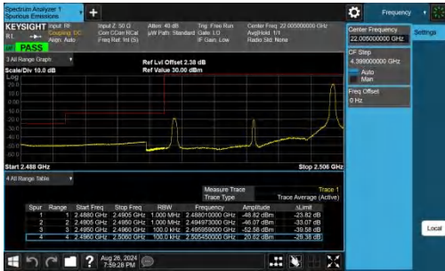
Band41-10MHz-QPSK-39700-1RB#49-PASS
