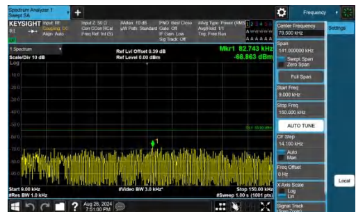
Band41-5MHz-QPSK-39675-1RB#24-0.009~0.15-PASS
