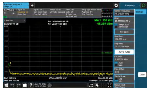
Band41-15MHz-QPSK-39725-1RB#0-0.15~30-PASS
