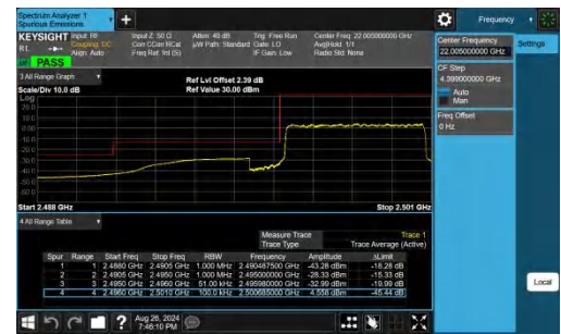
Band41-5MHz-QPSK-39675-25RB#0-PASS
