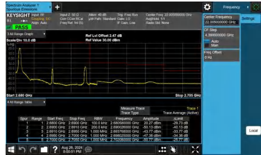
Band41-10MHz-QPSK-41540-1RB#0-PASS
