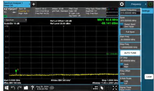
Band41-20MHz-QPSK-39750-1RB#99-30~1000-PASS
