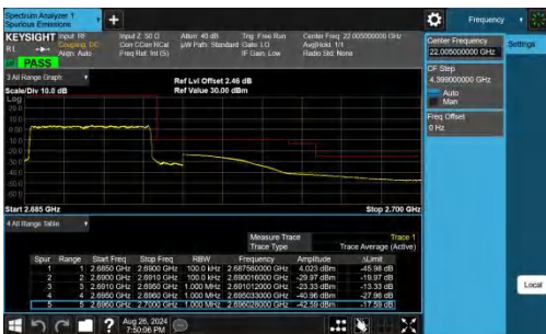
Band41-5MHz-QPSK-41565-1RB#0-PASS
