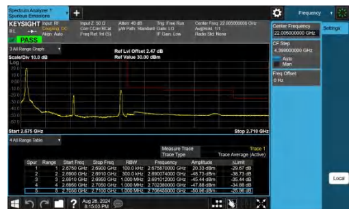
Band41-15MHz-QPSK-41515-1RB#0-PASS
