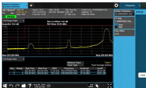
Band26(824-849)-5MHz-QPSK-26815-1RB#24-PASS
