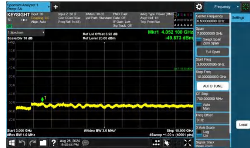
Band26(824-849)-1.4MHz-QPSK-26797-1RB#5-3000~10000-PAS
