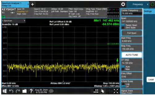
Band26(824-849)-15MHz-QPSK-26865-1RB#0-0.009~0.15-PASS
