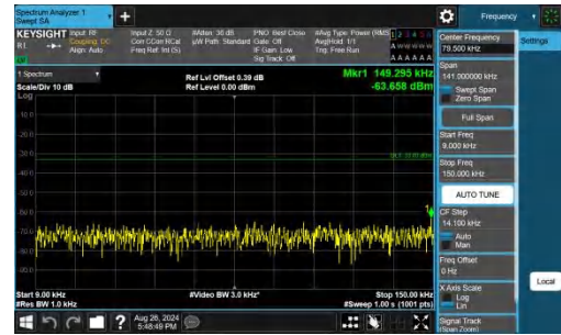
Band26(824-849)-3MHz-QPSK-26805-1RB#14-0.009~0.15-PASS
