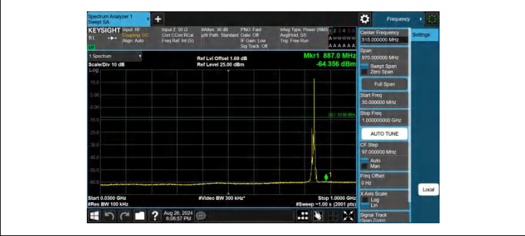
Band26(824-849)-10MHz-QPSK-26915-1RB#49-30~1000-PASS
