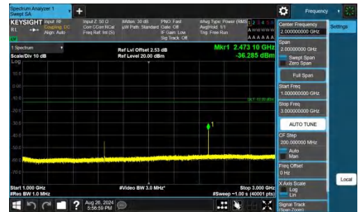
Band26(824-849)-5MHz-QPSK-26815-1RB#0-1000~3000-PASS
