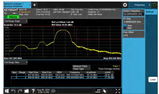
Band26(824-849)-1.4MHz-QPSK-27033-1RB#5-PASS
