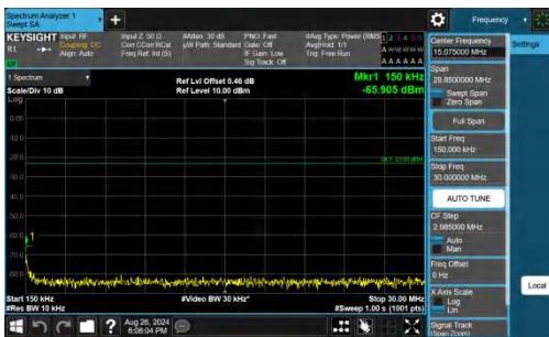
Band26(824-849)-10MHz-QPSK-26990-1RB#49-0.15~30-PASS
