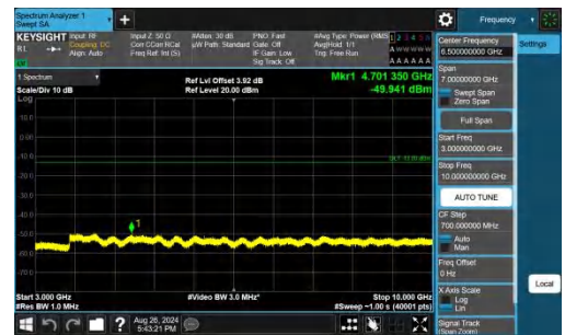
Band26(824-849)-1.4MHz-QPSK-27033-1RB#5-3000~10000-PAS
