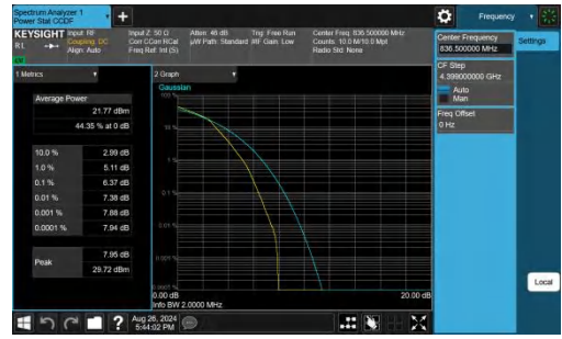
Band26(824-849)-1.4MHz-16QAM-26915-6RB#0-PASS
