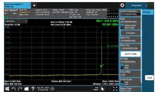
Band26(824-849)-1.4MHz-QPSK-27033-1RB#5-30~1000-PASS
