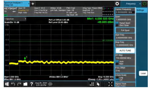
Band26(824-849)-3MHz-QPSK-27025-1RB#14-3000~10000-PASS
