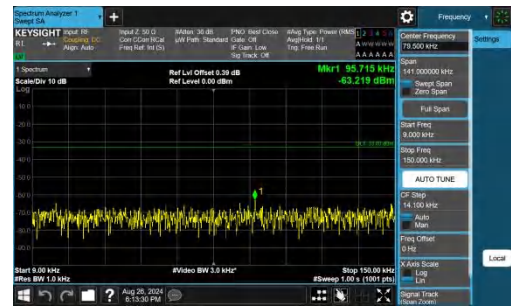
Band26(824-849)-15MHz-QPSK-26865-1RB#74-0.009~0.15-PASS
