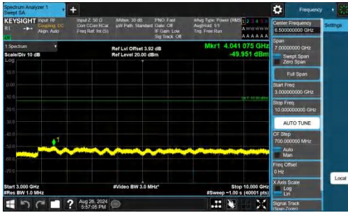
Band26(824-849)-5MHz-QPSK-26815-1RB#0-3000~10000-PASS
