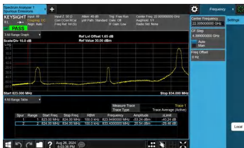
Band26(824-849)-10MHz-QPSK-26840-1RB#49-PASS
