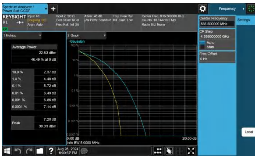
Band26(824-849)-5MHz-QPSK-26915-25RB#0-PASS
