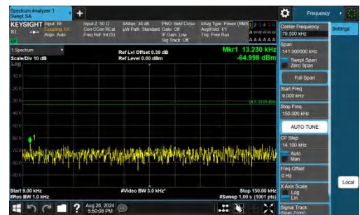
Band26(824-849)-3MHz-QPSK-26915-1RB#14-0.009~0.15-PASS
