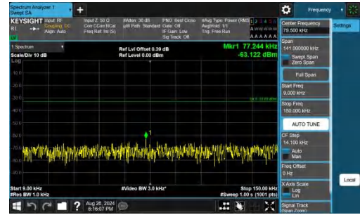
Band26(824-849)-15MHz-QPSK-26965-1RB#74-0.009~0.15-PASS
