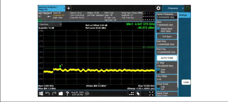
Band26(824-849)-10MHz-QPSK-26915-1RB#49-3000~10000-PAS
