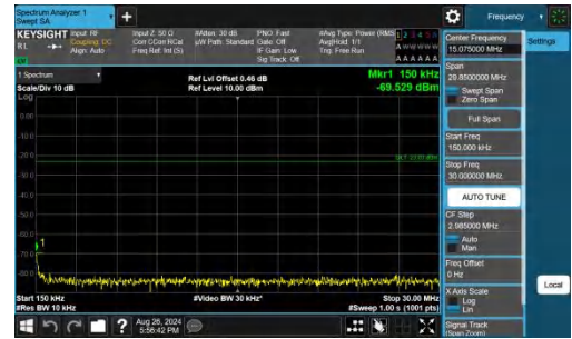
Band26(824-849)-5MHz-QPSK-26815-1RB#0-0.15~30-PASS
