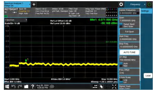
Band26(824-849)-10MHz-QPSK-26840-1RB#49-3000~10000-PAS
