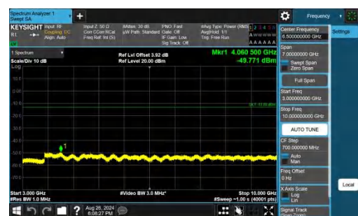
Band26(824-849)-10MHz-QPSK-26990-1RB#49-3000~10000-PASS S
