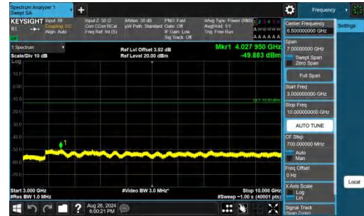
Band26(824-849)-5MHz-QPSK-27015-1RB#24-3000~10000-PASS
