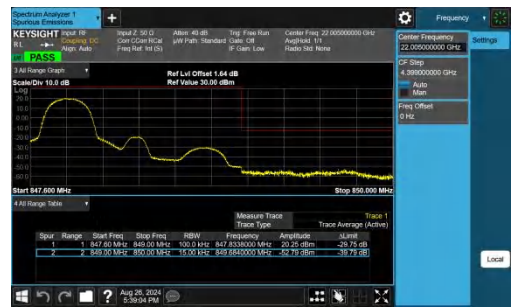
Band26(824-849)-1.4MHz-QPSK-27033-1RB#0-PASS
