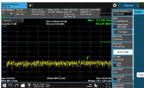
Band26(824-849)-3MHz-QPSK-26805-1RB#0-0.009~0.15-PASS
