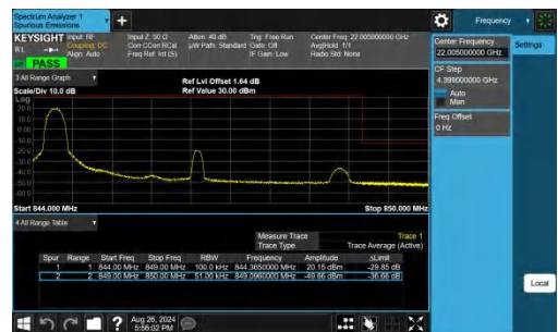
Band26(824-849)-5MHz-QPSK-27015-1RB#0-PASS
