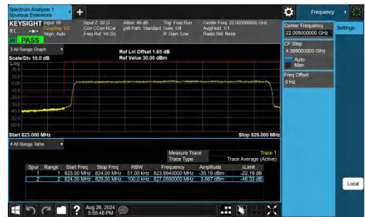
Band26(824-849)-5MHz-QPSK-26815-25RB#0-PASS
