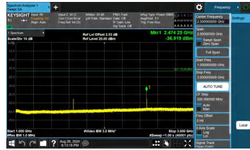
Band26(824-849)-15MHz-QPSK-26865-1RB#0-1000~3000-PASS
