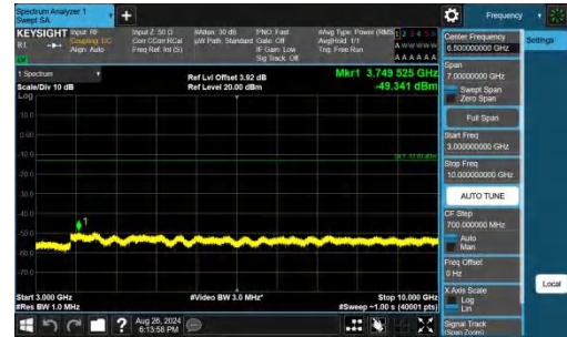
Band26(824-849)-15MHz-QPSK-26865-1RB#74-3000~10000-PAS
