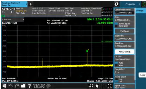
Band26(824-849)-15MHz-QPSK-26865-1RB#74-1000~3000-PAS
