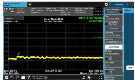
Band26(824-849)-5MHz-QPSK-26815-1RB#24-3000~10000-PASS
