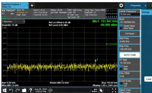
Band26(824-849)-1.4MHz-QPSK-26915-1RB#0-0.009~0.15-PASS
