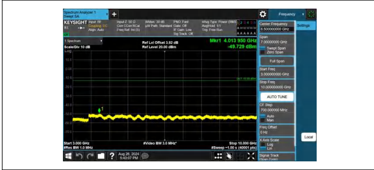
Band26(824-849)-1.4MHz-QPSK-26797-1RB#0-3000~10000-PAS
