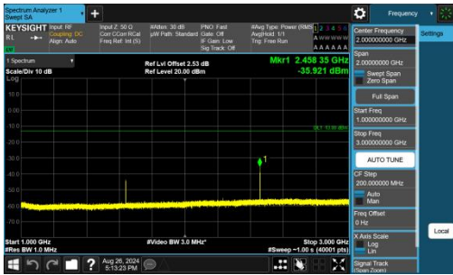
Band26(814-824)-1.4MHz-QPSK-26740-1RB#5-1000~3000-PASS
