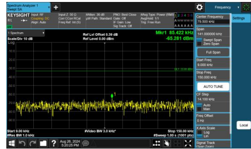
Band26(814-824)-3MHz-QPSK-26705-1RB#14-0.009~0.15-PASS
