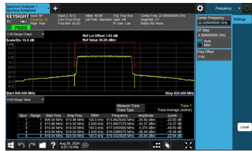
Band26(814-824)-5MHz-QPSK-26715-25RB#0-PASS
