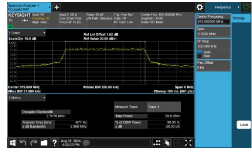
Band26(814-824)-3MHz-16QAM-26740-15RB#0-PASS
