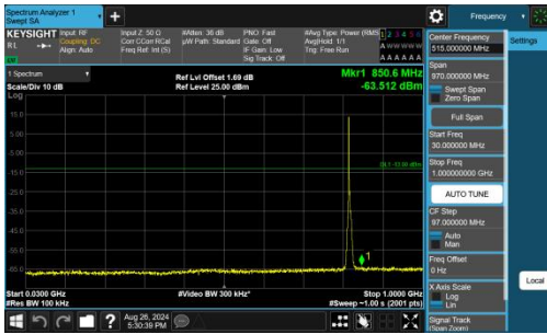
Band26(814-824)-5MHz-QPSK-26765-1RB#0-30~1000-PASS
