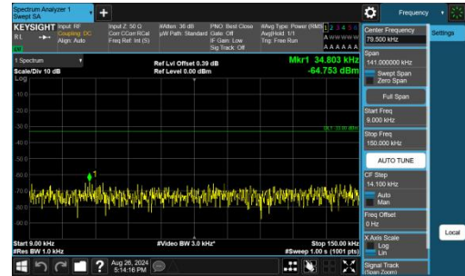
Band26(814-824)-1.4MHz-QPSK-26783-1RB#5-0.009~0.15-PASS
