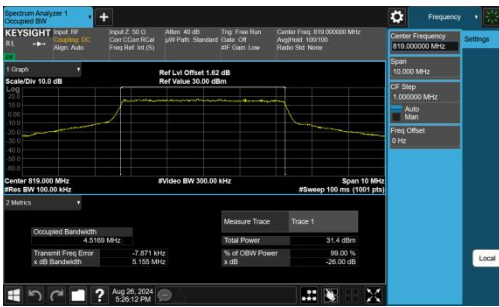
Band26(814-824)-5MHz-QPSK-26740-25RB#0-PASS
