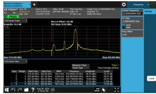
Band26(814-824)-3MHz-QPSK-26775-1RB#14-PASS
