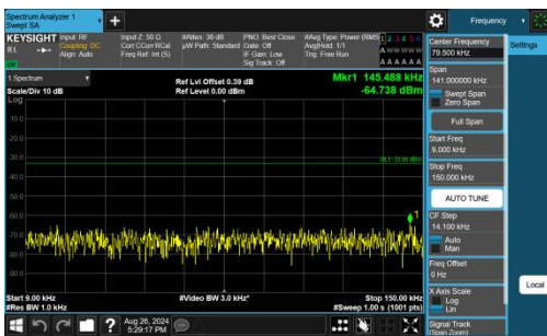
Band26(814-824)-5MHz-QPSK-26740-1RB#0-0.009~0.15-PASS
