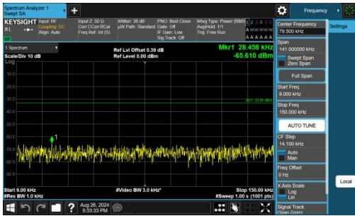
Band26(814-824)-10MHz-QPSK-26740-1RB#0-0.009~0.15-PASS
