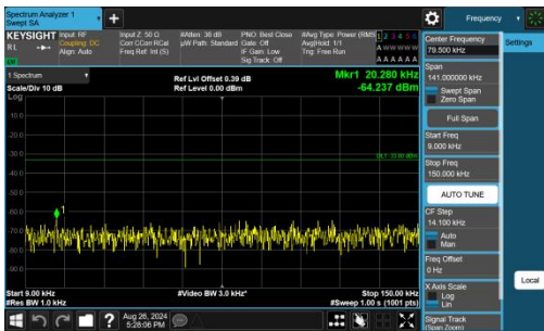
Band26(814-824)-5MHz-QPSK-26715-1RB#0-0.009~0.15-PASS
