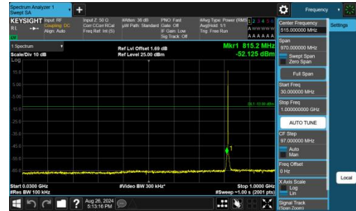
Band26(814-824)-1.4MHz-QPSK-26740-1RB#5-30~1000-PASS
