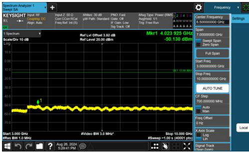
Band26(814-824)-5MHz-QPSK-26740-1RB#0-3000~10000-PASS
