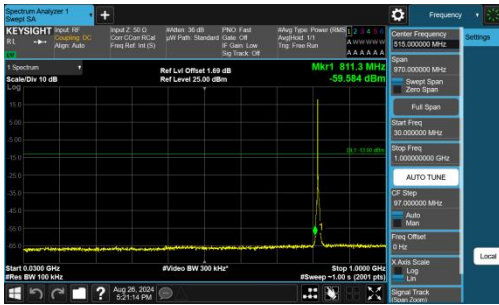
Band26(814-824)-3MHz-QPSK-26740-1RB#0-30~1000-PASS
