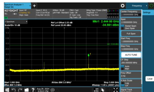
Band26(814-824)-10MHz-QPSK-26740-1RB#0-1000~3000-PASS
