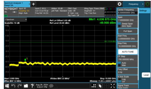
Band26(814-824)-3MHz-QPSK-26740-1RB#14-3000~10000-PASS
