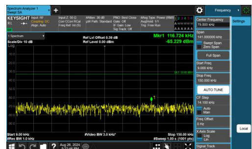
Band26(814-824)-3MHz-QPSK-26775-1RB#14-0.009~0.15-PASS
