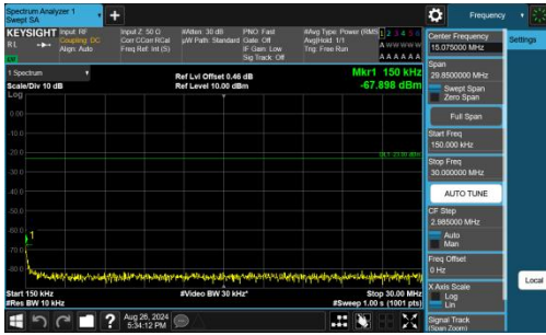
Band26(814-824)-10MHz-QPSK-26740-1RB#49-0.15~30-PASS
