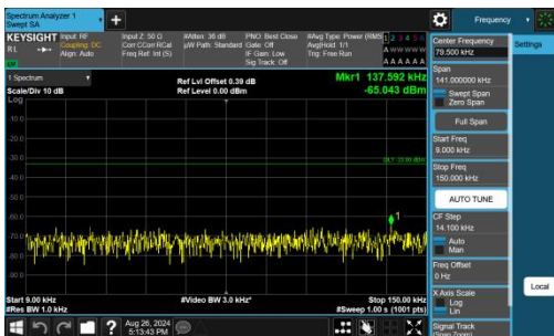
Band26(814-824)-1.4MHz-QPSK-26783-1RB#0-0.009~0.15-PASS
