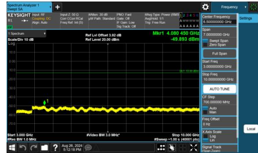
Band26(814-824)-1.4MHz-QPSK-26697-1RB#5-3000~10000-PAS
