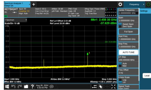
Band26(814-824)-5MHz-QPSK-26765-1RB#0-1000~3000-PASS
