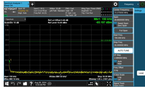
Band26(814-824)-10MHz-QPSK-26740-1RB#0-0.15~30-PASS
