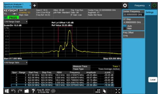
Band26(814-824)-1.4MHz-QPSK-26783-1RB#5-PASS
