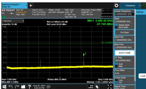
Band26(814-824)-3MHz-QPSK-26705-1RB#14-1000~3000-PASS
