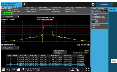
Band26(814-824)-1.4MHz-QPSK-26783-6RB#0-PASS
