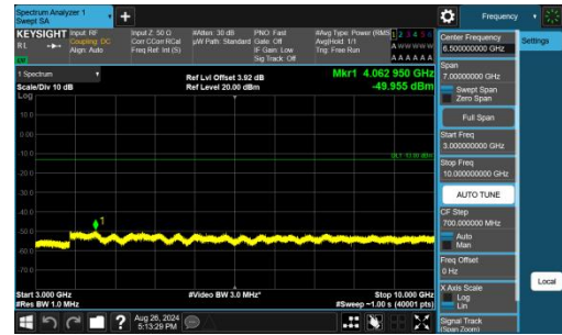
Band26(814-824)-1.4MHz-QPSK-26740-1RB#5-3000~10000-PASS S
