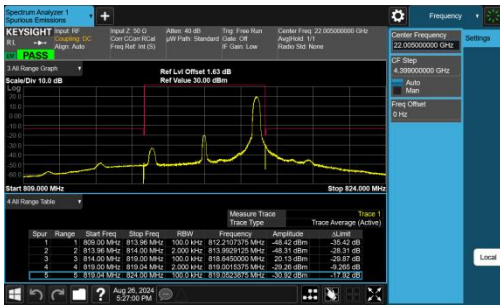
Band26(814-824)-5MHz-QPSK-26715-1RB#24-PASS
