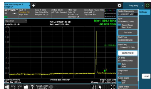
Band26(814-824)-5MHz-QPSK-26740-1RB#24-30~1000-PASS
