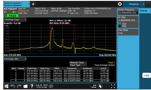
Band26(814-824)-3MHz-QPSK-26775-1RB#0-PASS
