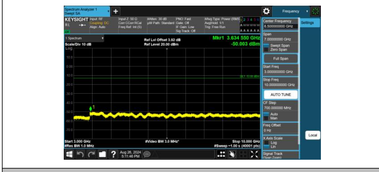
Band26(814-824)-1.4MHz-QPSK-26697-1RB#0-3000~10000-PAS
