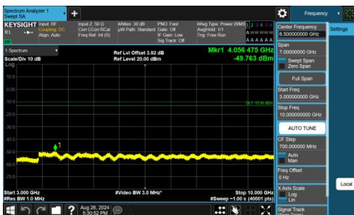
Band26(814-824)-5MHz-QPSK-26765-1RB#0-3000~10000-PASS
