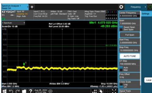
Band26(814-824)-1.4MHz-QPSK-26740-1RB#0-3000~10000-PAS
