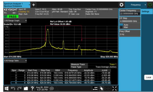
Band26(814-824)-5MHz-QPSK-26765-1RB#0-PASS
