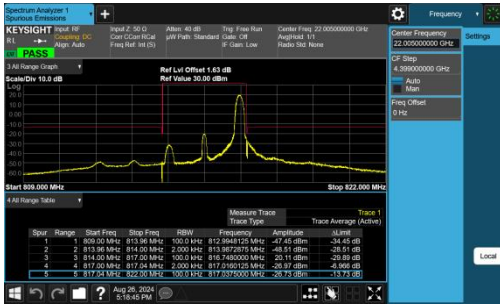
Band26(814-824)-3MHz-QPSK-26705-1RB#14-PASS
