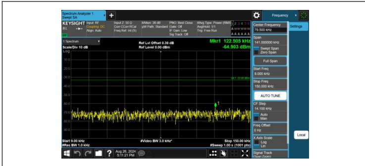
Band26(814-824)-1.4MHz-QPSK-26697-1RB#0-0.009~0.15-PASS
