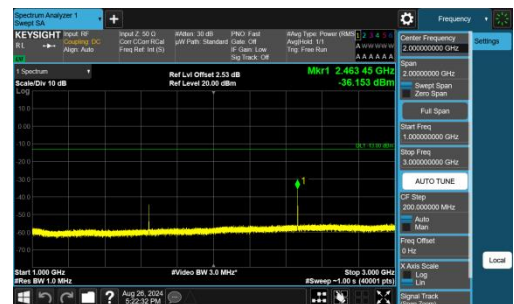
Band26(814-824)-3MHz-QPSK-26775-1RB#0-1000~3000-PASS
