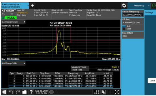
Band26(814-824)-1.4MHz-QPSK-26697-1RB#0-PASS
