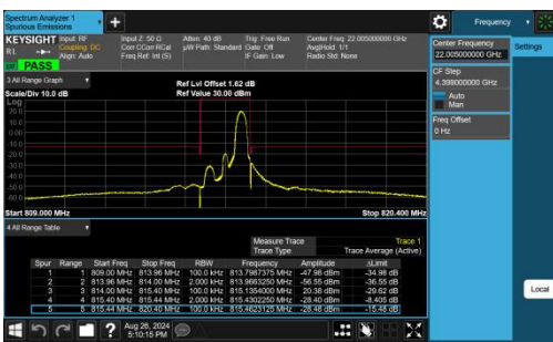
Band26(814-824)-1.4MHz-QPSK-26697-1RB#5-PASS
