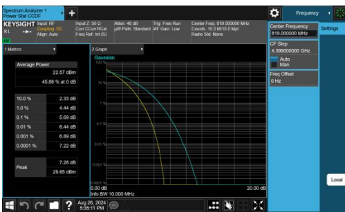
Band26(814-824)-10MHz-QPSK-26740-50RB#0-PASS
