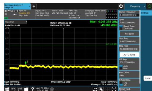
Band26(814-824)-1.4MHz-QPSK-26783-1RB#5-3000~10000-PAS
