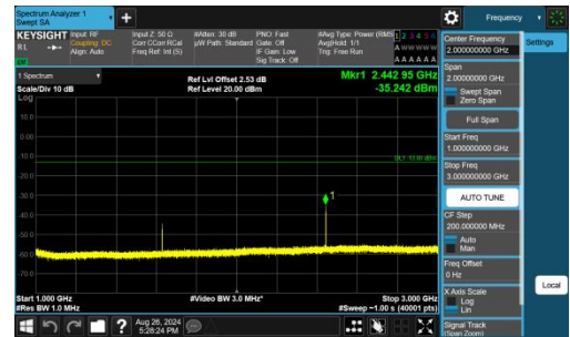
Band26(814-824)-5MHz-QPSK-26715-1RB#0-1000~3000-PASS
