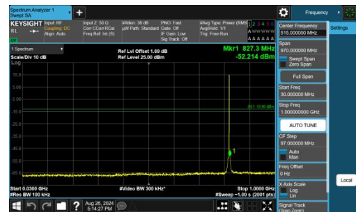
Band26(814-824)-1.4MHz-QPSK-26783-1RB#5-30~1000-PASS
