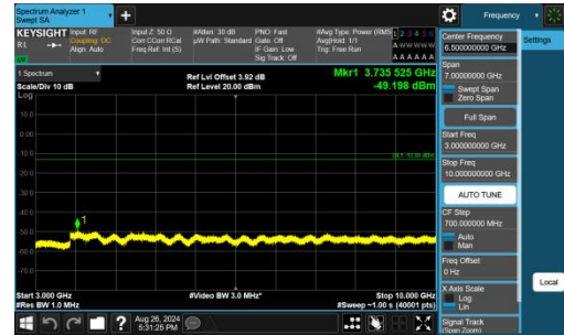
Band26(814-824)-5MHz-QPSK-26765-1RB#24-3000~10000-PASS
