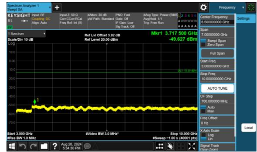
Band26(814-824)-10MHz-QPSK-26740-1RB#49-3000~10000-PAS
