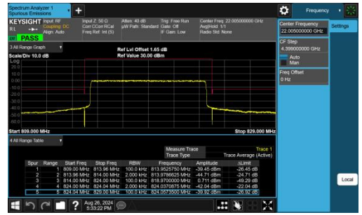
Band26(814-824)-10MHz-QPSK-26740-50RB#0-PASS
