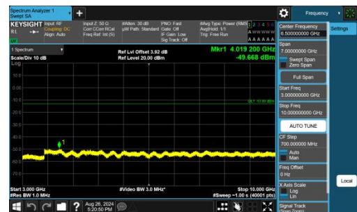
Band26(814-824)-3MHz-QPSK-26705-1RB#14-3000~10000-PASS
