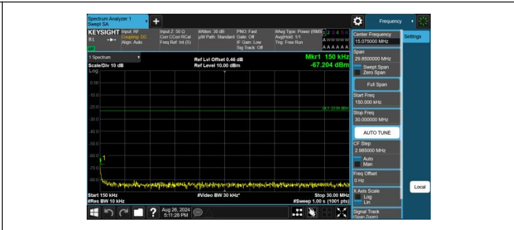
Band26(814-824)-1.4MHz-QPSK-26697-1RB#0-0.15~30-PASS
