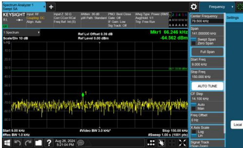
Band26(814-824)-3MHz-QPSK-26740-1RB#0-0.009~0.15-PASS
