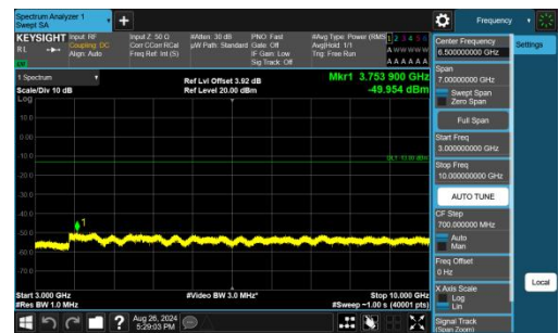
Band26(814-824)-5MHz-QPSK-26715-1RB#24-3000~10000-PASS
