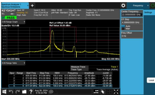
Band26(814-824)-3MHz-QPSK-26705-1RB#0-PASS
