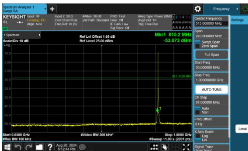
Band26(814-824)-1.4MHz-QPSK-26740-1RB#0-30~1000-PASS
