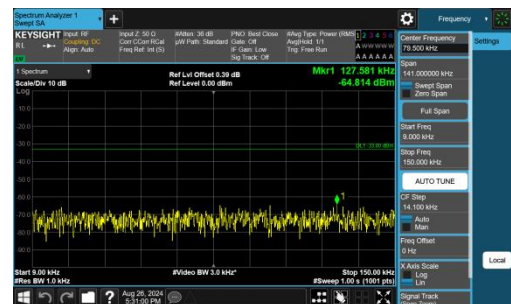
Band26(814-824)-5MHz-QPSK-26765-1RB#24-0.009~0.15-PASS
