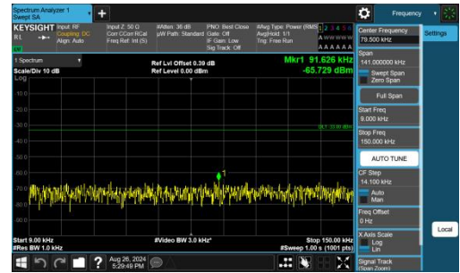
Band26(814-824)-5MHz-QPSK-26740-1RB#24-0.009~0.15-PASS
