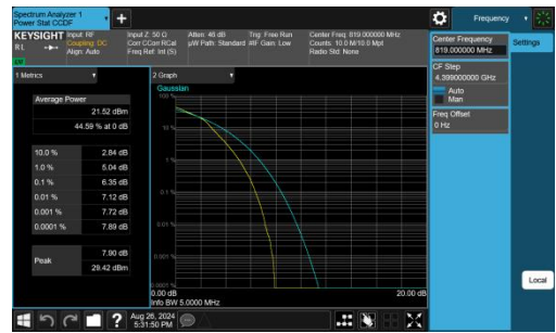
Band26(814-824)-5MHz-16QAM-26740-25RB#0-PASS
