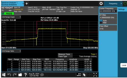
Band26(814-824)-5MHz-QPSK-26765-25RB#0-PASS
