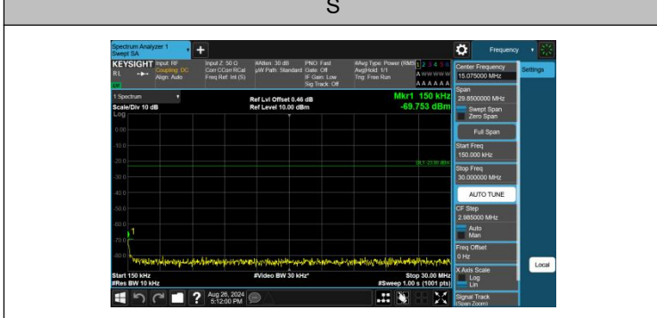
Band26(814-824)-1.4MHz-QPSK-26697-1RB#5-0.15~30-PASS
