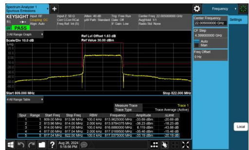
Band26(814-824)-3MHz-QPSK-26705-15RB#0-PASS
