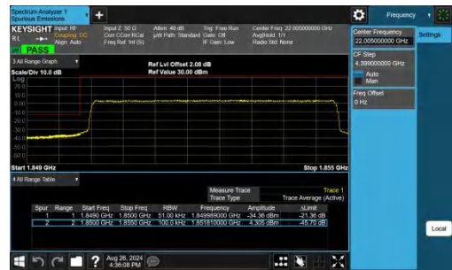
Band25-5MHz-QPSK-26065-25RB#0-PASS
