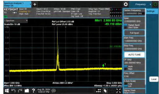
Band25-20MHz-QPSK-26140-1RB#0-1000~3000-PASS
