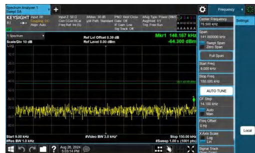
Band25-20MHz-QPSK-26590-1RB#99-0.009~0.15-PASS
