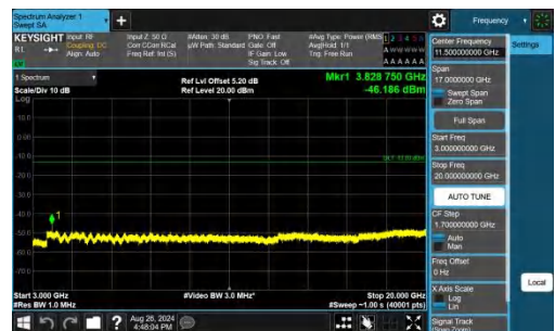
Band25-10MHz-QPSK-26640-1RB#49-3000~20000-PASS
