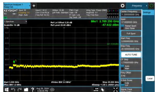
Band25-5MHz-QPSK-26365-1RB#24-3000~20000-PASS
