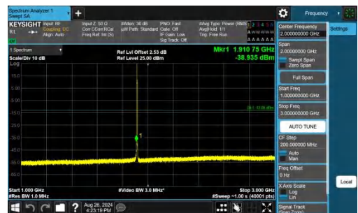
Band25-1.4MHz-QPSK-26683-1RB#0-1000~3000-PASS
