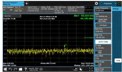
Band25-20MHz-QPSK-26140-1RB#99-0.009~0.15-PASS
