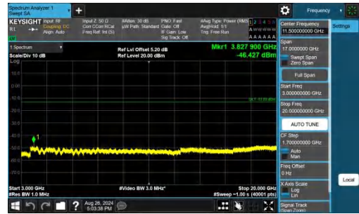
Band25-20MHz-QPSK-26590-1RB#99-3000~20000-PASS
