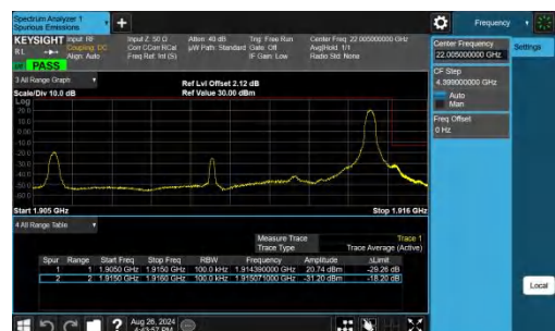
Band25-10MHz-QPSK-26640-1RB#49-PASS
