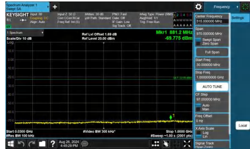
Band25-10MHz-QPSK-26090-1RB#49-30~1000-PASS
