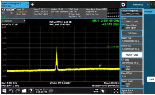
Band25-15MHz-QPSK-26365-1RB#74-1000~3000-PASS
