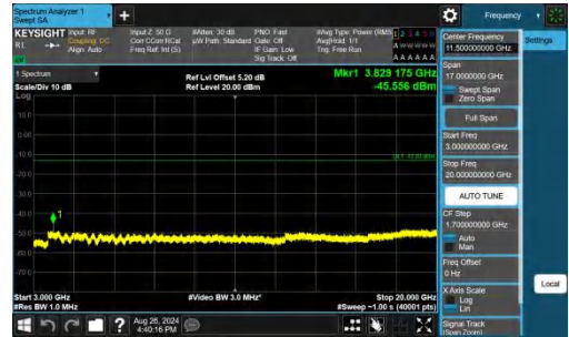
Band25-5MHz-QPSK-26665-1RB#24-3000~20000-PASS
