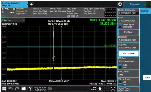
Band25-1.4MHz-QPSK-26047-1RB#5-1000~3000-PASS
