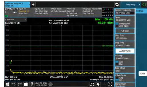
Band25-5MHz-QPSK-26365-1RB#0-0.15~30-PASS
