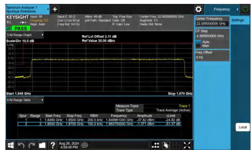
Band25-20MHz-QPSK-26140-100RB#0-PASS
