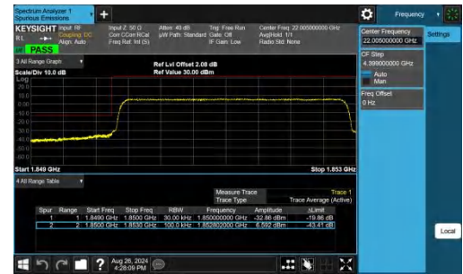
Band25-3MHz-QPSK-26055-15RB#0-PASS
