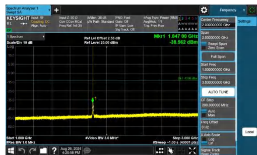
Band25-1.4MHz-QPSK-26047-1RB#0-1000~3000-PASS
