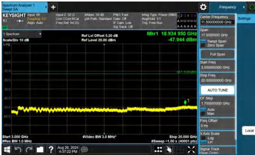
Band25-5MHz-QPSK-26065-1RB#0-3000~2000-PASS
