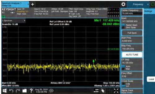
Band25-3MHz-QPSK-26365-1RB#0-0.009~0.15-PASS
