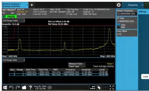
Band25-15MHz-QPSK-26115-1RB#74-PASS
