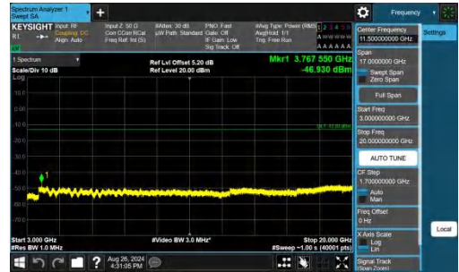
Band25-3MHz-QPSK-26365-1RB#14-3000~20000-PASS
