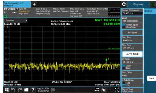
Band25-15MHz-QPSK-26615-1RB#74-0.009~0.15-PASS
