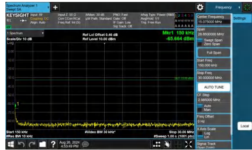
Band25-15MHz-QPSK-26365-1RB#0-0.15~30-PASS
