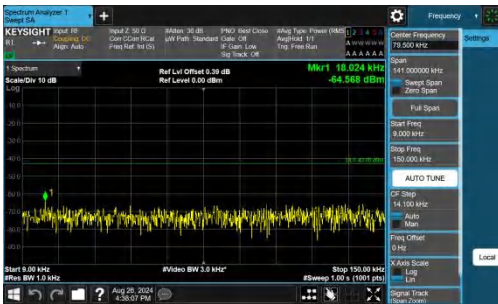
Band25-5MHz-QPSK-26365-1RB#0-0.009~0.15-PASS
