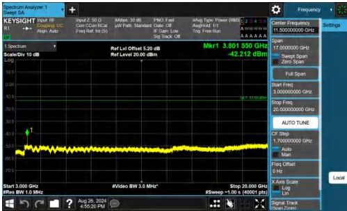
Band25-15MHz-QPSK-26615-1RB#0-3000~20000-PASS
