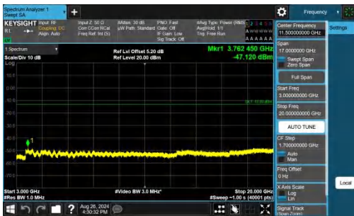
Band25-3MHz-QPSK-26365-1RB#0-3000~20000-PASS
