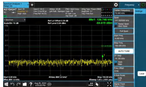
Band25-15MHz-QPSK-26115-1RB#74-0.009~0.15-PASS
