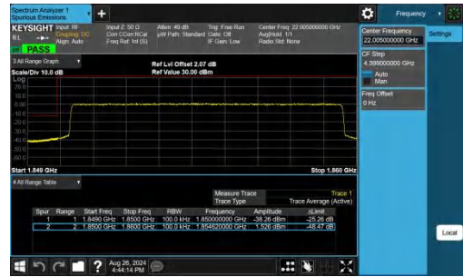
Band25-10MHz-QPSK-26090-50RB#0-PASS
