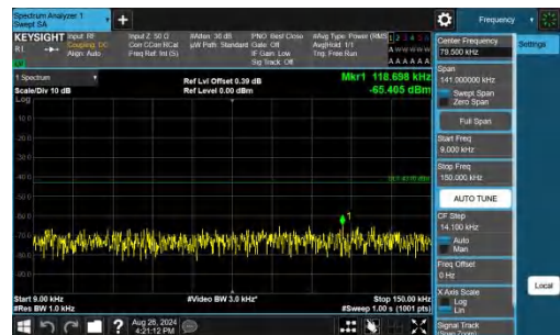
Band25-1.4MHz-QPSK-26047-1RB#5-0.009~0.15-PASS
