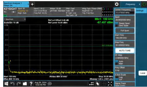
Band25-20MHz-QPSK-26590-1RB#0-0.15~30-PASS
