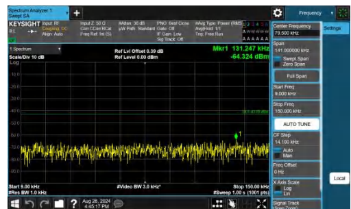
Band25-10MHz-QPSK-26090-1RB#49-0.009~0.15-PASS
