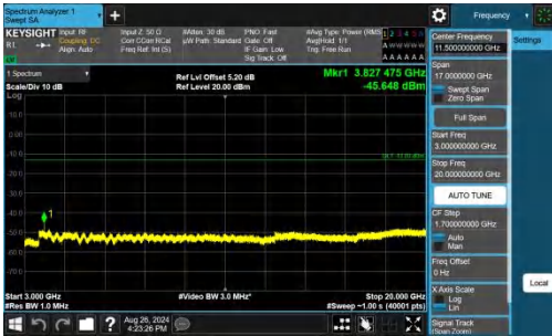
Band25-1.4MHz-QPSK-26683-1RB#0-3000~20000-PASS
