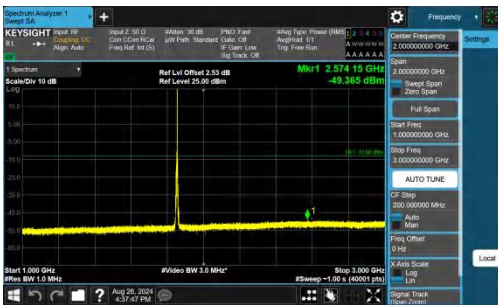
Band25-5MHz-QPSK-26065-1RB#24-1000~3000-PASS
