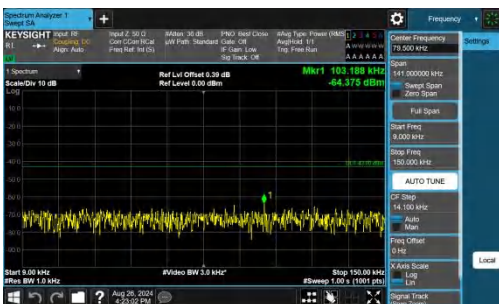
Band25-1.4MHz-QPSK-26683-1RB#0-0.009~0.15-PASS
