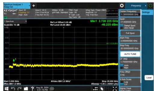
Band25-20MHz-QPSK-26140-1RB#99-3000~20000-PASS
