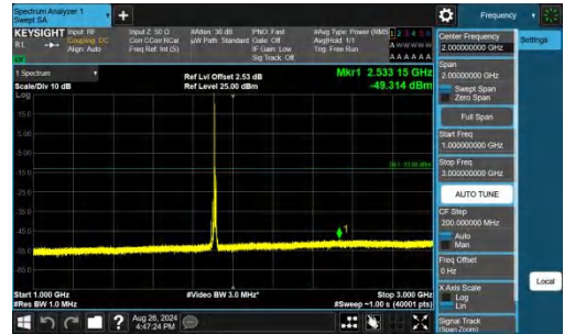
Band25-10MHz-QPSK-26640-1RB#0-1000~3000-PASS
