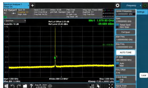
Band25-1.4MHz-QPSK-26365-1RB#0-1000~3000-PASS
