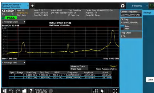
Band25-10MHz-QPSK-26090-1RB#49-PASS
