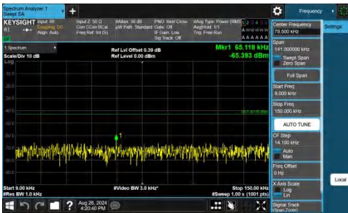
Band25-1.4MHz-QPSK-26047-1RB#0-0.009~0.15-PASS
