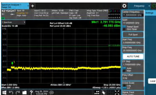
Band25-20MHz-QPSK-26590-1RB#0-3000~20000-PASS
