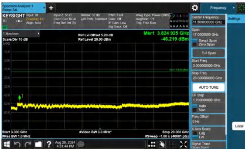
Band25-3MHz-QPSK-26675-1RB#0-3000~20000-PASS
