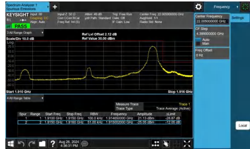
Band25-5MHz-QPSK-26665-1RB#24-PASS
