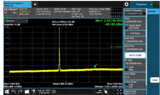
Band25-5MHz-QPSK-26365-1RB#0-1000~3000-PASS
