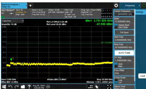
Band25-15MHz-QPSK-26365-1RB#0-3000~20000-PASS
