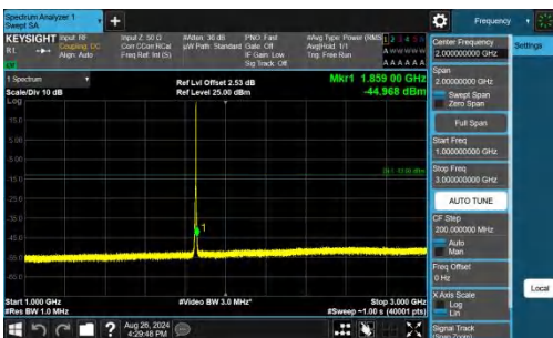
Band25-3MHz-QPSK-26055-1RB#14-1000~3000-PASS
