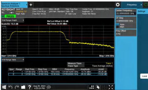
Band25-1.4MHz-QPSK-26683-6RB#0-PASS
