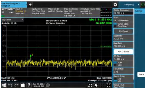
Band25-20MHz-QPSK-26140-1RB#0-0.009~0.15-PASS
