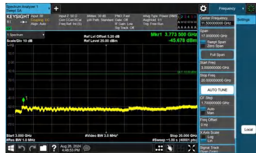
Band25-10MHz-QPSK-26365-1RB#49-3000~20000-PASS
