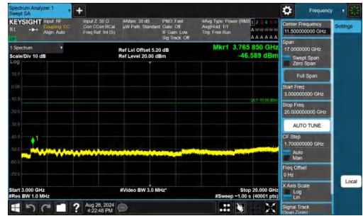
Band25-1.4MHz-QPSK-26365-1RB#5-3000~20000-PASS
