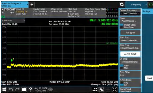
Band25-5MHz-QPSK-26365-1RB#0-3000~20000-PASS
