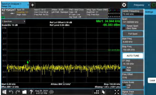
Band25-10MHz-QPSK-26640-1RB#0-0.009~0.15-PASS
