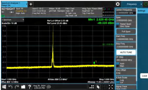
Band25-15MHz-QPSK-26115-1RB#74-1000~3000-PASS
