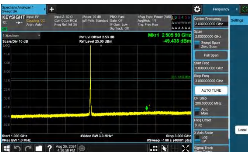
Band25-5MHz-QPSK-26365-1RB#24-1000~3000-PASS
