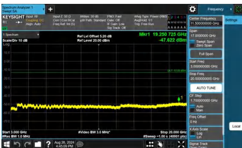
Band25-10MHz-QPSK-26090-1RB#0-3000~20000-PASS
