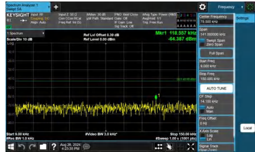
Band25-1.4MHz-QPSK-26683-1RB#5-0.009~0.15-PASS
