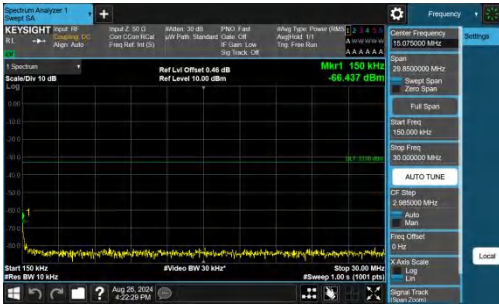
Band25-1.4MHz-QPSK-26365-1RB#5-0.15~30-PASS
