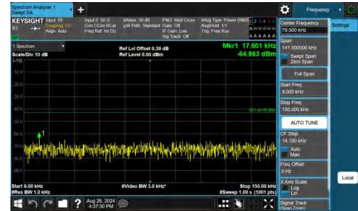
Band25-5MHz-QPSK-26065-1RB#24-0.009~0.15-PASS
