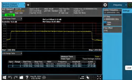
Band25-15MHz-QPSK-26615-75RB#0-PASS
