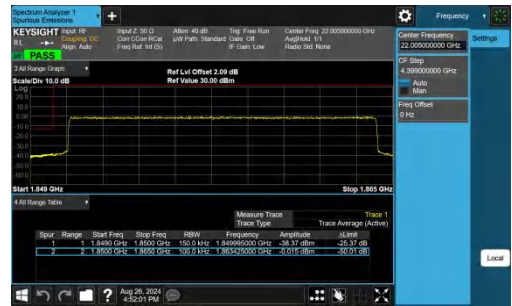
Band25-15MHz-QPSK-26115-75RB#0-PASS
