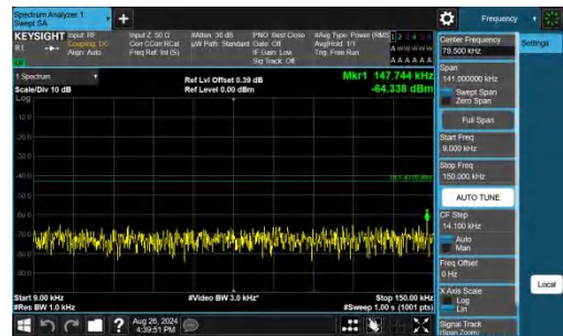
Band25-5MHz-QPSK-26665-1RB#24-0.009~0.15-PASS
