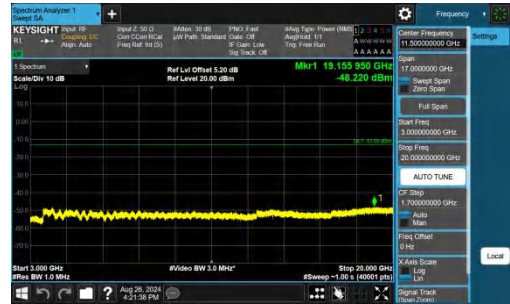
Band25-1.4MHz-QPSK-26047-1RB#5-3000~20000-PASS
