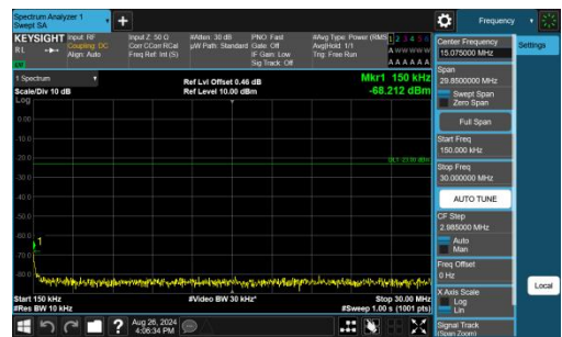
Band13-5MHz-QPSK-23230-1RB#0-0.15~30-PASS
