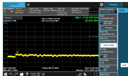
Band13-10MHz-QPSK-23230-1RB#49-3000~10000-PASS
