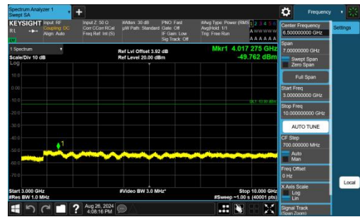
Band13-5MHz-QPSK-23255-1RB#0-3000~10000-PASS
