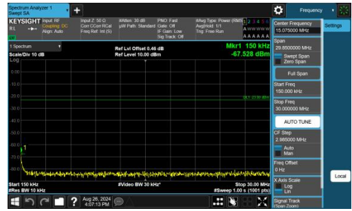
Band13-5MHz-QPSK-23230-1RB#24-0.15~30-PASS
