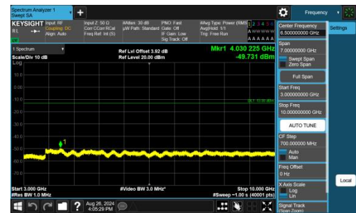
Band13-5MHz-QPSK-23205-1RB#0-3000~10000-PASS
