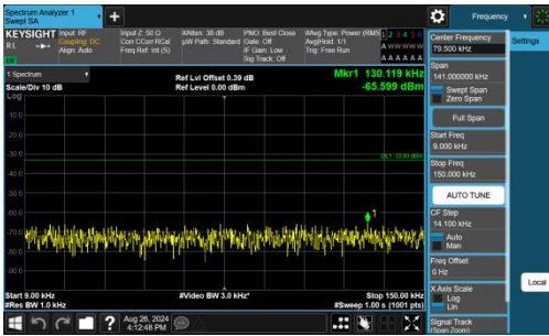
Band13-10MHz-QPSK-23230-50RB#0-0.009~0.15-PASS
