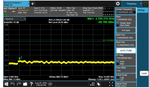
Band13-5MHz-QPSK-23205-1RB#24-3000~10000-PASS
