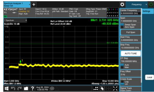
Band13-5MHz-QPSK-23255-1RB#24-3000~10000-PASS
