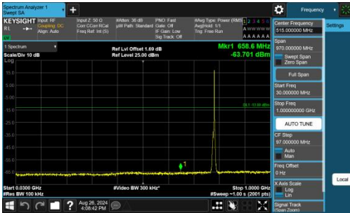
Band13-5MHz-QPSK-23255-1RB#24-30~1000-PASS
