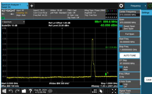
Band13-10MHz-QPSK-23230-50RB#0-30~1000-PASS
