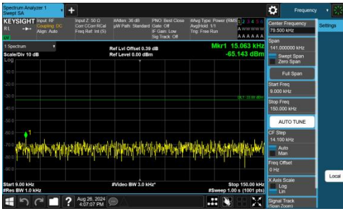
Band13-5MHz-QPSK-23230-1RB#24-0.009~0.15-PASS
