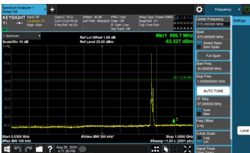
Band13-10MHz-QPSK-23230-1RB#0-30~1000-PASS
