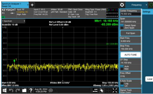
Band13-5MHz-QPSK-23255-1RB#24-0.009~0.15-PASS
