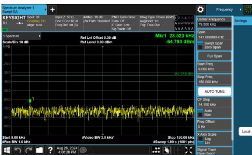
Band13-5MHz-QPSK-23230-1RB#0-0.009~0.15-PASS
