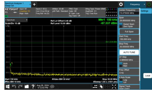
Band13-10MHz-QPSK-23230-50RB#0-0.15~30-PASS
