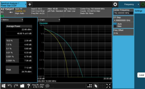
Band13-10MHz-QPSK-23230-50RB#0-PASS
