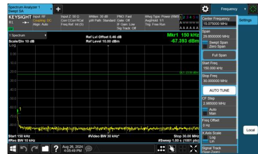
Band13-5MHz-QPSK-23205-1RB#24-0.15~30-PASS
