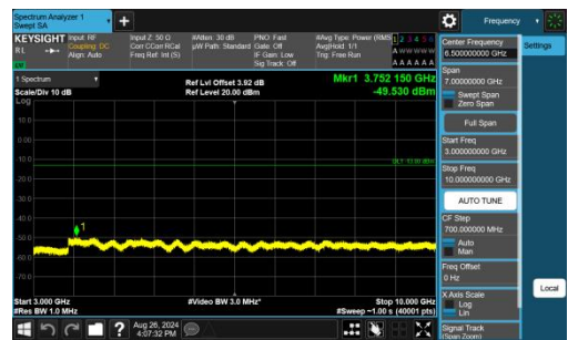
Band13-5MHz-QPSK-23230-1RB#24-3000~10000-PASS
