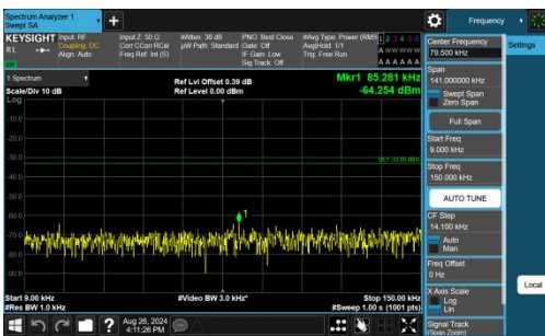
Band13-10MHz-QPSK-23230-1RB#0-0.009~0.15-PASS
