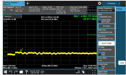
Band13-5MHz-QPSK-23230-1RB#0-3000~10000-PASS
