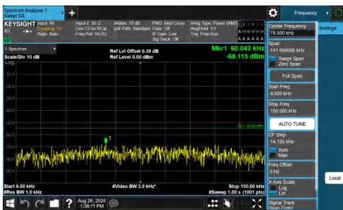
Band7-10MHz-QPSK-20800-1RB#0-0.009~0.15-PASS
