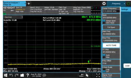
Band7-10MHz-QPSK-21400-1RB#49-30~1000-PASS
