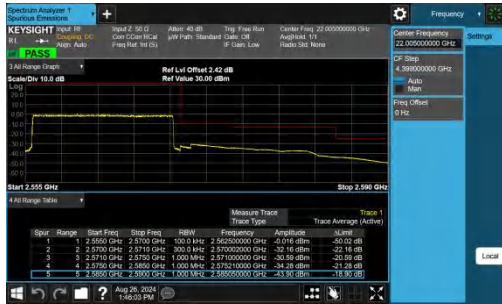
Band7-15MHz-QPSK-21375-75RB#0-PASS
