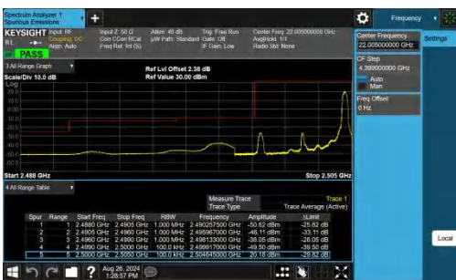
Band7-5MHz-QPSK-20775-1RB#24-PASS
