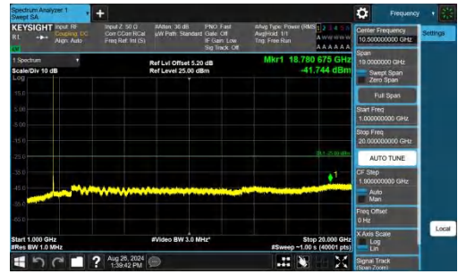
Band7-10MHz-QPSK-21100-1RB#0-1000~20000-PASS
