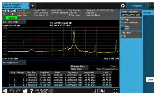
Band7-15MHz-QPSK-20825-1RB#0-PASS
