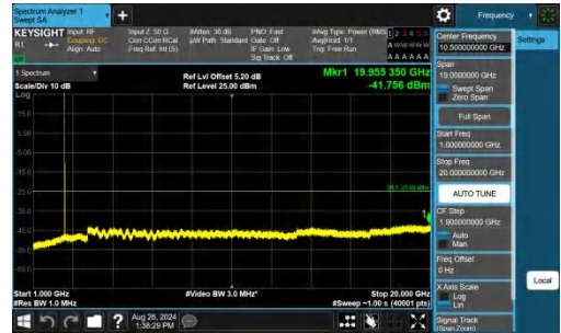
Band7-10MHz-QPSK-20800-1RB#0-1000~20000-PASS
