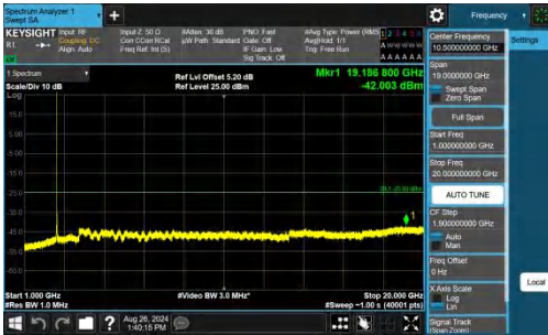
Band7-10MHz-QPSK-21100-1RB#49-1000~20000-PASS
