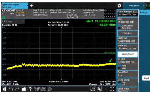
Band7-5MHz-QPSK-21425-1RB#24-1000~20000-PASS
