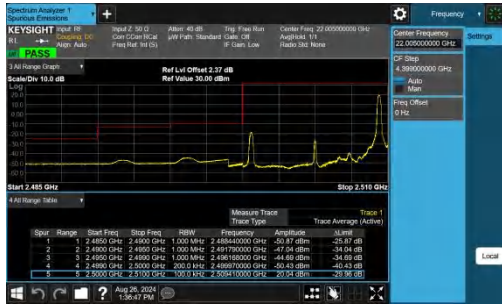
Band7-10MHz-QPSK-20800-1RB#49-PASS
