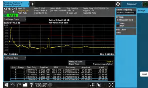
Band7-10MHz-QPSK-21400-1RB#0-PASS
