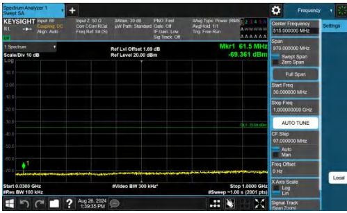
Band7-10MHz-QPSK-21100-1RB#0-30~1000-PASS
