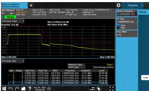
Band7-5MHz-QPSK-21425-25RB#0-PASS
