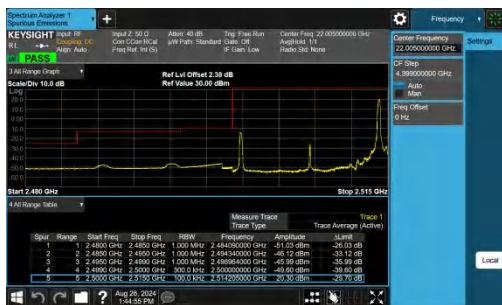
Band7-15MHz-QPSK-20825-1RB#74-PASS
