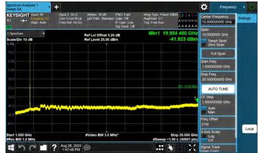
Band7-15MHz-QPSK-21100-1RB#0-1000~20000-PASS
