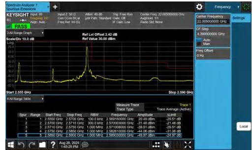
Band7-15MHz-QPSK-21375-1RB#74-PASS
