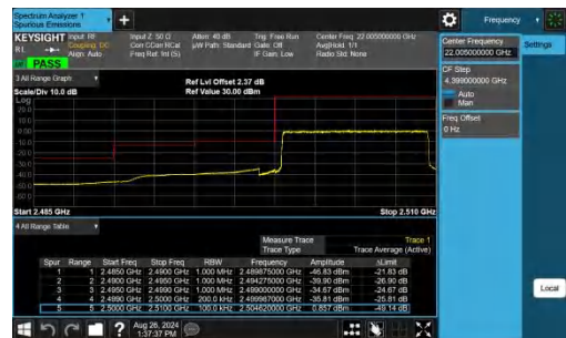
Band7-10MHz-QPSK-20800-50RB#0-PASS
