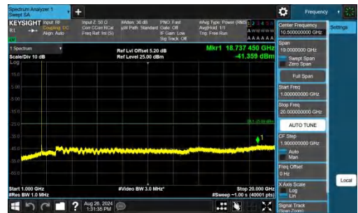
Band7-5MHz-QPSK-21100-1RB#0-1000~20000-PASS
