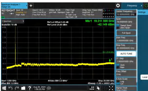
Band7-20MHz-QPSK-21100-1RB#99-1000~20000-PASS
