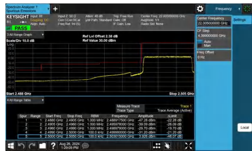
Band7-5MHz-QPSK-20775-25RB#0-PASS
