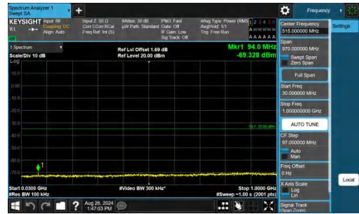
Band7-15MHz-QPSK-20825-1RB#74-30~1000-PASS
