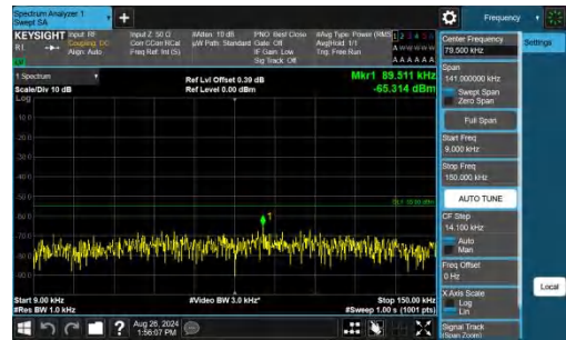
Band7-20MHz-QPSK-21100-1RB#99-0.009~0.15-PASS
