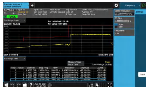
Band7-15MHz-QPSK-20825-75RB#0-PASS
