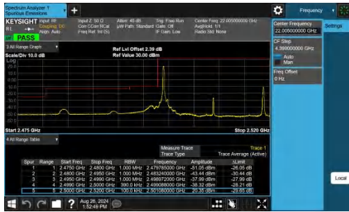
Band7-20MHz-QPSK-20850-1RB#0-PASS
