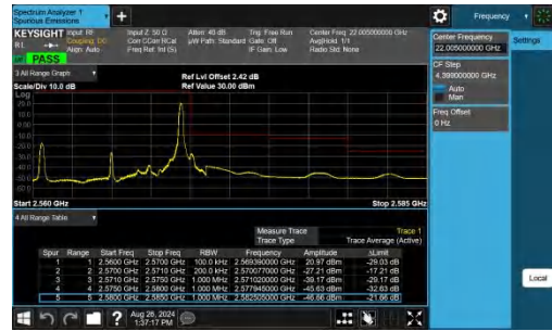
Band7-10MHz-QPSK-21400-1RB#49-PASS
