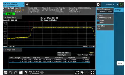
Band4-3MHz-QPSK-19965-15RB#0-PASS
