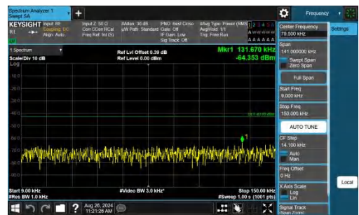
Band4-20MHz-QPSK-20300-1RB#99-0.009~0.15-PASS
