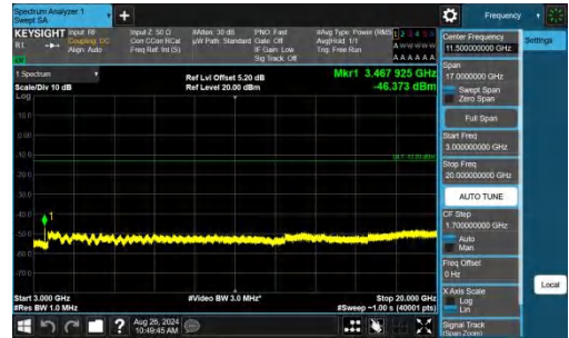
Band4-3MHz-QPSK-20175-1RB#14-3000~20000-PASS
