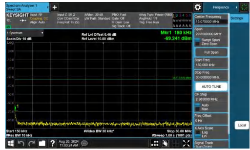
Band4-10MHz-QPSK-20000-1RB#0-0.15~30-PASS
