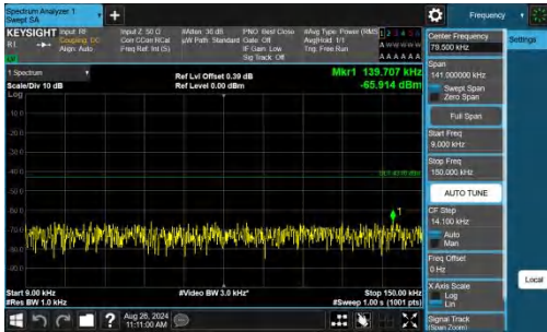
Band4-15MHz-QPSK-2025-1RB#0-0.009~0.15-PASS
