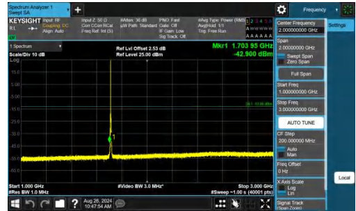
Band4-3MHz-QPSK-19965-1RB#0-1000~3000-PASS
