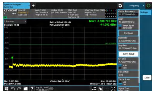
Band4-10MHz-QPSK-20350-1RB#49-3000~20000-PASS
