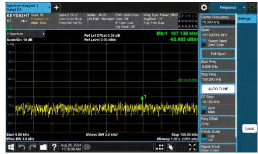
Band4-20MHz-QPSK-20050-1RB#99-0.009~0.15-PASS
