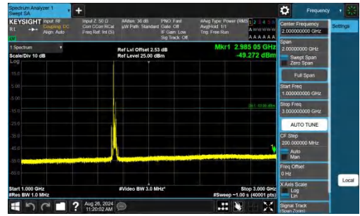
Band4-20MHz-QPSK-20175-1RB#0-1000~3000-PASS
