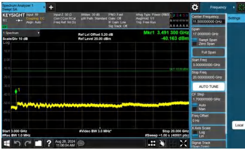
Band4-10MHz-QPSK-20350-1RB#0-3000~20000-PASS
