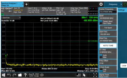
Band4-5MHz-QPSK-20175-1RB#24-0.15~30-PASS
