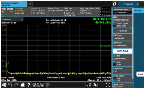
Band4-20MHz-QPSK-20300-1RB#99-0.15~30-PASS
