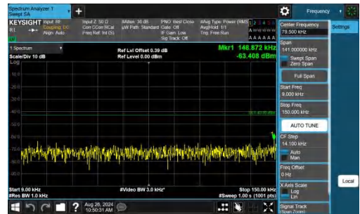
Band4-3MHz-QPSK-20385-1RB#14-0.009~0.15-PASS
