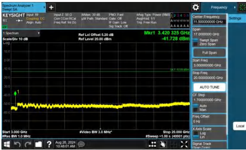
Band4-3MHz-QPSK-19965-1RB#0-3000~20000-PASS
