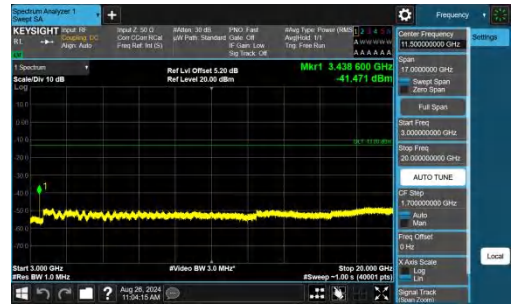
Band4-10MHz-QPSK-20000-1RB#49-3000~20000-PASS
