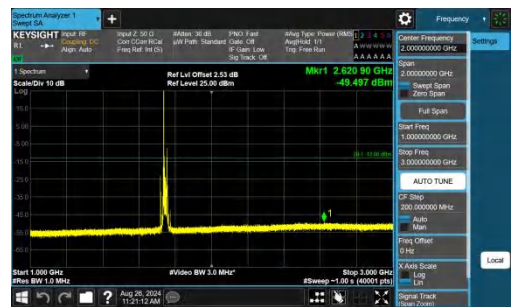
Band4-20MHz-QPSK-20300-1RB#0-1000~3000-PASS
