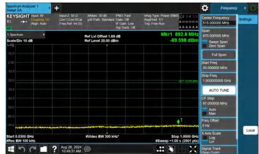
Band4-3MHz-QPSK-20175-1RB#14-30~1000-PASS
