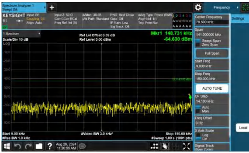
Band4-20MHz-QPSK-20300-1RB#0-0.009~0.15-PASS
