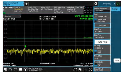
Band4-10MHz-QPSK-20000-1RB#49-0.009~0.15-PASS
