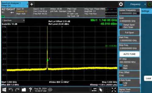
Band4-3MHz-QPSK-20175-1RB#14-1000~3000-PASS
