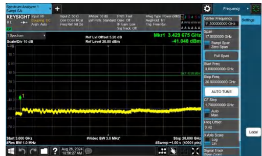
Band4-5MHz-QPSK-19975-1RB#24-3000~20000-PASS
