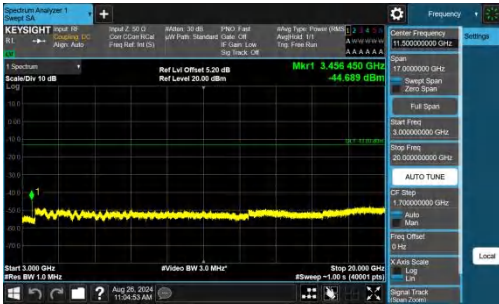
Band4-10MHz-QPSK-20175-1RB#0-3000~20000-PASS
