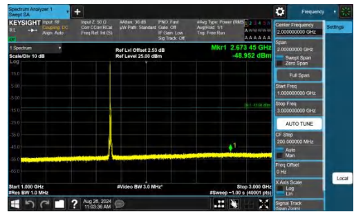
Band4-10MHz-QPSK-20000-1RB#0-1000~3000-PASS
