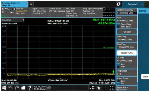
Band4-3MHz-QPSK-19965-1RB#0-30~1000-PASS
