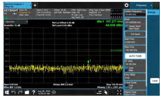
Band4-5MHz-QPSK-20375-1RB#24-0.009~0.15-PASS
