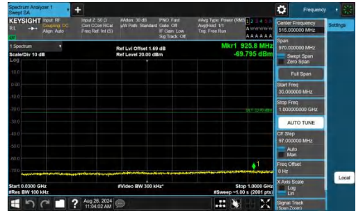
Band4-10MHz-QPSK-20000-1RB#49-30~1000-PASS
