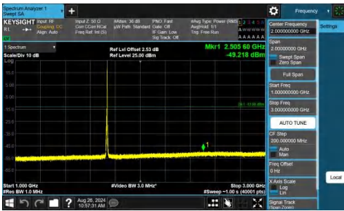
Band4-5MHz-QPSK-20175-1RB#24-1000~3000-PASS
