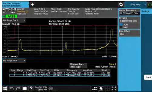
Band4-15MHz-QPSK-20025-1RB#74-PASS
