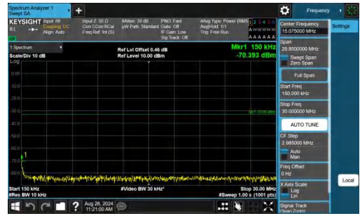
Band4-20MHz-QPSK-20300-1RB#0-0.15~30-PASS
