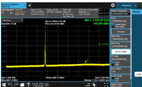
Band4-10MHz-QPSK-20350-1RB#49-1000~3000-PASS
