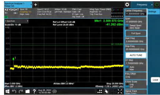
Band4-3MHz-QPSK-20385-1RB#14-3000~20000-PASS
