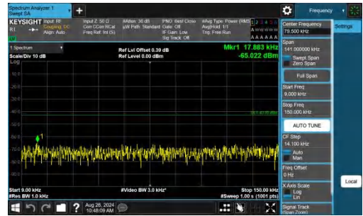
Band4-3MHz-QPSK-19965-1RB#14-0.009~0.15-PASS
