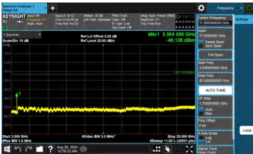
Band4-3MHz-QPSK-20385-1RB#0-3000~20000-PASS
