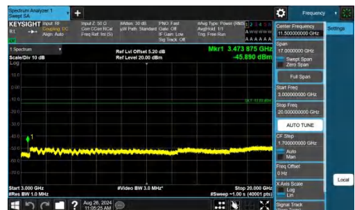
Band4-10MHz-QPSK-20175-1RB#49-3000~20000-PASS
