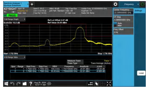
Band4-3MHz-QPSK-20385-1RB#14-PASS
