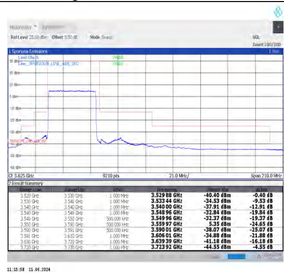
1-N48-30-40-L-3-DFT-PI2BPSK-Outer_Full-100@0-Ant0-1--PASS-see graph
