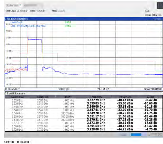
1-N48-30-20-L-3-DFT-PI2BPSK-Outer_Full-50@0-Ant0-1--PASS-see graph
