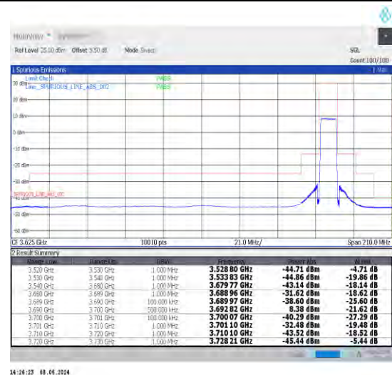
1-N48-30-10-H-6-CP-QPSK-Outer_Full-24@0-Ant 0-1--PASS-see graph
