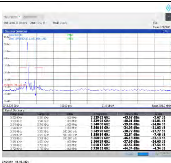
1-N48-30-10-L-1-DFT-PI2BPSK-Edge_1RB_Left-1@0-Ant0-1--PASS-see graph
