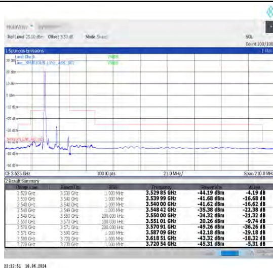
1-N48-30-20-L-4-CP-QPSK-Edge_1RB_Left-1@0-Ant0-1--PASS-see graph
