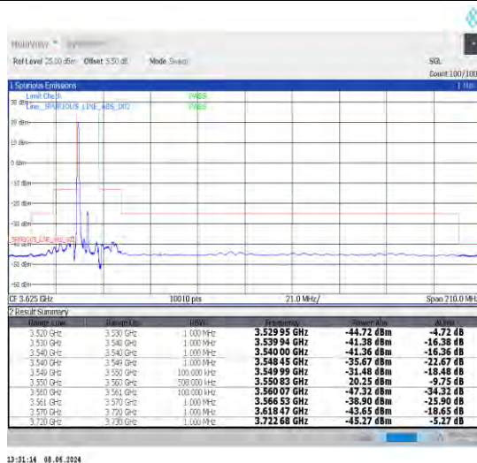
1-N48-30-10-L-4-CP-QPSK-Edge_1RB_Left-1@0-Ant0-1--PASS-see graph
