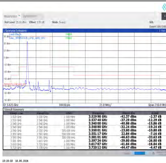
1-N48-30-30-L-1-DFT-PI2BPSK-Edge_1RB_Left-1@0-Ant0-1--PASS-see graph
