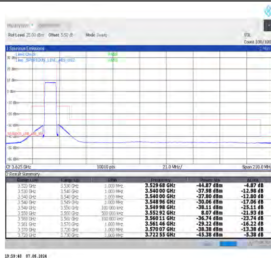
1-N48-30-10-L-6-CP-QPSK-Outer_Full-24@0-Ant0-1--PASS-see graph
