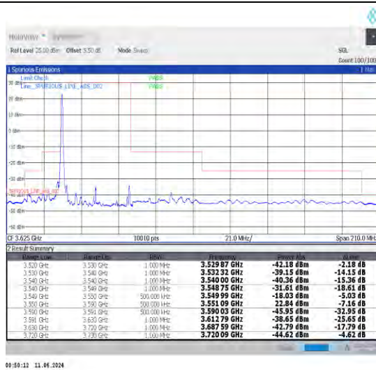
1-N48-30-40-L-1-DFT-PI2BPSK-Edge_1RB_Left-1@0-Ant0-1--PASS-see graph
