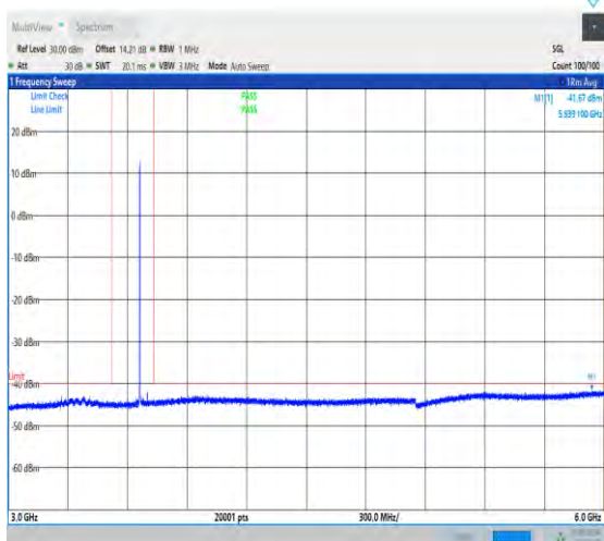
NTNV_N48_PC3_30_40_H_TID1_NS_01_3000_6000_#1
