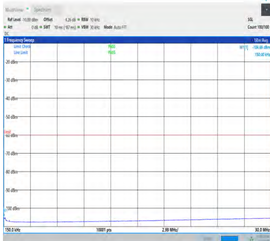
NTNV_N48_PC3_30_40_M_TID1_NS_01_0.15_30_#1
