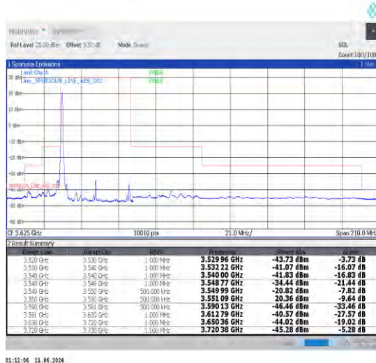
1-N48-30-40-L-4-CP-QPSK-Edge_1RB_Left-1@0-Ant0-1--PASS-see graph
