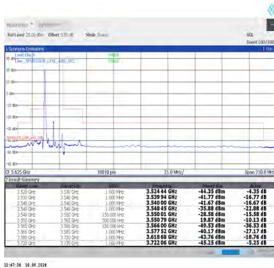
1-N48-30-15-L-4-CP-QPSK-Edge_1RB_Left-1@0-Ant0-1--PASS-see graph
