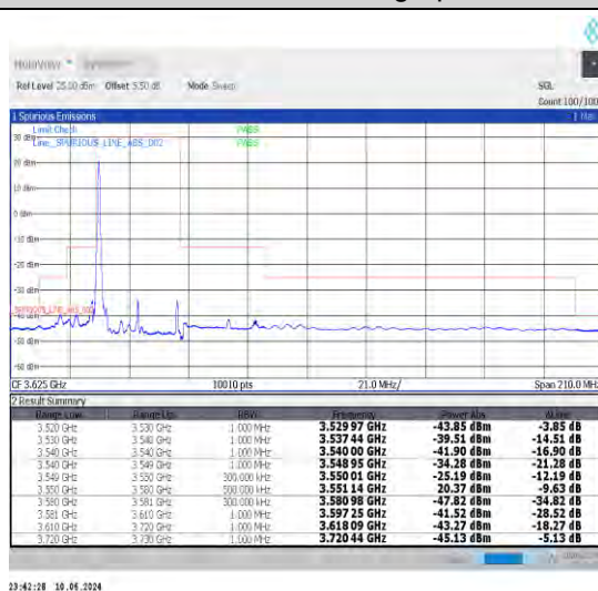
1-N48-30-30-L-4-CP-QPSK-Edge_1RB_Left-1@0-Ant0-1--PASS-see graph
