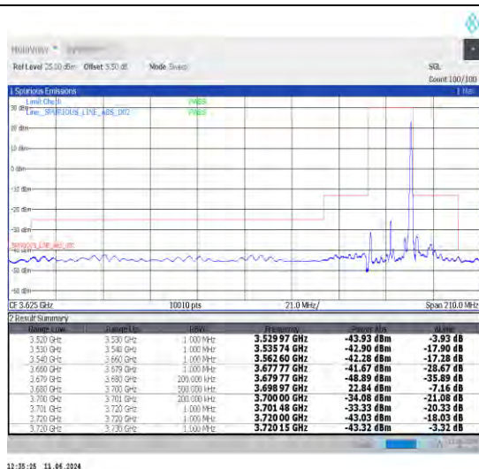
1-N48-30-20-H-2-DFT-PI2BPSK-Edge_1RB_Right-1@50-Ant0-1--PASS-see graph
