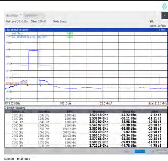
1-N48-30-15-L-3-DFT-PI2BPSK-Outer_Full-36@0-Ant0-1--PASS-see graph
