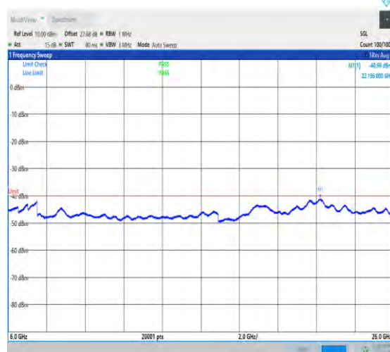
NTNV_N48_PC3_30_40_H_TID1_NS_01_6000_26000_#
