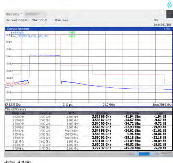
1-N48-30-40-L-6-CP-QPSK-Outer_Full-106@0-Ant0-1--PASS-see graph
