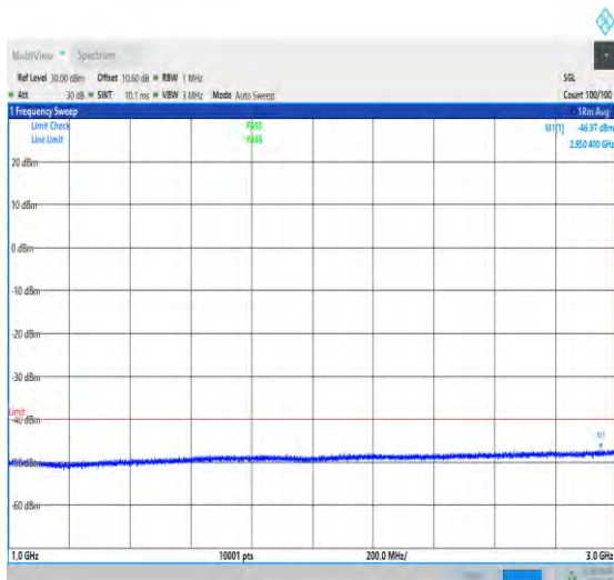
NTNV_N48_PC3_30_40_M_TID1_NS_01_1000_3000_#1
