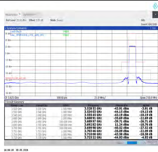
1-N48-30-10-H-3-DFT-PI2BPSK-Outer_Full-24@0 -Ant0-1--PASS-see graph
