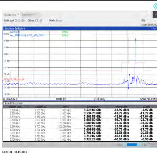
1-N48-30-10-H-2-DFT-PI2BPSK-Edge_1RB_Right-1@ 23-Ant0-1--PASS-see graph
