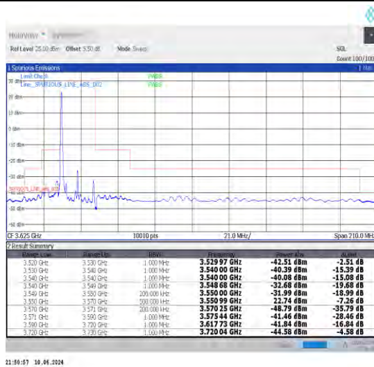
1-N48-30-20-L-1-DFT-PI2BPSK-Edge_1RB_Left-1@0-Ant0-1--PASS-see graph
