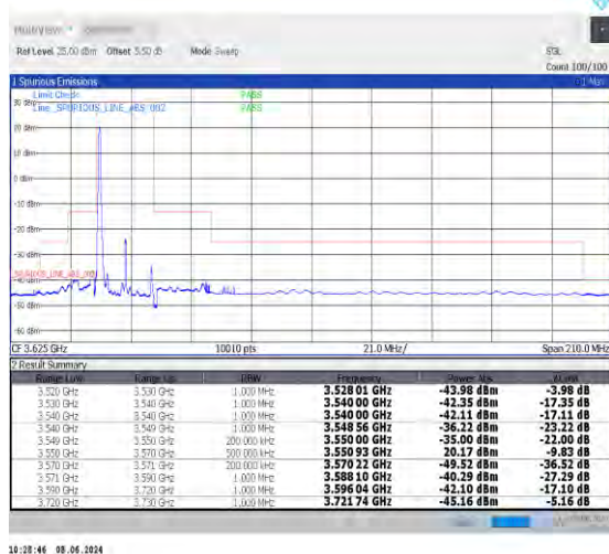
1-N48-30-20-L-4-CP-QPSK-Edge_1RB_Left-1@0-Ant0-1--PASS-see graph
