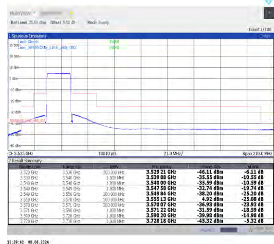
1-N48-30-20-L-6-CP-QPSK-Outer_Full-51@0-Ant0-1--PASS-see graph
