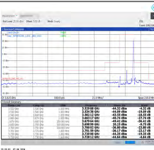
1-N48-30-20-H-5-CP-QPSK-Edge_1RB_Right-1@50-Ant0-1--PASS-see graph
