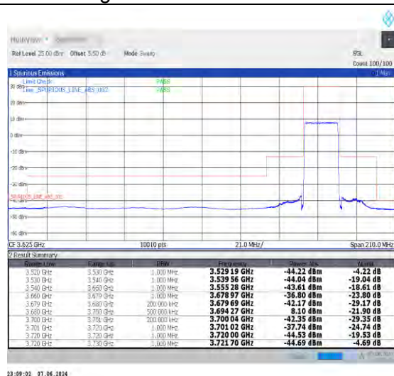
1-N48-30-20-H-3-DFT-PI2BPSK-Outer_Full-50@0-Ant0-1--PASS-see graph
