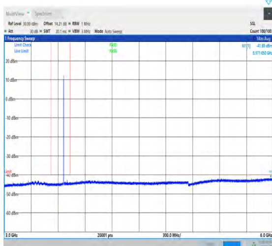
NTNV_N48_PC3_30_40_H_TID1_NS_01_3000_6000_#1
