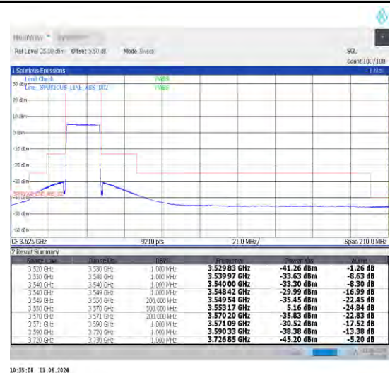
1-N48-30-20-L-6-CP-QPSK-Outer_Full-51@0-Ant0-1--PASS-see graph
