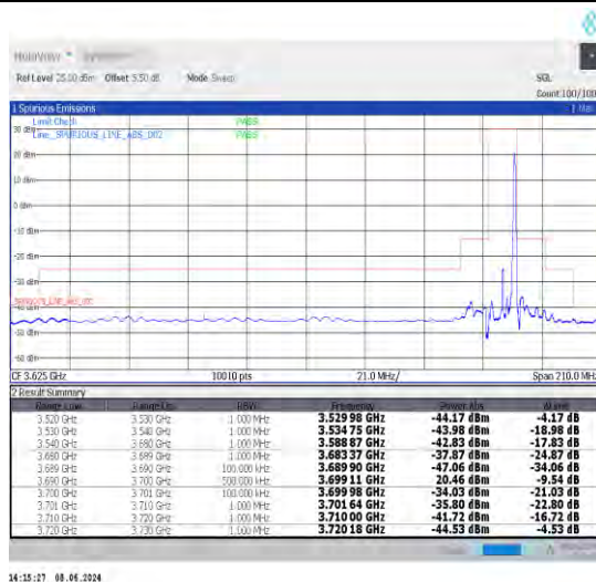
1-N48-30-10-H-5-CP-QPSK-Edge_1RB_Right-1@23-A nt0-1--PASS-see graph
