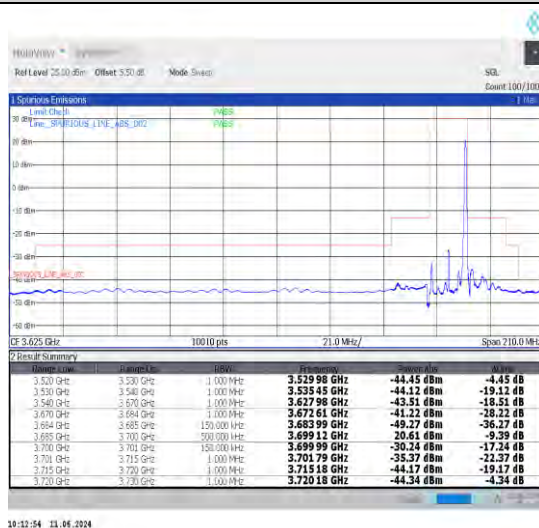
1-N48-30-15-H-5-CP-QPSK-Edge_1RB_Right-1@37-A nt0-1--PASS-see graph
