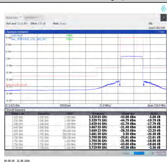
1-N48-30-30-H-6-CP-QPSK-Outer_Full-78@0-Ant0-1--PASS-see graph
