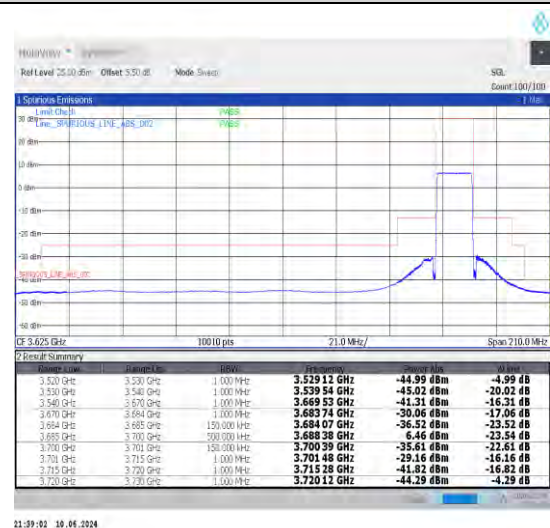
1-N48-30-15-H-6-CP-QPSK-Outer_Full-38@0-Ant 0-1--PASS-see graph
