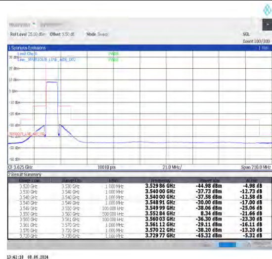
1-N48-30-10-L-6-CP-QPSK-Outer_Full-24@0-Ant0-1--PASS-see graph
