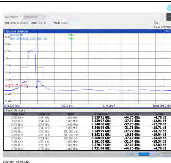
1-N48-30-10-L-3-DFT-PI2BPSK-Outer_Full-24@0-Ant0-1--PASS-see graph
