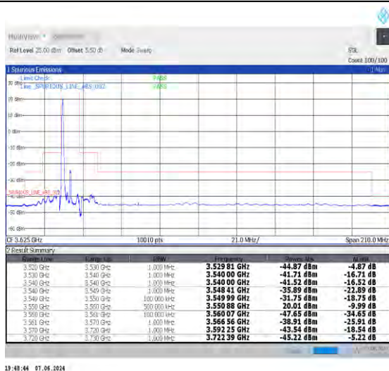
1-N48-30-10-L-4-CP-QPSK-Edge_1RB_Left-1@0-Ant0-1--PASS-see graph
