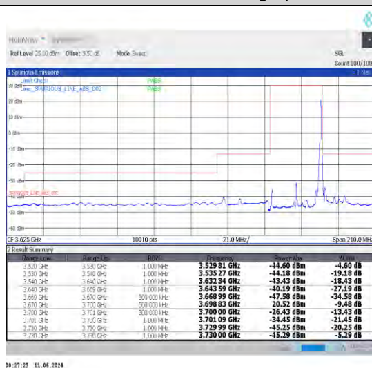
1-N48-30-30-H-5-CP-QPSK-Edge_1RB_Right-1@77-Ant0-1--PASS-see graph
