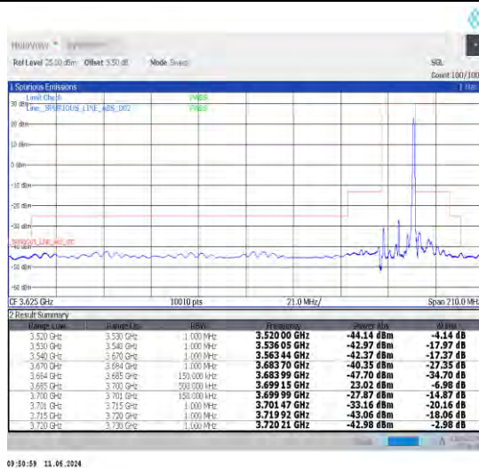
1-N48-30-15-H-2-DFT-PI2BPSK-Edge_1RB_Right-1@ 37-Ant0-1--PASS-see graph
