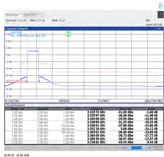
1-N48-30-15-L-6-CP-QPSK-Outer_Full-38@0-Ant0-1--PASS-see graph
