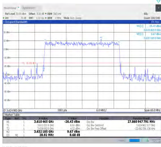
1-N48-30-30-M-6-CP-QPSK-Outer_Full-78@0-Ant0 27.861-28.920-≤30-PASS
