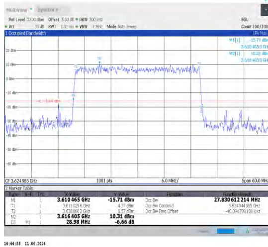
1-N48-30-30-M-7-CP-16QAM-Outer_Full-78@0-Ant0 -27.831-28.980-≤30-PASS
