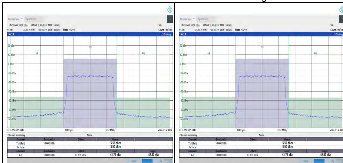
NTNV_N48_PC3_30_10_L_TID4_#1_-10_10
