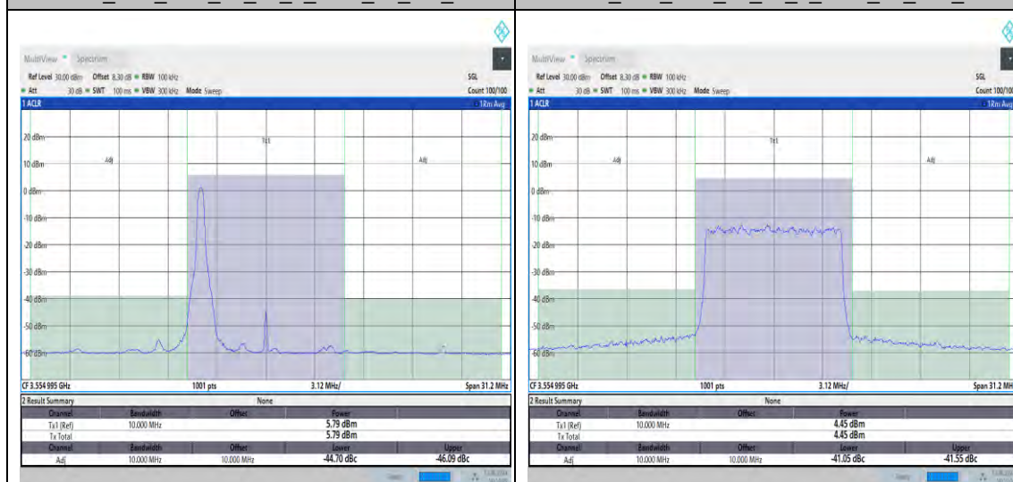
NTNV_N48_PC3_30_10_L_TID5_#1_-10_10
