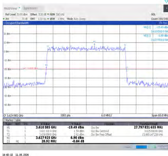
1-N48-30-30-M-9-CP-256QAM-Outer_Full-78@0-Ant0 0-27.8-28.920-≤30-PASS
