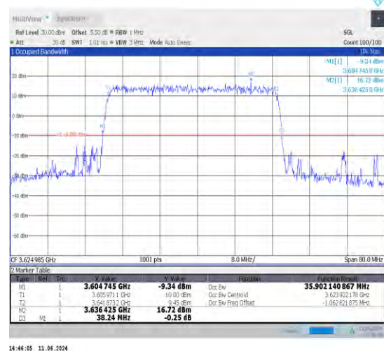
1-N48-30-40-M-1-DFT-QPSK-Outer_Full-100@0-Ant0 0-35.902-38.240-≤40-PASS
