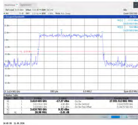
1-N48-30-30-M-8-CP-64QAM-Outer_Full-78@0-Ant0 0-27.937-28.980-≤30-PASS
