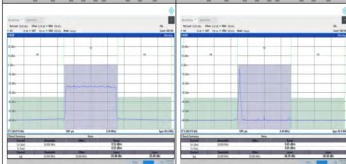
NTNV_N48_PC3_30_30_L_TID25_#1_-30_30
