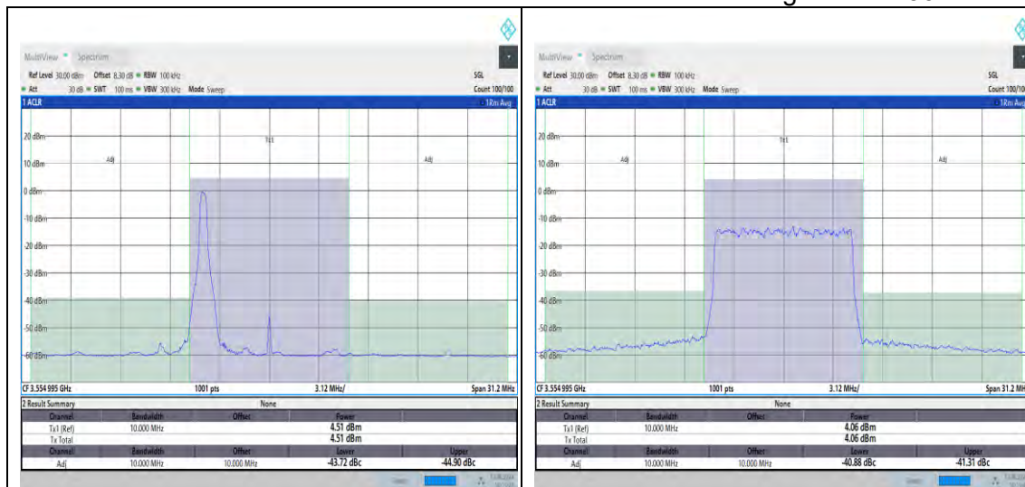
NTNV_N48_PC3_30_10_L_TID8_#1_-10_10
