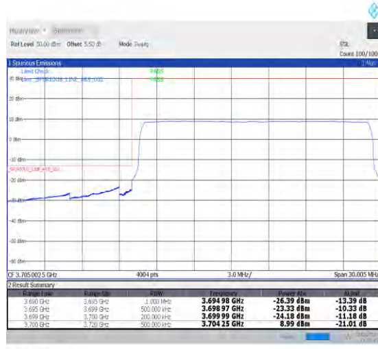
1-N78-3700-3800-PC2-30-20-L-6-CP-QPSK-Outer_Full-51@0-Ant0-1--PASS-see graph
