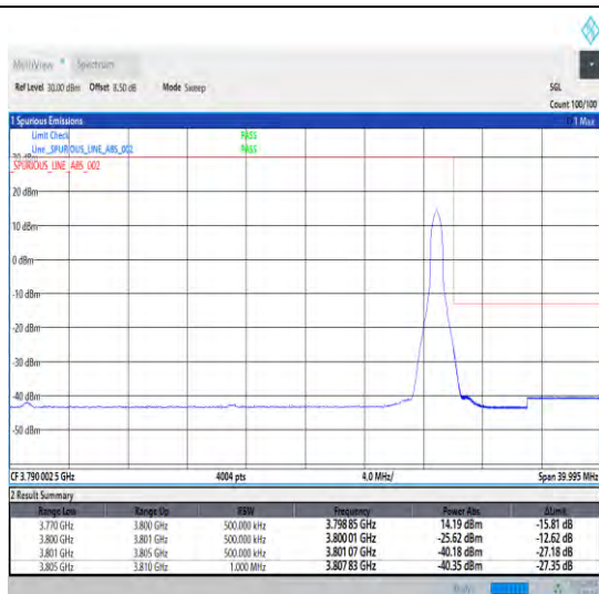
1-N78-3700-3800-30-30-H-2-DFT-PI2BPSK-Edge_1R_B_Right-1@77-Ant0-1--PASS-see graph
