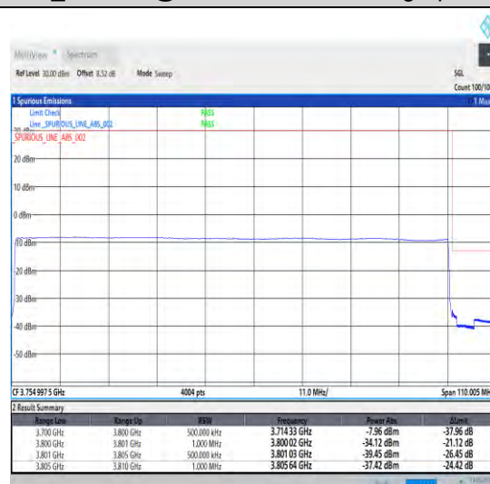
1-N78-3700-3800-30-100-H-6-CP-QPSK-Outer_Full-273@0-Ant0-1--PASS-see graph
