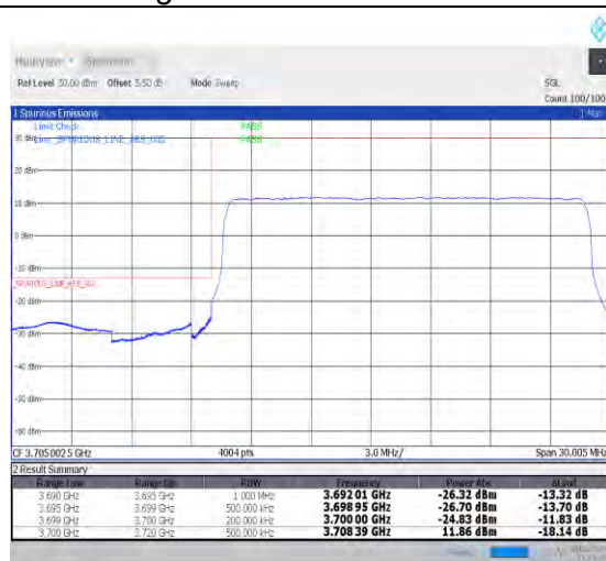
1-N78-3700-3800-PC2-30-20-L-3-DFT-PI2BPSK-Outer_Full-50@0-Ant0-1--PASS-see graph
