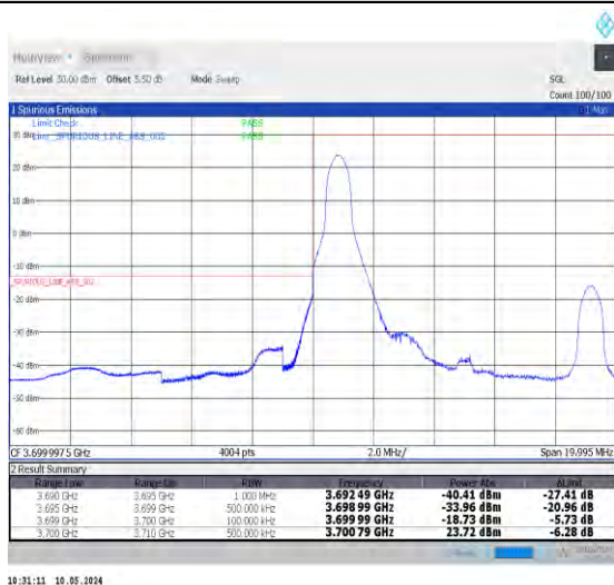
1-N78-3700-3800-PC2-30-10-L-4-CP-QPSK-Edge_1RB_Left-1@0-Ant0-1--PASS-see graph
