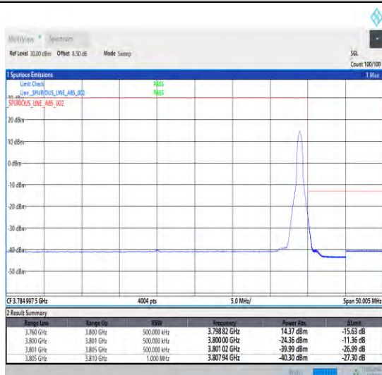
1-N78-3700-3800-30-40-H-5-CP-QPSK-Edge_1RB_Ri ght-1@105-Ant0-1--PASS-see graph
