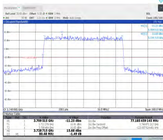
1-N78-3700-3800-PC2-30-80-M-4-DFT-64QAM-Out er_Full-216@0-Ant0-77.185-80.480-≤80-PASS
