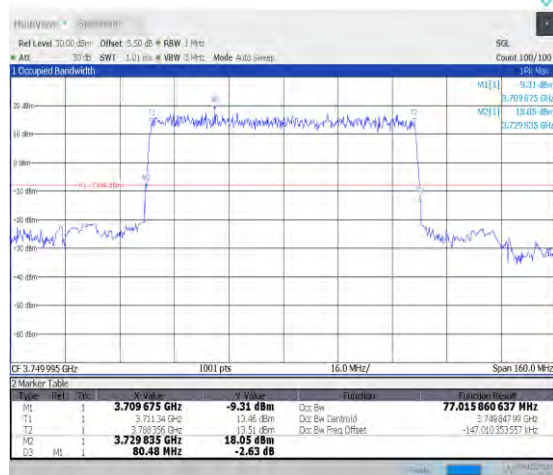
1-N78-3700-3800-PC2-30-80-M-2-DFT-PI2BPSK-Out er_Full-216@0-Ant0-77.016-80.480-≤80-PASS
