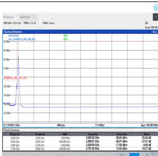
1-N78-3700-3800-30-100-L-1-DFT-PI2BPSK-Edge_1R B_Left-1@0-Ant0-1--PASS-see graph
