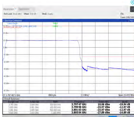
1-N78-3700-3800-PC2-30-15-H-6-CP-QPSK-Outer_Full-38@0-Ant0-1--PASS-see graph
