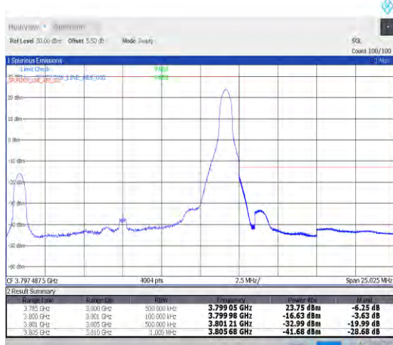
1-N78-3700-3800-PC2-30-15-H-5-CP-QPSK-Edge_1R_B_Right-1@37-Ant0-1--PASS-see graph
