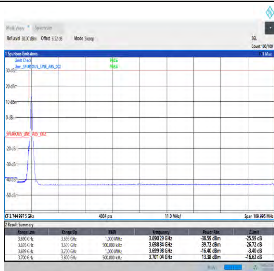
1-N78-3700-3800-30-100-L-4-CP-QPSK-Edge_1RB_Left-1@0-Ant0-1--PASS-see graph
