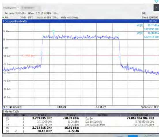
1-N78-3700-3800-PC2-30-80-M-3-DFT-16QAM-Out er_Full-216@0-Ant0-77.069-80.160-≤80-PASS
