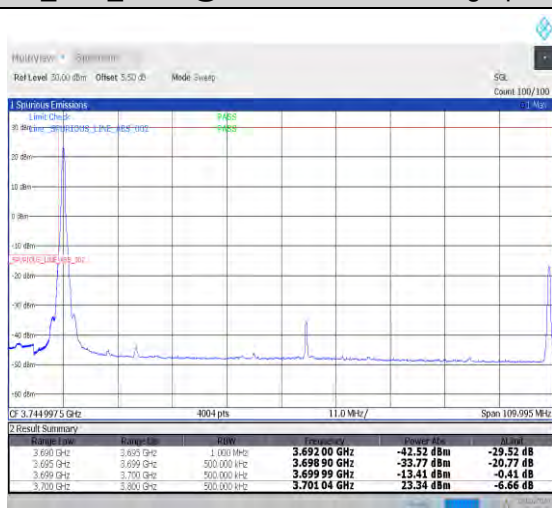
1-N78-3700-3800-PC2-30-100-L-1-DFT-PI2BPSK-Edge_1RB_Left-1@0-Ant0-1--PASS-see graph
