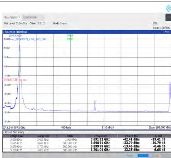
1-N78-3700-3800-PC2-30-100-L-1-DFT-PI2BPSK-Edge_1RB_Left-1@0-Ant0-1--PASS-see graph
