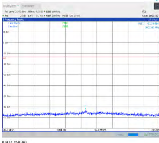
1-N78-3700-3800-PC2-30-100-L-1-DFT-PI2BPSK-In ner_1RB_Left-1@1-30-1000-Ant0-542.16--62.58--13 -PASS
