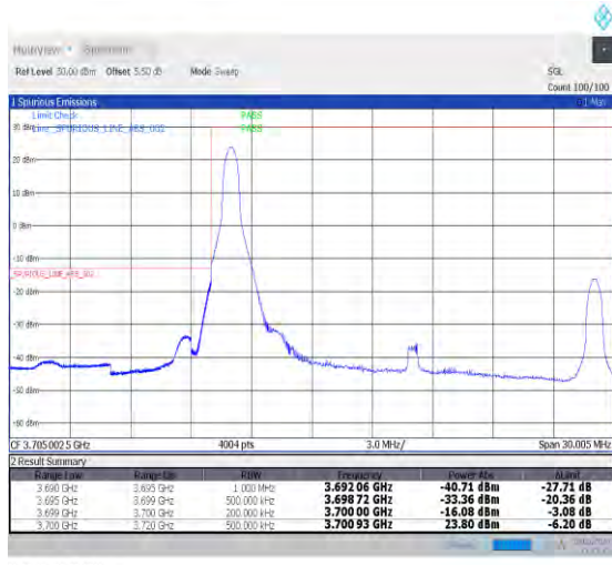
1-N78-3700-3800-PC2-30-20-L-4-CP-QPSK-Edge_1RB_Left-1@0-Ant0-1--PASS-see graph
