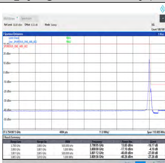
1-N78-3700-3800-30-100-H-5-CP-QPSK-Edge_1RB_Right-1@272-Ant0-1--PASS-see graph
