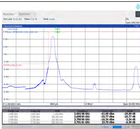
1-N78-3700-3800-PC2-30-20-L-1-DFT-PI2BPSK-Edge_1RB_Left-1@0-Ant0-1--PASS-see graph
