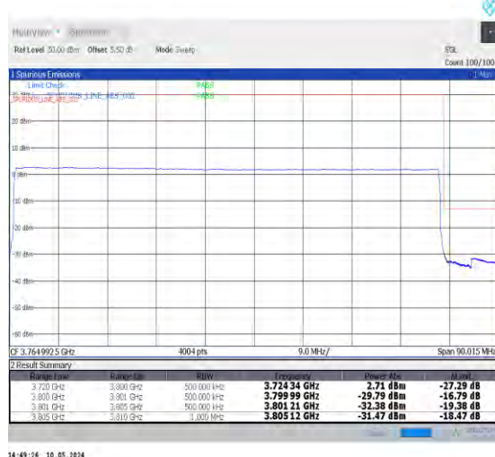
1-N78-3700-3800-PC2-30-80-H-6-CP-QPSK-Outer_Full-217@0-Ant0-1--PASS-see graph
