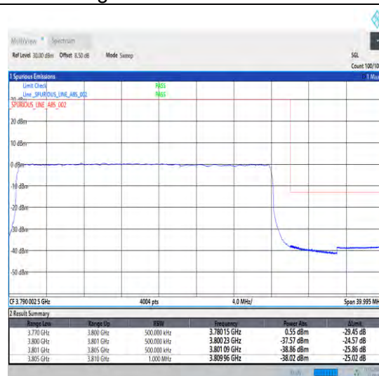
1-N78-3700-3800-30-30-H-3-DFT-PI2BPSK-Outer_Full-75@0-Ant0-1--PASS-see graph
