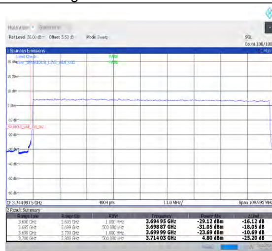
1-N78-3700-3800-PC2-30-100-L-3-DFT-PI2BPSK-Outer_Full-270@0-Ant0-1--PASS-see graph
