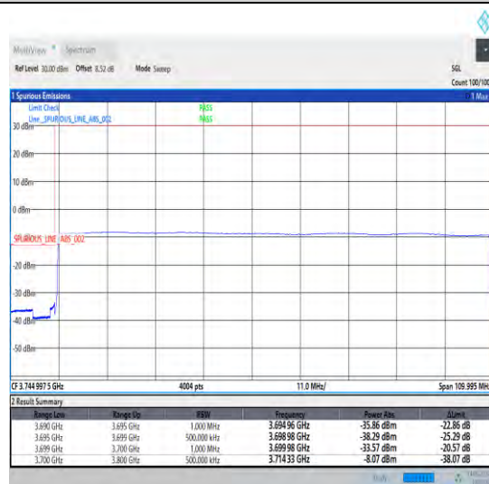
1-N78-3700-3800-30-100-L-6-CP-QPSK-Outer_Full-273@0-Ant0-1--PASS-see graph
