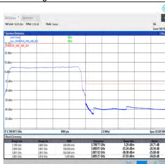
1-N78-3700-3800-30-10-H-3-DFT-PI2BPSK-Outer_Full-24@0-Ant0-1--PASS-see graph
