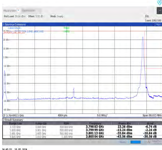
1-N78-3700-3800-PC2-30-80-H-5-CP-QPSK-Edge_1RB_Right-1@216-Ant0-1--PASS-see graph
