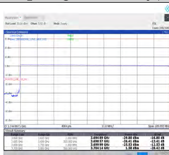
1-N78-3700-3800-PC2-30-100-L-3-DFT-PI2BPSK-Outer_Full-270@0-Ant0-1--PASS-see graph
