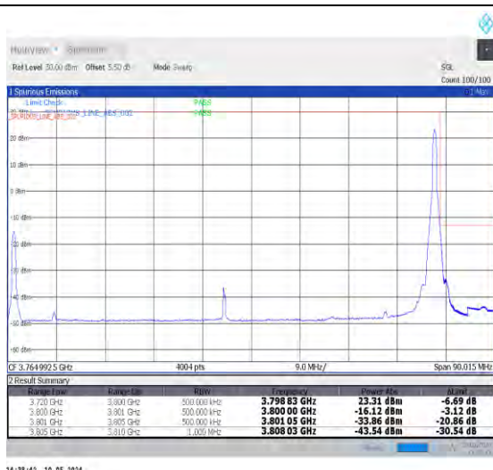
1-N78-3700-3800-PC2-30-80-H-2-DFT-PI2BPSK-Edge_1RB_Right-1@216-Ant0-1--PASS-see graph
