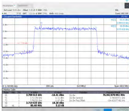
1-N78-3700-3800-PC2-30-80-M-1-DFT-QPSK-Out _Full-216@0-Ant0-76.943-80.480-≤80-PASS
