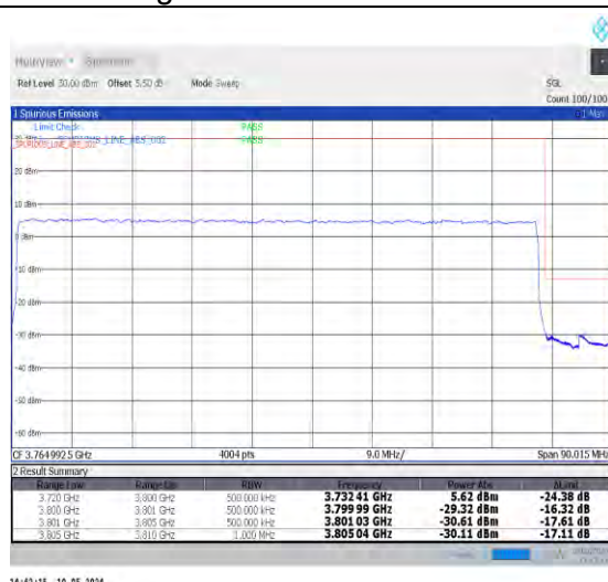
1-N78-3700-3800-PC2-30-80-H-3-DFT-PI2BPSK-Outer_Full-216@0-Ant0-1--PASS-see graph
