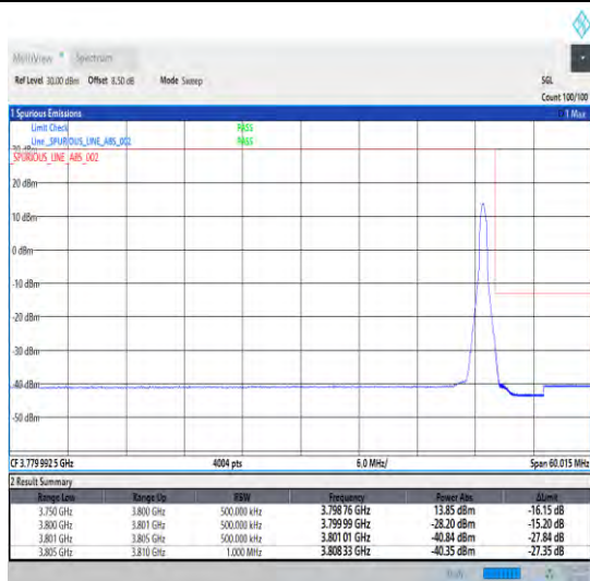
1-N78-3700-3800-30-50-H-5-CP-QPSK-Edge_1RB_Ri ght-1@132-Ant0-1--PASS-see graph
