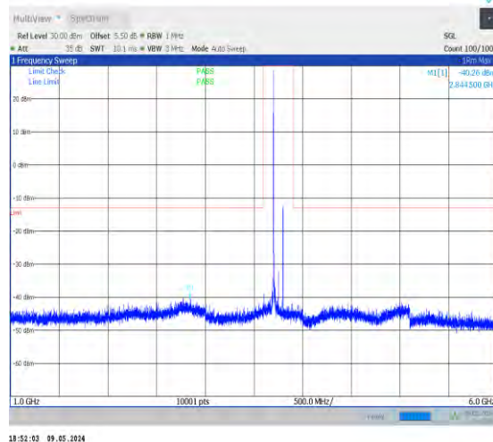
1-N78-3700-3800-PC2-30-100-L-1-DFT-PI2BPSK-In ner_1RB_Left-1@1-1000-6000-Ant0-2844.50--40.26- -13-PASS
