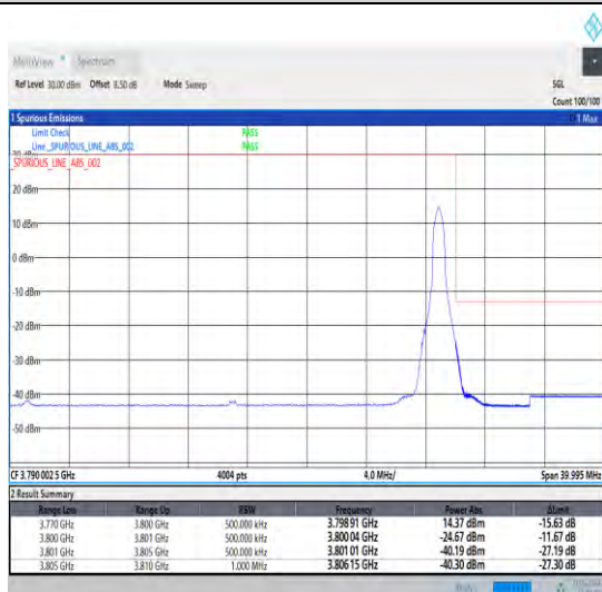
1-N78-3700-3800-30-30-H-5-CP-QPSK-Edge_1RB_Right-1@77-Ant0-1--PASS-see graph
