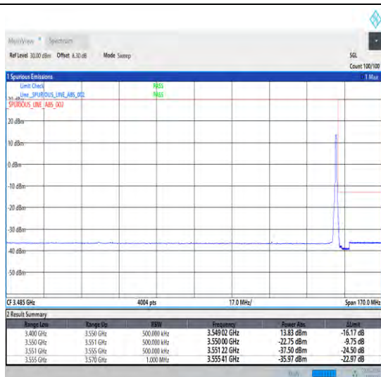
1-N78-3450-3550-30-60-H-2-DFT-PI2BPSK-Edge_1R B_Right-1@161-Ant0-1--PASS-see graph
