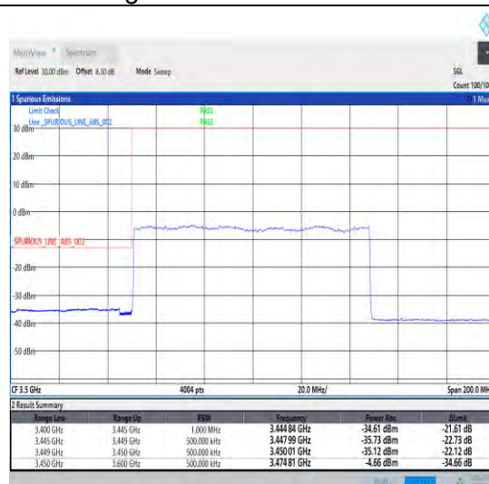
1-N78-3450-3550-30-100-L-3-DFT-PI2BPSK-Outer_Full-270@0-Ant0-1--PASS-see graph
