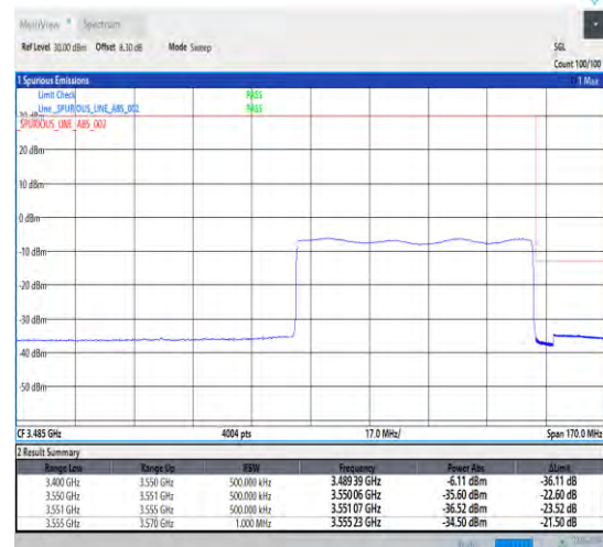
1-N78-3450-3550-30-70-H-6-CP-QPSK-Outer_Full -189@0-Ant0-1--PASS-see graph
