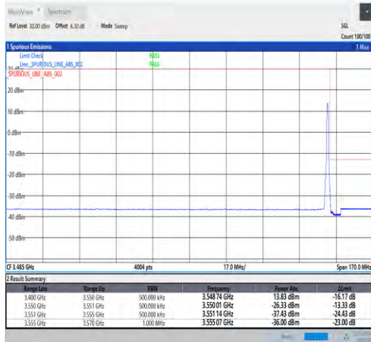
1-N78-3450-3550-30-70-H-2-DFT-PI2BPSK-Edge_1R B_Right-1@188-Ant0-1--PASS-see graph
