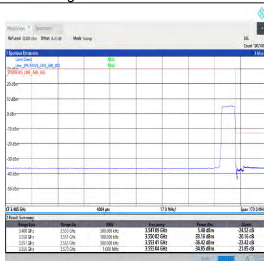
1-N78-3450-3550-30-10-H-3-DFT-PI2BPSK-Outer_Full-24@0-Ant0-1--PASS-see graph
