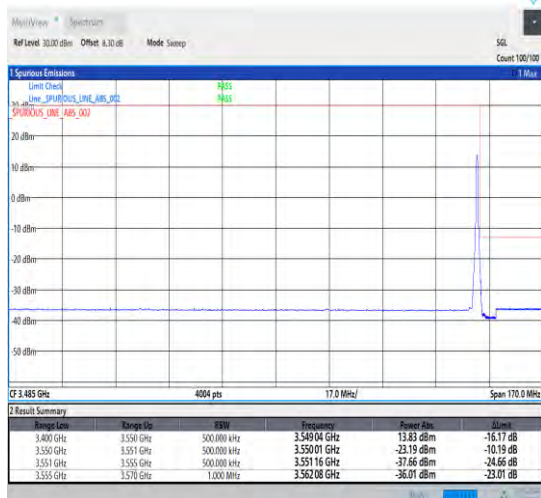
1-N78-3450-3550-30-100-H-2-DFT-PI2BPSK-Edge_1R_B_Right-1@272-Ant0-1--PASS-see graph
