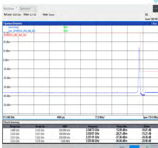
1-N78-3450-3550-30-50-H-5-CP-QPSK-Edge_1RB_Ri ght-1@132-Ant0-1--PASS-see graph
