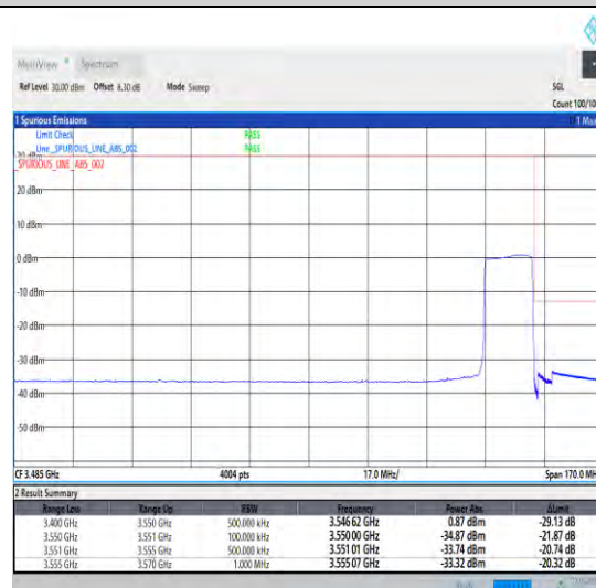
1-N78-3450-3550-30-15-H-6-CP-QPSK-Outer_Full-38@0-Ant0-1--PASS-see graph
