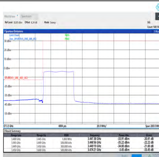
1-N78-3450-3550-30-40-L-6-CP-QPSK-Outer_Full -106@0-Ant0-1--PASS-see graph
