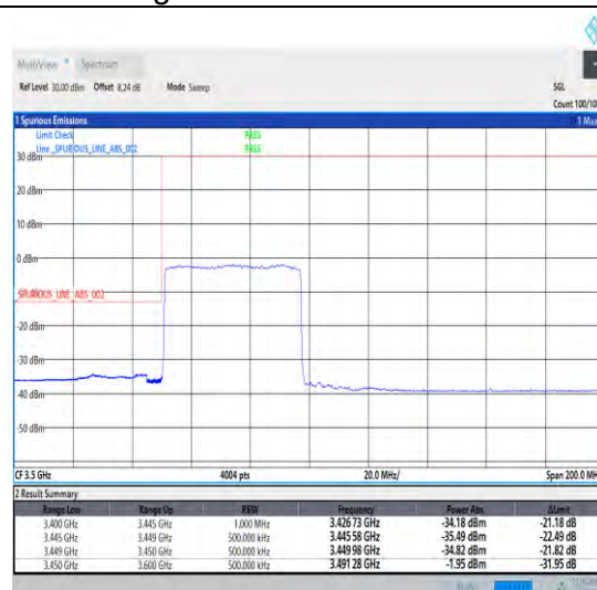
1-N78-3450-3550-30-50-L-3-DFT-PI2BPSK-Outer _Full-128@0-Ant0-1--PASS-see graph
