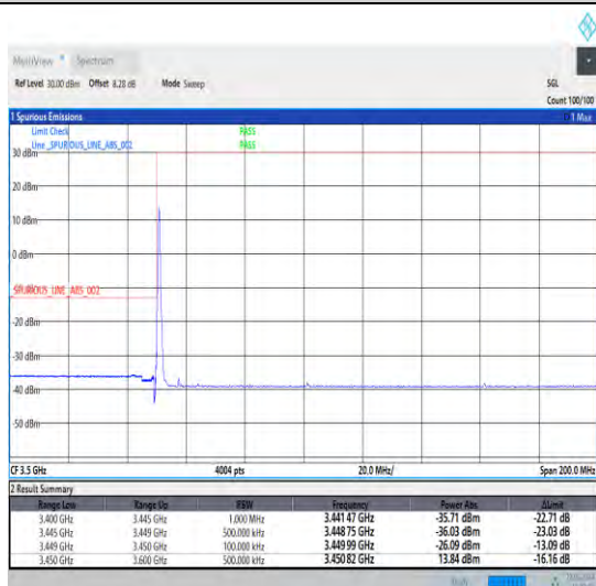
1-N78-3450-3550-30-15-L-4-CP-QPSK-Edge_1RB_Lef t-1@0-Ant0-1--PASS-see graph
