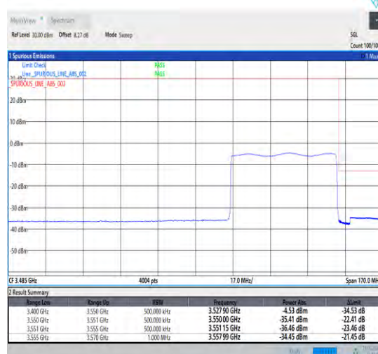
1-N78-3450-3550-30-50-H-6-CP-QPSK-Outer_Full -133@0-Ant0-1--PASS-see graph
