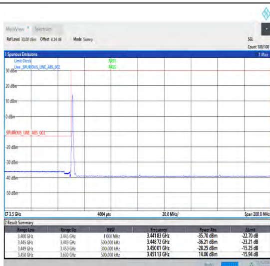
1-N78-3450-3550-30-40-L-1-DFT-PI2BPSK-Edge_1RB _Left-1@0-Ant0-1--PASS-see graph
