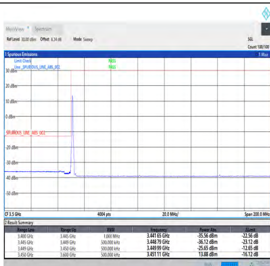
1-N78-3450-3550-30-80-L-1-DFT-PI2BPSK-Edge_1RB _Left-1@0-Ant0-1--PASS-see graph
