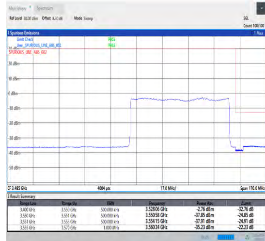
1-N78-3450-3550-30-70-H-3-DFT-PI2BPSK-Outer _Full-180@0-Ant0-1--PASS-see graph
