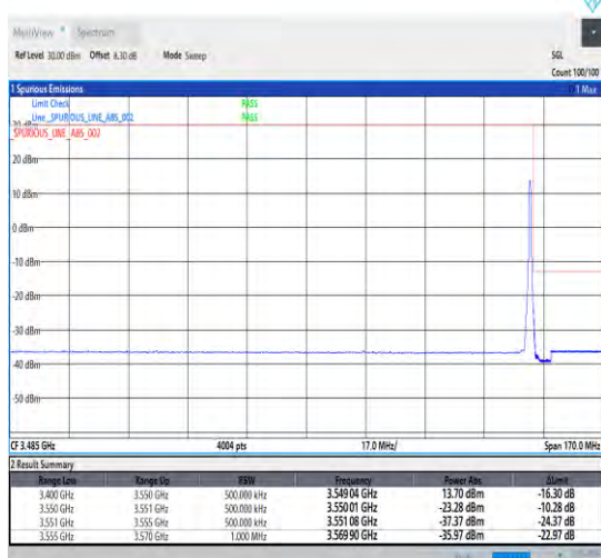
1-N78-3450-3550-30-100-H-5-CP-QPSK-Edge_1RB_Right-1@272-Ant0-1--PASS-see graph
