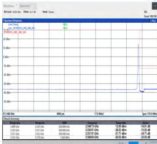
1-N78-3450-3550-30-50-H-2-DFT-PI2BPSK-Edge_1R B_Right-1@132-Ant0-1--PASS-see graph
