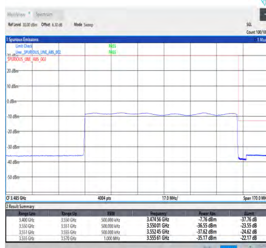
1-N78-3450-3550-30-100-H-6-CP-QPSK-Outer_Full-273@0-Ant0-1--PASS-see graph
