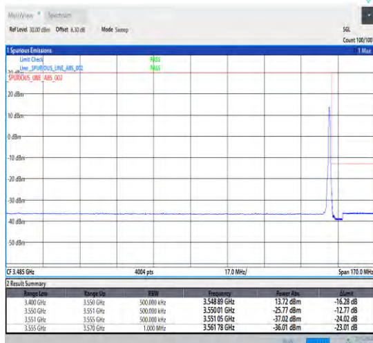
1-N78-3450-3550-30-70-H-5-CP-QPSK-Edge_1RB_Ri ght-1@188-Ant0-1--PASS-see graph
