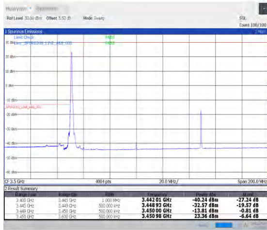
1-N78-3450-3550-PC2-30-100-L-1-DFT-PI2BPSK-Edge_1RB_Left-1@0-Ant0-1--PASS-see graph
