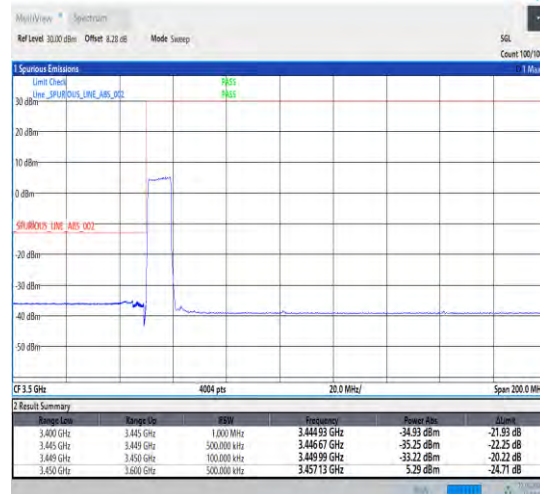
1-N78-3450-3550-30-10-L-3-DFT-PI2BPSK-Outer _Full-24@0-Ant0-1--PASS-see graph
