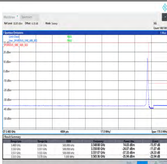
1-N78-3450-3550-30-80-H-5-CP-QPSK-Edge_1RB_Ri ght-1@216-Ant0-1--PASS-see graph
