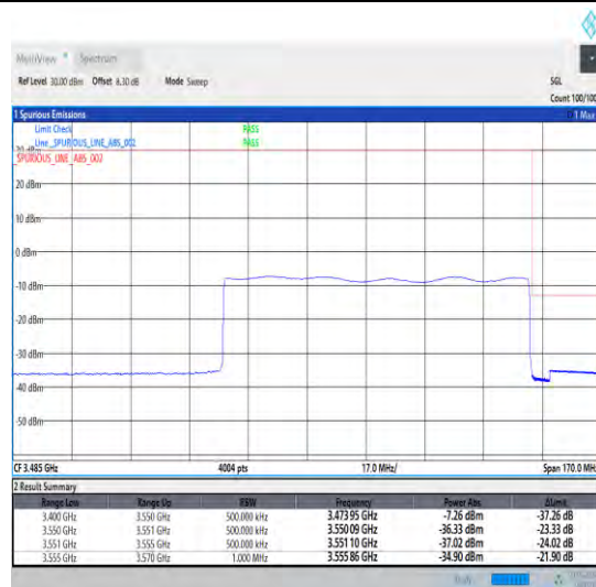
1-N78-3450-3550-30-90-H-6-CP-QPSK-Outer_Full -245@0-Ant0-1--PASS-see graph
