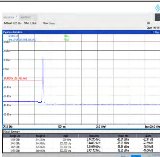
1-N78-3450-3550-30-90-L-4-CP-QPSK-Edge_1RB_Lef t-1@0-Ant0-1--PASS-see graph
