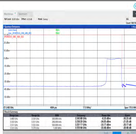
1-N78-3450-3550-30-20-H-6-CP-QPSK-Outer_Full-51@0-Ant0-1--PASS-see graph
