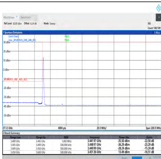
1-N78-3450-3550-30-50-L-1-DFT-PI2BPSK-Edge_1RB _Left-1@0-Ant0-1--PASS-see graph
