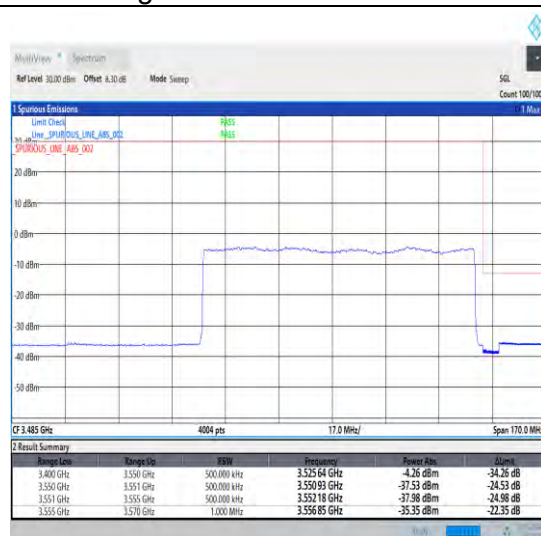
1-N78-3450-3550-30-90-H-3-DFT-PI2BPSK-Outer _Full-240@0-Ant0-1--PASS-see graph
