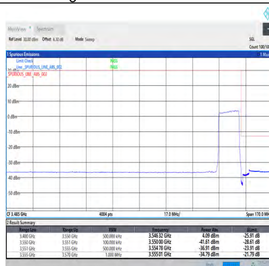
1-N78-3450-3550-30-15-H-3-DFT-PI2BPSK-Outer_Full-36@0-Ant0-1--PASS-see graph
