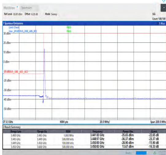
1-N78-3450-3550-30-10-L-4-CP-QPSK-Edge_1RB_Lef t-1@0-Ant0-1--PASS-see graph
