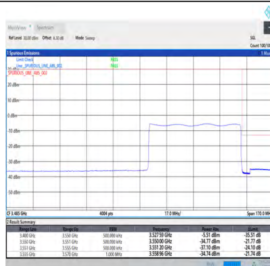
1-N78-3450-3550-30-60-H-6-CP-QPSK-Outer_Full -162@0-Ant0-1--PASS-see graph
