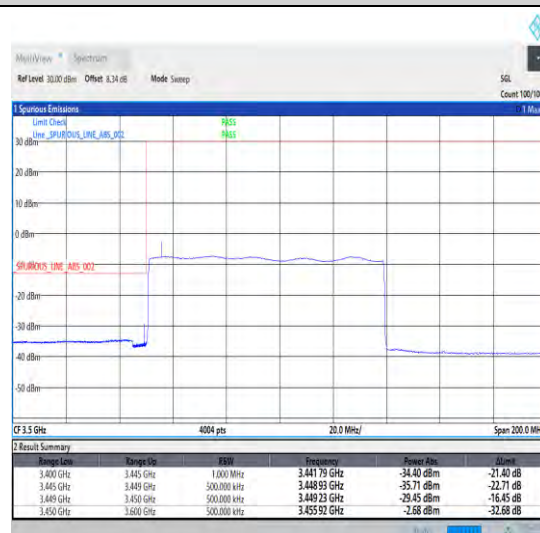
1-N78-3450-3550-30-90-L-6-CP-QPSK-Outer_Full -245@0-Ant0-1--PASS-see graph
