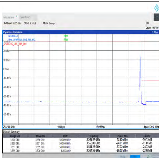
1-N78-3450-3550-30-90-H-2-DFT-PI2BPSK-Edge_1R B_Right-1@244-Ant0-1--PASS-see graph
