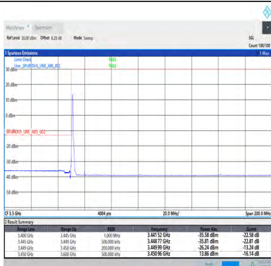
1-N78-3450-3550-30-20-L-4-CP-QPSK-Edge_1RB_Lef t-1@0-Ant0-1--PASS-see graph
