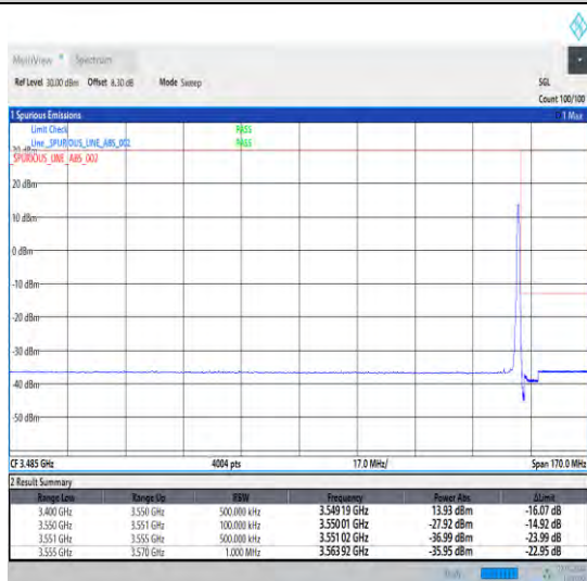
1-N78-3450-3550-30-10-H-5-CP-QPSK-Edge_1RB_Right-1@23-Ant0-1--PASS-see graph
