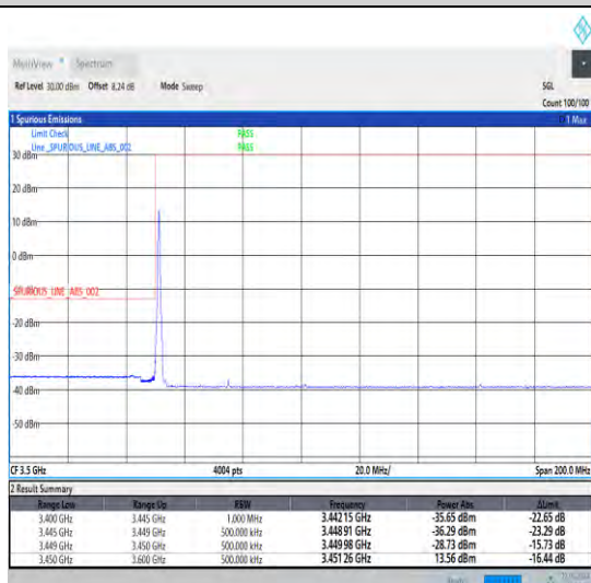
1-N78-3450-3550-30-50-L-4-CP-QPSK-Edge_1RB_Lef t-1@0-Ant0-1--PASS-see graph
