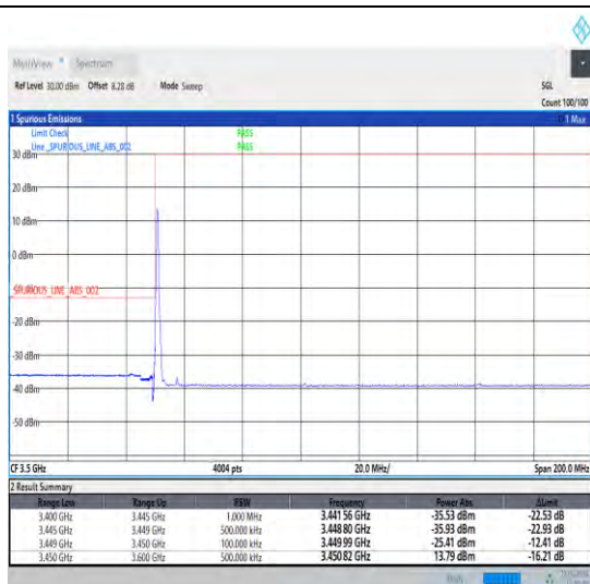
1-N78-3450-3550-30-15-L-1-DFT-PI2BPSK-Edge_1RB_Left-1@0-Ant0-1--PASS-see graph
