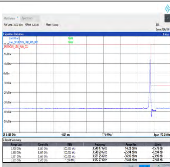
1-N78-3450-3550-30-15-H-5-CP-QPSK-Edge_1RB_Right-1@37-Ant0-1--PASS-see graph
