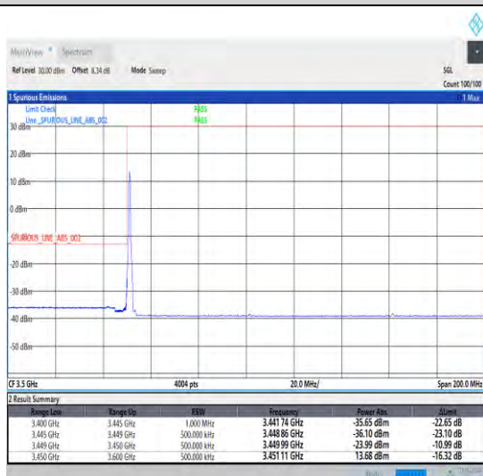
1-N78-3450-3550-30-80-L-4-CP-QPSK-Edge_1RB_Lef t-1@0-Ant0-1--PASS-see graph
