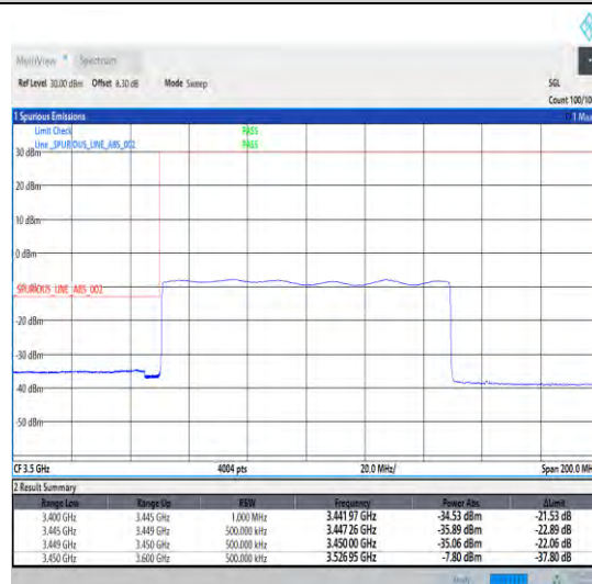
1-N78-3450-3550-30-100-L-6-CP-QPSK-Outer_Full-273@0-Ant0-1--PASS-see graph
