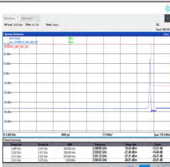
1-N78-3450-3550-30-40-H-5-CP-QPSK-Edge_1RB_Ri ght-1@105-Ant0-1--PASS-see graph
