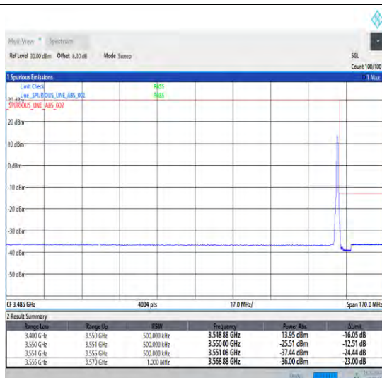
1-N78-3450-3550-30-80-H-2-DFT-PI2BPSK-Edge_1R B_Right-1@216-Ant0-1--PASS-see graph
