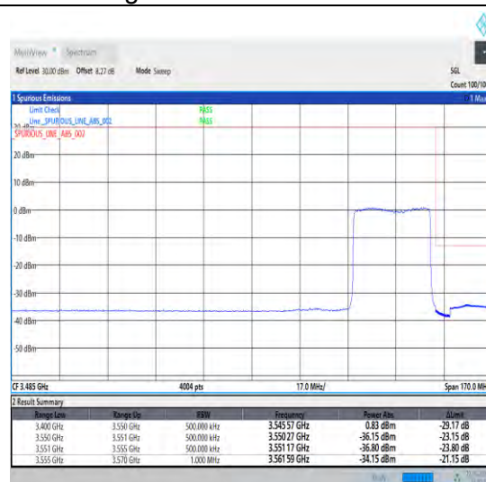
1-N78-3450-3550-30-30-H-3-DFT-PI2BPSK-Outer_Full-75@0-Ant0-1--PASS-see graph
