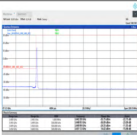
1-N78-3450-3550-30-30-L-4-CP-QPSK-Edge_1RB_Lef t-1@0-Ant0-1--PASS-see graph
