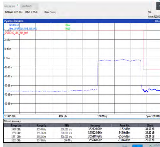
1-N78-3450-3550-30-50-H-3-DFT-PI2BPSK-Outer _Full-128@0-Ant0-1--PASS-see graph
