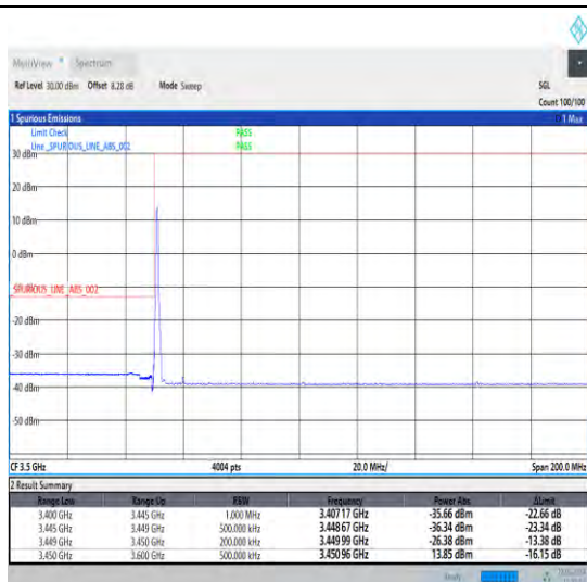
1-N78-3450-3550-30-20-L-1-DFT-PI2BPSK-Edge_1RB _Left-1@0-Ant0-1--PASS-see graph
