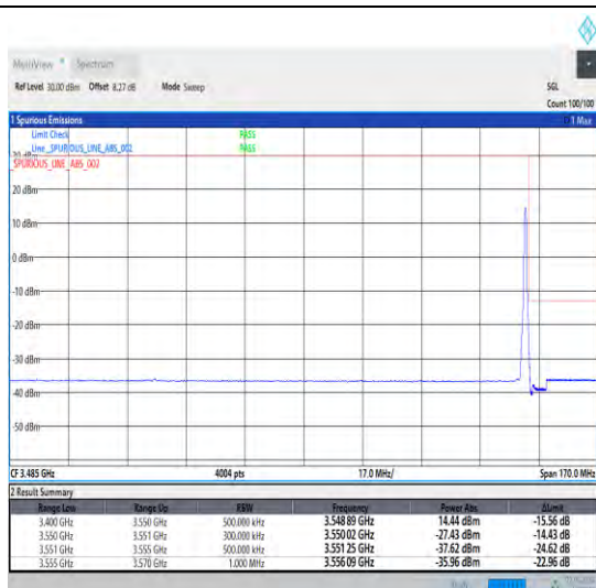
1-N78-3450-3550-30-40-H-2-DFT-PI2BPSK-Edge_1R B_Right-1@105-Ant0-1--PASS-see graph
