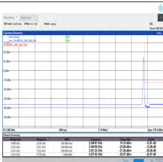
1-N78-3450-3550-30-30-H-2-DFT-PI2BPSK-Edge_1R_B_Right-1@77-Ant0-1--PASS-see graph
