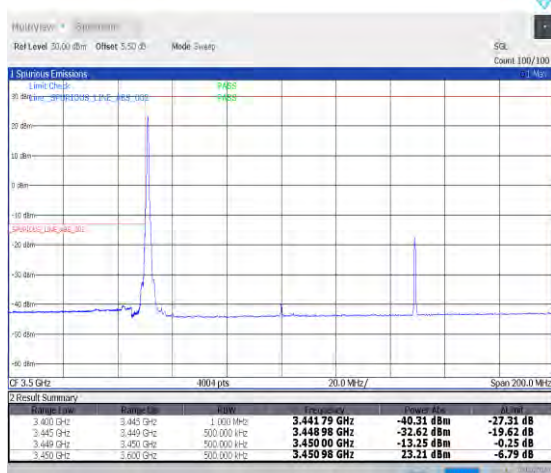
1-N78-3450-3550-PC2-30-100-L-4-CP-QPSK-Edge_1RB_Left-1@0-Ant0-1--PASS-see graph
