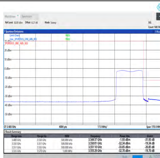
1-N78-3450-3550-30-30-H-6-CP-QPSK-Outer_Full-78@0-Ant0-1--PASS-see graph
