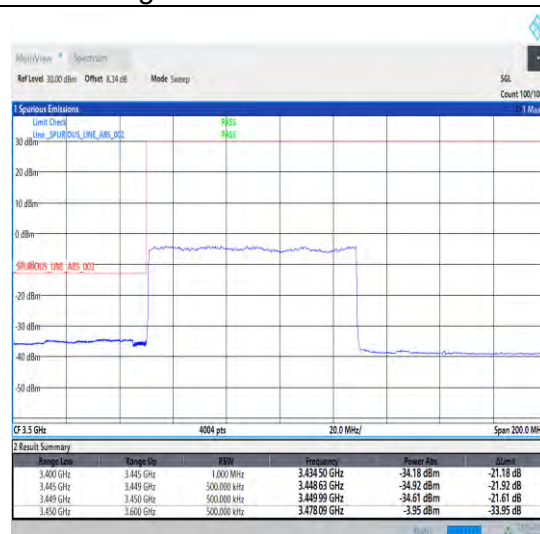
1-N78-3450-3550-30-80-L-3-DFT-PI2BPSK-Outer _Full-216@0-Ant0-1--PASS-see graph
