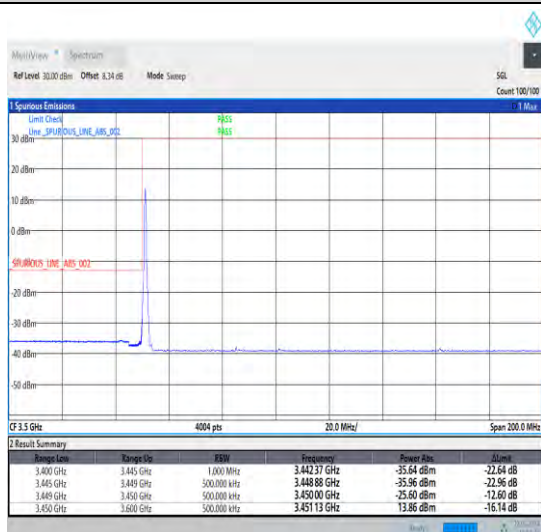
1-N78-3450-3550-30-70-L-4-CP-QPSK-Edge_1RB_Lef t-1@0-Ant0-1--PASS-see graph
