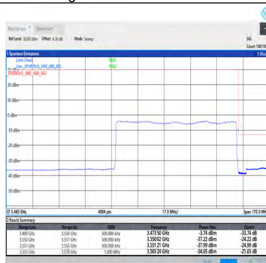
1-N78-3450-3550-30-80-H-3-DFT-PI2BPSK-Outer_Full-216@0-Ant0-1--PASS-see graph
