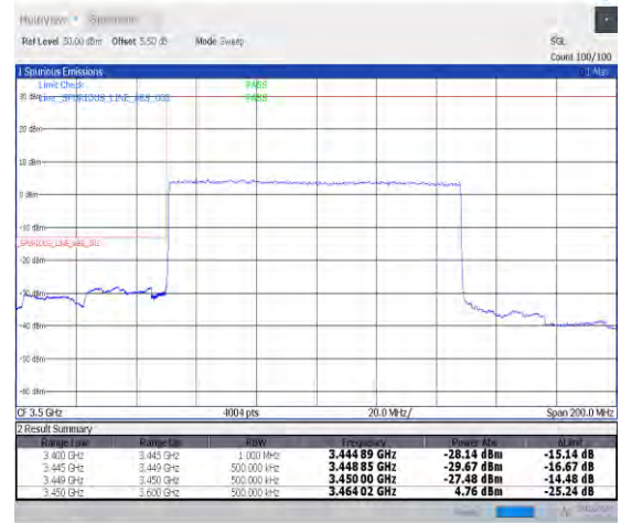
1-N78-3450-3550-PC2-30-100-L-3-DFT-PI2BPSK-Outer_Full-270@0-Ant0-1--PASS-see graph
