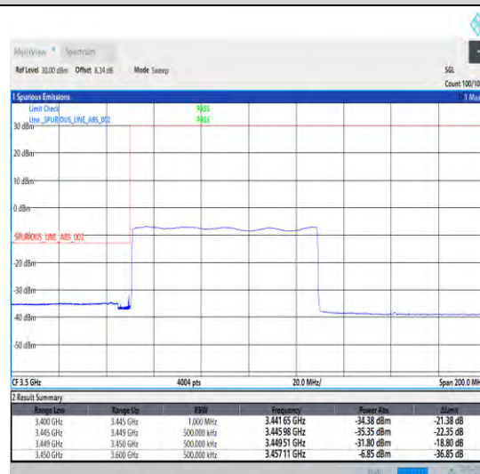
1-N78-3450-3550-30-80-L-6-CP-QPSK-Outer_Full -217@0-Ant0-1--PASS-see graph
