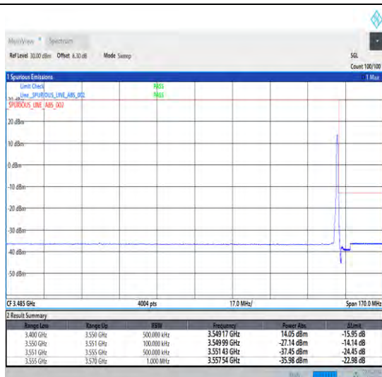
1-N78-3450-3550-30-15-H-2-DFT-PI2BPSK-Edge_1R_B_Right-1@37-Ant0-1--PASS-see graph
