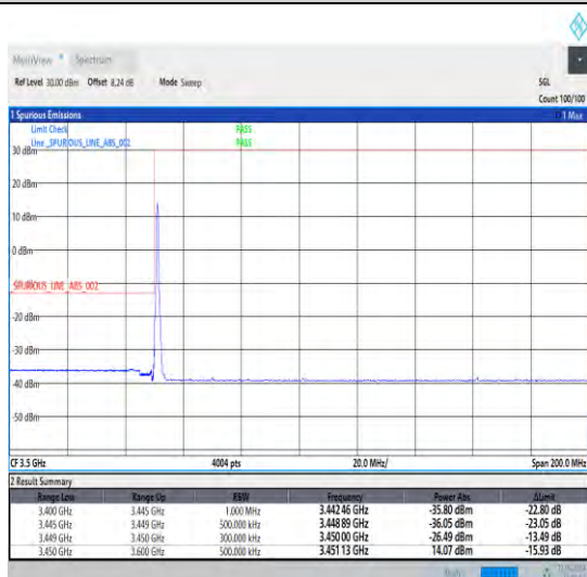
1-N78-3450-3550-30-40-L-4-CP-QPSK-Edge_1RB_Lef t-1@0-Ant0-1--PASS-see graph
