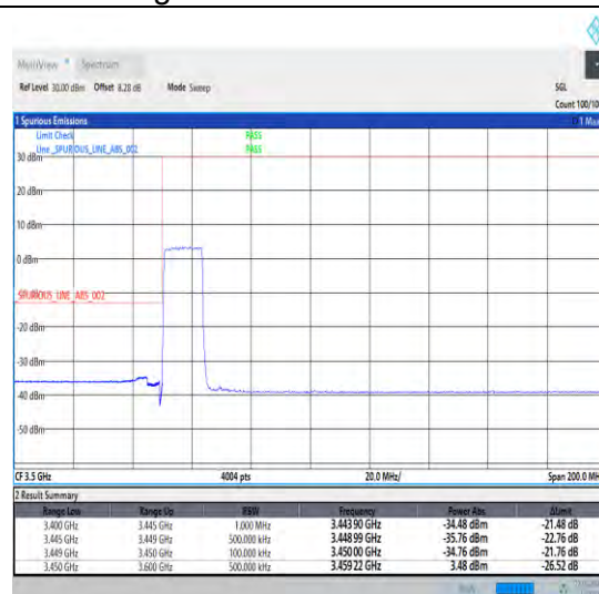
1-N78-3450-3550-30-15-L-3-DFT-PI2BPSK-Outer_Full-36@0-Ant0-1--PASS-see graph
