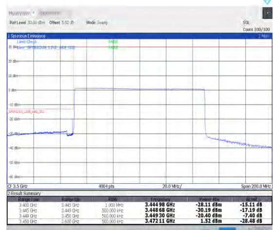
1-N78-3450-3550-PC2-30-100-L-6-CP-QPSK-Outer_Full-273@0-Ant0-1--PASS-see graph
