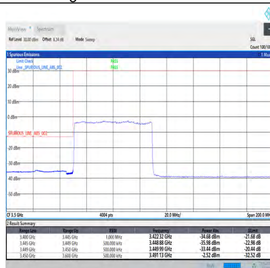
1-N78-3450-3550-30-60-L-3-DFT-PI2BPSK-Outer _Full-162@0-Ant0-1--PASS-see graph
