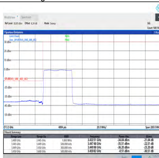
1-N78-3450-3550-30-40-L-3-DFT-PI2BPSK-Outer _Full-100@0-Ant0-1--PASS-see graph
