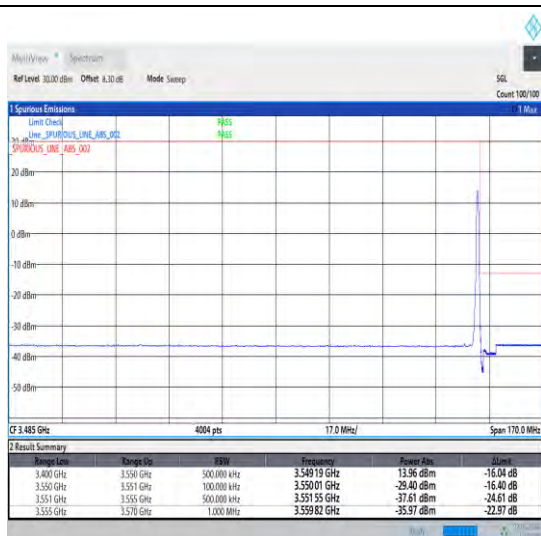
1-N78-3450-3550-30-10-H-2-DFT-PI2BPSK-Edge_1R_B_Right-1@23-Ant0-1--PASS-see graph
