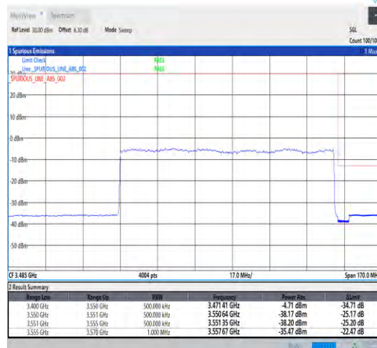
1-N78-3450-3550-30-100-H-3-DFT-PI2BPSK-Outer_Full-270@0-Ant0-1--PASS-see graph
