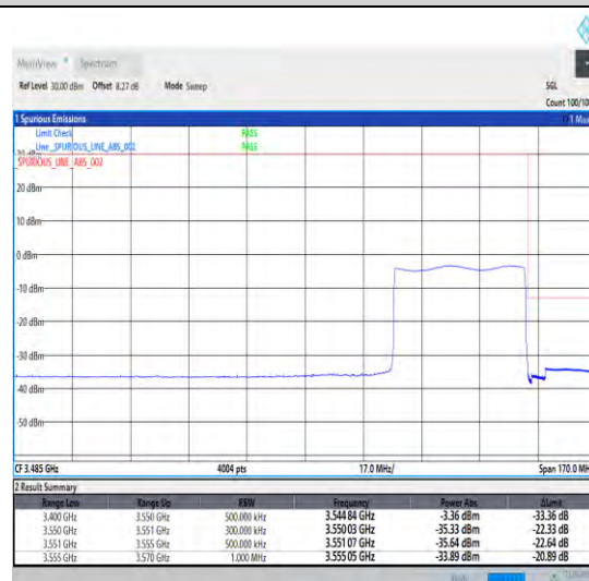
1-N78-3450-3550-30-40-H-6-CP-QPSK-Outer_Full -106@0-Ant0-1--PASS-see graph
