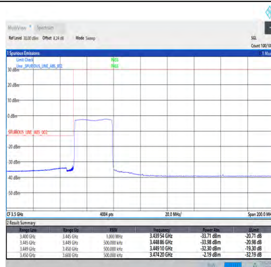
1-N78-3450-3550-30-30-L-6-CP-QPSK-Outer_Full -78@0-Ant0-1--PASS-see graph
