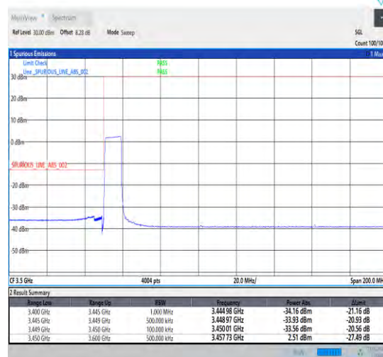
1-N78-3450-3550-30-10-L-6-CP-QPSK-Outer_Full -24@0-Ant0-1--PASS-see graph
