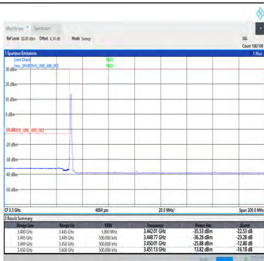
1-N78-3450-3550-30-70-L-1-DFT-PI2BPSK-Edge_1RB _Left-1@0-Ant0-1--PASS-see graph
