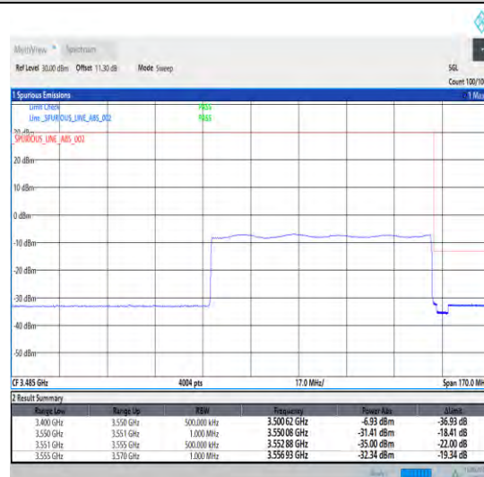
1-N78-3450-3550-30-80-H-6-CP-QPSK-Outer_Full -217@0-Ant0-1--PASS-see graph
