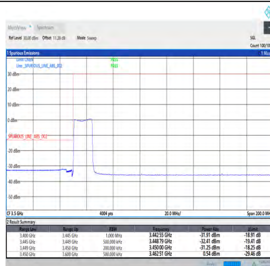
1-N78-3450-3550-30-15-L-6-CP-QPSK-Outer_Full -38@0-Ant0-1--PASS-see graph
