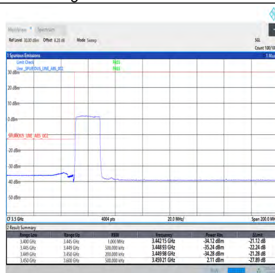
1-N78-3450-3550-30-20-L-3-DFT-PI2BPSK-Outer _Full-50@0-Ant0-1--PASS-see graph
