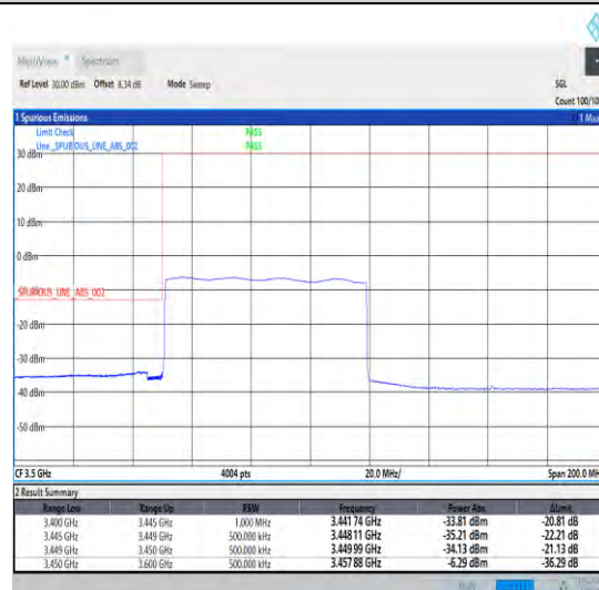
1-N78-3450-3550-30-70-L-6-CP-QPSK-Outer_Full -189@0-Ant0-1--PASS-see graph
