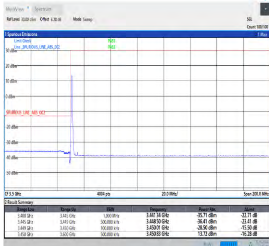
1-N78-3450-3550-30-10-L-1-DFT-PI2BPSK-Edge_1RB _Left-1@0-Ant0-1--PASS-see graph
