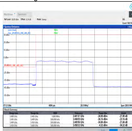
1-N78-3450-3550-30-90-L-3-DFT-PI2BPSK-Outer_Full-240@0-Ant0-1--PASS-see graph
