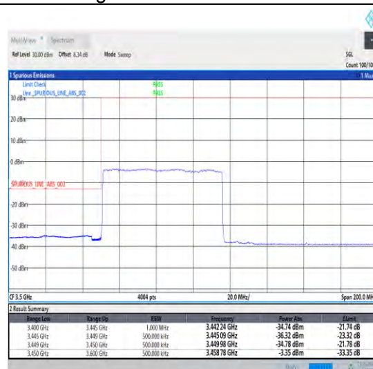
1-N78-3450-3550-30-70-L-3-DFT-PI2BPSK-Outer _Full-180@0-Ant0-1--PASS-see graph
