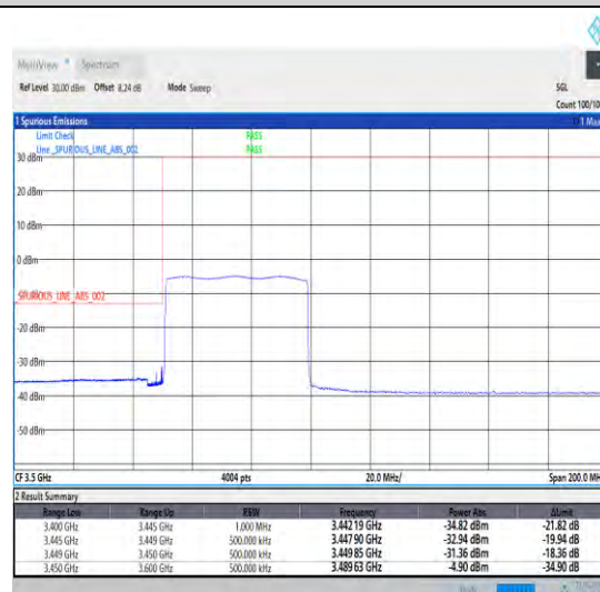
1-N78-3450-3550-30-50-L-6-CP-QPSK-Outer_Full -133@0-Ant0-1--PASS-see graph
