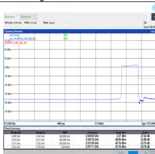
1-N78-3450-3550-30-20-H-3-DFT-PI2BPSK-Outer_Full-50@0-Ant0-1--PASS-see graph
