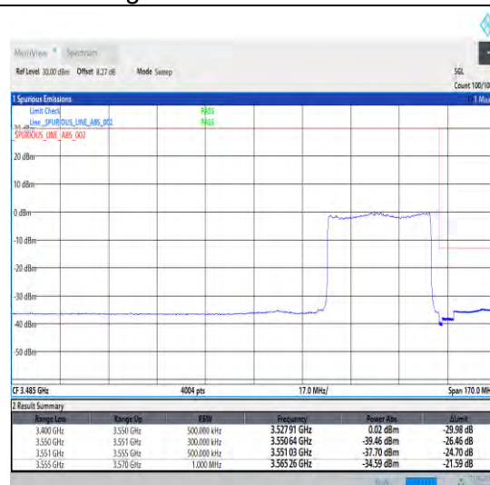
1-N78-3450-3550-30-40-H-3-DFT-PI2BPSK-Outer _Full-100@0-Ant0-1--PASS-see graph
