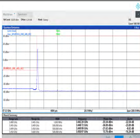
1-N78-3450-3550-30-60-L-4-CP-QPSK-Edge_1RB_Lef t-1@0-Ant0-1--PASS-see graph
