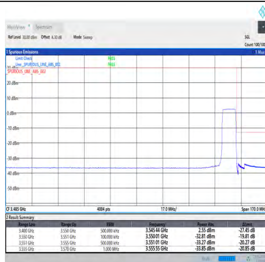
1-N78-3450-3550-30-10-H-6-CP-QPSK-Outer_Full-24@0-Ant0-1--PASS-see graph
