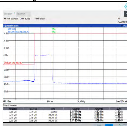
1-N78-3450-3550-30-30-L-3-DFT-PI2BPSK-Outer _Full-75@0-Ant0-1--PASS-see graph
