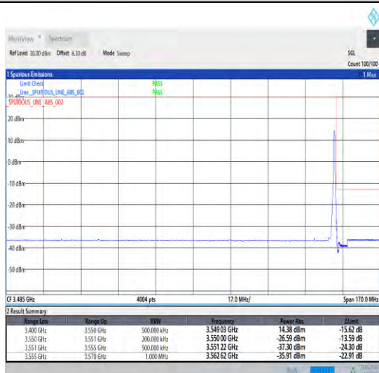
1-N78-3450-3550-30-20-H-5-CP-QPSK-Edge_1RB_Right-1@50-Ant0-1--PASS-see graph
