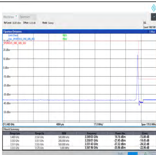
1-N78-3450-3550-30-20-H-2-DFT-PI2BPSK-Edge_1R_B_Right-1@50-Ant0-1--PASS-see graph
