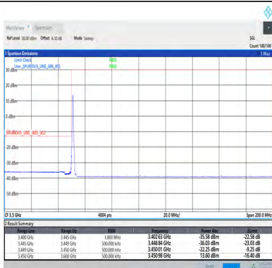
1-N78-3450-3550-30-100-L-4-CP-QPSK-Edge_1RB_Left-1@0-Ant0-1--PASS-see graph
