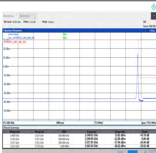
1-N78-3450-3550-30-60-H-5-CP-QPSK-Edge_1RB_Ri ght-1@161-Ant0-1--PASS-see graph
