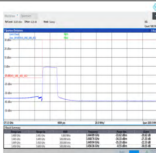
1-N78-3450-3550-30-20-L-6-CP-QPSK-Outer_Full -51@0-Ant0-1--PASS-see graph
