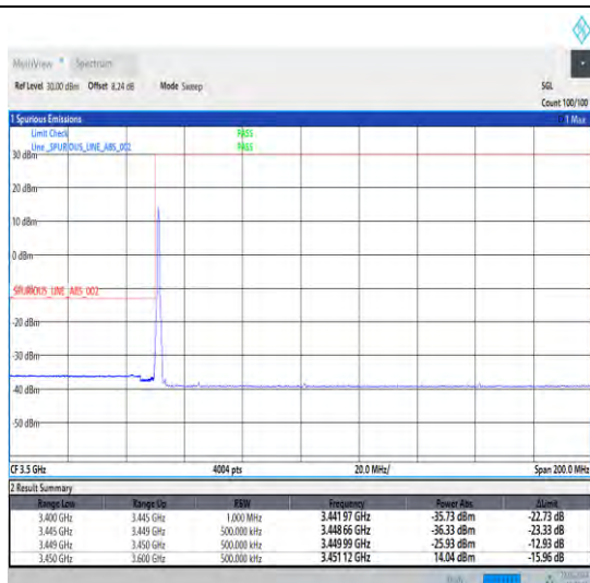
1-N78-3450-3550-30-30-L-1-DFT-PI2BPSK-Edge_1RB _Left-1@0-Ant0-1--PASS-see graph
