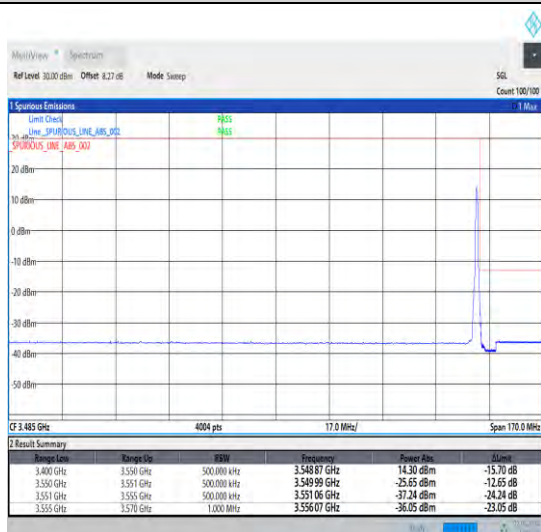
1-N78-3450-3550-30-30-H-5-CP-QPSK-Edge_1RB_Right-1@77-Ant0-1--PASS-see graph
