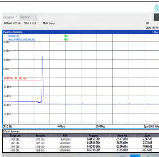
1-N78-3450-3550-30-100-L-1-DFT-PI2BPSK-Edge_1R_B_Left-1@0-Ant0-1--PASS-see graph
