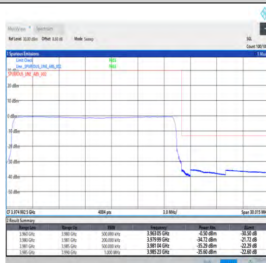
1-N77-3700-3980-30-20-H-6-CP-QPSK-Outer_Full-51@0-Ant0-1--PASS-see graph
