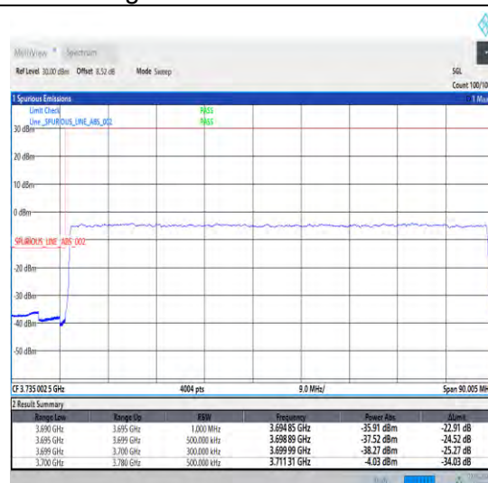
1-N77-3700-3980-30-80-L-3-DFT-PI2BPSK-Outer_Full-216@0-Ant0-1--PASS-see graph
