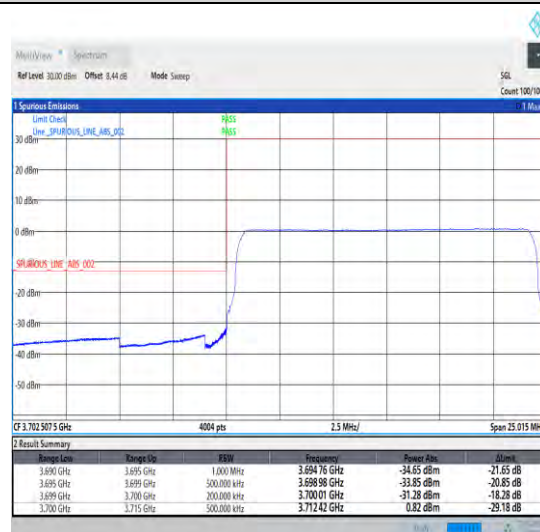
1-N77-3700-3980-30-15-L-6-CP-QPSK-Outer_Full -38@0-Ant0-1--PASS-see graph
