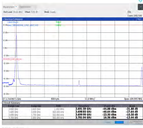
1-N77-3700-3980-PC2-30-100-L-4-CP-QPSK-Edge_1RB_Left-1@0-Ant0-1--PASS-see graph
