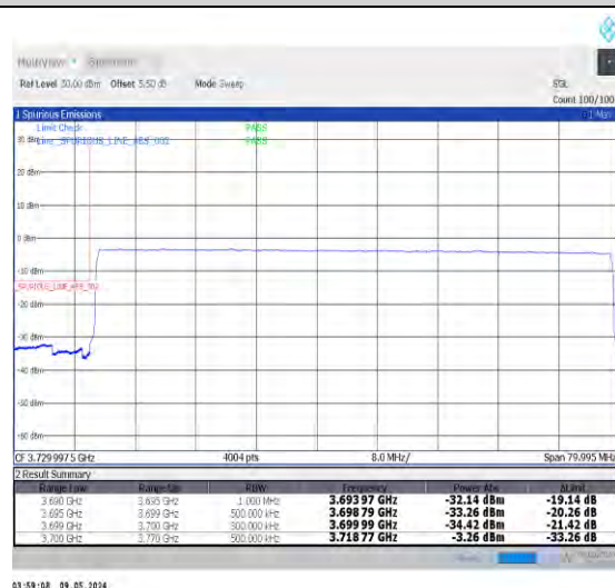
1-N77-3700-3980-PC2-30-70-L-6-CP-QPSK-Outer_Full-189@0-Ant0-1--PASS-see graph
