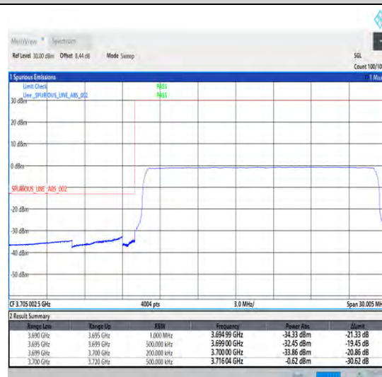
1-N77-3700-3980-30-20-L-6-CP-QPSK-Outer_Full -51@0-Ant0-1--PASS-see graph
