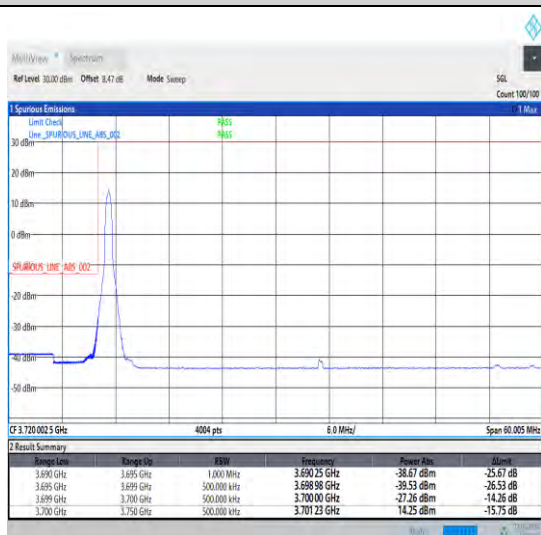
1-N77-3700-3980-30-50-L-4-CP-QPSK-Edge_1RB_Lef t-1@0-Ant0-1--PASS-see graph
