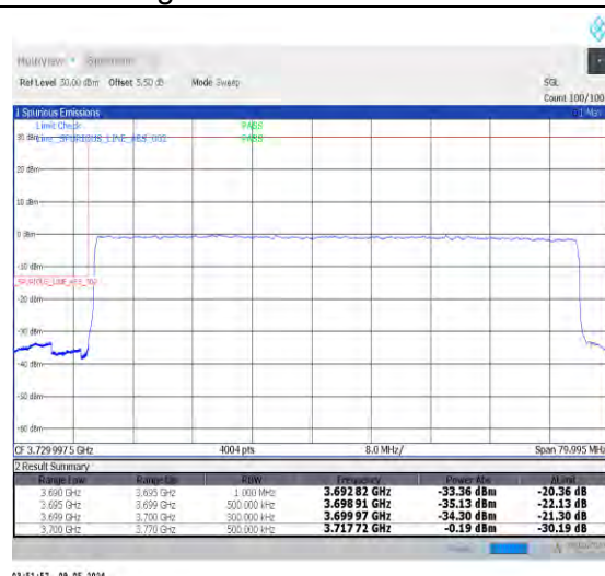
1-N77-3700-3980-PC2-30-70-L-3-DFT-PI2BPSK-Outer_Full-180@0-Ant0-1--PASS-see graph
