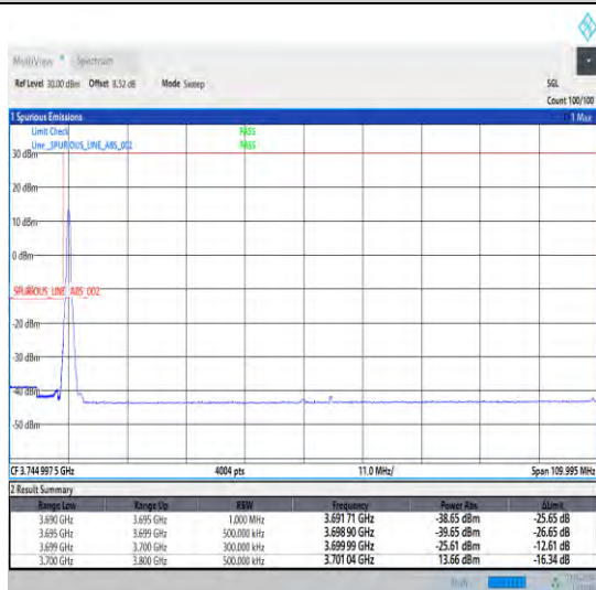
1-N77-3700-3980-30-100-L-4-CP-QPSK-Edge_1RB_Left-1@0-Ant0-1--PASS-see graph
