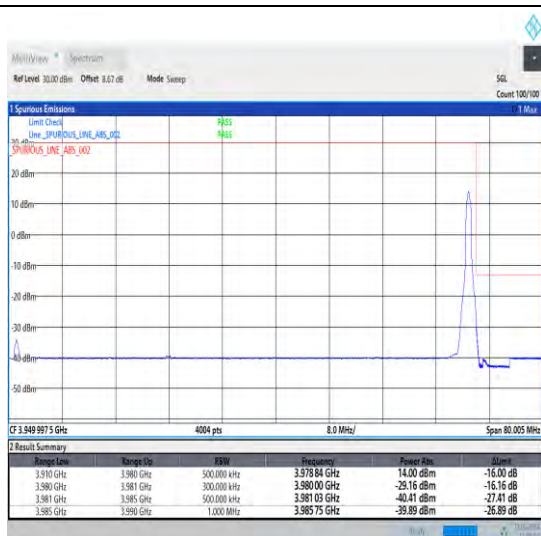
1-N77-3700-3980-30-70-H-2-DFT-PI2BPSK-Edge_1R B_Right-1@188-Ant0-1--PASS-see graph
