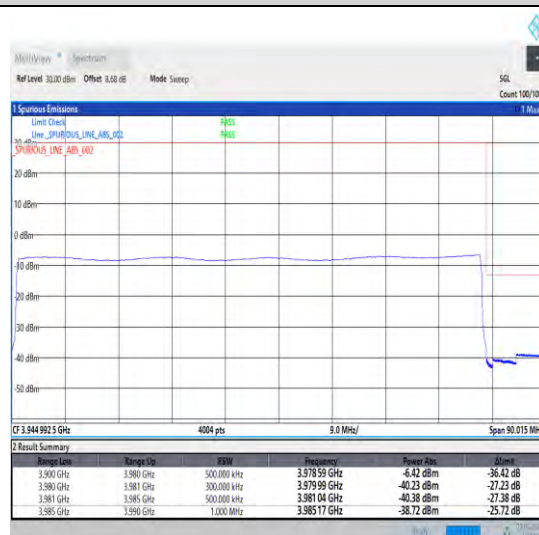
1-N77-3700-3980-30-80-H-6-CP-QPSK-Outer_Full -217@0-Ant0-1--PASS-see graph
