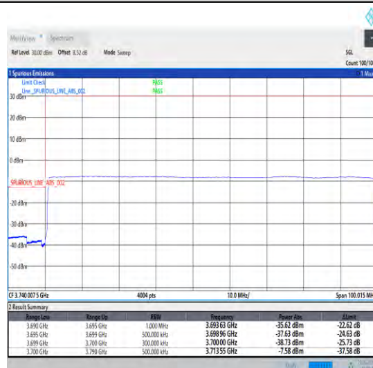
1-N77-3700-3980-30-90-L-6-CP-QPSK-Outer_Full -245@0-Ant0-1--PASS-see graph
