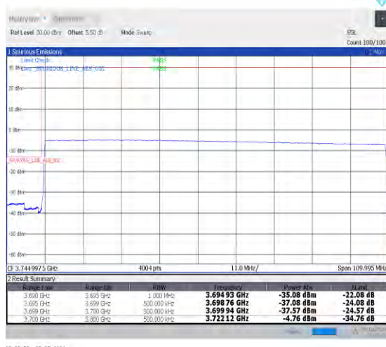
1-N77-3700-3980-PC2-30-100-L-6-CP-QPSK-Outer_Full-273@0-Ant0-1--PASS-see graph
