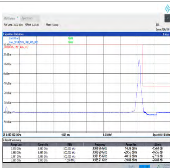
1-N77-3700-3980-30-50-H-2-DFT-PI2BPSK-Edge_1R B_Right-1@132-Ant0-1--PASS-see graph
