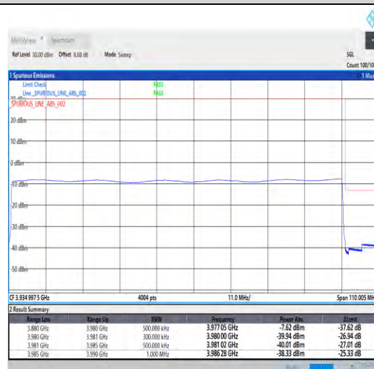
1-N77-3700-3980-30-100-H-6-CP-QPSK-Outer_Full-273@0-Ant0-1--PASS-see graph
