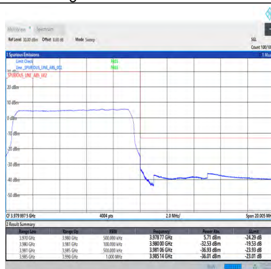
1-N77-3700-3980-30-10-H-3-DFT-PI2BPSK-Outer_Full-24@0-Ant0-1--PASS-see graph
