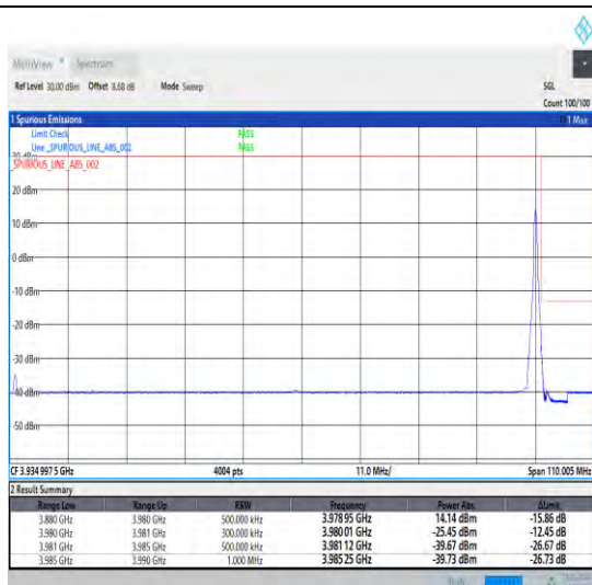
1-N77-3700-3980-30-100-H-2-DFT-PI2BPSK-Edge_1R_B_Right-1@272-Ant0-1--PASS-see graph
