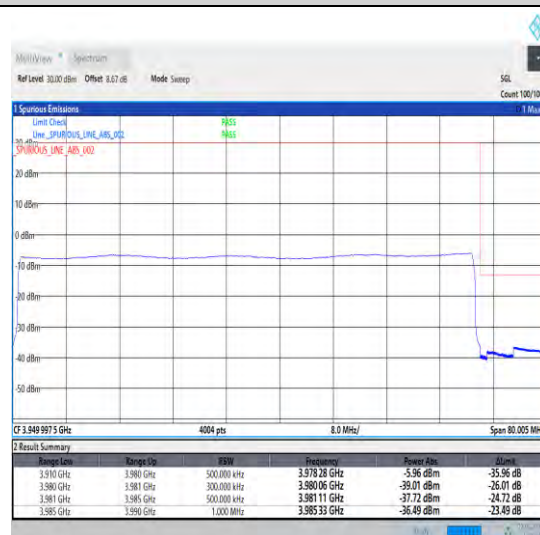
1-N77-3700-3980-30-70-H-6-CP-QPSK-Outer_Full -189@0-Ant0-1--PASS-see graph
