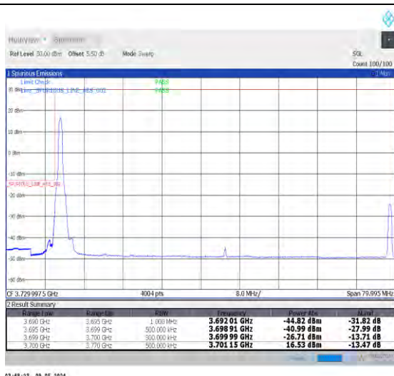
1-N77-3700-3980-PC2-30-70-L-1-DFT-PI2BPSK-Edge_1RB_Left-1@0-Ant0-1--PASS-see graph
