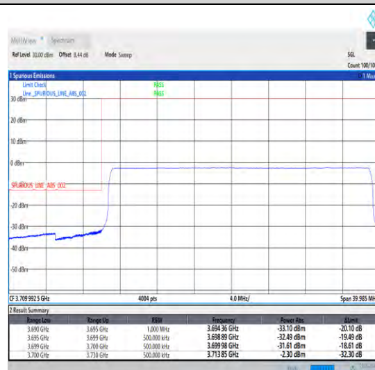
1-N77-3700-3980-30-30-L-6-CP-QPSK-Outer_Full -78@0-Ant0-1--PASS-see graph
