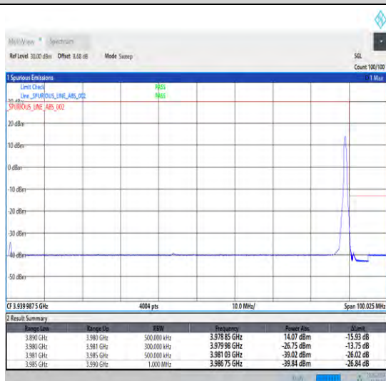
1-N77-3700-3980-30-90-H-5-CP-QPSK-Edge_1RB_Ri ght-1@244-Ant0-1--PASS-see graph
