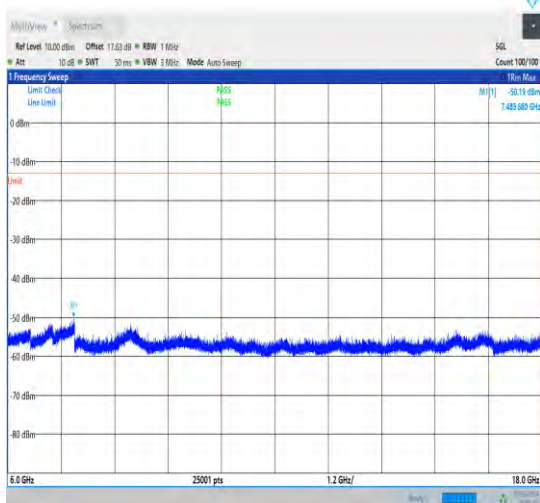
1-N77-3700-3980-30-100-M-1-DFT-PI2BPSK-Inner_1RB_Left-1@1-6000-18000-Ant0-7483.68--50.19--1 3-PASS
