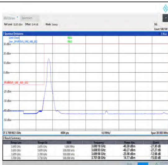
1-N77-3700-3980-30-30-L-1-DFT-PI2BPSK-Edge_1RB_Left-1@0-Ant0-1--PASS-see graph
