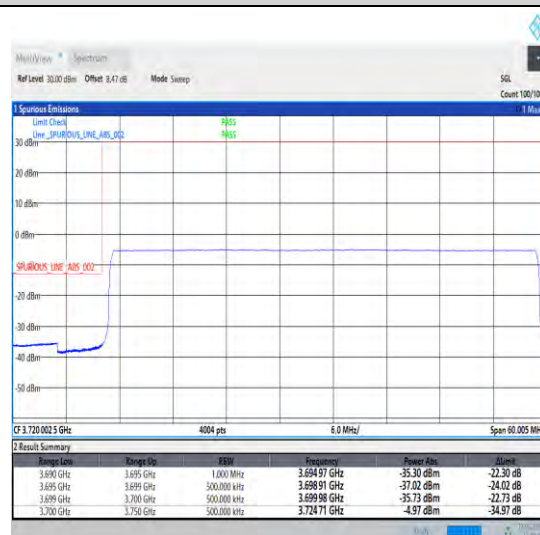
1-N77-3700-3980-30-50-L-6-CP-QPSK-Outer_Full -133@0-Ant0-1--PASS-see graph
