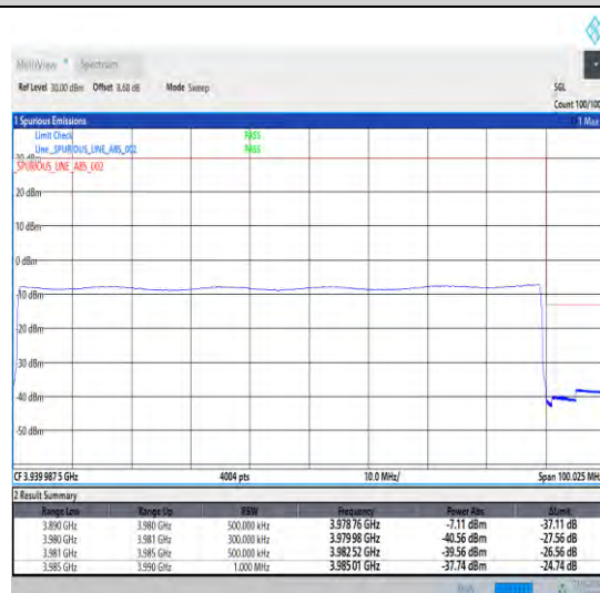
1-N77-3700-3980-30-90-H-6-CP-QPSK-Outer_Full -245@0-Ant0-1--PASS-see graph
