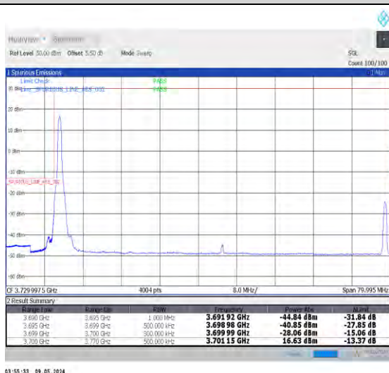
1-N77-3700-3980-PC2-30-70-L-4-CP-QPSK-Edge_1RB_Left-1@0-Ant0-1--PASS-see graph
