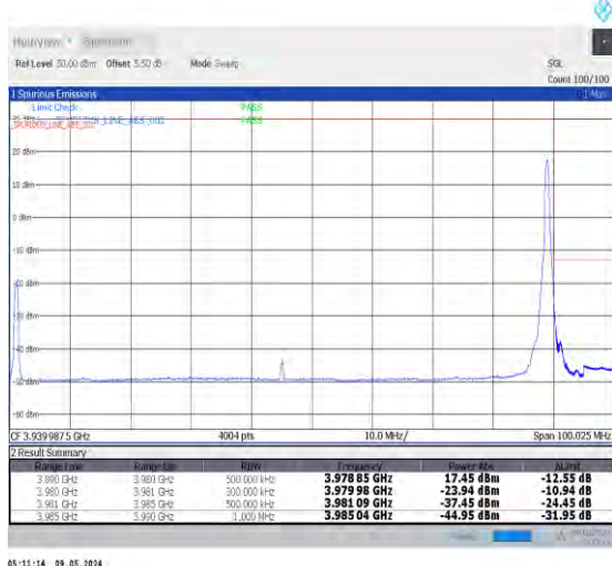
1-N77-3700-3980-PC2-30-90-H-5-CP-QPSK-Edge_1RB_Right-1@244-Ant0-1--PASS-see graph
