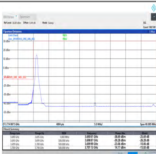
1-N77-3700-3980-30-40-L-4-CP-QPSK-Edge_1RB_Lef t-1@0-Ant0-1--PASS-see graph
