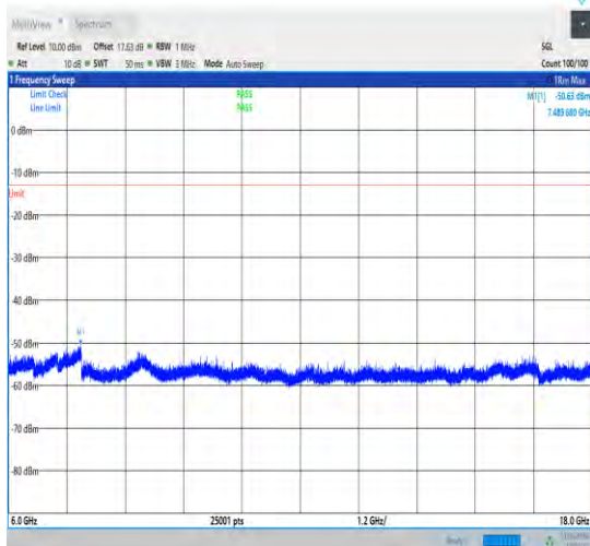
1-N77-3700-3980-30-100-L-1-DFT-PI2BPSK-Inner_1RB_Left-1@1-6000-18000-Ant0-7483.68--50.63--1 3-PASS
