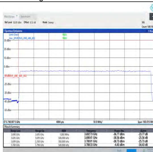
1-N77-3700-3980-30-90-L-3-DFT-PI2BPSK-Outer _Full-240@0-Ant0-1--PASS-see graph
