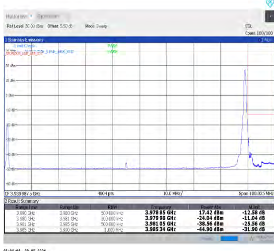
1-N77-3700-3980-PC2-30-90-H-2-DFT-PI2BPSK-Edge_1RB_Right-1@244-Ant0-1--PASS-see graph
