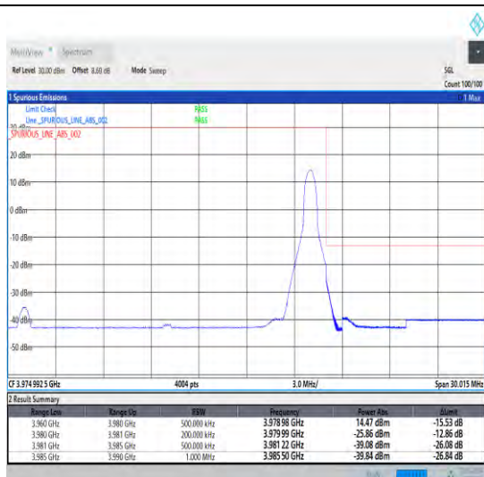
1-N77-3700-3980-30-20-H-2-DFT-PI2BPSK-Edge_1R_B_Right-1@50-Ant0-1--PASS-see graph
