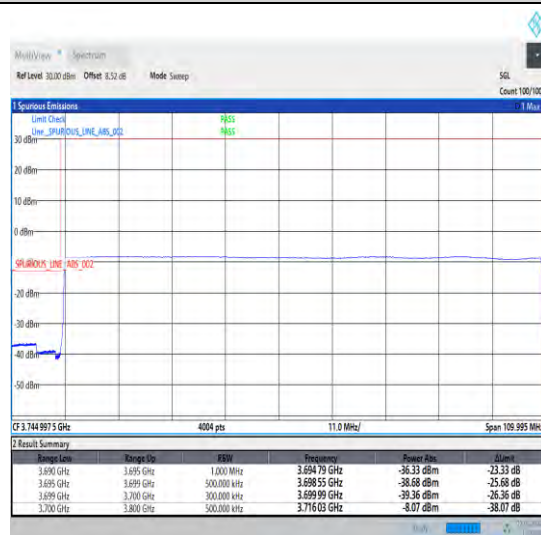
1-N77-3700-3980-30-100-L-6-CP-QPSK-Outer_Full-273@0-Ant0-1--PASS-see graph
