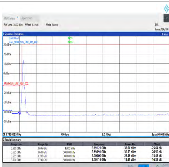
1-N77-3700-3980-30-80-L-1-DFT-PI2BPSK-Edge_1RB_Left-1@0-Ant0-1--PASS-see graph
