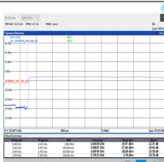
1-N77-3700-3980-30-60-L-6-CP-QPSK-Outer_Full -162@0-Ant0-1--PASS-see graph
