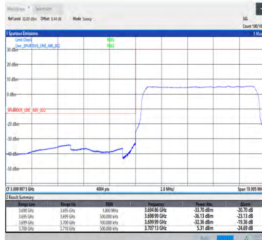
1-N77-3700-3980-30-10-L-3-DFT-PI2BPSK-Outer _Full-24@0-Ant0-1--PASS-see graph
