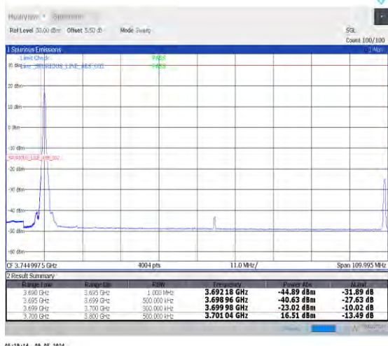
1-N77-3700-3980-PC2-30-100-L-1-DFT-PI2BPSK-Edge_1RB_Left-1@0-Ant0-1--PASS-see graph
