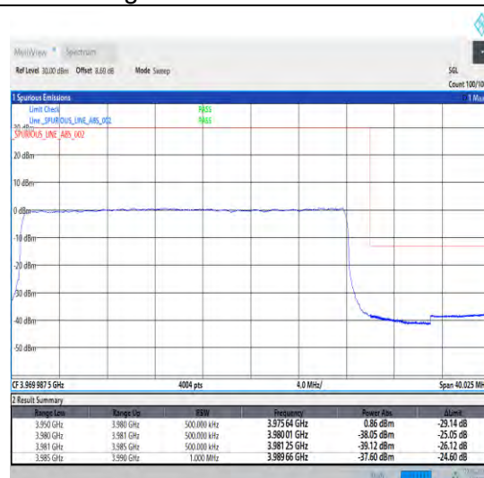
1-N77-3700-3980-30-30-H-3-DFT-PI2BPSK-Outer_Full-75@0-Ant0-1--PASS-see graph
