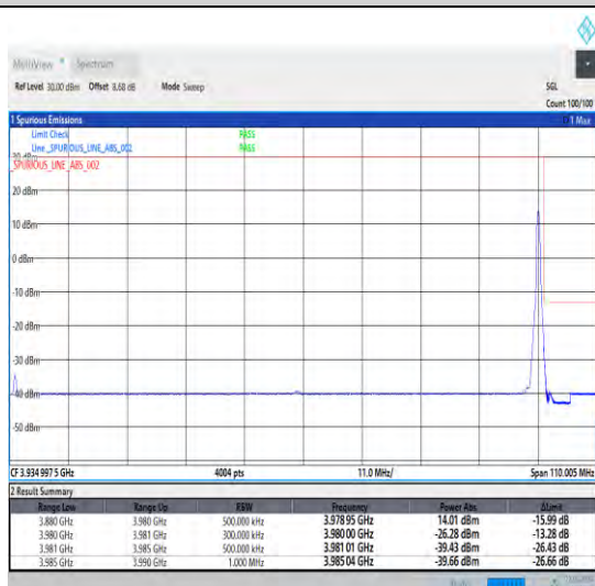
1-N77-3700-3980-30-100-H-5-CP-QPSK-Edge_1RB_Right-1@272-Ant0-1--PASS-see graph
