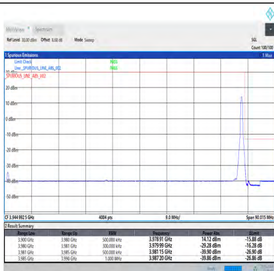
1-N77-3700-3980-30-80-H-2-DFT-PI2BPSK-Edge_1R B_Right-1@216-Ant0-1--PASS-see graph
