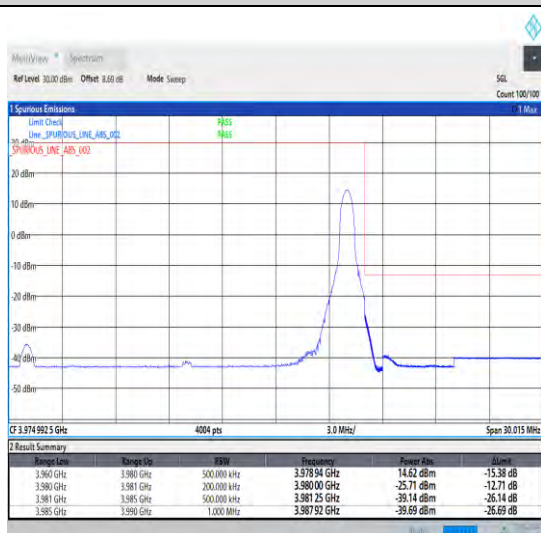
1-N77-3700-3980-30-20-H-5-CP-QPSK-Edge_1RB_Right-1@50-Ant0-1--PASS-see graph
