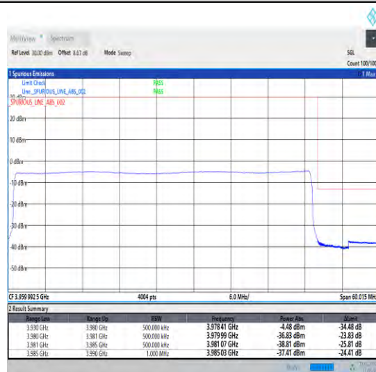
1-N77-3700-3980-30-50-H-6-CP-QPSK-Outer_Full -133@0-Ant0-1--PASS-see graph
