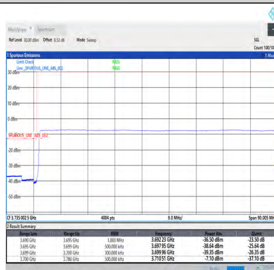
1-N77-3700-3980-30-80-L-6-CP-QPSK-Outer_Full -217@0-Ant0-1--PASS-see graph
