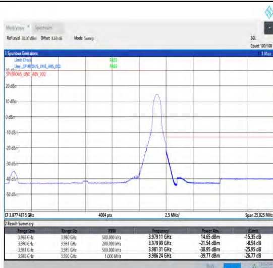
1-N77-3700-3980-30-15-H-5-CP-QPSK-Edge_1RB_Right-1@37-Ant0-1--PASS-see graph
