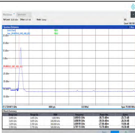
1-N77-3700-3980-30-70-L-4-CP-QPSK-Edge_1RB_Lef t-1@0-Ant0-1--PASS-see graph
