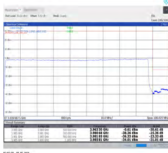
1-N77-3700-3980-PC2-30-90-H-3-DFT-PI2BPSK-Outer_Full-240@0-Ant0-1--PASS-see graph
