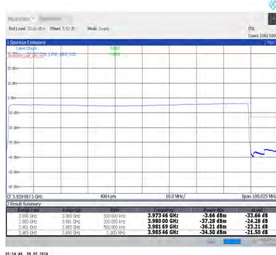
1-N77-3700-3980-PC2-30-90-H-6-CP-QPSK-Outer_Full-245@0-Ant0-1--PASS-see graph
