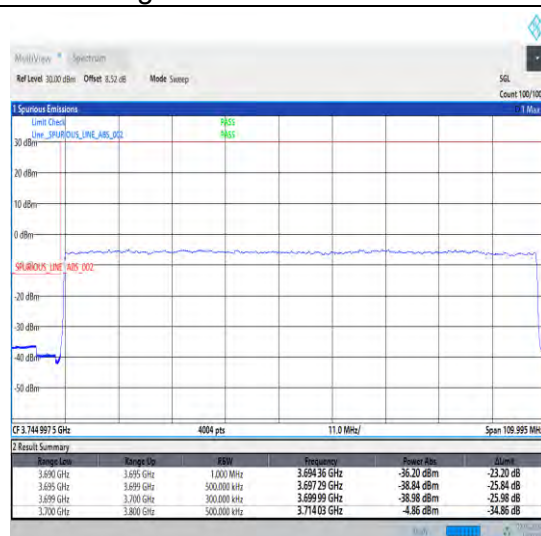
1-N77-3700-3980-30-100-L-3-DFT-PI2BPSK-Outer_Full-270@0-Ant0-1--PASS-see graph
