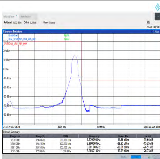
1-N77-3700-3980-30-10-H-5-CP-QPSK-Edge_1RB_Right-1@23-Ant0-1--PASS-see graph
