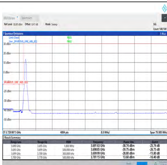
1-N77-3700-3980-30-70-L-1-DFT-PI2BPSK-Edge_1RB _Left-1@0-Ant0-1--PASS-see graph
