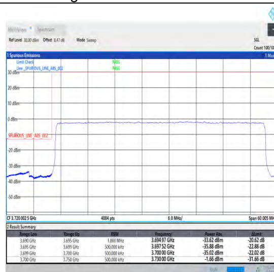
1-N77-3700-3980-30-50-L-3-DFT-PI2BPSK-Outer _Full-128@0-Ant0-1--PASS-see graph
