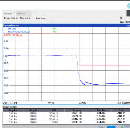
1-N77-3700-3980-30-15-H-6-CP-QPSK-Outer_Full-38@0-Ant0-1--PASS-see graph
