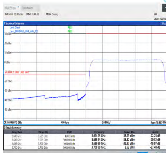
1-N77-3700-3980-30-10-L-6-CP-QPSK-Outer_Full -24@0-Ant0-1--PASS-see graph
