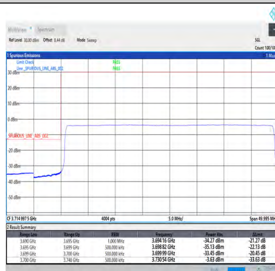
1-N77-3700-3980-30-40-L-6-CP-QPSK-Outer_Full -106@0-Ant0-1--PASS-see graph
