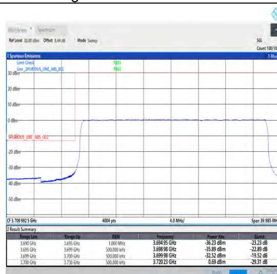
1-N77-3700-3980-30-30-L-3-DFT-PI2BPSK-Outer_Full-75@0-Ant0-1--PASS-see graph
