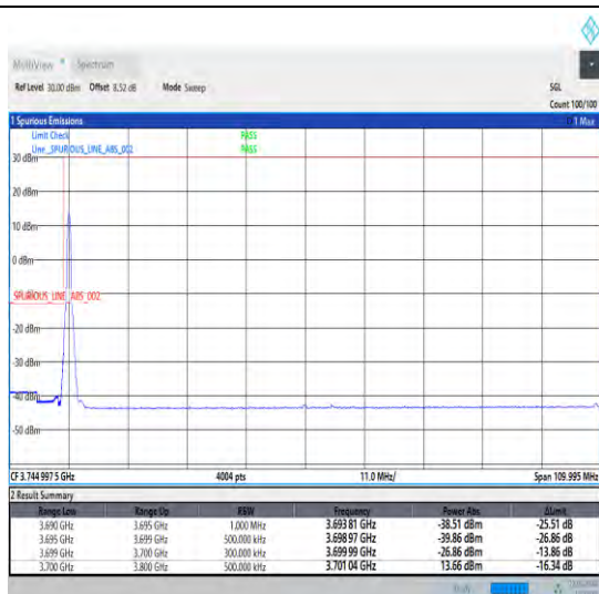
1-N77-3700-3980-30-100-L-1-DFT-PI2BPSK-Edge_1R B_Left-1@0-Ant0-1--PASS-see graph
