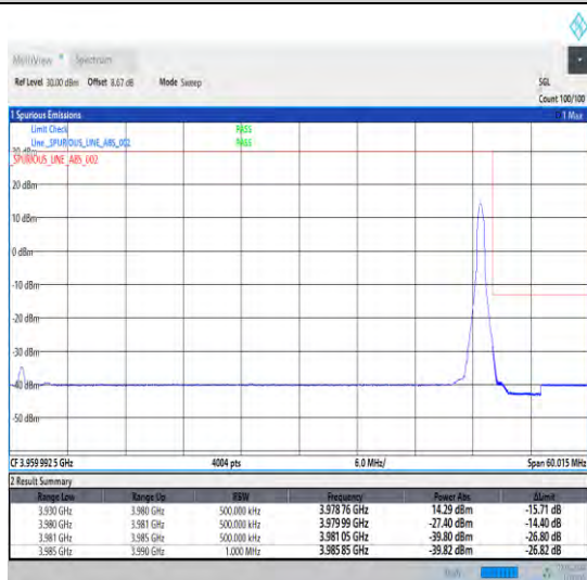
1-N77-3700-3980-30-50-H-5-CP-QPSK-Edge_1RB_Ri ght-1@132-Ant0-1--PASS-see graph
