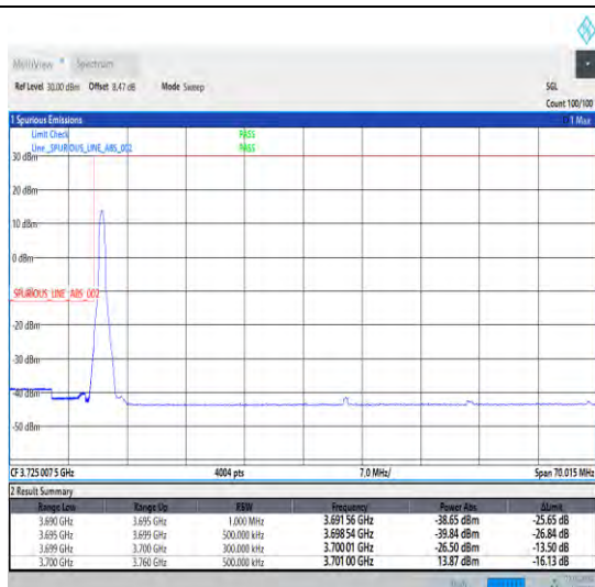
1-N77-3700-3980-30-60-L-1-DFT-PI2BPSK-Edge_1RB _Left-1@0-Ant0-1--PASS-see graph
