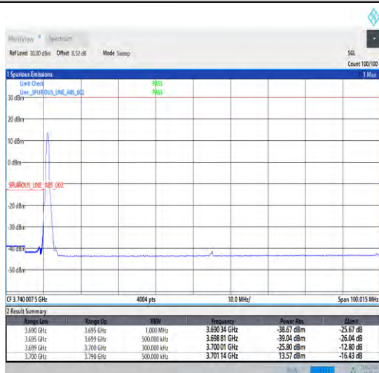
1-N77-3700-3980-30-90-L-4-CP-QPSK-Edge_1RB_Lef t-1@0-Ant0-1--PASS-see graph
