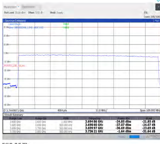
1-N77-3700-3980-PC2-30-100-L-3-DFT-PI2BPSK-Outer_Full-270@0-Ant0-1--PASS-see graph
