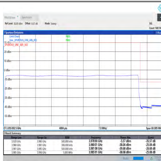
1-N77-3700-3980-30-60-H-6-CP-QPSK-Outer_Full -162@0-Ant0-1--PASS-see graph
