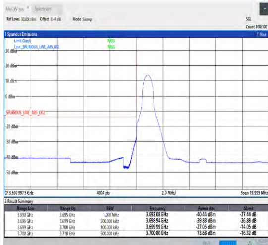
1-N77-3700-3980-30-10-L-1-DFT-PI2BPSK-Edge_1RB _Left-1@0-Ant0-1--PASS-see graph
