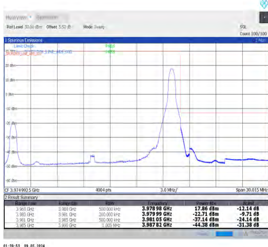
1-N77-3700-3980-PC2-30-20-H-5-CP-QPSK-Edge_1R B_Right-1@50-Ant0-1--PASS-see graph
