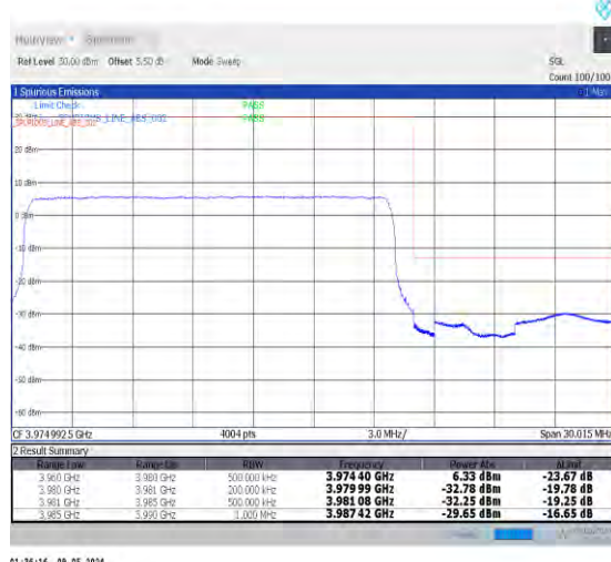
1-N77-3700-3980-PC2-30-20-H-3-DFT-PI2BPSK- Outer_Full-50@0-Ant0-1--PASS-see graph
