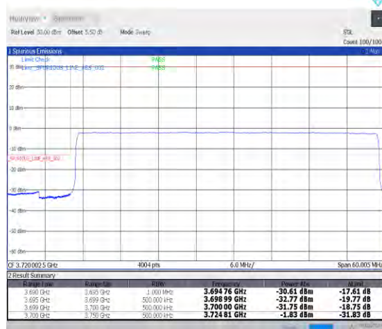
1-N77-3700-3980-PC2-30-50-L-6-CP-QPSK-Outer_Full-133@0-Ant0-1--PASS-see graph
