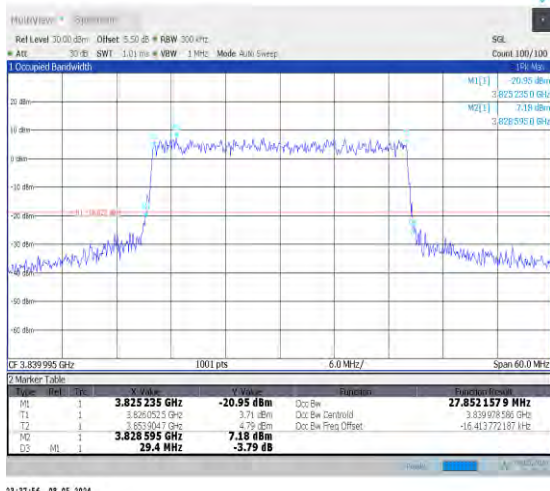
1-N77-3700-3980-PC2-30-30-M-6-CP-QPSK-Out Full-78@0-Ant0-27.853-29.400-≤30-PASS
