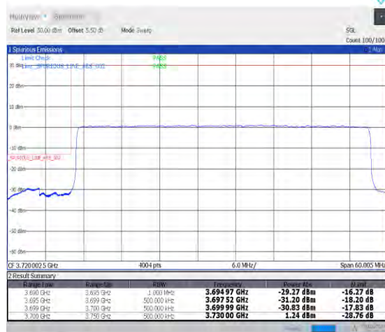
1-N77-3700-3980-PC2-30-50-L-3-DFT-PI2BPSK-Outer_Full-128@0-Ant0-1--PASS-see graph
