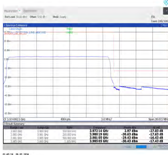
1-N77-3700-3980-PC2-30-20-H-6-CP-QPSK-Outer _Full-51@0-Ant0-1--PASS-see graph
