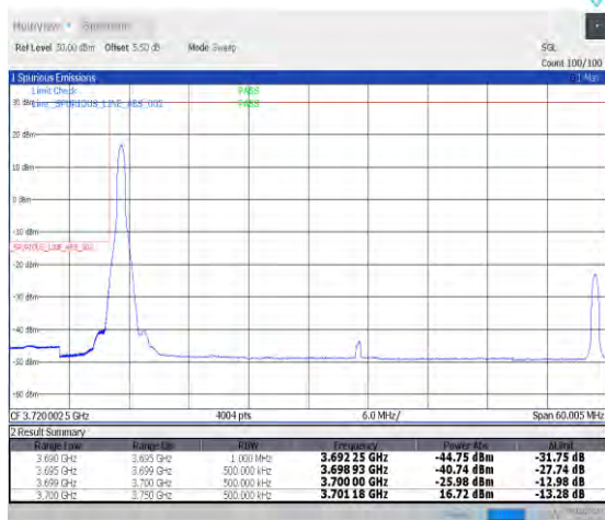
1-N77-3700-3980-PC2-30-50-L-1-DFT-PI2BPSK-Edge_1RB_Left-1@0-Ant0-1--PASS-see graph
