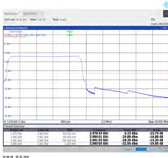
1-N77-3700-3980-PC2-30-10-H-6-CP-QPSK-Outer_Full-24@0-Ant0-1--PASS-see graph
