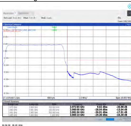
1-N77-3700-3980-PC2-30-10-H-3-DFT-PI2BPSK-Outer_Full-24@0-Ant0-1--PASS-see graph
