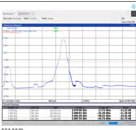
1-N77-3700-3980-PC2-30-10-H-2-DFT-PI2BPSK-Edge_1RB_Right-1@23-Ant0-1--PASS-see graph
