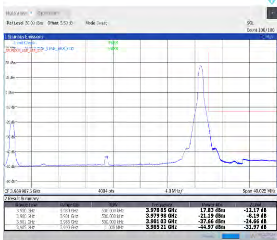
1-N77-3700-3980-PC2-30-30-H-5-CP-QPSK-Edge_1R_B_Right-1@77-Ant0-1--PASS-see graph
