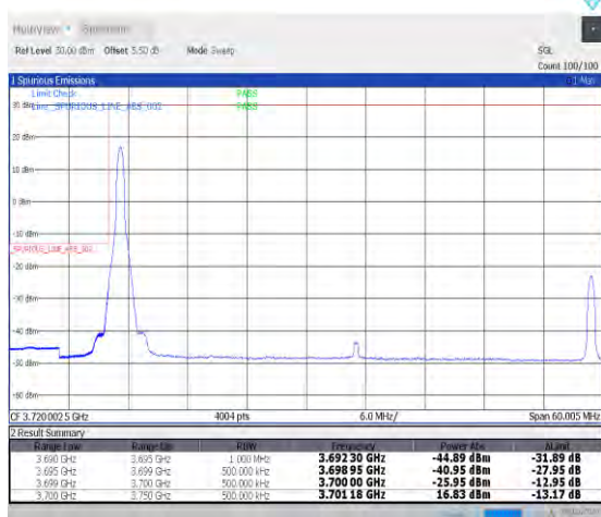
1-N77-3700-3980-PC2-30-50-L-4-CP-QPSK-Edge_1RB_Left-1@0-Ant0-1--PASS-see graph
