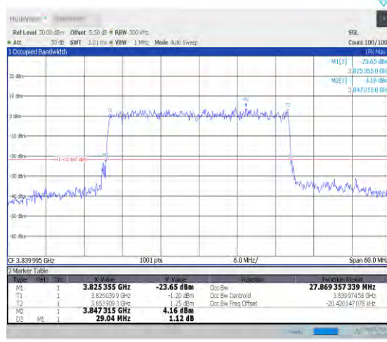
1-N77-3700-3980-PC2-30-30-M-9-CP-256QAM-Out Full-78@0-Ant0-27.87-29.040-≤30-PASS
