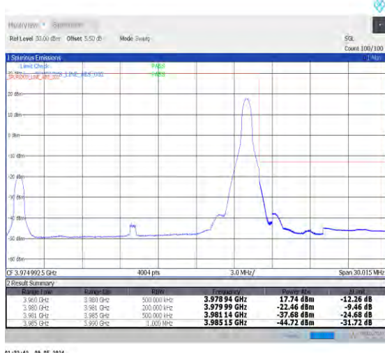
1-N77-3700-3980-PC2-30-20-H-2-DFT-PI2BPSK-Edge _1RB_Right-1@50-Ant0-1--PASS-see graph
