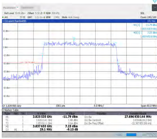
1-N77-3700-3980-PC2-30-30-M-8-CP-64QAM-Out Full-78@0-Ant0-27.692-29.100-≤30-PASS
