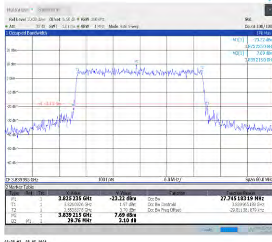
1-N77-3700-3980-PC2-30-30-M-7-CP-16QAM-Out Full-78@0-Ant0-27.745-29.760-≤30-PASS
