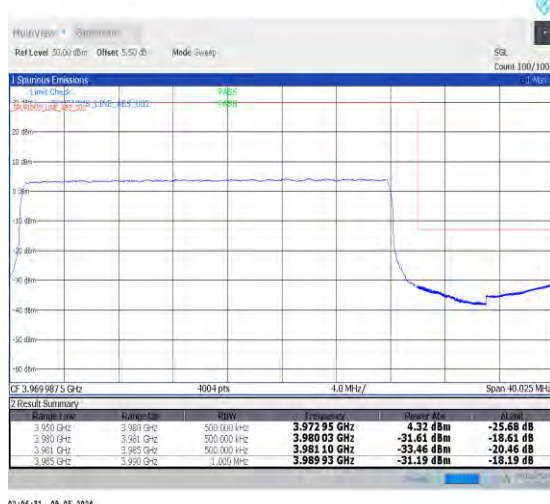
1-N77-3700-3980-PC2-30-30-H-3-DFT-PI2BPSK-Outer_Full-75@0-Ant0-1--PASS-see graph
