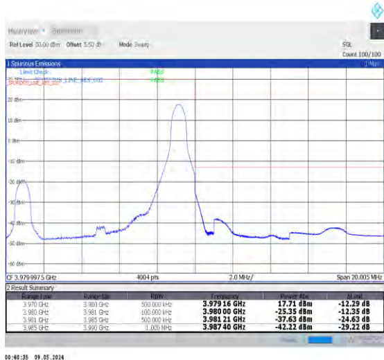
1-N77-3700-3980-PC2-30-10-H-5-CP-QPSK-Edge_1R_B_Right-1@23-Ant0-1--PASS-see graph
