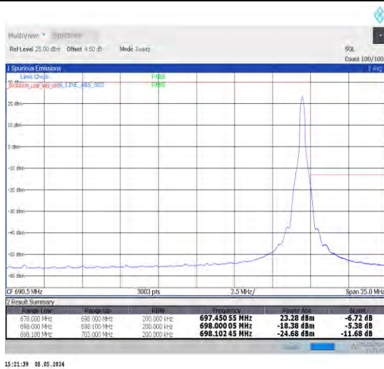
1-N71-PC3-15-20-H-2-DFT-PI2BPSK-Edge_1RB_Righ t-1@105-Ant0-1--PASS-see graph
