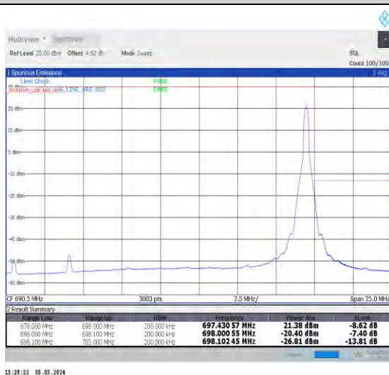
1-N71-PC3-15-20-H-5-CP-QPSK-Edge_1RB_Right-1 @105-Ant0-1--PASS-see graph
