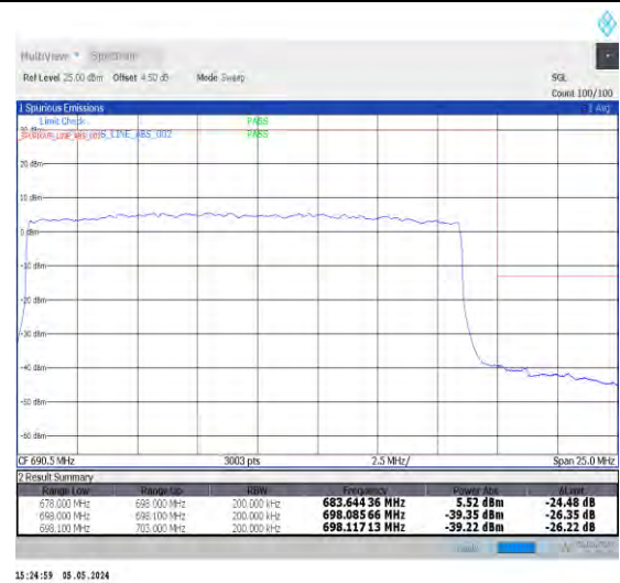
1-N71-PC3-15-20-H-3-DFT-PI2BPSK-Outer_Full-1 00@0-Ant0-1--PASS-see graph
