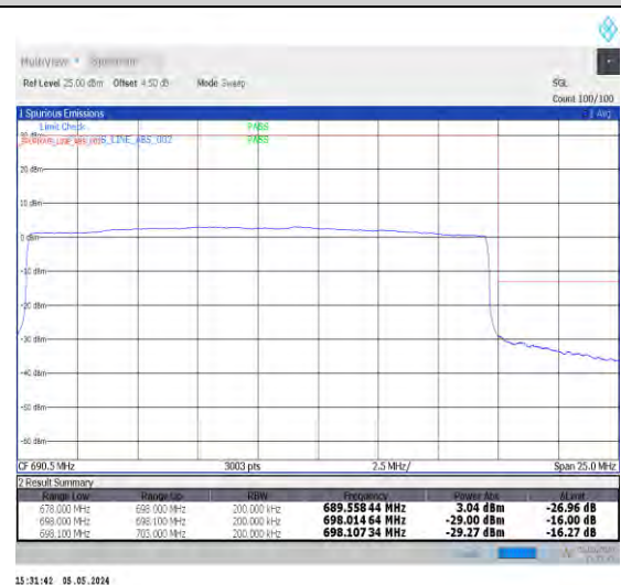
1-N71-PC3-15-20-H-6-CP-QPSK-Outer_Full-106 @0-Ant0-1--PASS-see graph
