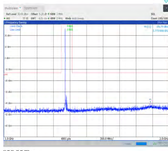
1-N66-15-40-H-1-DFT-PI2BPSK-Inner_1RB_Left-1@ 1-1000-3000-Ant0-2772.00--39.79--13-PASS
