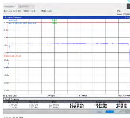
1-N66-15-30-L-6-CP-QPSK-Outer_Full-160@0-Ant0-1-seegraph-PASS-see graph
