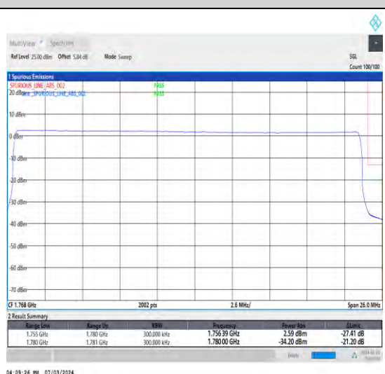
1-N66-15-25-H-6-CP-QPSK-Outer_Full-133@0-Ant1-1-seegraph-PASS-see graph
