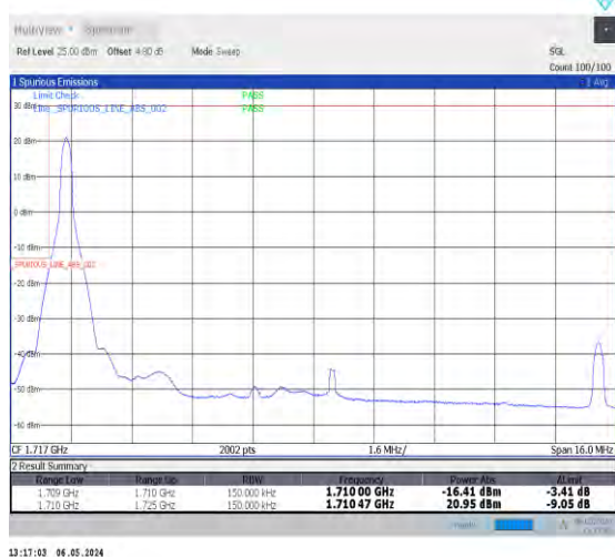
1-N66-15-15-L-4-CP-QPSK-Edge_1RB_Left-1@0-Ant0-1-seegraph-PASS-see graph
