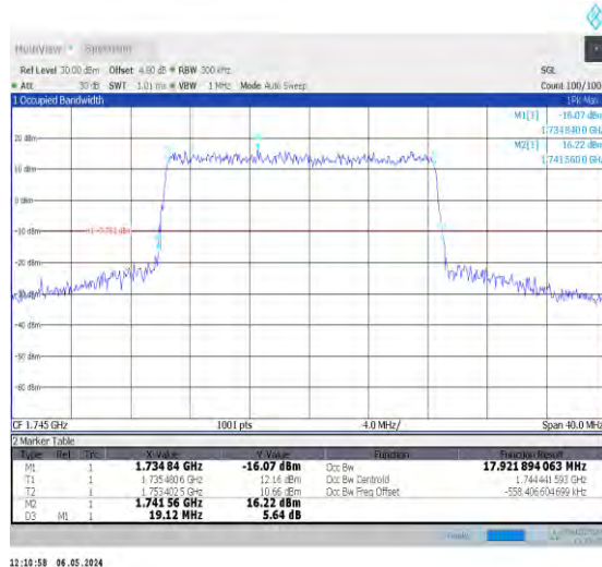
1-N66-15-20-M-1-DFT-QPSK-Outer_Full-100@0-Ant 0-17.922-19.120≤20-PASS
