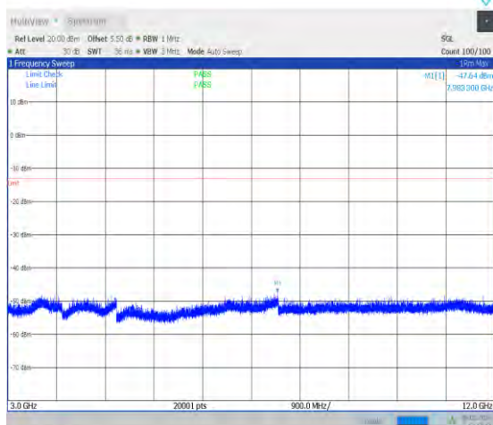
1-N66-15-40-L-1-DFT-PI2BPSK-Inner_1RB_Left-1 @ 1-3000-12000-Ant0-7983.30--47.64--13-PASS
