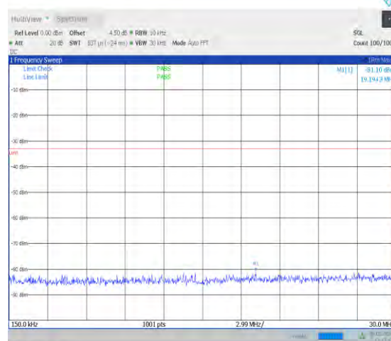
1-N66-15-40-M-1-DFT-PI2BPSK-Inner_1RB_Left-1@ 1-0.15-30-Ant0-19.19--81.10--33-PASS
