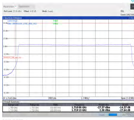
1-N66-15-10-L-6-CP-QPSK-Outer_Full-52@0-Ant0-1-seegraph-PASS-see graph
