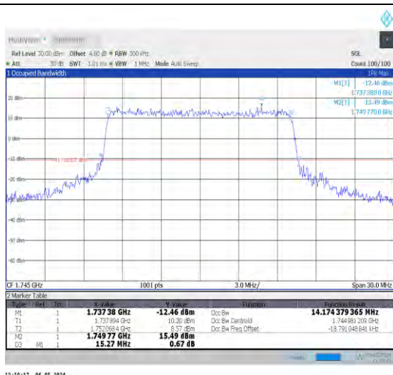
1-N66-15-15-M-7-CP-16QAM-Outer_Full-79@0-Ant0 -14.174-15.270≤15-PASS
