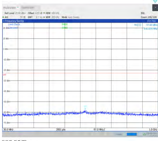
1-N66-15-40-H-1-DFT-PI2BPSK-Inner_1RB_Left-1 @1-30-1000-Ant0-545.07--57.65--23-PASS
