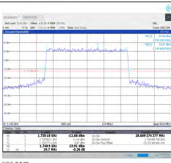
1-N66-15-30-M-1-DFT-QPSK-Outter_Full-160@0-Ant 0-28.61-29.700-≤30-PASS
