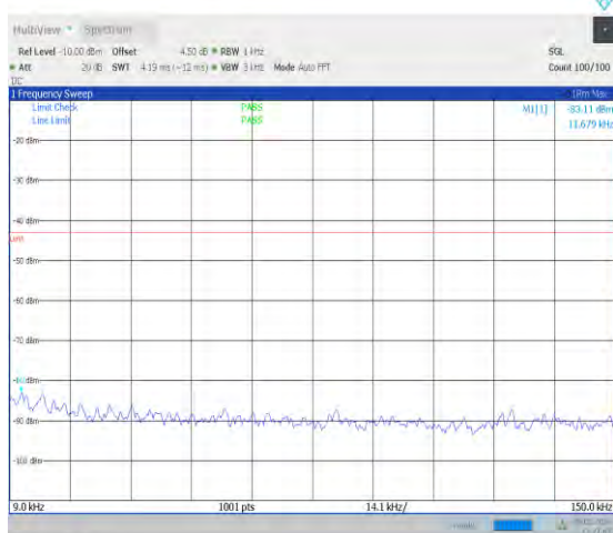
1-N66-15-40-M-1-DFT-PI2BPSK-Inner_1RB_Left-1 @ 1-0.009-0.15-Ant0-0.01--83.11--43-PASS
