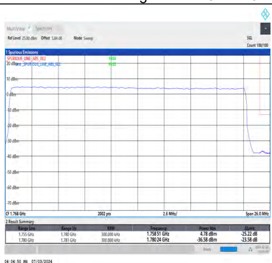
1-N66-15-25-H-3-DFT-PI2BPSK-Outer_Full-128@0-Ant1-1-seegraph-PASS-see graph
