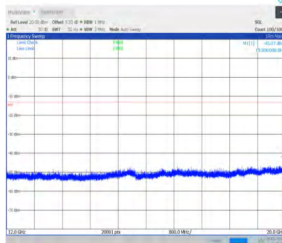
1-N66-15-40-L-1-DFT-PI2BPSK-Inner_1RB_Left-1@ 1-12000-20000-Ant0-19930.00--45.07--13-PASS
