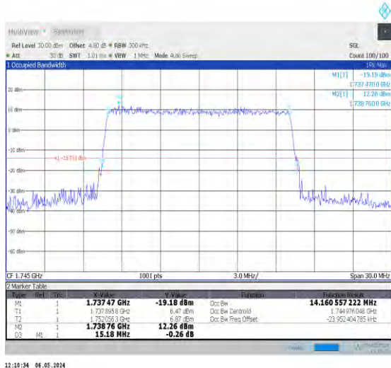
1-N66-15-15-M-9-CP-256QAM-Outer_Full-79@0-Ant 0-14.161-15.180≤15-PASS
