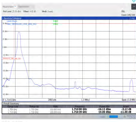
1-N66-15-10-L-4-CP-QPSK-Edge_1RB_Left-1@0-Ant0-1-seegraph-PASS-see graph
