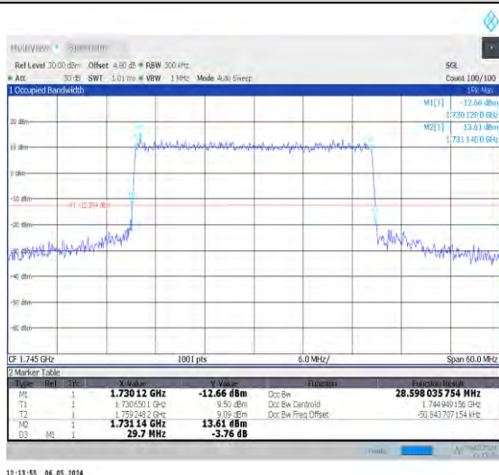
1-N66-15-30-M-3-DFT-16QAM-Outter_Full-160@0-Ant 0-28.6-29.700-≤30-PASS
