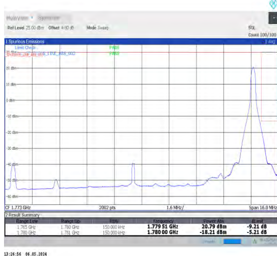
1-N66-15-15-H-5-CP-QPSK-Edge_1RB_Right-1@78-Ant0-1-seegraph-PASS-see graph
