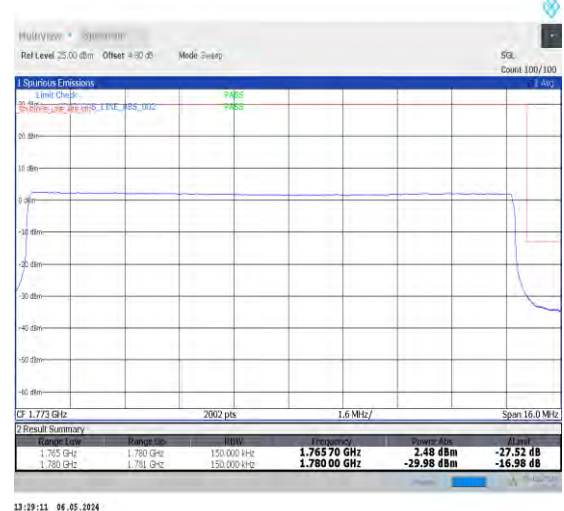
1-N66-15-15-H-6-CP-QPSK-Outer_Full-79@0-Ant0-1-seegraph-PASS-see graph
