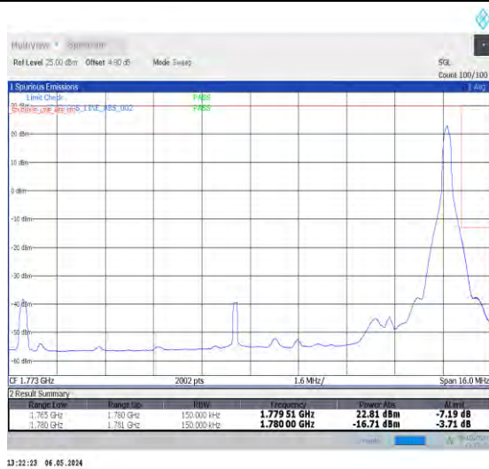
1-N66-15-15-H-2-DFT-PI2BPSK-Edge_1RB_Right-1@78-Ant0-1-seegraph-PASS-see graph
