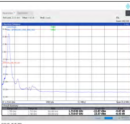
1-N66-15-30-L-1-DFT-PI2BPSK-Edge_1RB_Left-1@0-Ant0-1-seegraph-PASS-see graph
