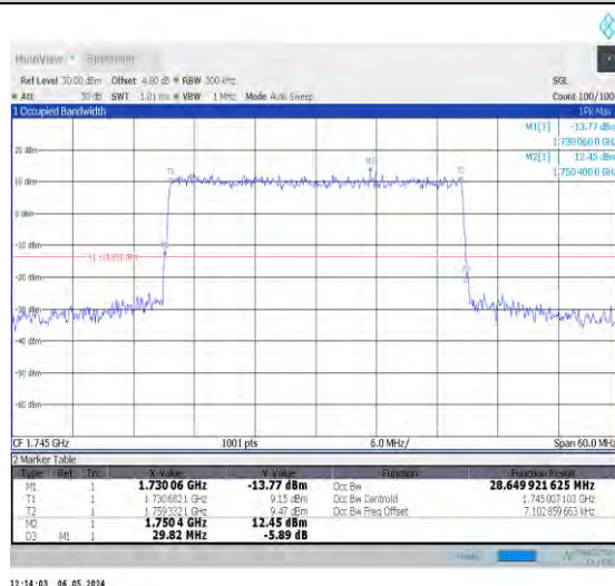
1-N66-15-30-M-4-DFT-64QAM-Outter_Full-160@0-Ant 0-28.651-29.820-≤30-PASS
