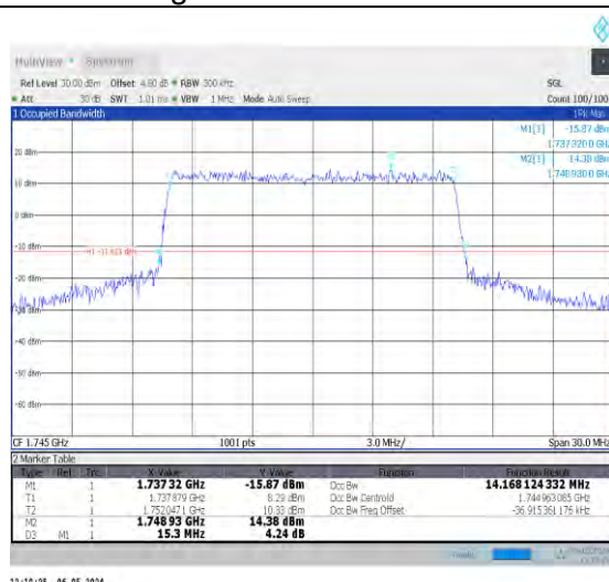
1-N66-15-15-M-8-CP-64QAM-Outer_Full-79@0-Ant0 -14.168-15.300≤15-PASS
