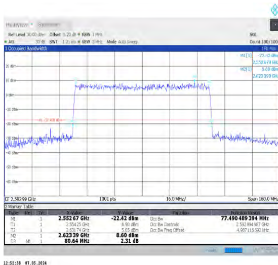
1-N41-30-80-M-9-CP-256QAM-Outer_Full-217@0-A nt0-77.49-80.640-≤80-PASS
