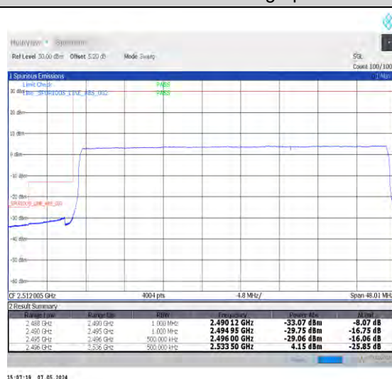
1-N41-30-40-L-6-CP-QPSK-Outer_Full-106@0-Ant0-1--PASS-see graph
