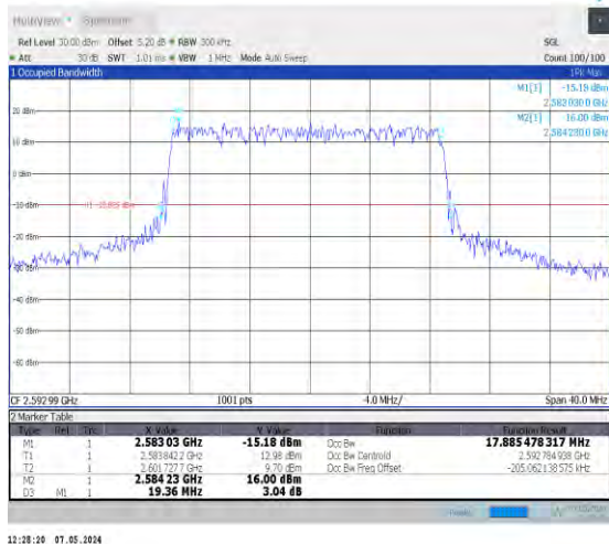
1-N41-30-20-M-1-DFT-QPSK-Outer_Full-50@0-Ant0 -17.885-19.360-≤20-PASS
