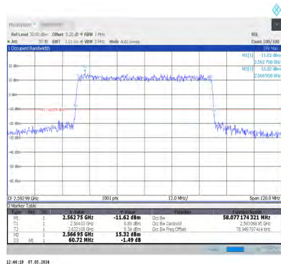
1-N41-30-60-M-4-DFT-64QAM-Outter_Full-162@0-A nt0-58.077-60.720-≤60-PASS
