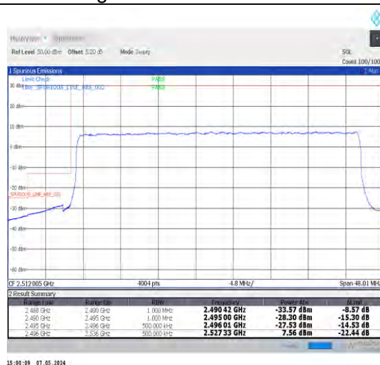
1-N41-30-40-L-3-DFT-PI2BPSK-Outer_Full-100@0-Ant0-1--PASS-see graph
