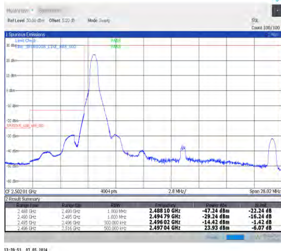
1-N41-30-20-L-4-CP-QPSK-Edge_1RB_Left-1@0-Ant0-1--PASS-see graph
