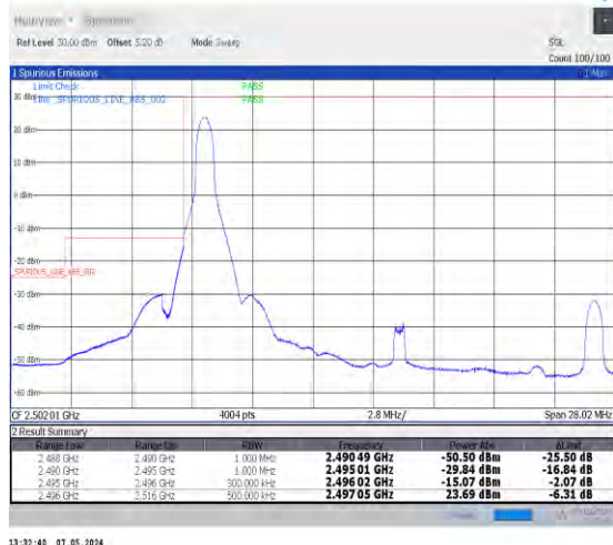
1-N41-30-20-L-1-DFT-PI2BPSK-Edge_1RB_Left-1@0-Ant0-1--PASS-see graph
