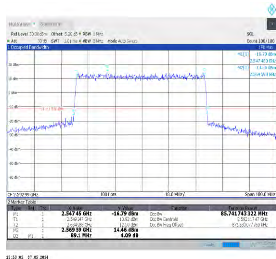
1-N41-30-90-M-1-DFT-QPSK-Outer_Full-240@0-Ant 0-85.742-89.100-≤90-PASS
