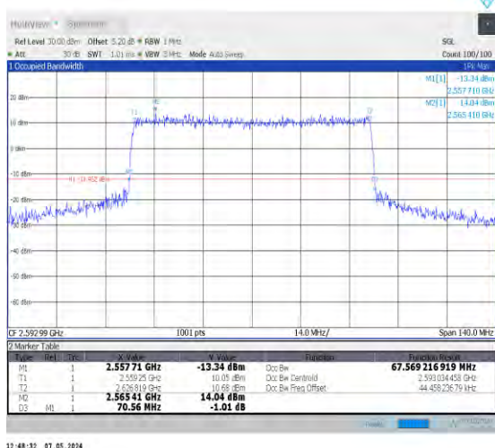
1-N41-30-70-M-6-CP-QPSK-Outer_Full-189@0-Ant0 -67.569-70.560-≤70-PASS
