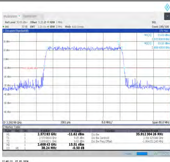
1-N41-30-40-M-5-DFT-256QAM-Outer_Full-100@0-A Ant0-35.912-38.240-≤40-PASS
