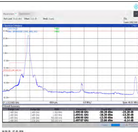
1-N41-30-40-L-1-DFT-PI2BPSK-Edge_1RB_Left-1@0-Ant0-1--PASS-see graph
