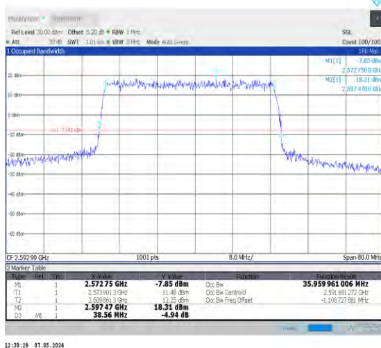
1-N41-30-40-M-1-DFT-QPSK-Outer_Full-100@0-Ant 0-35.96-38.560-≤40-PASS
