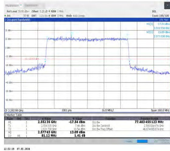
1-N41-30-80-M-8-CP-64QAM-Outer_Full-217@0-Ant 0-77.403-81.120-≤80-PASS
