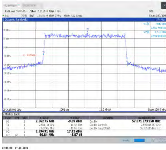
1-N41-30-60-M-1-DFT-QPSK-Outter_Full-162@0-Ant 0-57.872-60.840-≤60-PASS
