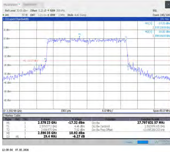
1-N41-30-30-M-8-CP-64QAM-Outer_Full-78@0-Ant0 -27.8-29.400-≤30-PASS
