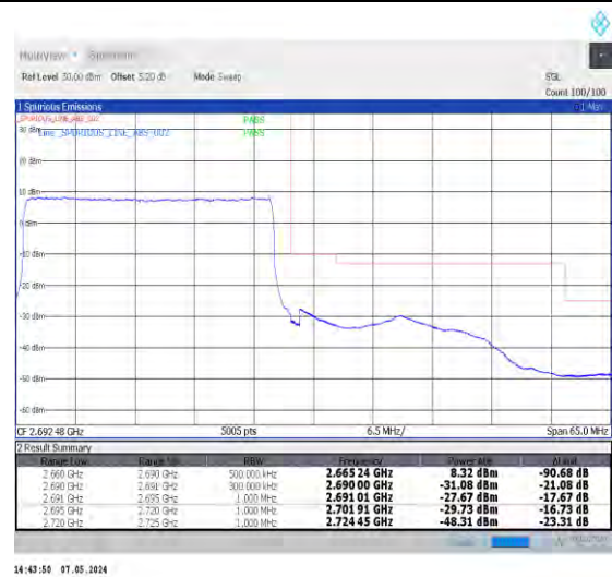
1-N41-30-30-H-3-DFT-PI2BPSK-Outer_Full-75@0-Ant0-1--PASS-see graph
