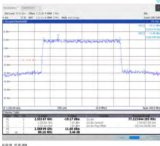
1-N41-30-80-M-5-DFT-256QAM-Outer_Full-216@0-A Ant0-77.214-80.160-<80-PASS
