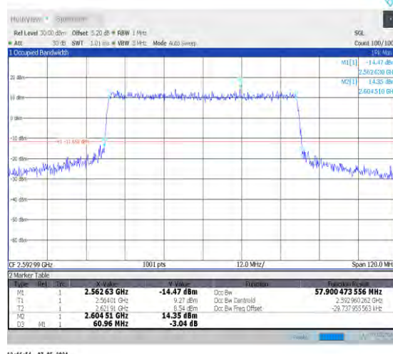
1-N41-30-60-M-8-CP-64QAM-Outer_Full-162@0-Ant0-57.900-60.960-≤60-PASS
