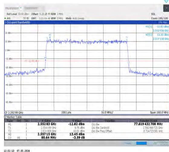
1-N41-30-80-M-6-CP-QPSK-Outer_Full-217@0-Ant0 -77.619-80.640-<80-PASS
