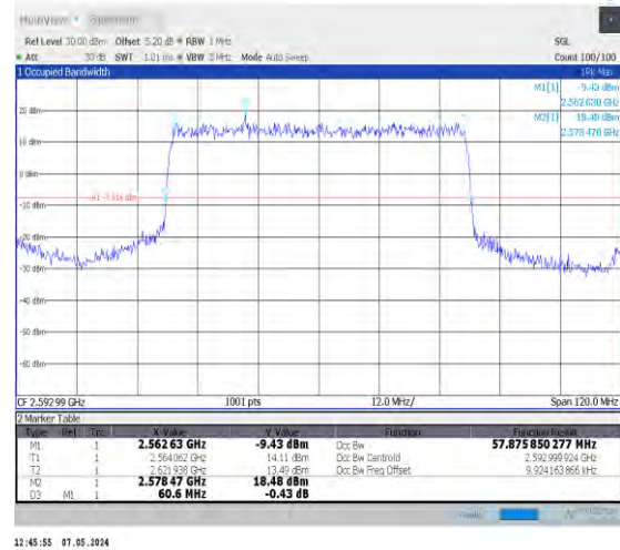
1-N41-30-60-M-2-DFT-PI2BPSK-Outter_Full-162@0-Ant 0-57.876-60.600-≤60-PASS
