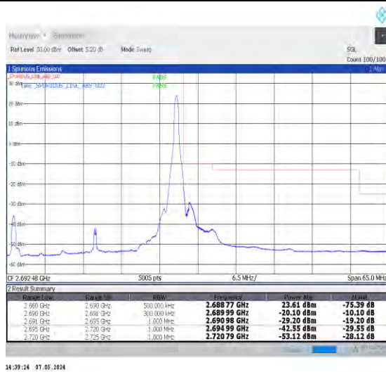
1-N41-30-30-H-2-DFT-PI2BPSK-Edge_1RB_Right-1@77-Ant0-1--PASS-see graph
