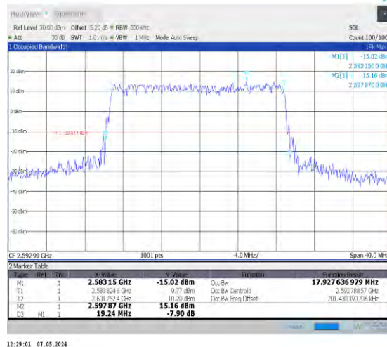
1-N41-30-20-M-4-DFT-64QAM-Outer_Full-50@0-Ant0 0-17.928-19.240-≤20-PASS
