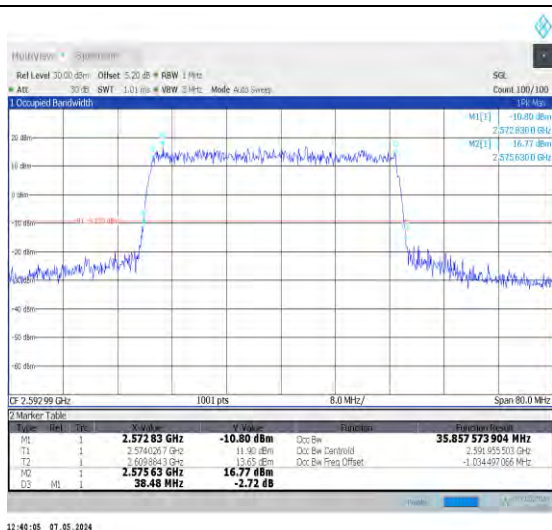
1-N41-30-40-M-3-DFT-16QAM-Outer_Full-100@0-A nt0-35.858-38.480-≤40-PASS
