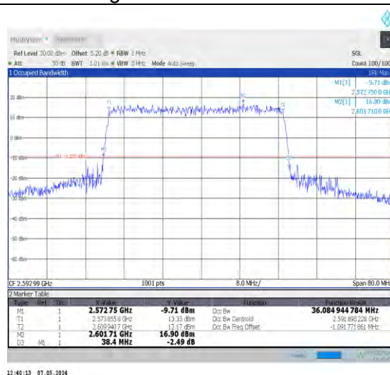
1-N41-30-40-M-4-DFT-64QAM-Outer_Full-100@0-A nt0-36.085-38.400-≤40-PASS
