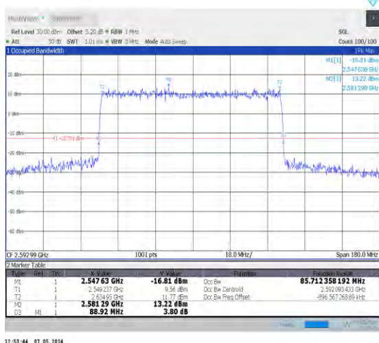
1-N41-30-90-M-4-DFT-64QAM-Outer_Full-240@0-A nt0-85.712-88.920-≤90-PASS
