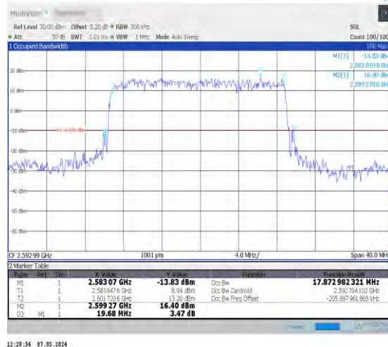
1-N41-30-20-M-2-DFT-PI2BPSK-Outer_Full-50@0-Ant0 -17.873-19.680-≤20-PASS
