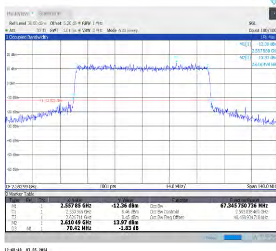
1-N41-30-70-M-7-CP-16QAM-Outer_Full-189@0-Ant 0-67.346-70.420-≤70-PASS
