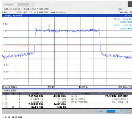
1-N41-30-80-M-7-CP-16QAM-Outer_Full-217@0-Ant 0-77.325-80.640-≤80-PASS
