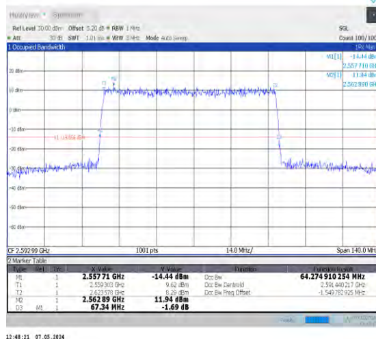
1-N41-30-70-M-5-DFT-256QAM-Outer_Full-180@0-A Ant0-64.275-67.340-≤70-PASS
