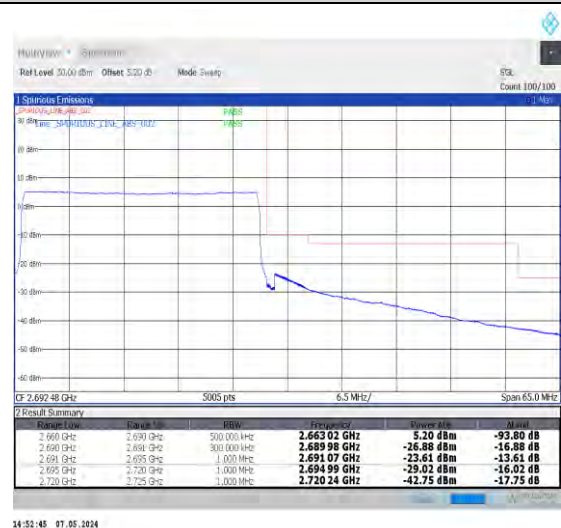
1-N41-30-30-H-6-CP-QPSK-Outer_Full-78@0-Ant0-1--PASS-see graph
