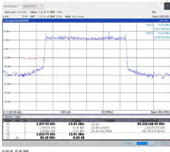
1-N41-30-90-M-2-DFT-PI2BPSK-Outer_Full-240@0-A Ant0-85.526-89.280-≤90-PASS
