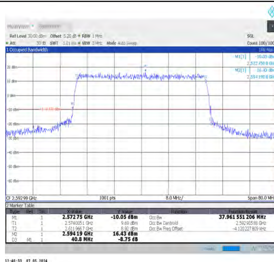
1-N41-30-40-M-6-CP-QPSK-Outer_Full-106@0-A nt0-37.962-40.800-≤40-PASS
