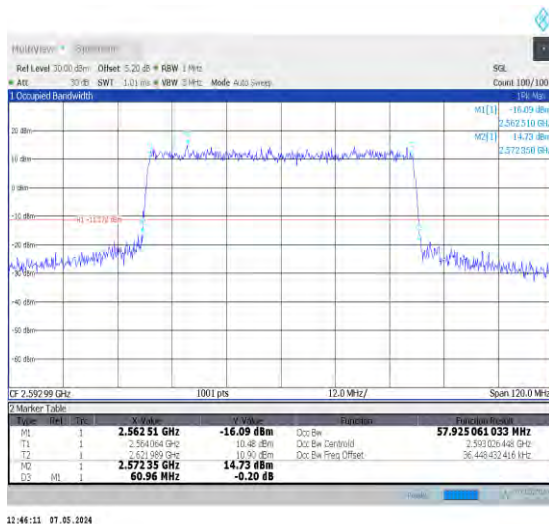
1-N41-30-60-M-3-DFT-16QAM-Outter_Full-162@0-A nt0-57.925-60.960-≤60-PASS
