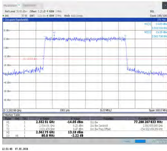
1-N41-30-80-M-3-DFT-16QAM-Outer_Full-216@0-A nt0-77.288-80.800-<80-PASS
