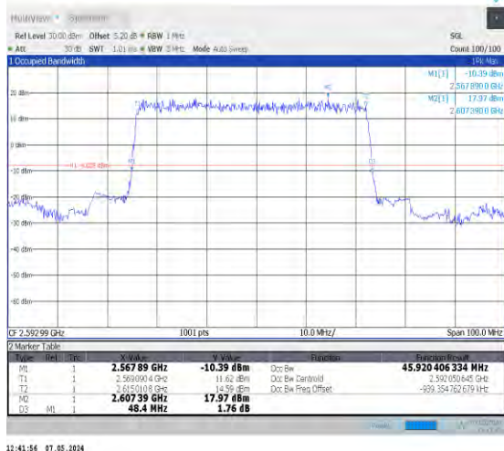
1-N41-30-50-M-2-DFT-PI2BPSK-Outer_Full-128@0-Ant0-45.92-48.400-≤50-PASS
