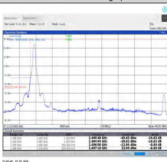
1-N41-30-40-L-4-CP-QPSK-Edge_1RB_Left-1@0-Ant0-1--PASS-see graph
