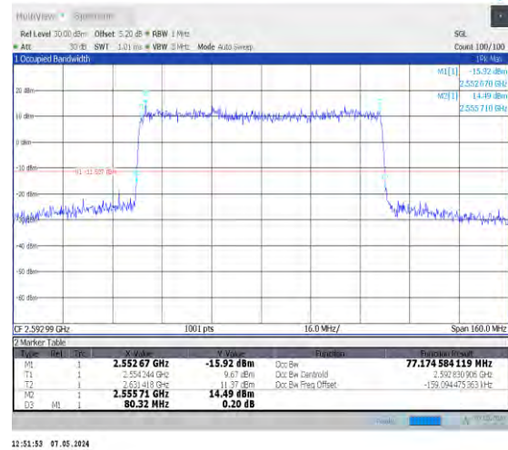
1-N41-30-80-M-4-DFT-64QAM-Outer_Full-216@0-A nt0-77.175-80.320-<80-PASS
