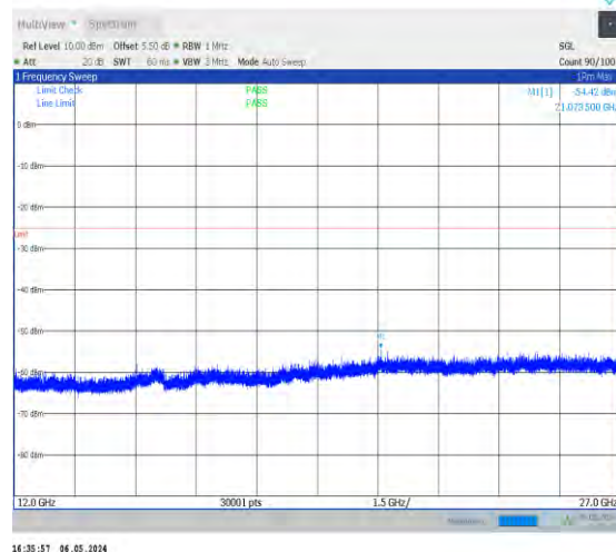
1-N38-30-40-H-1-DFT-PI2BPSK-Inner_1RB_Left-1@ 1-12000-27000-Ant0-21073.50--54.42--25-PASS
