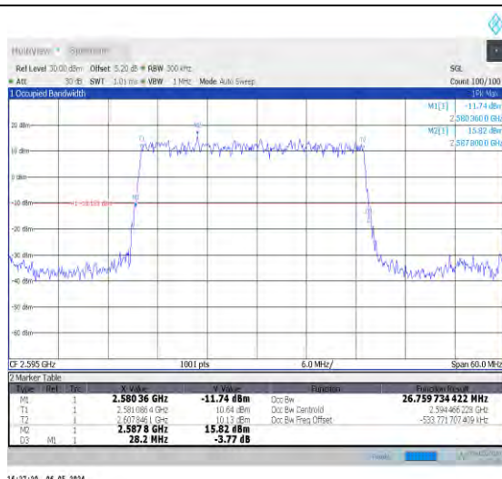
1-N38-30-30-M-2-DFT-PI2BPSK-Outer_Full-75@0-A nt0-26.762-28.200-≤30-PASS
