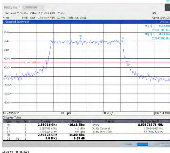
1-N38-30-10-M-3-DFT-16QAM-Outer_Full-24@0-Ant0 0-8.58-9.800-≤10-PASS
