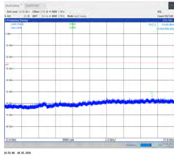
1-N38-30-40-L-1-DFT-PI2BPSK-Inner_1RB_Left-1@ 1-12000-27000-Ant0-25005.00--54.60--25-PASS
