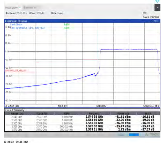
1-N38-30-20-L-6-CP-QPSK-Outer_Full-51@0-Ant0-1--PASS-see graph
