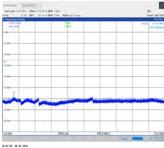
1-N38-30-40-L-1-DFT-PI2BPSK-Inner_1RB_Left-1 @ 1-3000-12000-Ant0-3621.90--57.45--25-PASS
