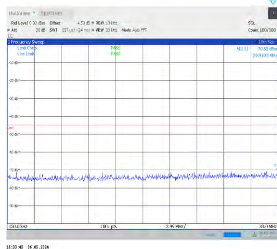
1-N38-30-40-M-1-DFT-PI2BPSK-Inner_1RB_Left-1@ 1-0.15-30-Ant0-29.91--70.55--45-PASS
