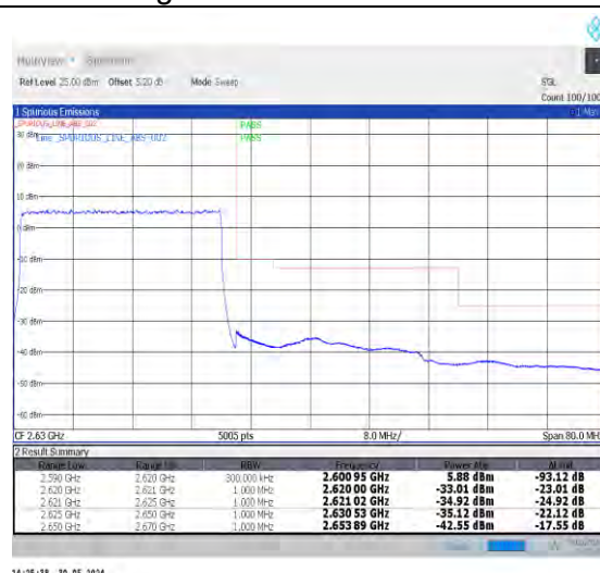
1-N38-30-30-H-3-DFT-PI2BPSK-Outer_Full-75@0-Ant0-1--PASS-see graph
