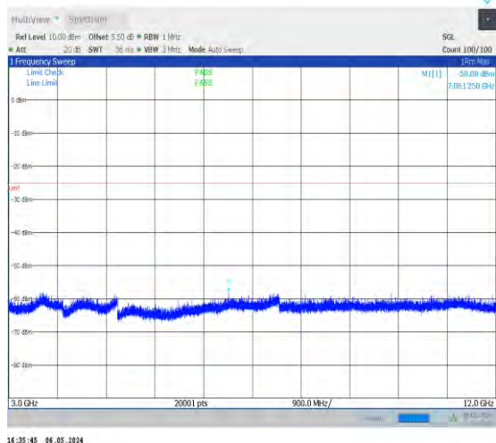
1-N38-30-40-H-1-DFT-PI2BPSK-Inner_1RB_Left-1 @1-3000-12000-Ant0-7061.25--58.08--25-PASS
