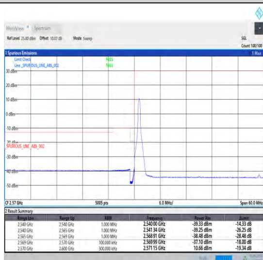
1-N38-30-30-L-4-CP-QPSK-Edge_1RB_Left-1@0-Ant0-1--PASS-see graph
