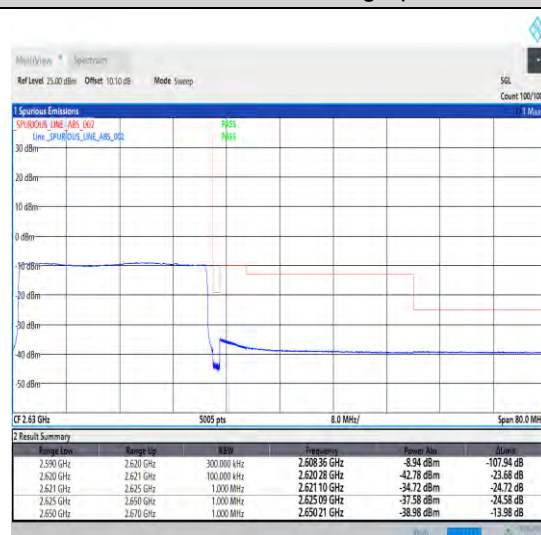
1-N38-30-30-H-6-CP-QPSK-Outer_Full-78@0-Ant0-1--PASS-see graph
