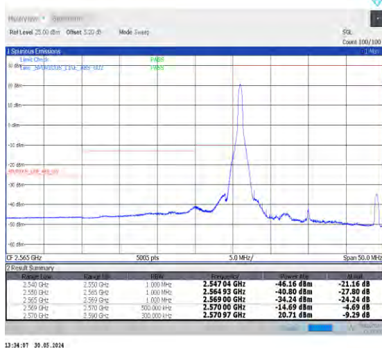
1-N38-30-20-L-4-CP-QPSK-Edge_1RB_Left-1@0-Ant0-1--PASS-see graph
