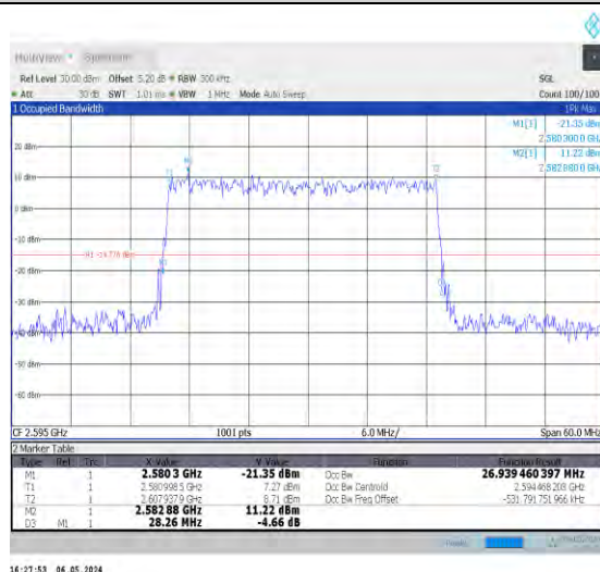
1-N38-30-30-M-5-DFT-256QAM-Outer_Full-75@0-A nt0-26.941-28.260-≤30-PASS
