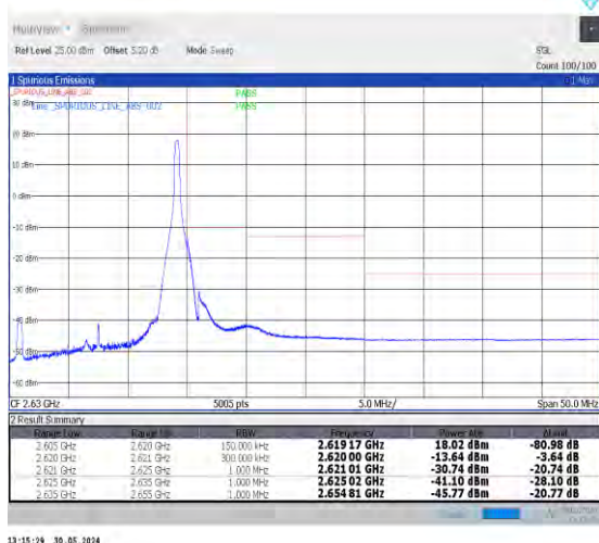
1-N38-30-15-H-5-CP-QPSK-Edge_1RB_Right-1@37-Ant0-1--PASS-see graph
