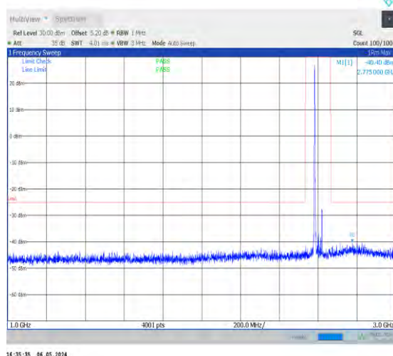
1-N38-30-40-H-1-DFT-PI2BPSK-Inner_1RB_Left-1@ 1-1000-3000-Ant0-2775.00--40.40--25-PASS
