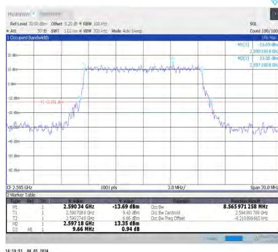
1-N38-30-10-M-2-DFT-PI2BPSK-Outer_Full-24@0-Ant0 -8.566-9.660-≤10-PASS
