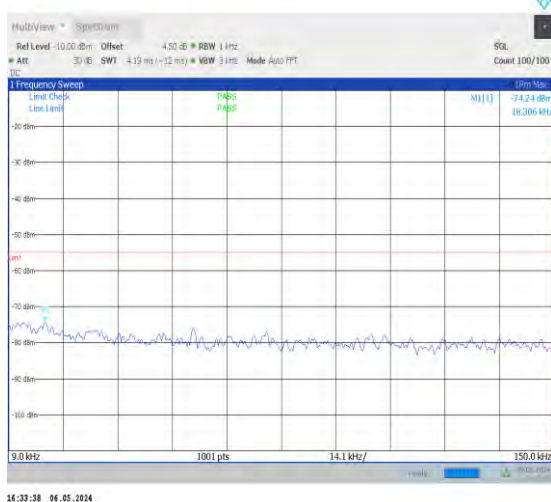
1-N38-30-40-M-1-DFT-PI2BPSK-Inner_1RB_Left-1 @ 1-0.009-0.15-Ant0-0.02--74.24--55-PASS
