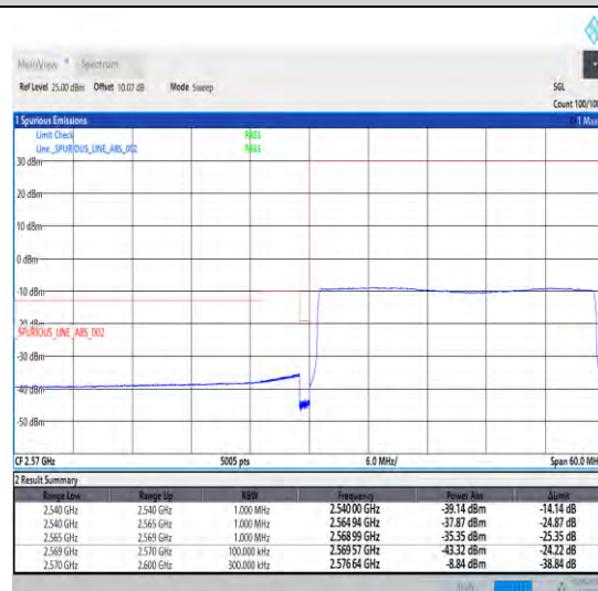
1-N38-30-30-L-6-CP-QPSK-Outer_Full-78@0-Ant0-1--PASS-see graph
