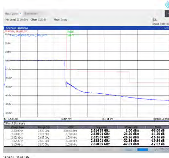
1-N38-30-30-H-6-CP-QPSK-Outer_Full-78@0-Ant0-1--PASS-see graph
