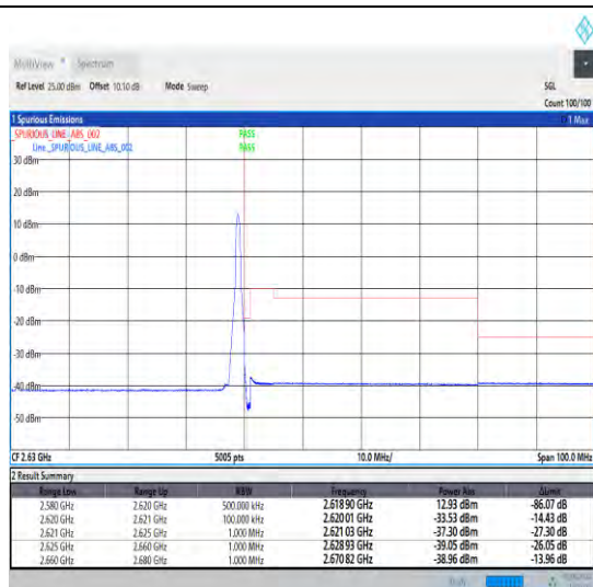
1-N38-30-40-H-2-DFT-PI2BPSK-Edge_1RB_Right-1@105-Ant0-1--PASS-see graph
