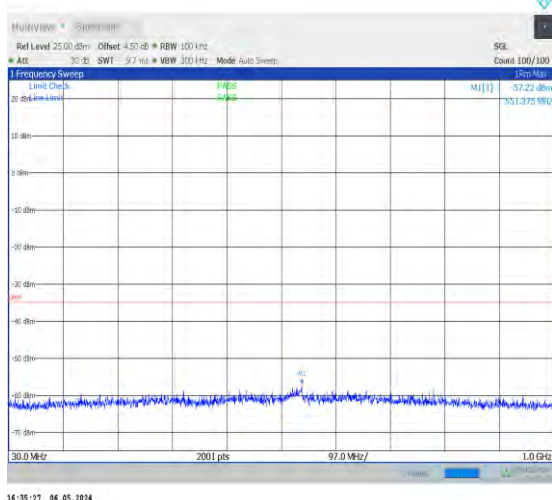
1-N38-30-40-H-1-DFT-PI2BPSK-Inner_1RB_Left-1 @1-30-1000-Ant0-551.38--57.22--35-PASS
