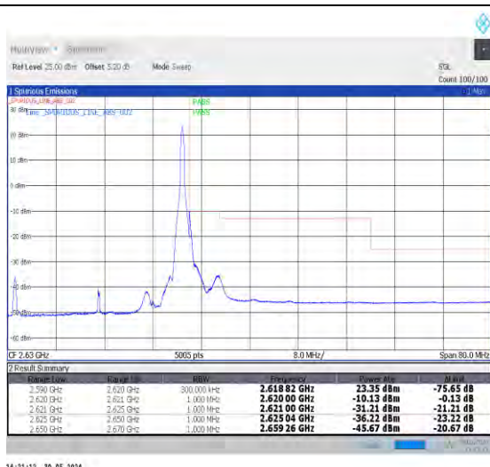
1-N38-30-30-H-2-DFT-PI2BPSK-Edge_1RB_Right-1@77-Ant0-1--PASS-see graph
