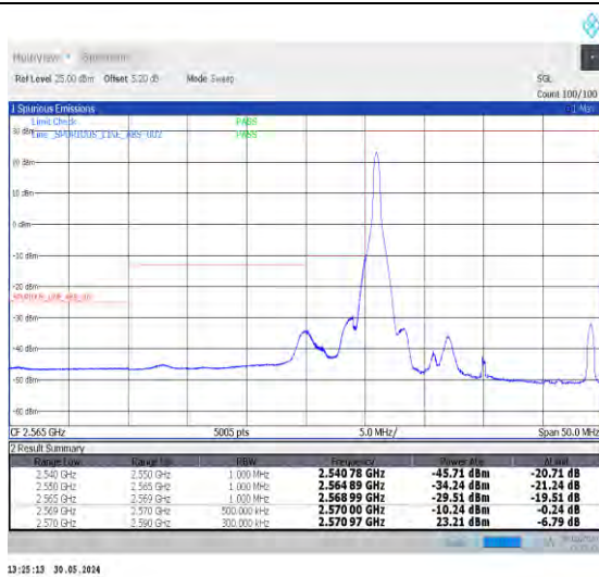
1-N38-30-20-L-1-DFT-PI2BPSK-Edge_1RB_Left-1@0-Ant0-1--PASS-see graph
