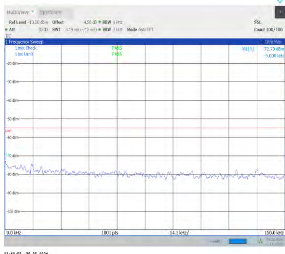
1-N38-30-40-H-1-DFT-PI2BPSK-Inner_1RB_Left-1 @1-0.009-0.15-Ant0-0.01--72.79--55-PASS
