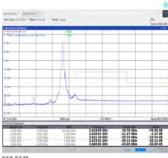
1-N38-30-30-H-5-CP-QPSK-Edge_1RB_Right-1@77-Ant0-1--PASS-see graph
