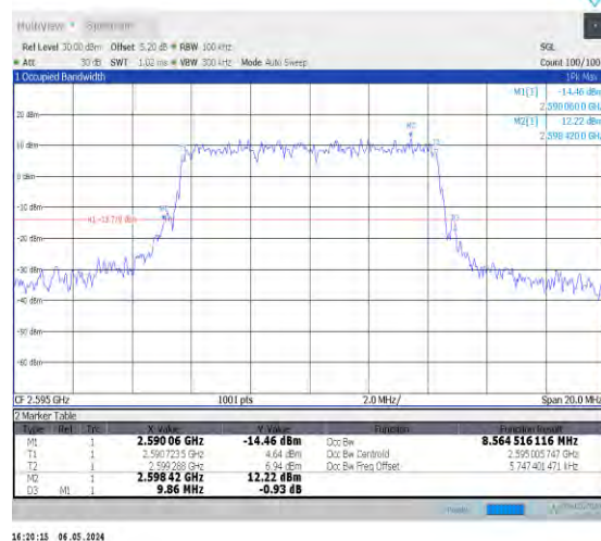
1-N38-30-10-M-4-DFT-64QAM-Outer_Full-24@0-Ant0 0-8.565-9.860-≤10-PASS
