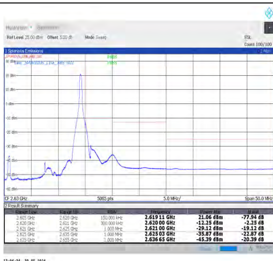
1-N38-30-15-H-2-DFT-PI2BPSK-Edge_1RB_Right-1@37-Ant0-1--PASS-see graph
