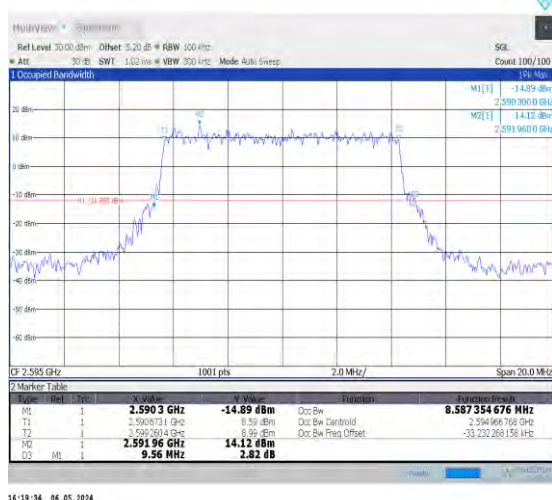
1-N38-30-10-M-1-DFT-QPSK-Outer_Full-24@0-Ant0 -8.587-9.560-≤10-PASS
