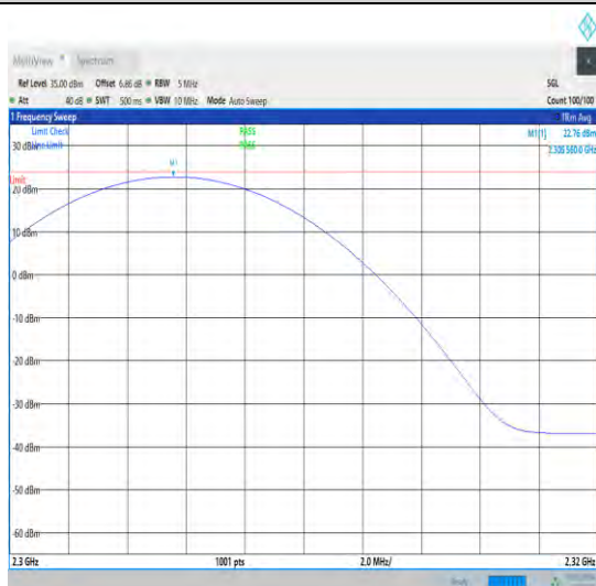
1-N30-15-10-H-1-DFT-PI2BPSK-Inner_1RB_Left-1@ 1-2300-2320-Ant1-2305.56-22.76-23.98-PASS
