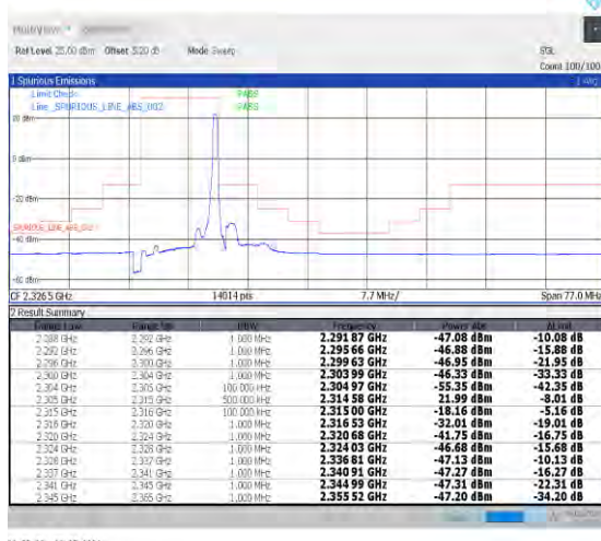
1-N30-PC3-15-10-H-5-CP-QPSK-Edge_1RB_Right-1@51-Ant0-1--PASS-see graph
