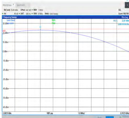
1-N30-15-5-L-1-DFT-PI2BPSK-Inner_1RB_Left-1@1 -2302.5-2312.5-Ant1-2305.51-22.67-23.98-PASS
