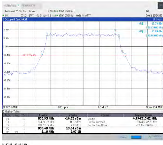
1-N26-824-849-15-5-M-1-DFT-QPSK-Outet_Full-25 @0-Ant0-4.494-5.160-≤5-PASS
