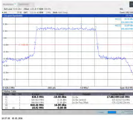
1-N26-824-849-15-20-M-2-DFT-PI2BPSK-Outer_Full -100@0-Ant0-17.882-18.920-≤20-PASS
