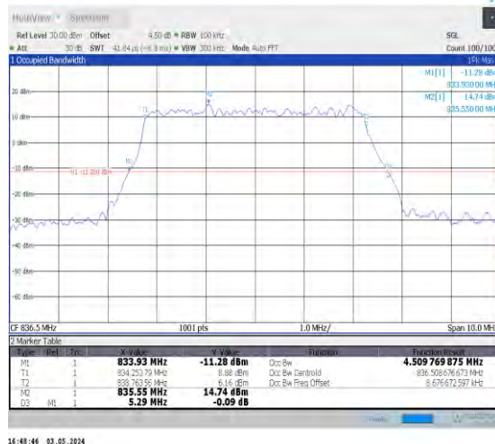
1-N26-824-849-15-5-M-6-CP-QPSK-Outer_Full-25@ 0-Ant0-4.51-5.290≤5-PASS
