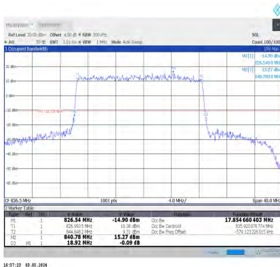
1-N26-824-849-15-20-M-4-DFT-64QAM-Outer_Full-1 00@0-Ant0-17.855-18.920-≤20-PASS
