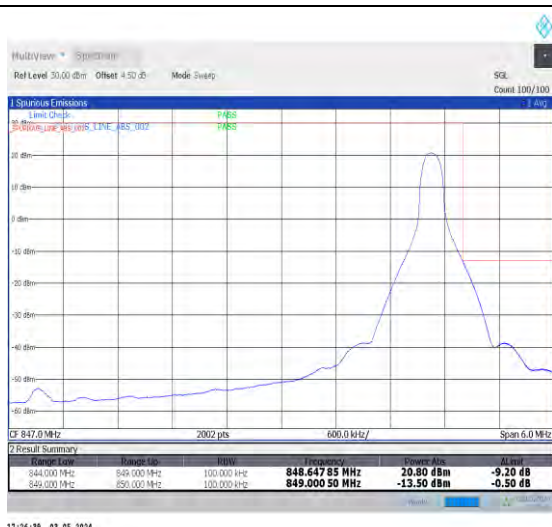
1-N26-824-849-15-5-H-2-DFT-PI2BPSK-Edge_1RB_Right-1@24-Ant0-1-seegraph-PASS-see graph
