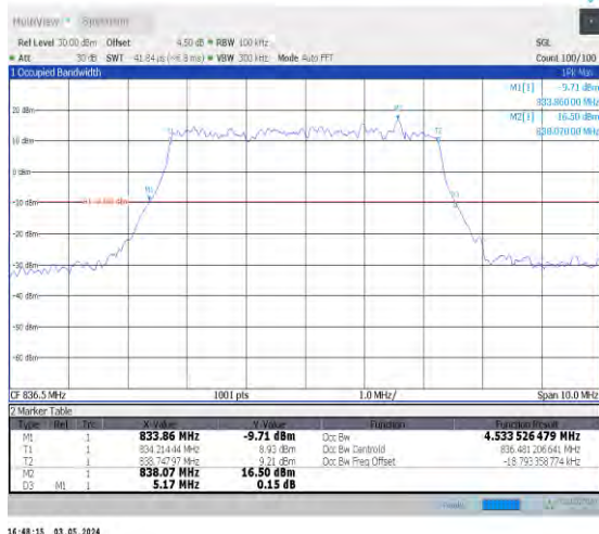
1-N26-824-849-15-5-M-3-DFT-16QAM-Outet_Full-25 @0-Ant0-4.534-5.170-≤5-PASS
