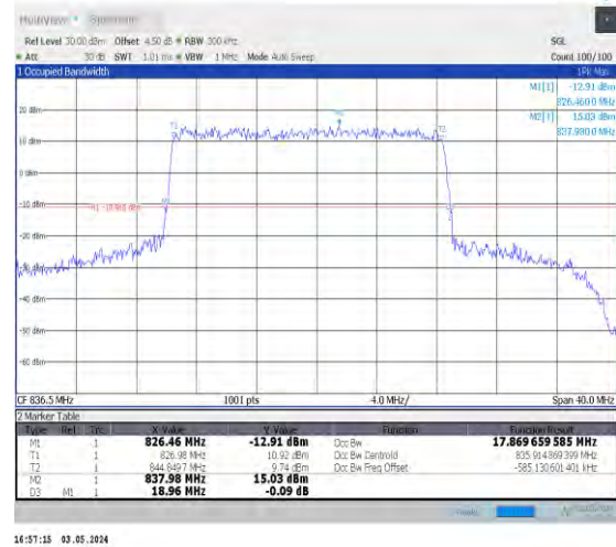
1-N26-824-849-15-20-M-3-DFT-16QAM-Outer_Full- 100@0-Ant0-17.87-18.960-≤20-PASS
