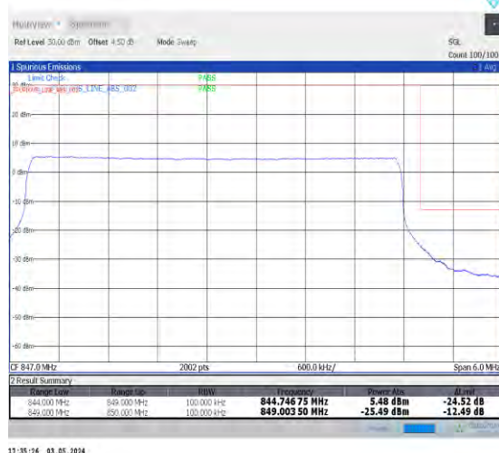
1-N26-824-849-15-5-H-6-CP-QPSK-Outer_Full-25@0-Ant0-1-seegraph-PASS-see graph
