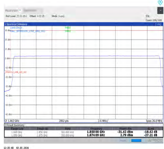
1-N25-PC3-15-25-L-6-CP-QPSK-Outer_Full-133@0-Ant0-1-seegraph-PASS-see graph
