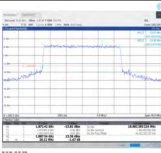
1-N25-PC3-15-20-M-8-CP-64QAM-Outer_Full-106@ 0-Ant0-18.982-20.120-≤20-PASS
