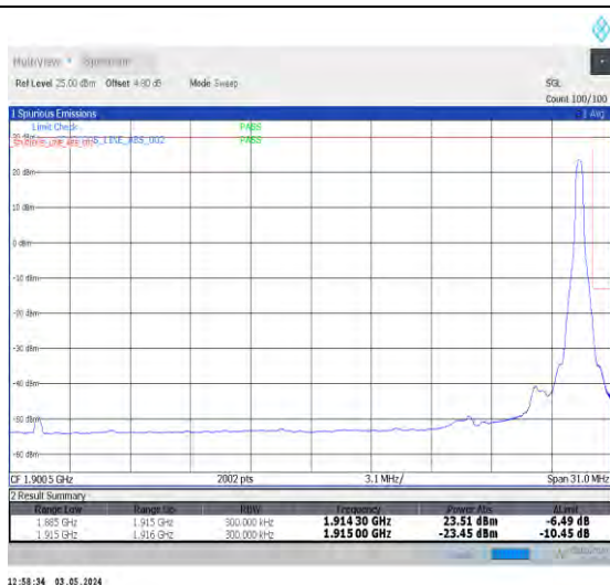
1-N25-PC3-15-30-H-2-DFT-PI2BPSK-Edge_1RB_Right-t-1@159-Ant0-1-seegraph-PASS-see graph
