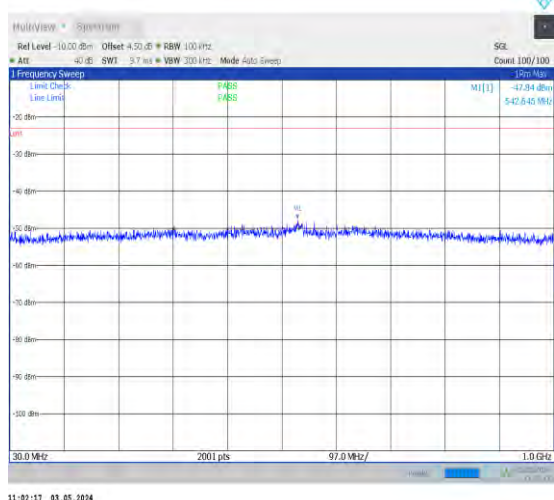
1-N25-PC3-15-40-H-1-DFT-PI2BPSK-Inner_1RB_L eft-1@1-30-1000-Ant0-542.65--47.84--23-PASS
