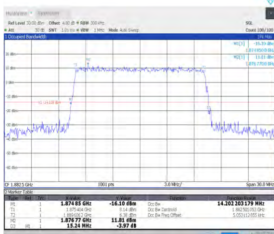
1-N25-PC3-15-15-M-9-CP-256QAM-Outer_Full-79@0 0-Ant0-14.202-15.240-≤15-PASS
