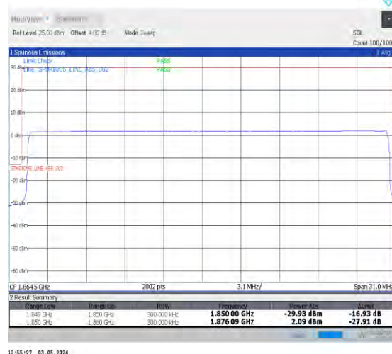
1-N25-PC3-15-30-L-6-CP-QPSK-Outer_Full-160@0-Ant0-1-seegraph-PASS-see graph
