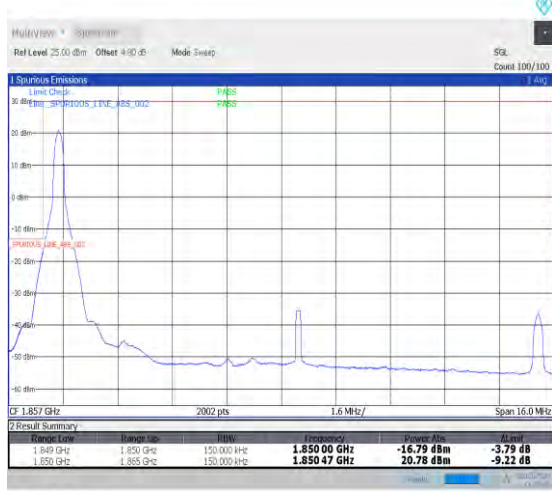
1-N25-PC3-15-15-L-4-CP-QPSK-Edge_1RB_Left-1@0-Ant0-1-seegraph-PASS-see graph
