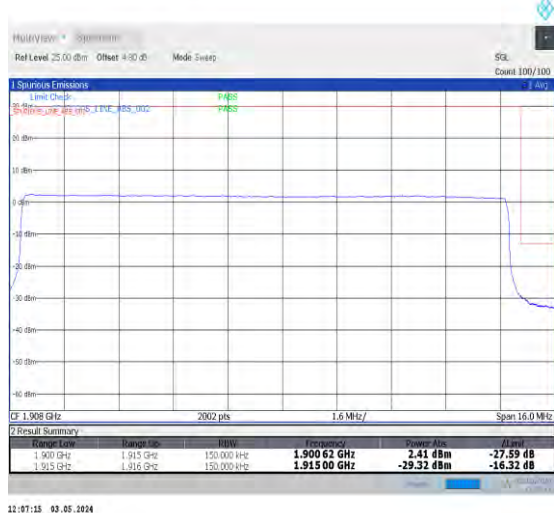
1-N25-PC3-15-15-H-6-CP-QPSK-Outer_Full-79@0-Ant0-1-seegraph-PASS-see graph
