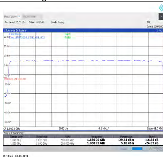
1-N25-PC3-15-40-L-3-DFT-PI2BPSK-Outer_Full-216@0-Ant0-1-seegraph-PASS-see graph
