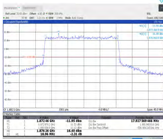
1-N25-PC3-15-20-M-1-DFT-QPSK-Outer_Full-100@0 0-Ant0-17.928-18.960-≤20-PASS
