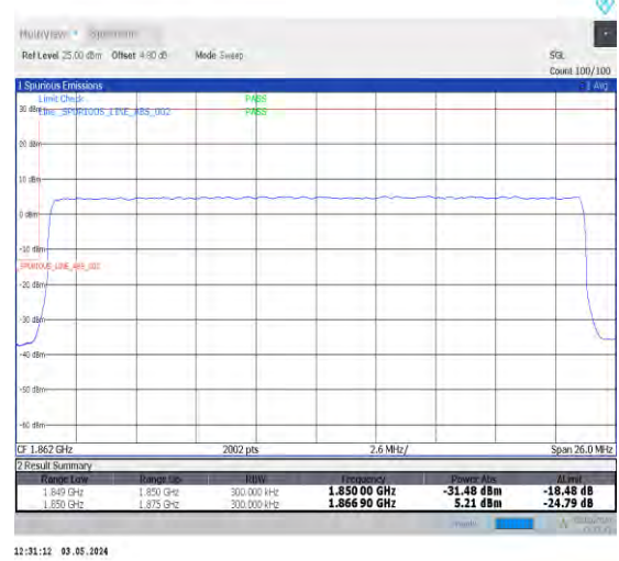
1-N25-PC3-15-25-L-3-DFT-PI2BPSK-Outer_Full-128@0-Ant0-1-seegraph-PASS-see graph
