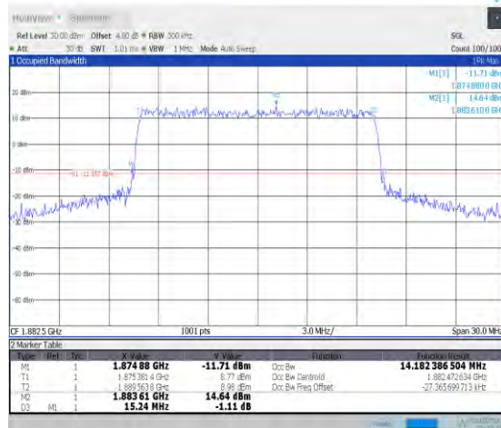
1-N25-PC3-15-15-M-8-CP-64QAM-Outer_Full-79@0 -Ant0-14.182-15.240-≤15-PASS
