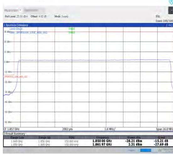
1-N25-PC3-15-15-L-6-CP-QPSK-Outer_Full-79@0-Ant0-1-seegraph-PASS-see graph
