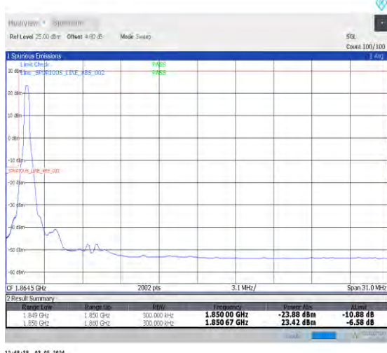
1-N25-PC3-15-30-L-1-DFT-PI2BPSK-Edge_1RB_Left-1@0-Ant0-1-seegraph-PASS-see graph
