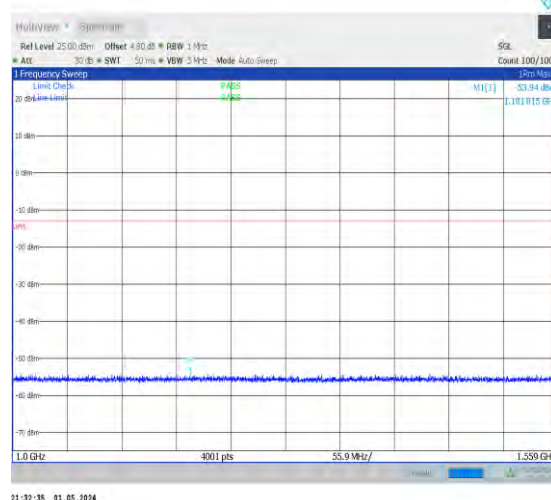
1-N14-PC3-15-10-H-1-DFT-PI2BPSK-Inner_1RB_L ef t-1@1-1000-1559-Ant0-1181.81--53.94--13-PASS
