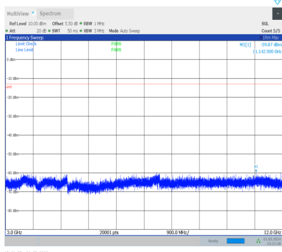
1-N13-PC3-15-10-H-1-DFT-PI2BPSK-Inner_1RB_Lef ft-1@1-3000-12000-Ant0-11142.30--59.87--13-PASS
