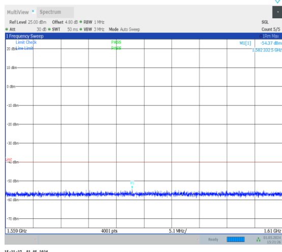
1-N13-PC3-15-10-H-1-DFT-PI2BPSK-Inner_1RB_Lef ft-1@1-1559-1610-Ant0-1582.33--54.37--40-PASS
