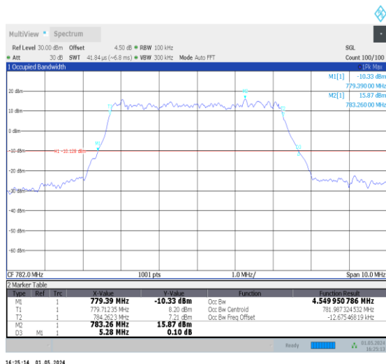
1-N13-PC3-15-5-M-3-DFT-16QAM-Outter_Full-25@0 -Ant0-4.55-5.280-≤5-PASS
