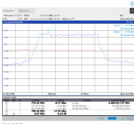
1-N13-PC3-15-5-M-1-DFT-QPSK-Outter_Full-25@0- Ant0-4.486-5.070-≤5-PASS
