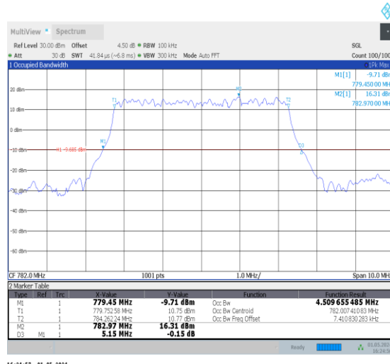
1-N13-PC3-15-5-M-2-DFT-PI2BPSK-Outter_Full-25 @0-Ant0-4.51-5.150-≤5-PASS
