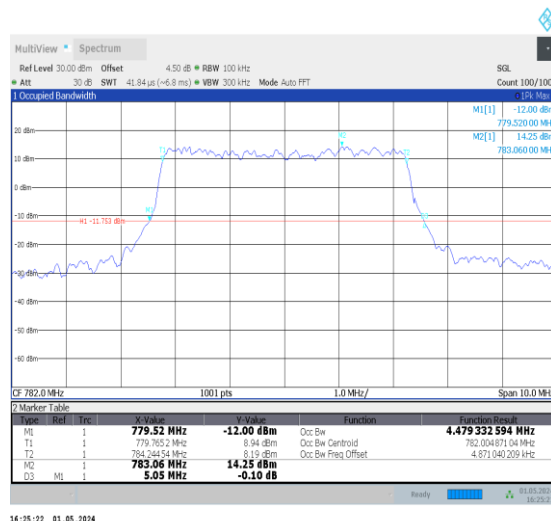
1-N13-PC3-15-5-M-4-DFT-64QAM-Outter_Full-25@0 -Ant0-4.479-5.050-≤5-PASS
