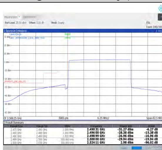
1-N7-PC3-15-25-L-3-DFT-PI2BPSK-Outer_Full-12 8@0-Ant0-1--PASS-see graph
