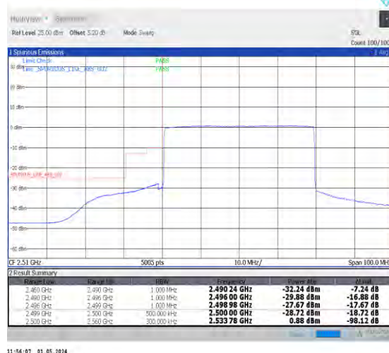
1-N7-PC3-15-40-L-6-CP-QPSK-Outer_Full-216@ 0-Ant0-1--PASS-see graph
