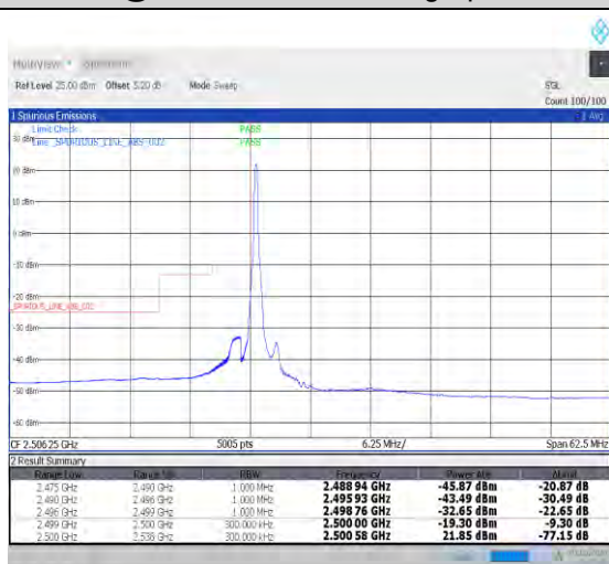
1-N7-PC3-15-25-L-1-DFT-PI2BPSK-Edge_1RB_Left-1 @0-Ant0-1--PASS-see graph
