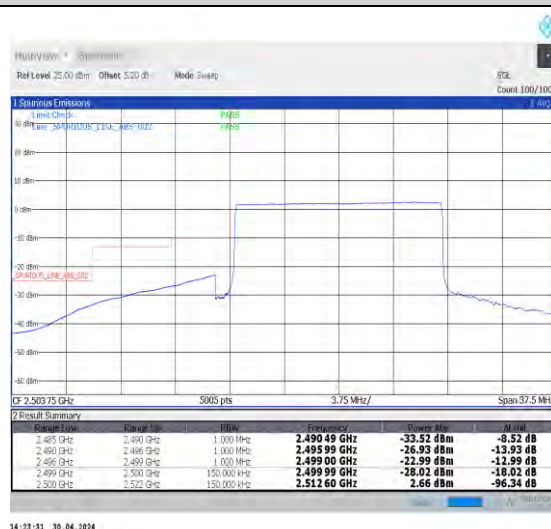
1-N7-PC3-15-15-L-6-CP-QPSK-Outer_Full-79@0- Ant0-1--PASS-see graph
