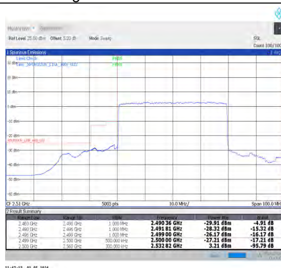
1-N7-PC3-15-40-L-3-DFT-PI2BPSK-Outer_Full-21 6@0-Ant0-1--PASS-see graph
