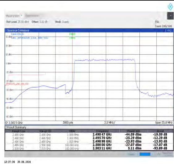
1-N7-PC3-15-10-L-3-DFT-PI2BPSK-Outer_Full-50 @0-Ant0-1--PASS-see graph
