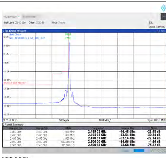
1-N7-PC3-15-40-L-1-DFT-PI2BPSK-Edge_1RB_Left-1 @0-Ant0-1--PASS-see graph
