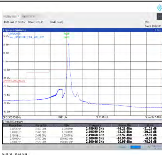
1-N7-PC3-15-15-L-4-CP-QPSK-Edge_1RB_Left-1@0- Ant0-1--PASS-see graph
