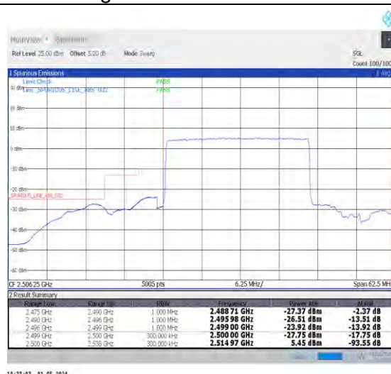
1-N7-PC3-15-25-L-3-DFT-PI2BPSK-Outer_Full-12 8@0-Ant0-1--PASS-see graph
