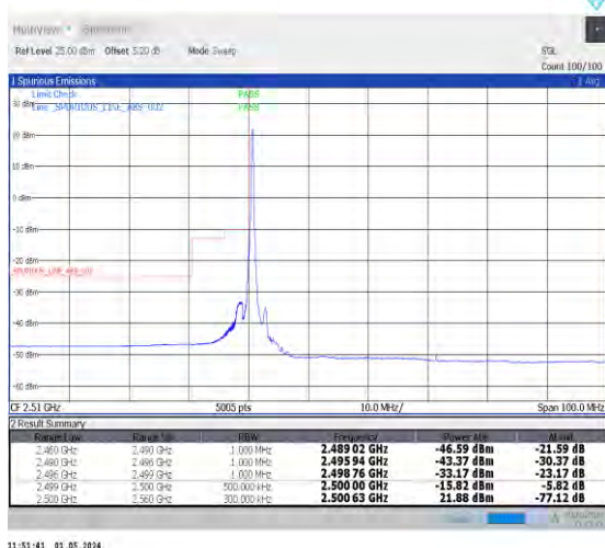
1-N7-PC3-15-40-L-4-CP-QPSK-Edge_1RB_Left-1@0- Ant0-1--PASS-see graph
