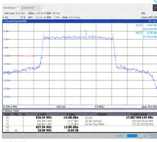
1-N5-15-20-M-4-DFT-64QAM-Outer_Full-100@0-Ant 0-17.868-18.960-≤20-PASS
