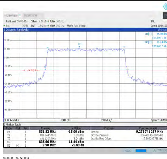
1-N5-15-10-M-7-CP-16QAM-Outer_Full-52@0-Ant0- 9.276-9.980≤10-PASS
