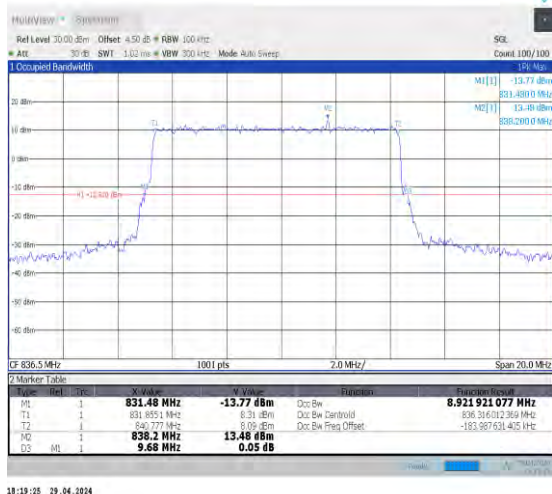
1-N5-15-10-M-4-DFT-64QAM-Outer_Full-50@0-Ant0 -8.922-9.680≤10-PASS
