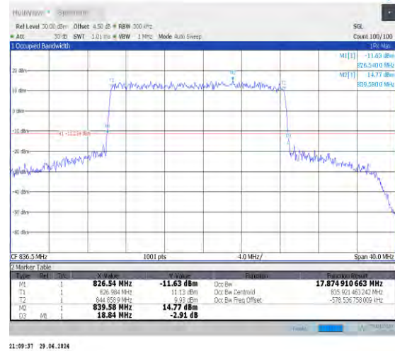
1-N5-15-20-M-3-DFT-16QAM-Outer_Full-100@0-Ant 0-17.875-18.840-≤20-PASS
