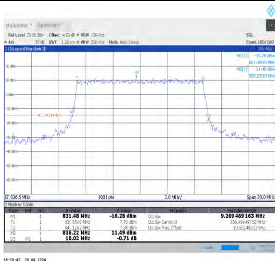
1-N5-15-10-M-6-CP-QPSK-Outer_Full-52@0-Ant0-9. 269-10.020≤10-PASS
