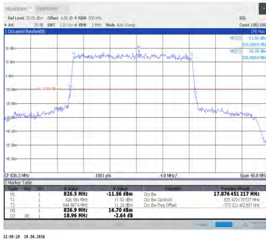
1-N5-15-20-M-2-DFT-PI2BPSK-Outer_Full-100@0-A nt0-17.876-18.960-≤20-PASS
