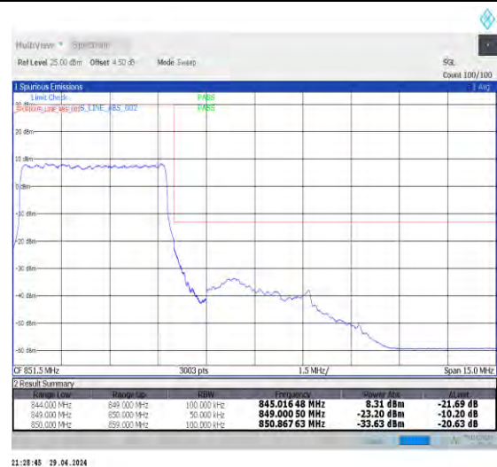
1-N5-15-5-H-3-DFT-PI2BPSK-Outer_Full-25@0-Ant0-1--PASS-see graph
