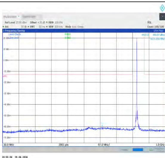
1-N5-15-20-H-1-DFT-PI2BPSK-Inner_1RB_Left-1@1 -30-1000-Ant0-623.16--60.07--13-PASS
