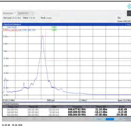
1-N5-15-5-H-5-CP-QPSK-Edge_1RB_Right-1@24-Ant0-1--PASS-see graph
