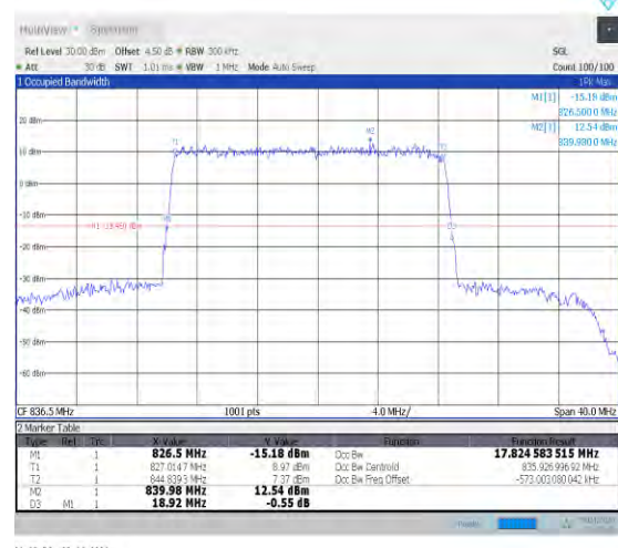
1-N5-15-20-M-5-DFT-256QAM-Outer_Full-100@0-A nt0-17.825-18.920-≤20-PASS
