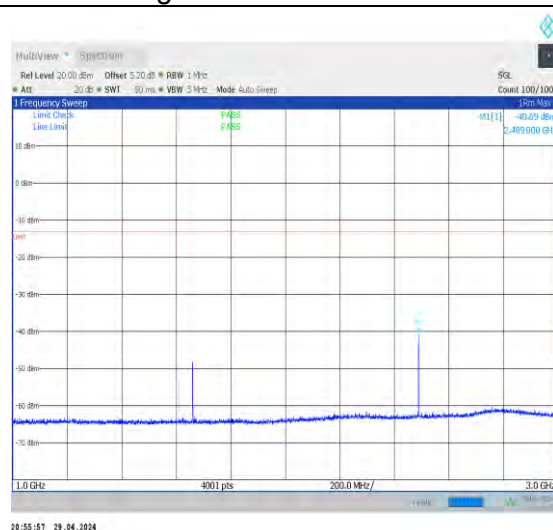
1-N5-15-20-H-1-DFT-PI2BPSK-Inner_1RB_Left-1@1 -1000-3000-Ant0-2489.00--40.69--13-PASS
