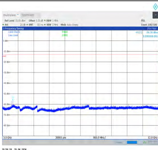
1-N5-15-20-H-1-DFT-PI2BPSK-Inner_1RB_Left-1@1 -3000-12000-Ant0-3590.85--56.36--13-PASS
