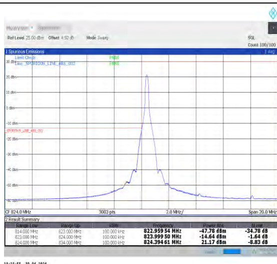
1-N5-15-10-L-1-DFT-PI2BPSK-Edge_1RB_Left-1@0-A nt0-1--PASS-see graph
