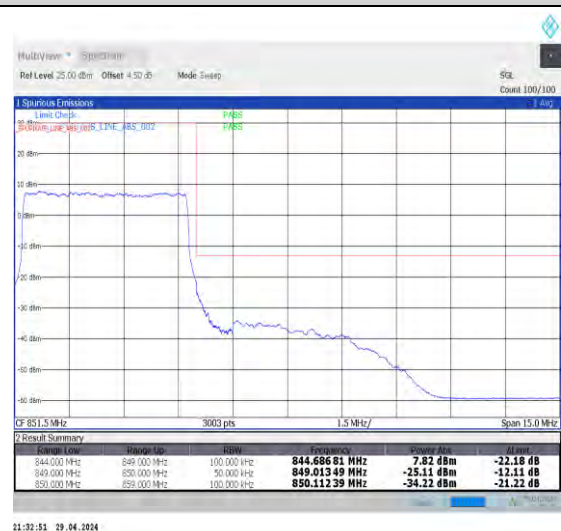
1-N5-15-5-H-6-CP-QPSK-Outer_Full-25@0-Ant0-1--PASS-see graph
