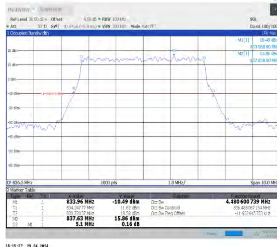
1-N5-15-5-M-2-DFT-PI2BPSK-Outet_Full-25@0-Ant 0-4.481-5.100-≤5-PASS
