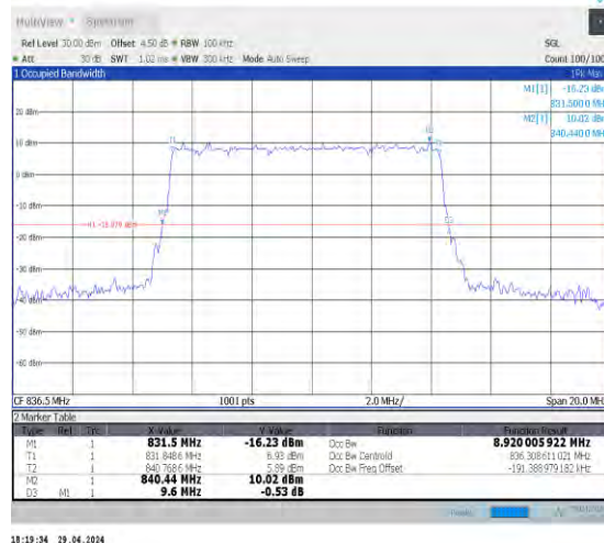
1-N5-15-10-M-5-DFT-256QAM-Outer_Full-50@0-Ant 0-8.92-9.600≤10-PASS
