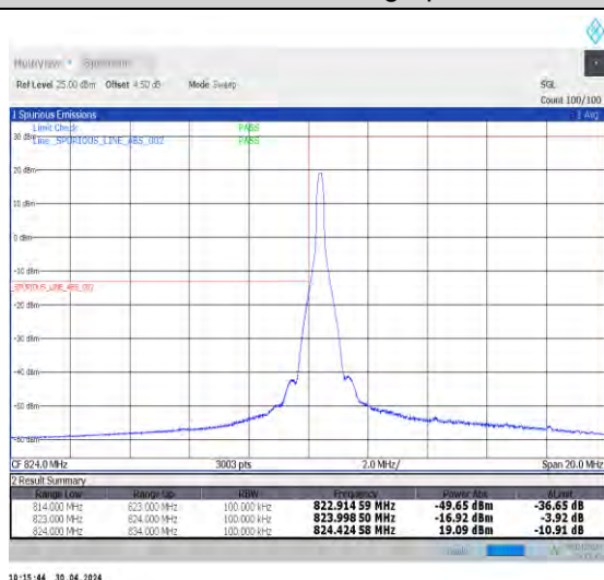
1-N5-15-10-L-4-CP-QPSK-Edge_1RB_Left-1@0-Ant0-1 1--PASS-see graph
