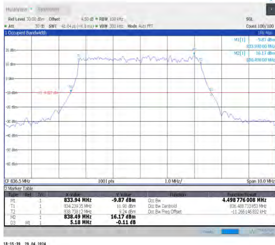
1-N5-15-5-M-1-DFT-QPSK-Outet_Full-25@0-Ant0-4. 499-5.180-≤5-PASS
