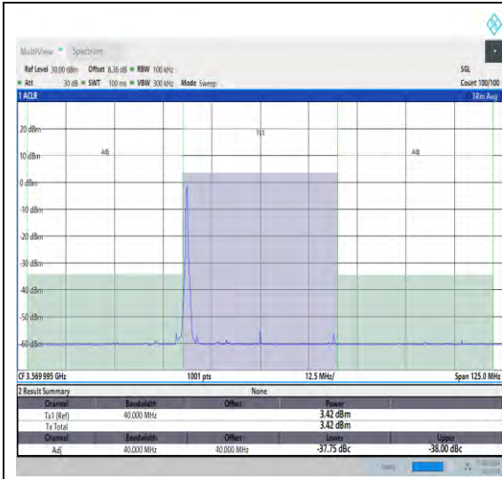
NTNV_N48_PC3_30_40_L_TID20_#1_-40_40
