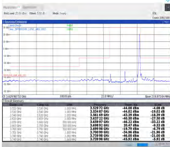
1-N48-30-40-H-5-CP-QPSK-Edge_1RB_Right-1@105-Ant0-1--PASS-see graph
