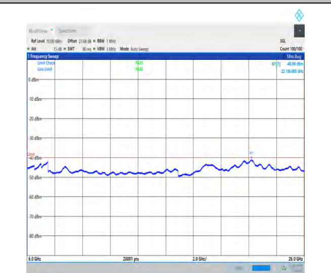
NTNV_N48_PC3_30_40_H_TID1_NS_01_6000_26000_#
