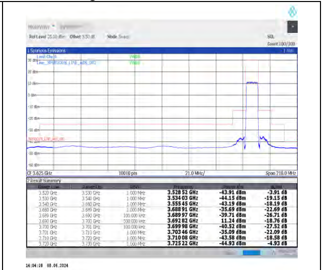
1-N48-30-10-H-3-DFT-PI2BPSK-Outer_Full-24@0-Ant0-1--PASS-see graph
