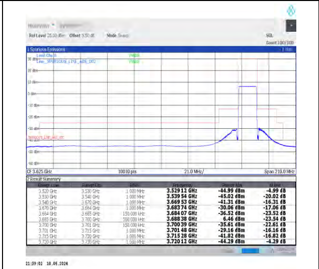
1-N48-30-15-H-6-CP-QPSK-Outer_Full-38@0-Ant0-1--PASS-see graph
