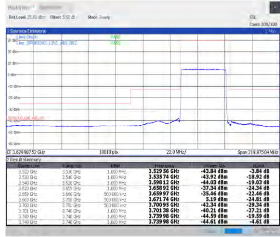
1-N48-30-40-H-3-DFT-PI2BPSK-Outer_Full-100@0-Ant0-1--PASS-see graph
