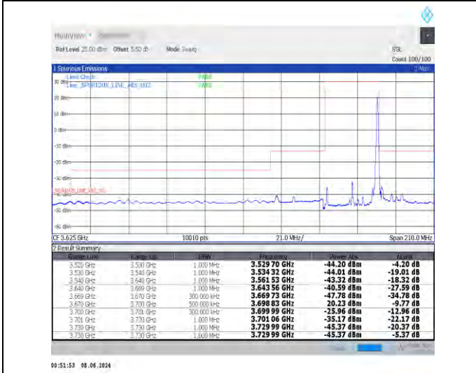
1-N48-30-30-H-5-CP-QPSK-Edge_1RB_Right-1@77-Ant0-1--PASS-see graph
