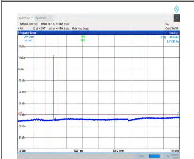
NTNV_N48_PC3_30_40_H_TID1_NS_01_30_1000_#1
