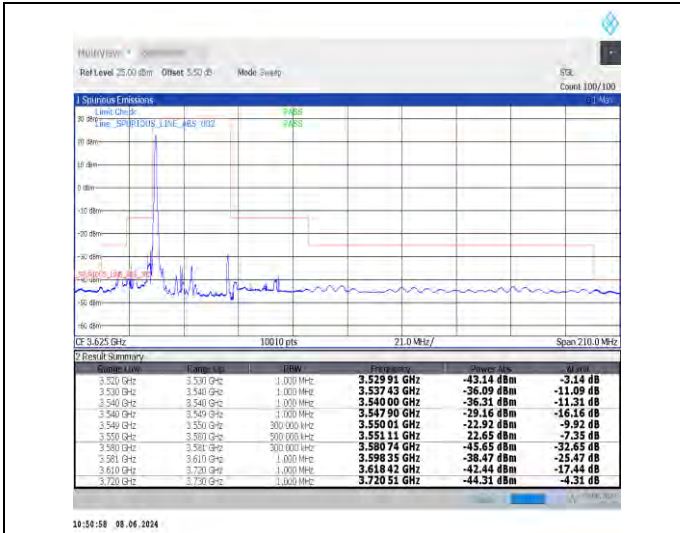
1-N48-30-30-L-1-DFT-PI2BPSK-Edge_1RB_Left-1@0-Ant0-1--PASS-see graph
