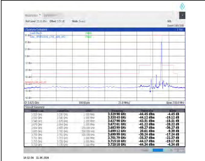
1-N48-30-15-H-5-CP-QPSK-Edge_1RB_Right-1@37-Ant0-1--PASS-see graph
