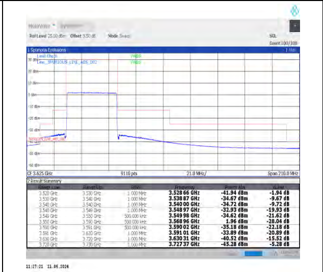
1-N48-30-40-L-6-CP-QPSK-Outer_Full-106@0-Ant0-1--PASS-see graph
