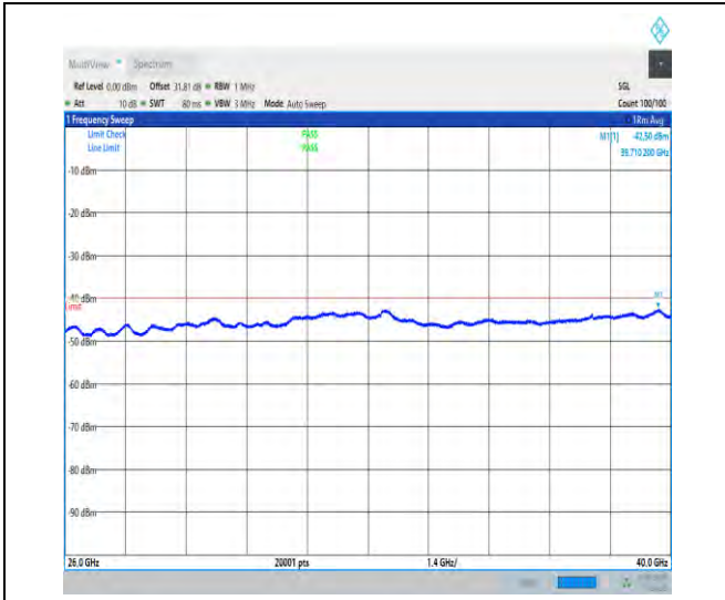
NTNV_N48_PC3_30_40_H_TID1_NS_01_26000_40000_#1
