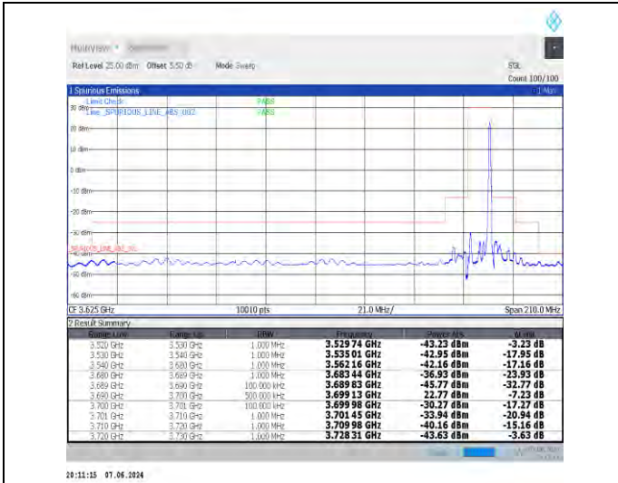
1-N48-30-10-H-2-DFT-PI2BPSK-Edge_1RB_Right-1@23-Ant0-1--PASS-see graph
