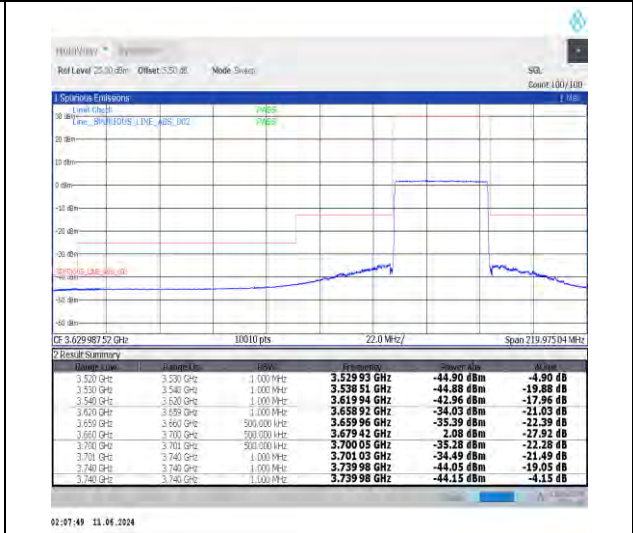
1-N48-30-40-H-6-CP-QPSK-Outer_Full-106@0-Ant0-1--PASS-see graph
