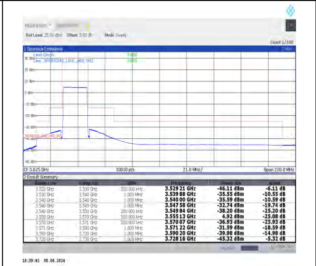
1-N48-30-20-L-6-CP-QPSK-Outer_Full-51@0-Ant0-1--PASS-see graph
