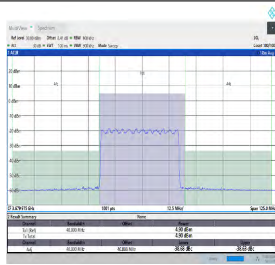
NTNV_N48_PC3_30_40_H_TID7_#1_-40_40
