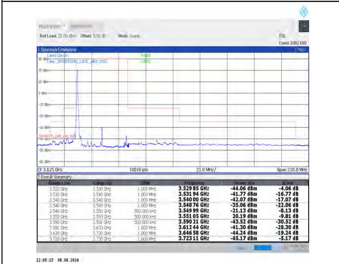
1-N48-30-40-L-4-CP-QPSK-Edge_1RB_Left-1@0-Ant0-1--PASS-see graph
