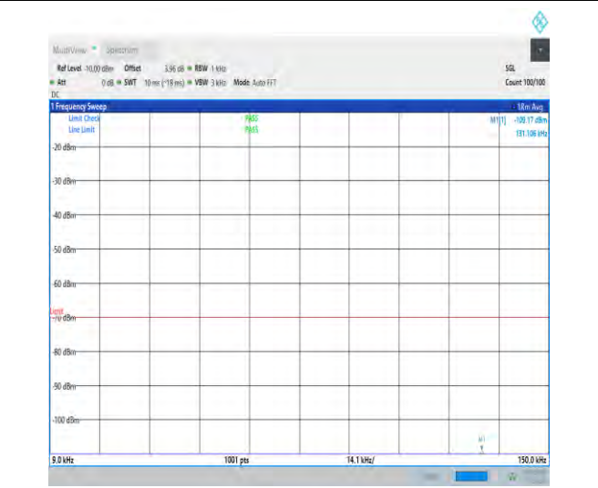
NTVN_N48_PC3_30_40_M_TID1_NS_01_0.009_0.15_#1
