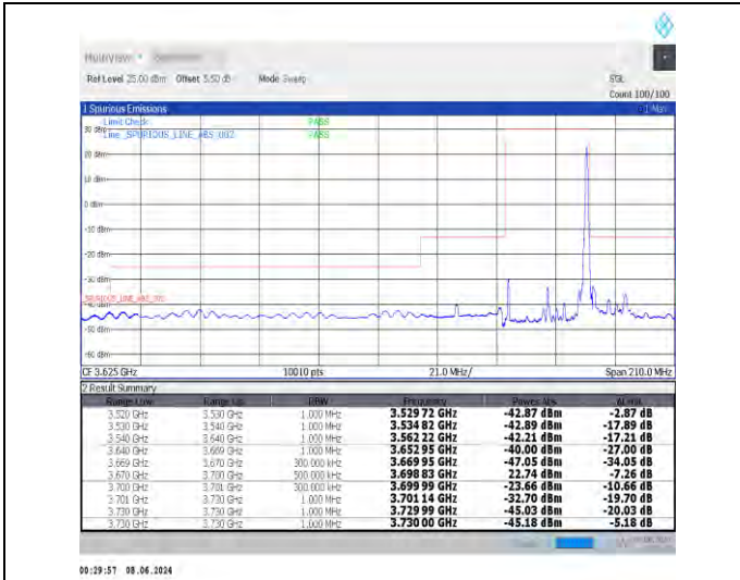
1-N48-30-30-H-2-DFT-PI2BPSK-Edge_1RB_Right-1@77-Ant0-1--PASS-see graph
