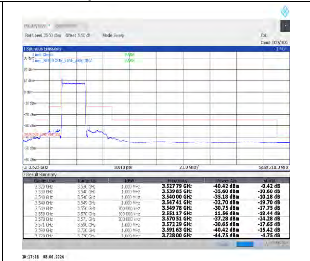
1-N48-30-20-L-3-DFT-PI2BPSK-Outer_Full-50@0-Ant0-1--PASS-see graph
