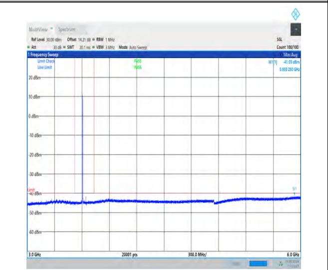
NTNV_N48_PC3_30_40_M_TID1_NS_01_3000_6000_#1
