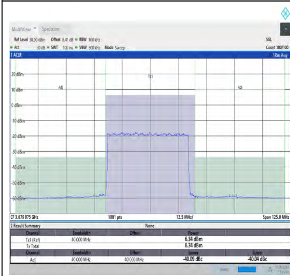
NTNV_N48_PC3_30_40_H_TID1_#1_+40_40
