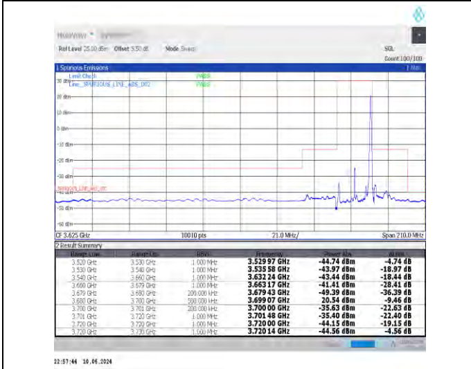
1-N48-30-20-H-5-CP-QPSK-Edge_1RB_Right-1@50-Ant0-1--PASS-see graph
