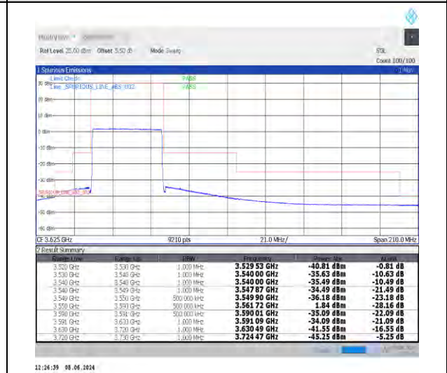
1-N48-30-40-L-6-CP-QPSK-Outer_Full-106@0-Ant0-1--PASS-see graph
