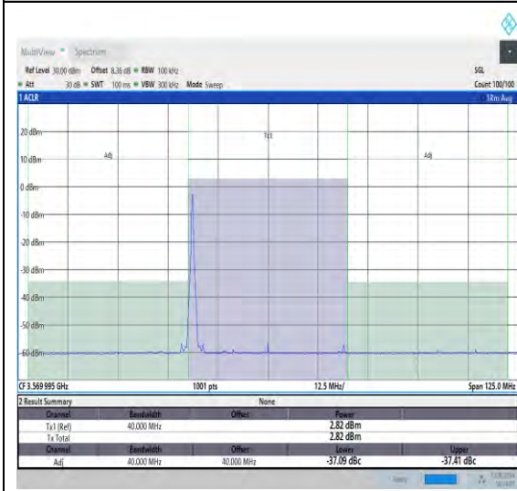
NTNV_N48_PC3_30_40_L_TID23_#1_-40_40
