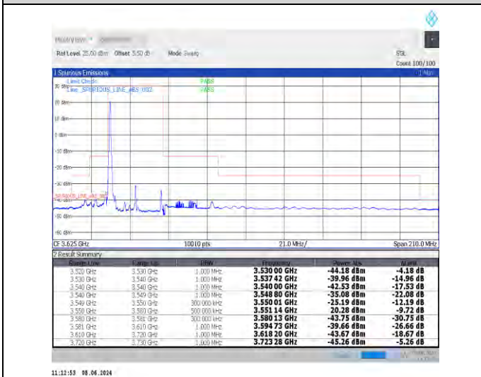
1-N48-30-30-L-4-CP-QPSK-Edge_1RB_Left-1@0-Ant0-1--PASS-see graph
