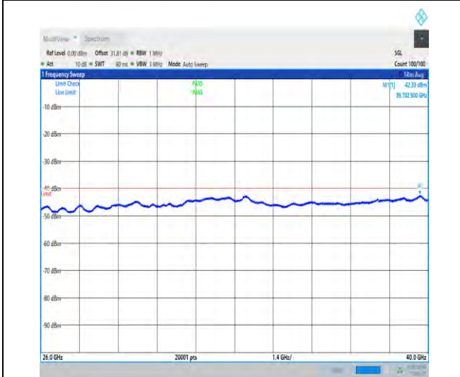
NTVN_N48_PC3_30_40_L_TID1_NS_01_26000_40000_#1
