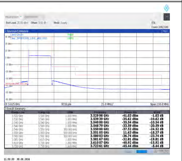
1-N48-30-30-L-6-CP-QPSK-Outer_Full-78@0-Ant0-1--PASS-see graph
