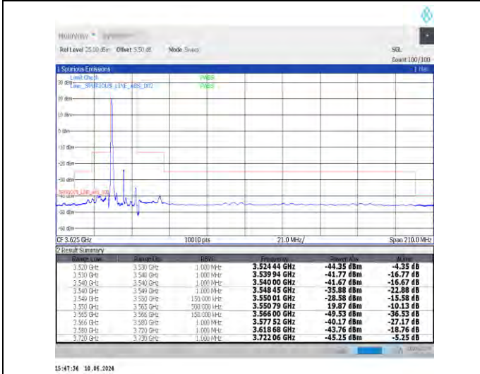
1-N48-30-15-L-4-CP-QPSK-Edge_1RB_Left-1@0-Ant0-1--PASS-see graph
