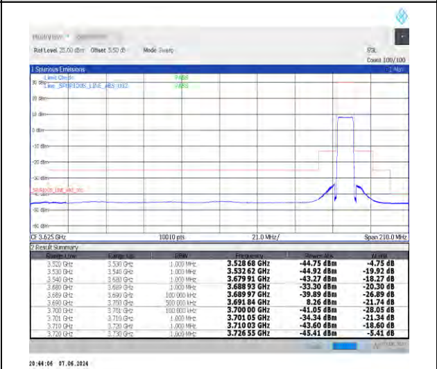
1-N48-30-10-H-6-CP-QPSK-Outer_Full-24@0-Ant0-1--PASS-see graph
