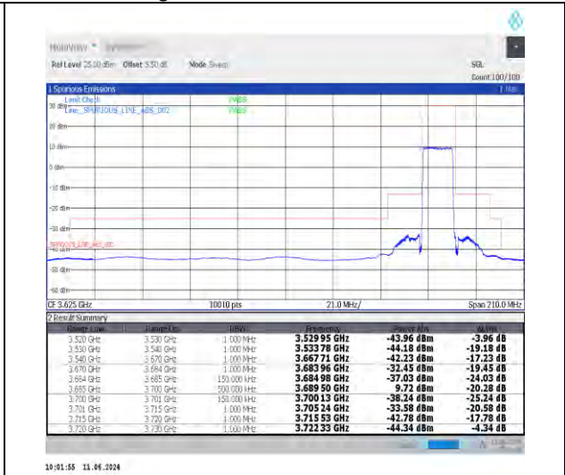
1-N48-30-15-H-3-DFT-PI2BPSK-Outer_Full-36@0-Ant0-1--PASS-see graph
