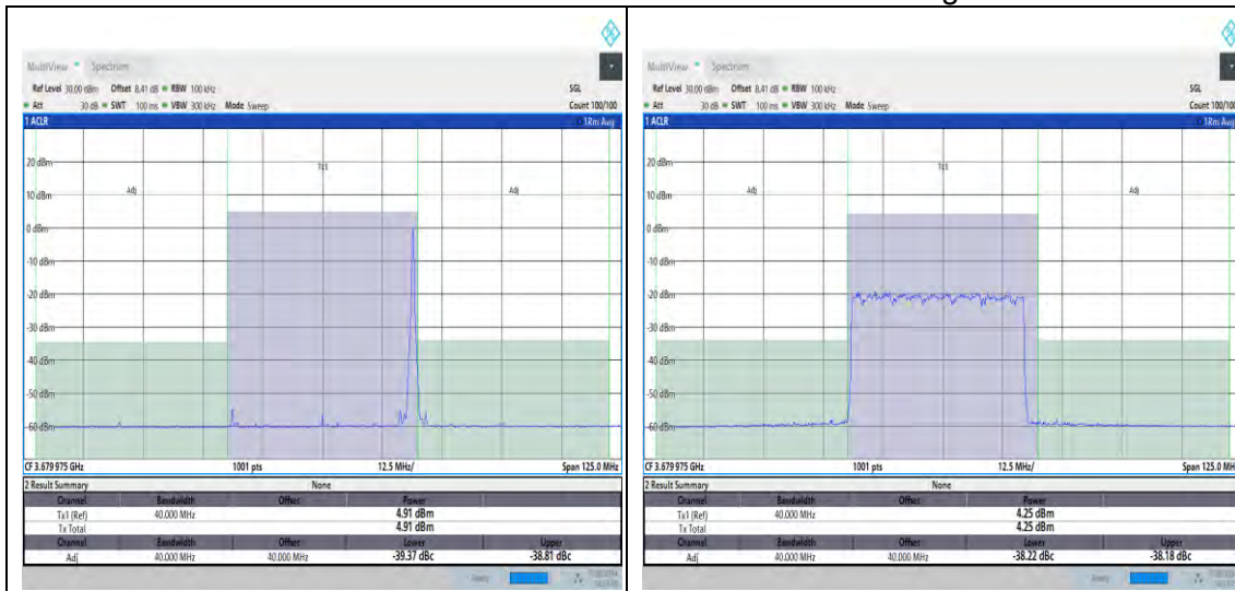
NTNV_N48_PC3_30_40_H_TID9_#1_-40_40
