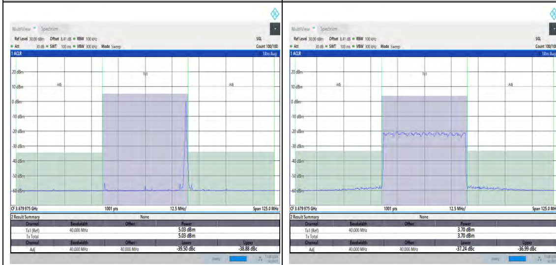
NTNV_N48_PC3_30_40_H_TID12_#1_-40_40
