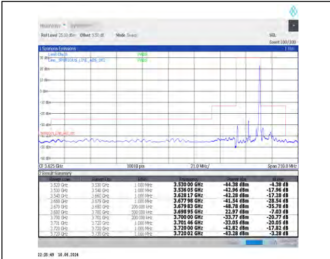
1-N48-30-20-H-2-DFT-PI2BPSK-Edge_1RB_Right-1@50-Ant0-1--PASS-see graph
