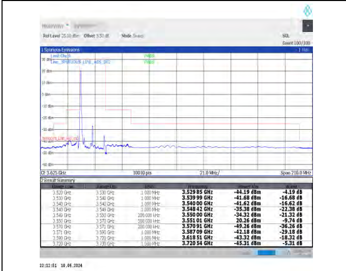
1-N48-30-20-L-4-CP-QPSK-Edge_1RB_Left-1@0-Ant0-1--PASS-see graph
