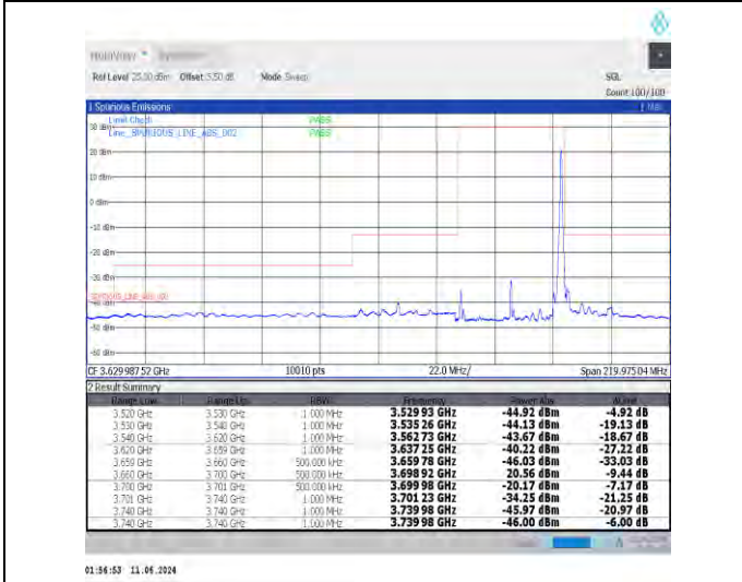
1-N48-30-40-H-5-CP-QPSK-Edge_1RB_Right-1@105-Ant0-1--PASS-see graph
