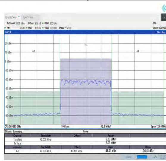
NTNV_N48_PC3_30_40_L_TID22_#1_-40_40
