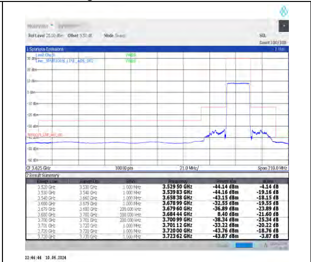
1-N48-30-20-H-3-DFT-PI2BPSK-Outer_Full-50@0-Ant0-1--PASS-see graph
