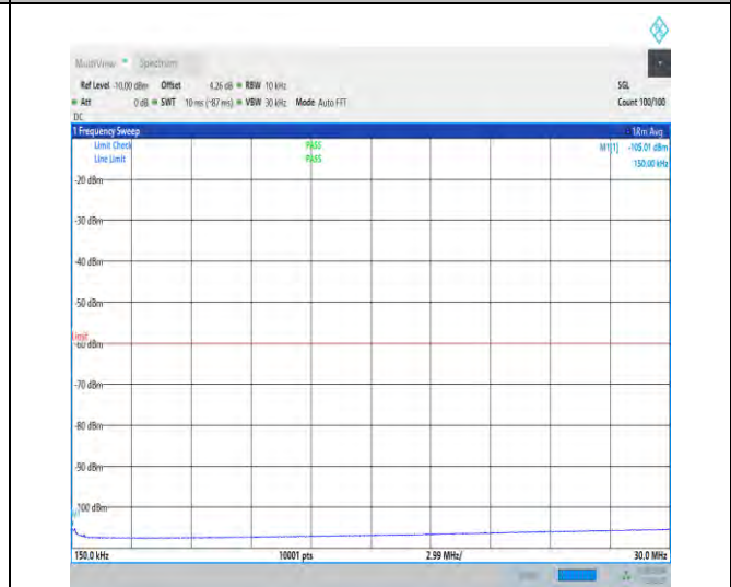
NTVN_N48_PC3_30_40_H_TID1_NS_01_0.15_30_#1
