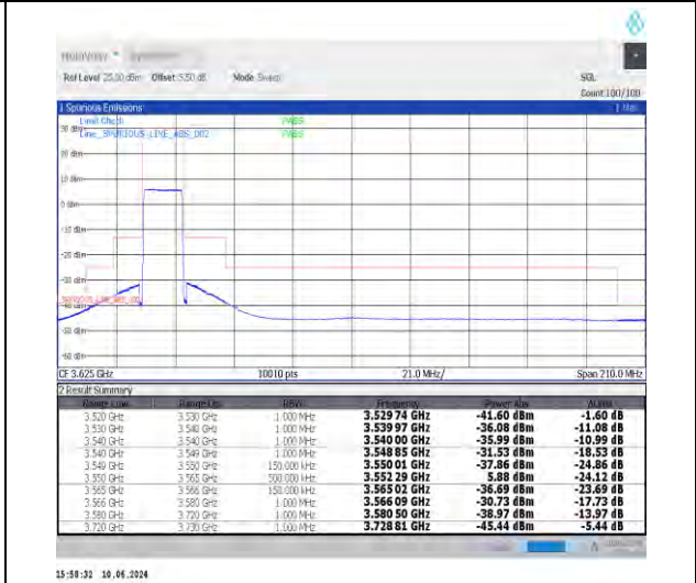
1-N48-30-15-L-6-CP-QPSK-Outer_Full-38@0-Ant0-1--PASS-see graph
