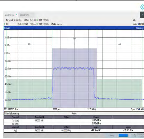
NTNV_N48_PC3_30_40_H_TID4_#1_+40_40
