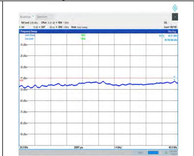
NTVN_N48_PC3_30_40_M_TID1_NS_01_26000_40000_#1
