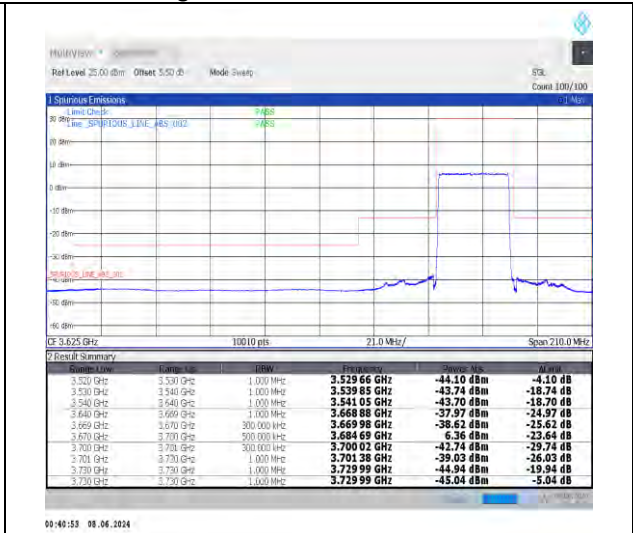
1-N48-30-30-H-3-DFT-PI2BPSK-Outer_Full-75@0-Ant0-1--PASS-see graph
