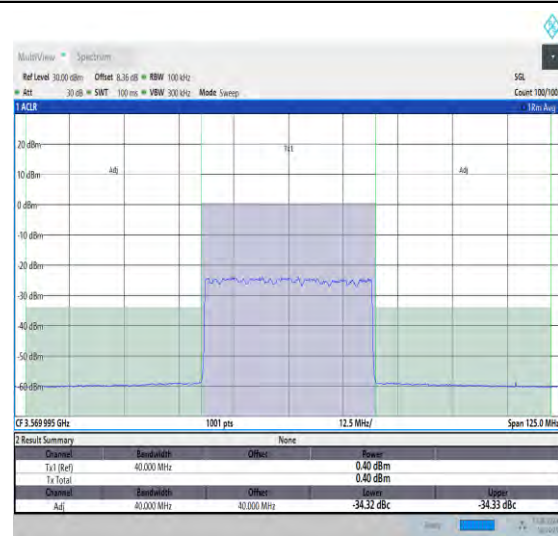
NTNV_N48_PC3_30_40_L_TID25_#1_-40_40
