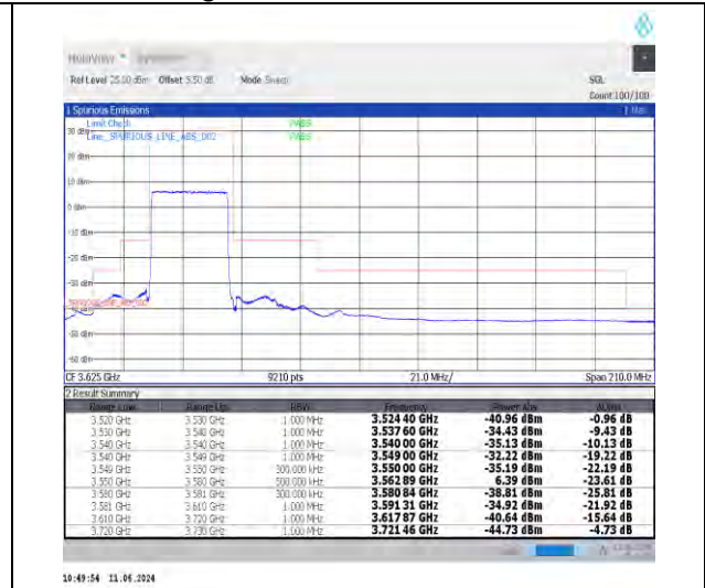
1-N48-30-30-L-3-DFT-PI2BPSK-Outer_Full-75@0-Ant0-1--PASS-see graph
