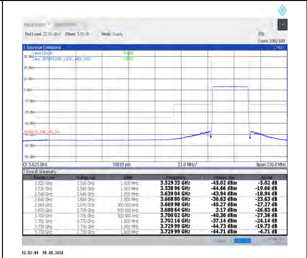
1-N48-30-30-H-6-CP-QPSK-Outer_Full-78@0-Ant0-1--PASS-see graph
