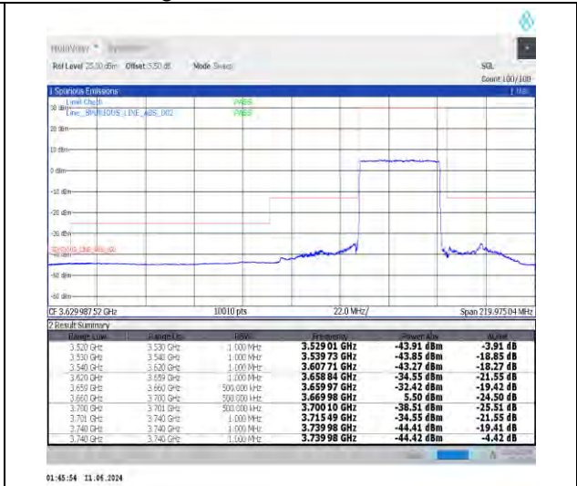
1-N48-30-40-H-3-DFT-PI2BPSK-Outer_Full-100@0-Ant0-1--PASS-see graph
