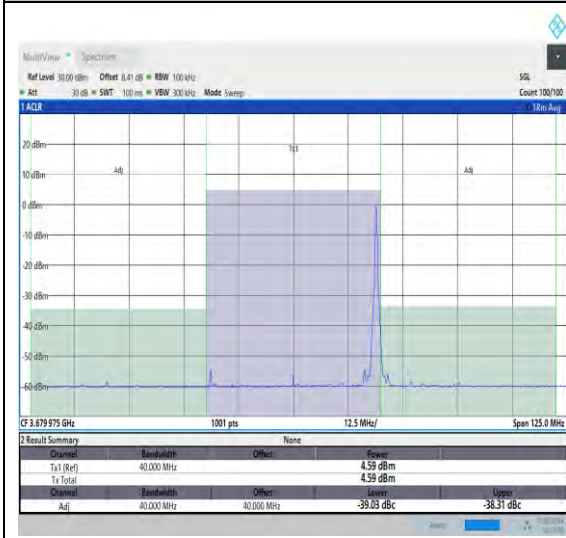
NTNV_N48_PC3_30_40_H_TID6_#1_-40_40
