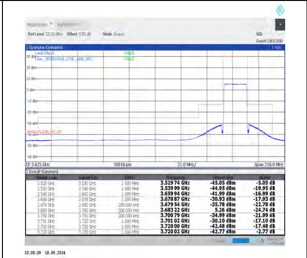
1-N48-30-20-H-6-CP-QPSK-Outer_Full-51@0-Ant0-1--PASS-see graph
