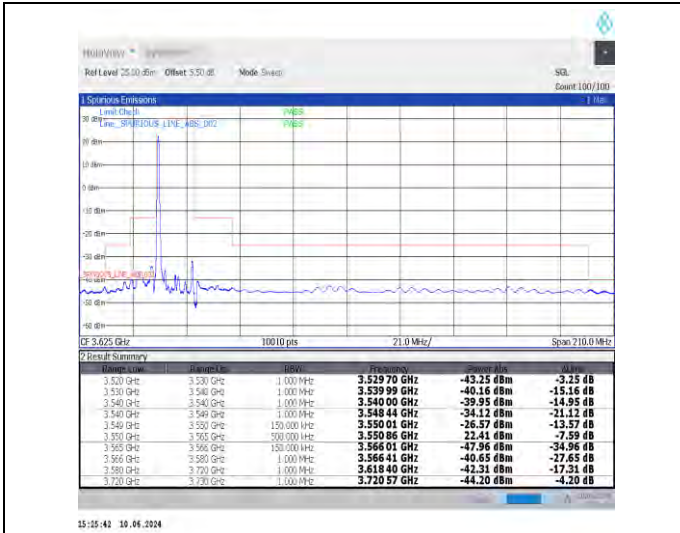
1-N48-30-15-L-1-DFT-PI2BPSK-Edge_1RB_Left-1@0-Ant0-1--PASS-see graph
