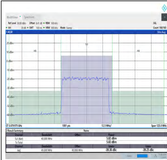
NTNV_N48_PC3_30_40_H_TID4_#1_-40_40
