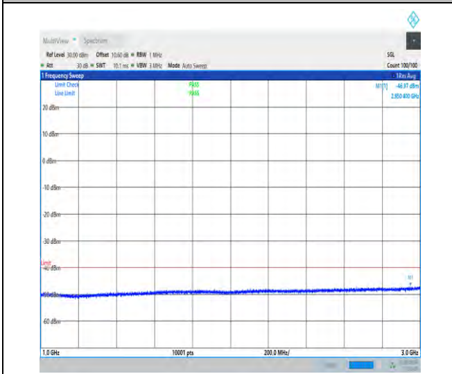
NTNV_N48_PC3_30_40_M_TID1_NS_01_1000_3000_#1
