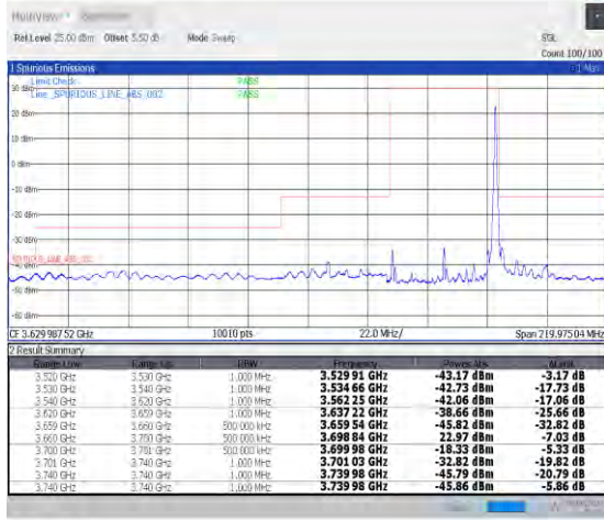
1-N48-30-40-H-2-DFT-PI2BPSK-Edge_1RB_Right-1@105-Ant0-1--PASS-see graph
