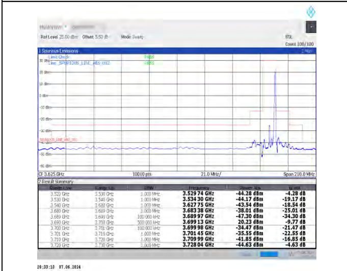
1-N48-30-10-H-5-CP-QPSK-Edge_1RB_Right-1@23-Ant0-1--PASS-see graph
