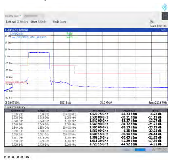
1-N48-30-30-L-3-DFT-PI2BPSK-Outer_Full-75@0-Ant0-1--PASS-see graph
