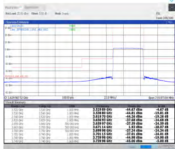
1-N48-30-40-H-6-CP-QPSK-Outer_Full-106@0-Ant0-1--PASS-see graph
