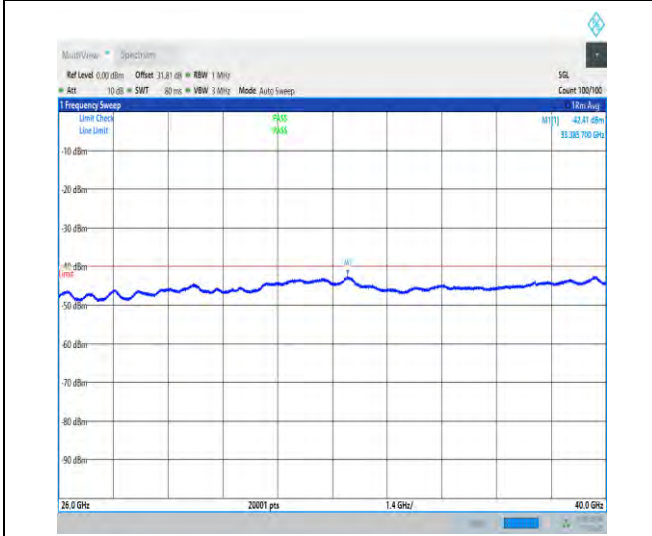
NTVN_N48_PC3_30_40_L_TID1_NS_01_26000_40000_#1
