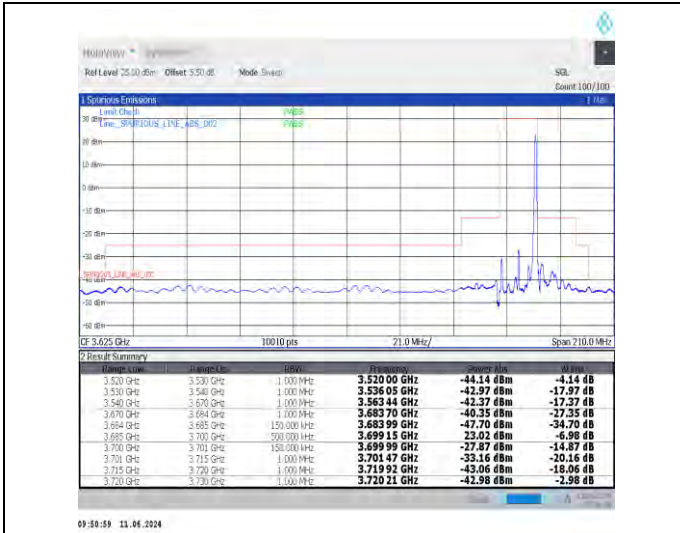
1-N48-30-15-H-2-DFT-PI2BPSK-Edge_1RB_Right-1@37-Ant0-1--PASS-see graph
