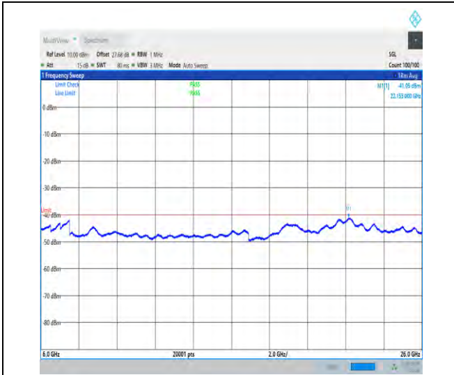
NTVN_N48_PC3_30_40_M_TID1_NS_01_6000_26000_#1
