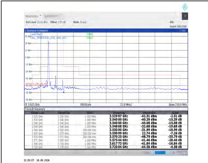
1-N48-30-20-L-1-DFT-PI2BPSK-Edge_1RB_Left-1@0-Ant0-1--PASS-see graph
